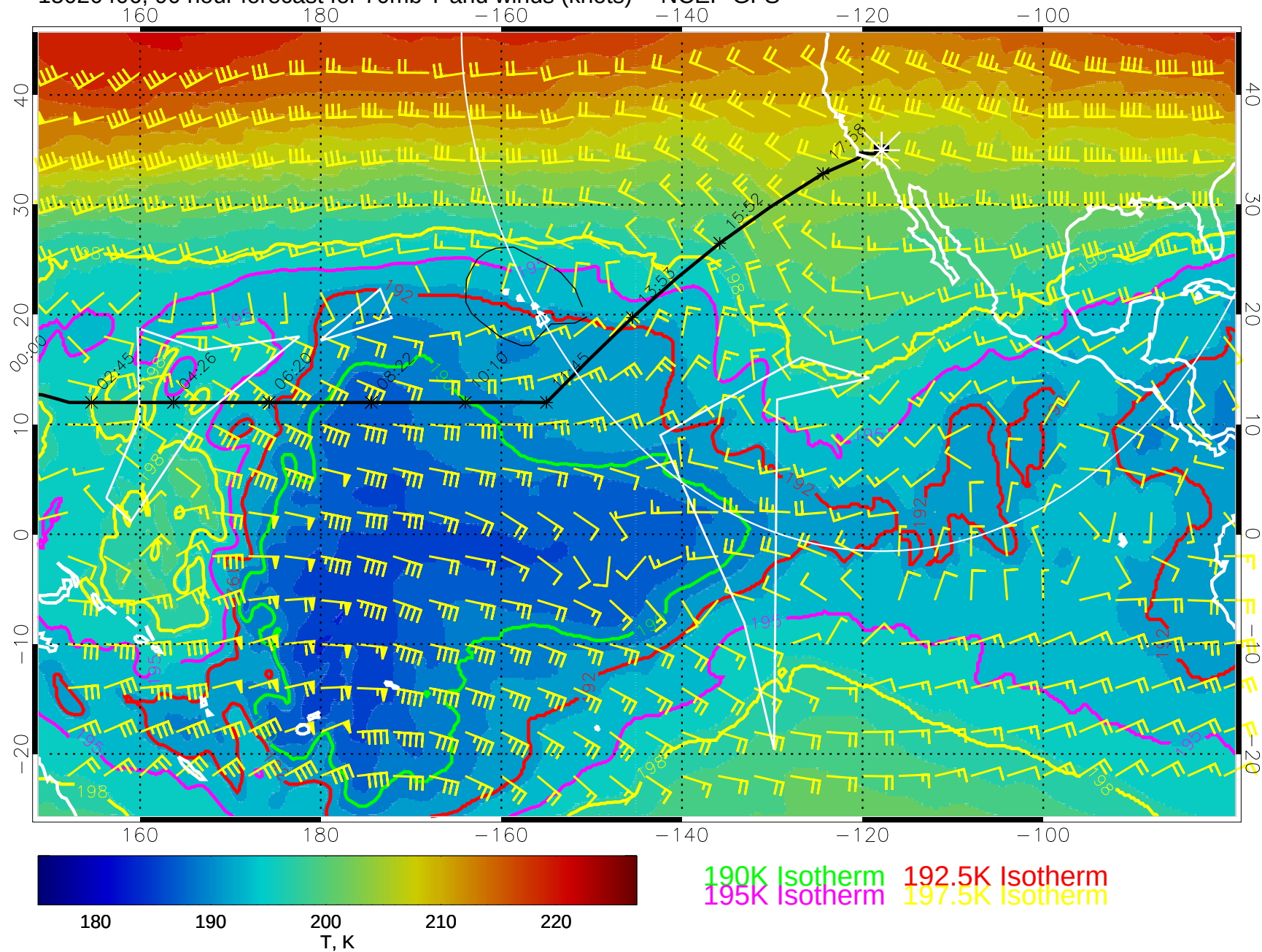
15020406, 90 hour forecast for 70mb T and winds (knots) -- NCEP GFS
