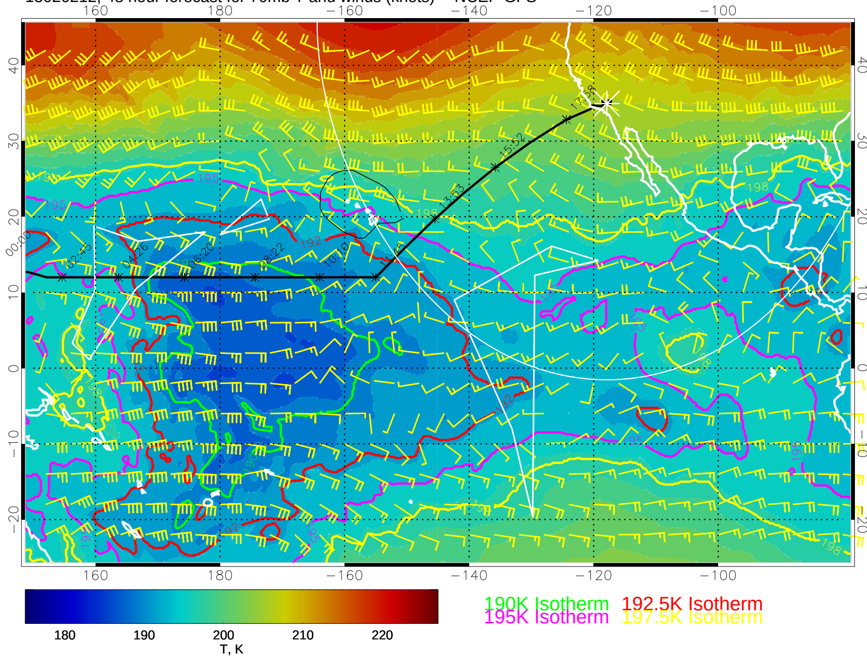
15020212, 48 hour forecast for 70mb T and winds (knots) -- NCEP GFS
