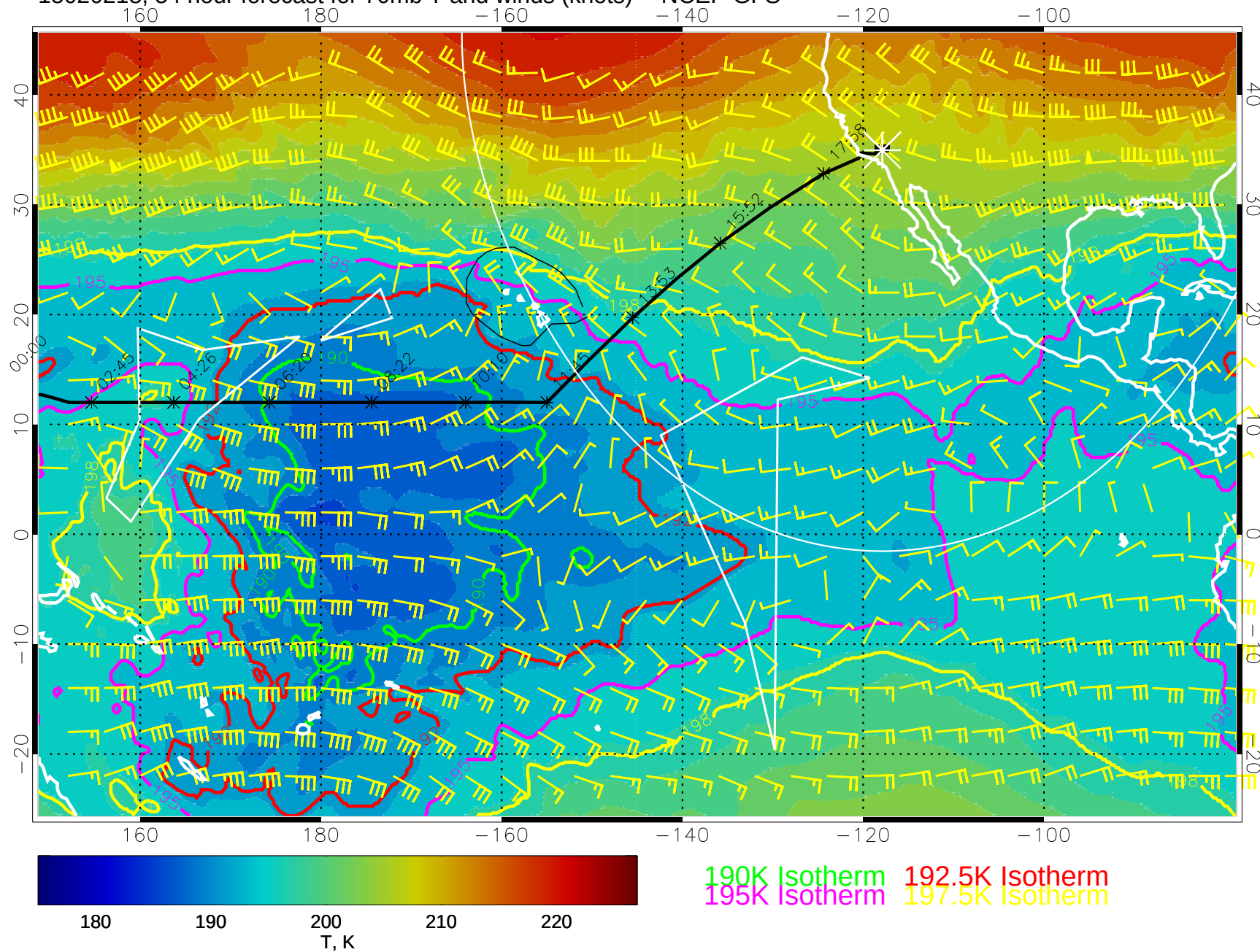
15020218, 54 hour forecast for 70mb T and winds (knots) -- NCEP GFS
