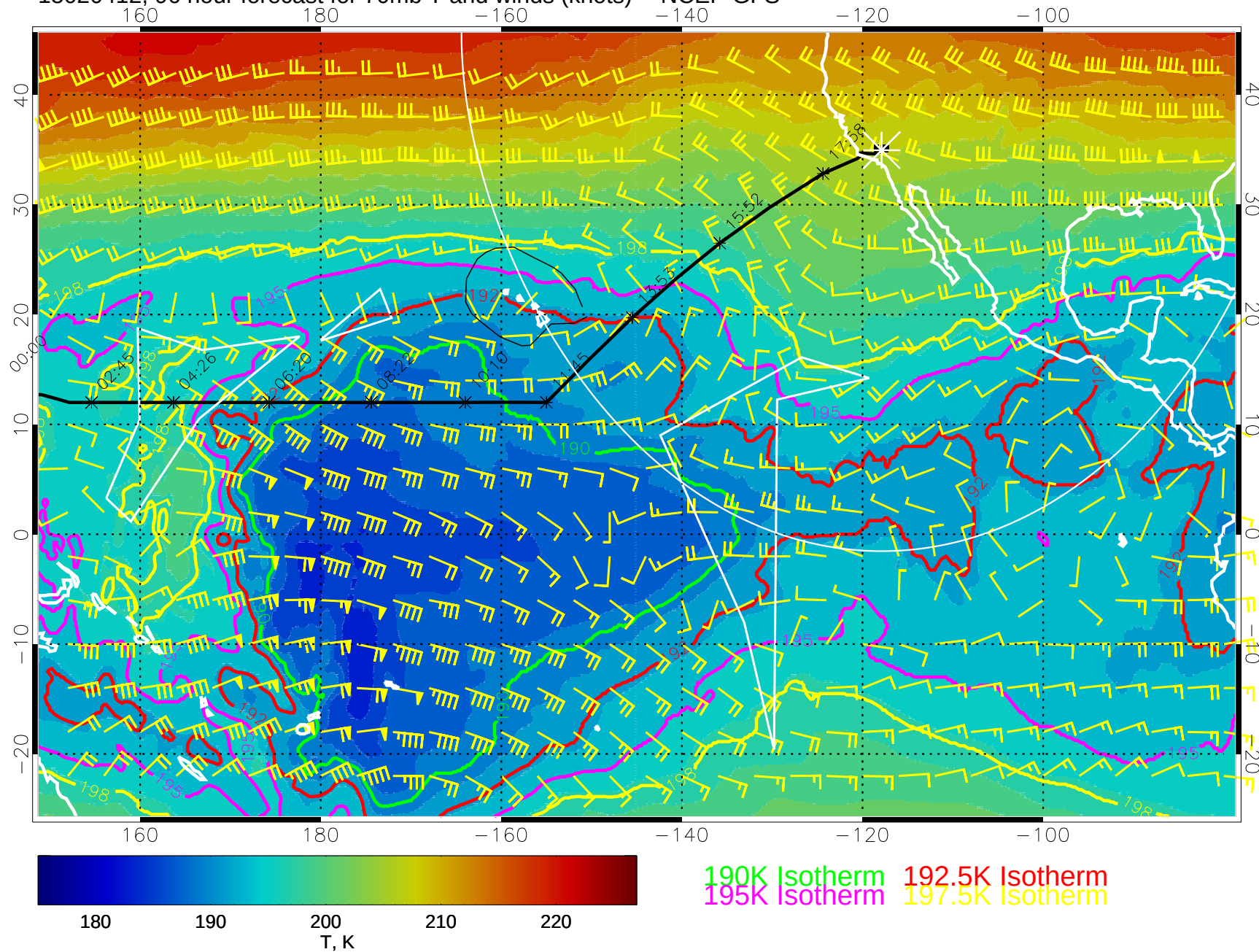
15020412, 96 hour forecast for 70mb T and winds (knots) -- NCEP GFS
