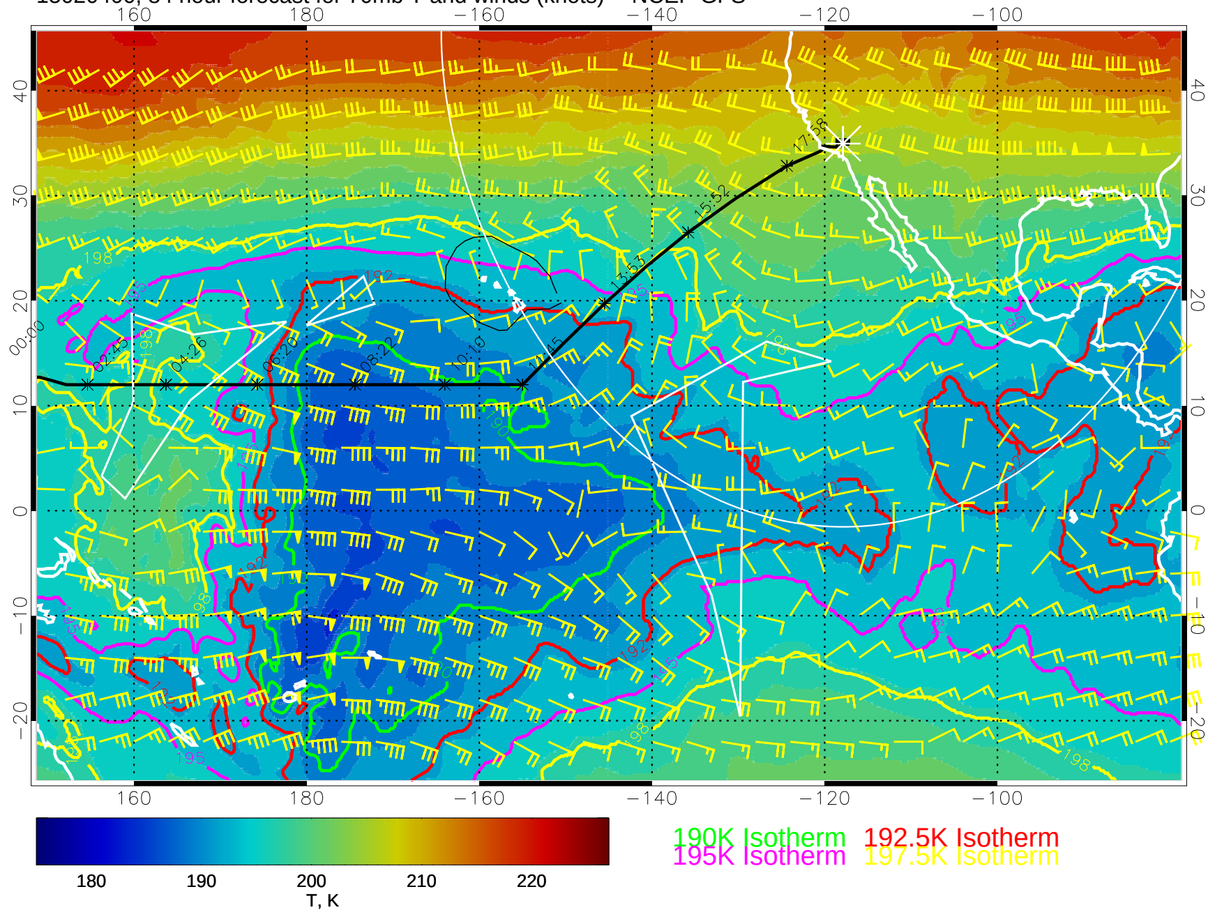
15020400, 84 hour forecast for 70mb T and winds (knots) -- NCEP GFS
