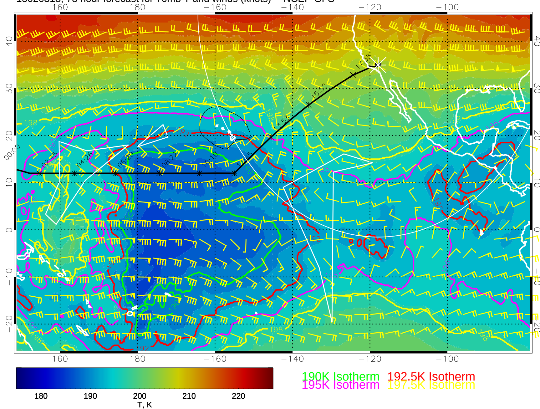
15020318, 78 hour forecast for 70mb T and winds (knots) -- NCEP GFS
