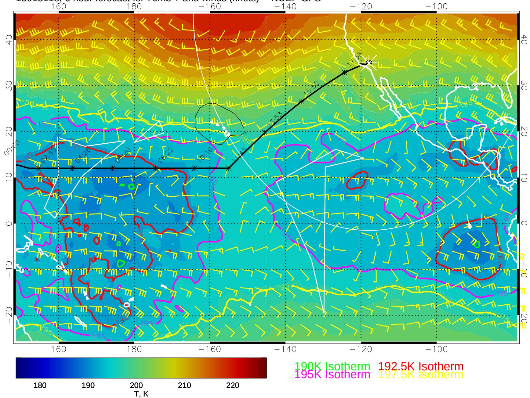
15013118, 6 hour forecast for 70mb T and winds (knots) -- NCEP GFS
