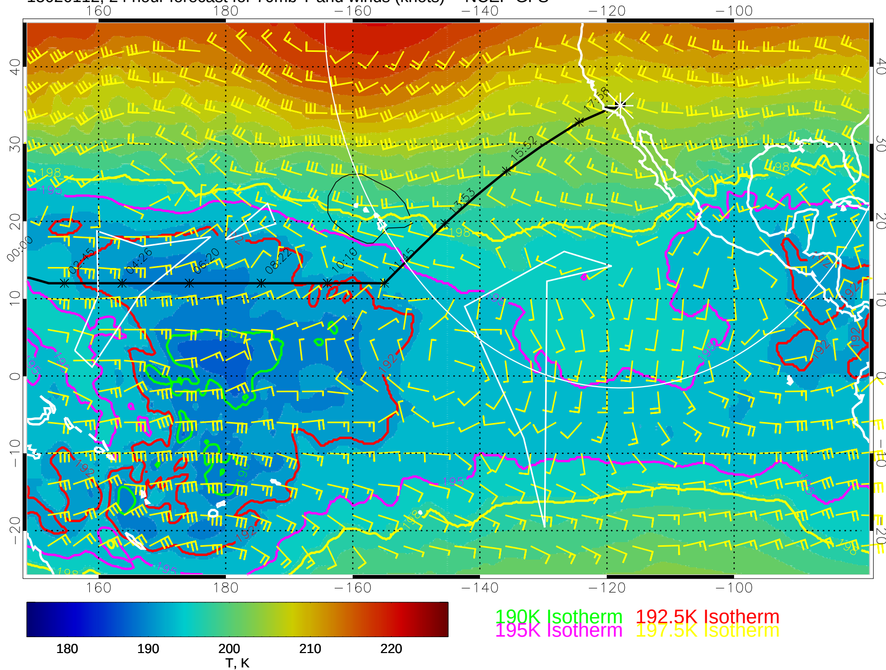
15020112, 24 hour forecast for 70mb T and winds (knots) -- NCEP GFS
