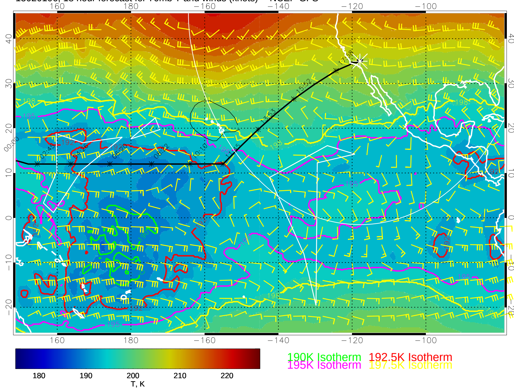
15020106, 18 hour forecast for 70mb T and winds (knots) -- NCEP GFS
