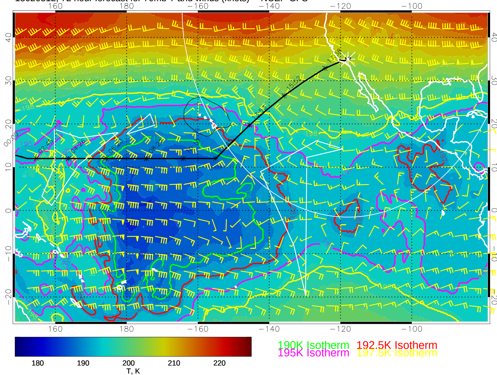
15020312, 72 hour forecast for 70mb T and winds (knots) -- NCEP GFS
