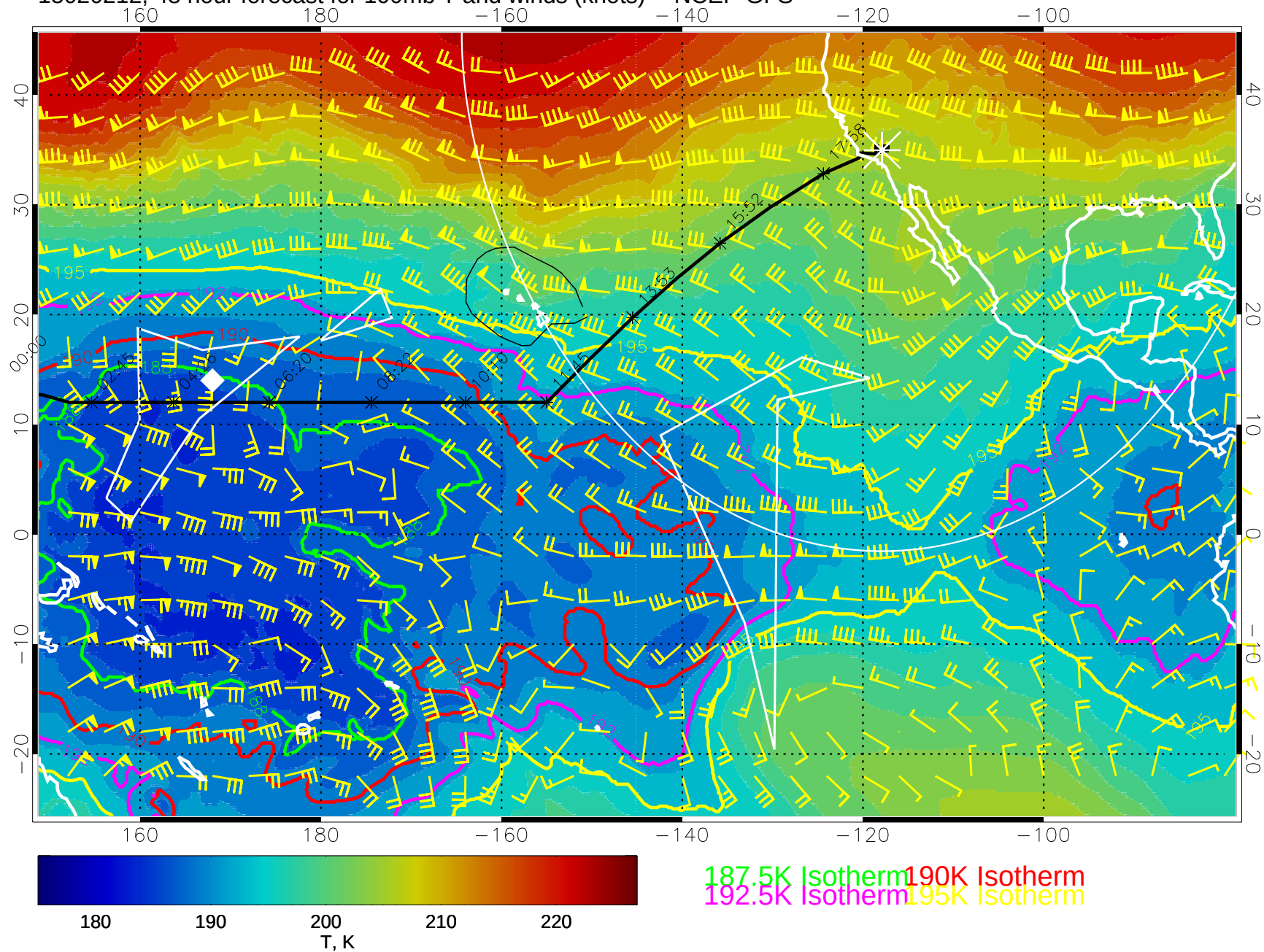
15020212, 48 hour forecast for 100mb T and winds (knots) -- NCEP GFS
