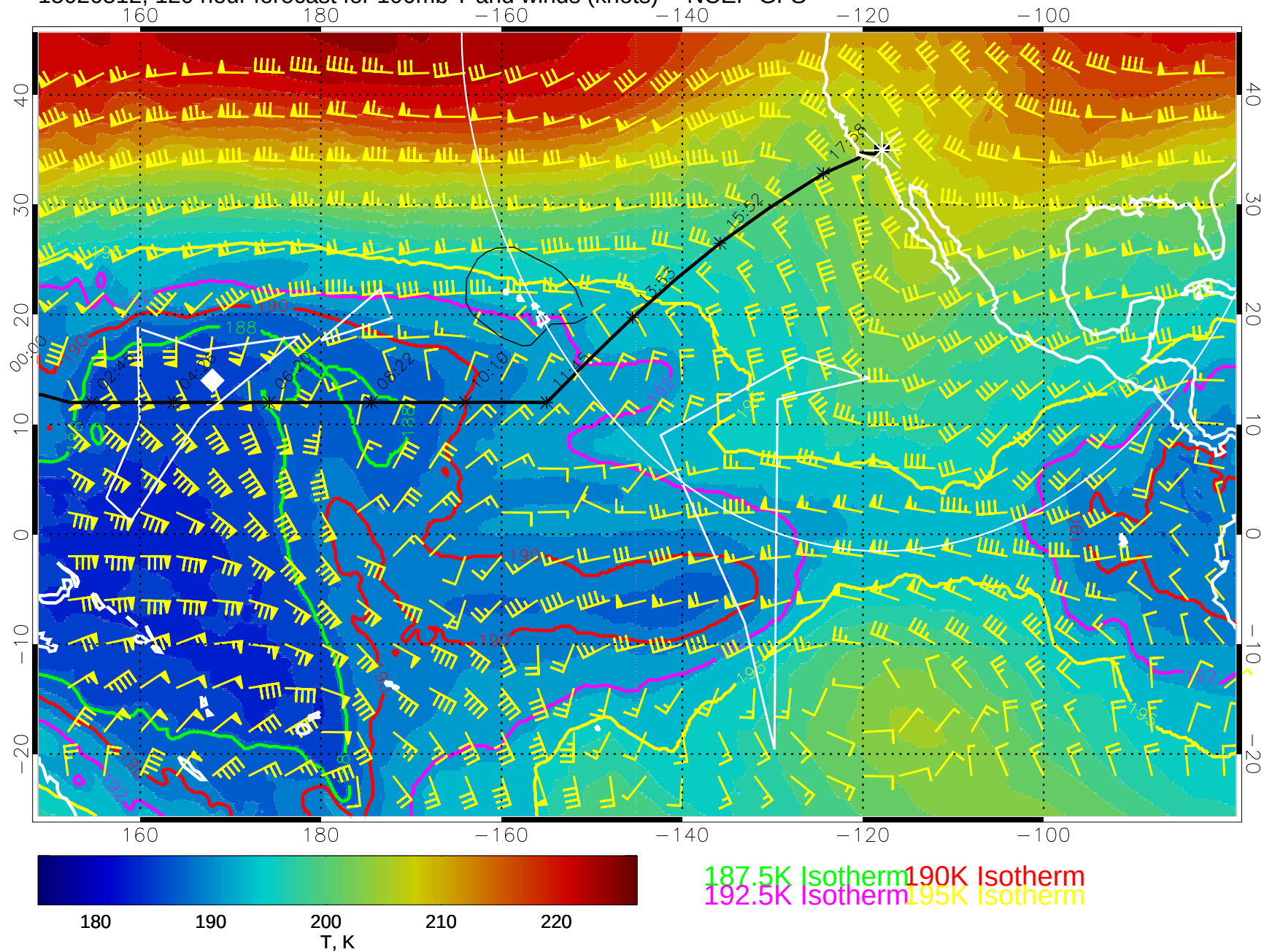
15020512, 120 hour forecast for 100mb T and winds (knots) -- NCEP GFS
