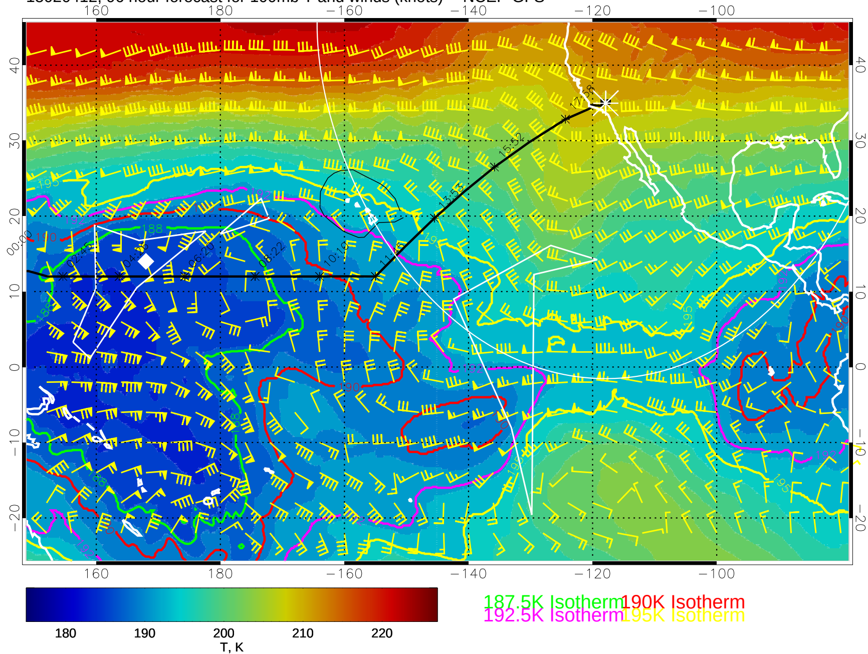
15020412, 96 hour forecast for 100mb T and winds (knots) -- NCEP GFS
