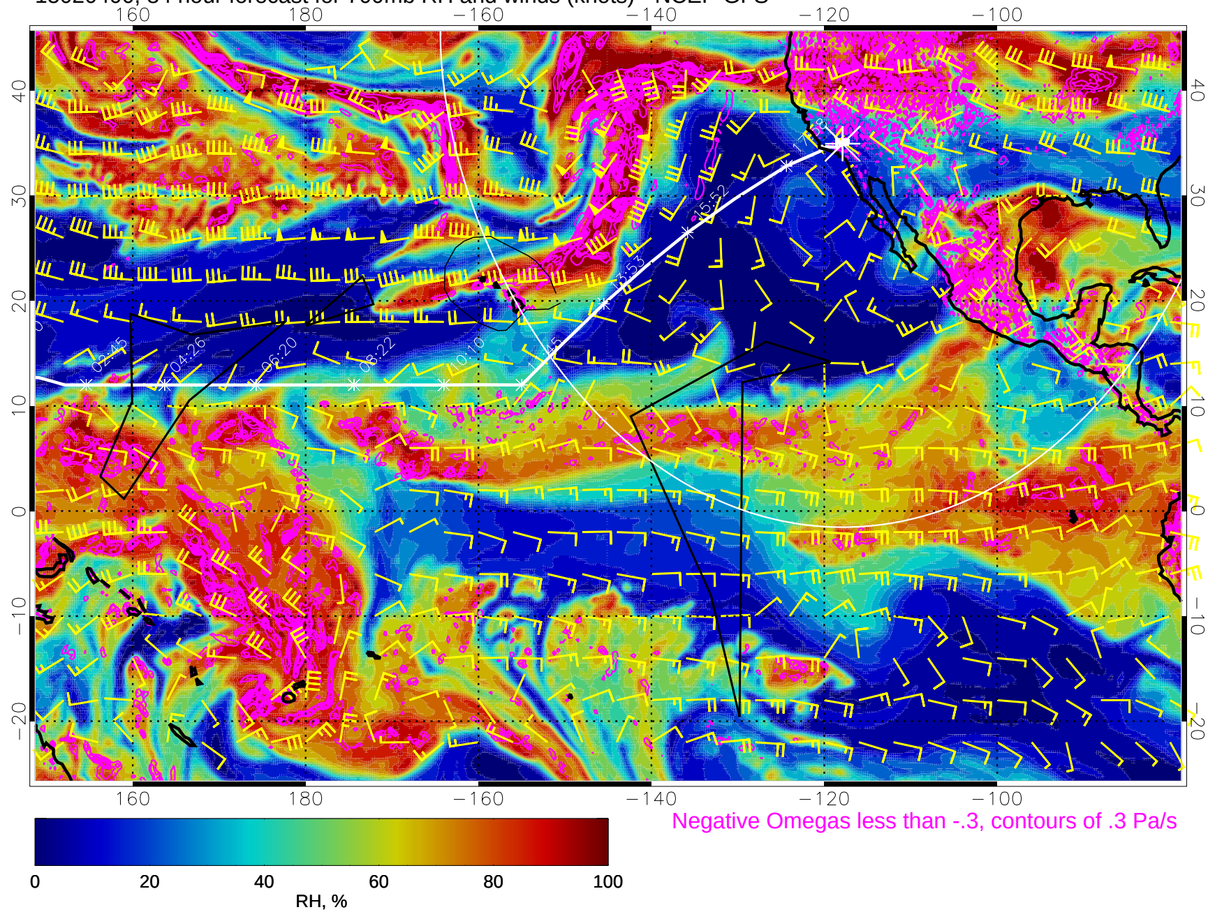
15020400, 84 hour forecast for 700mb RH and winds (knots) - NCEP GFS
