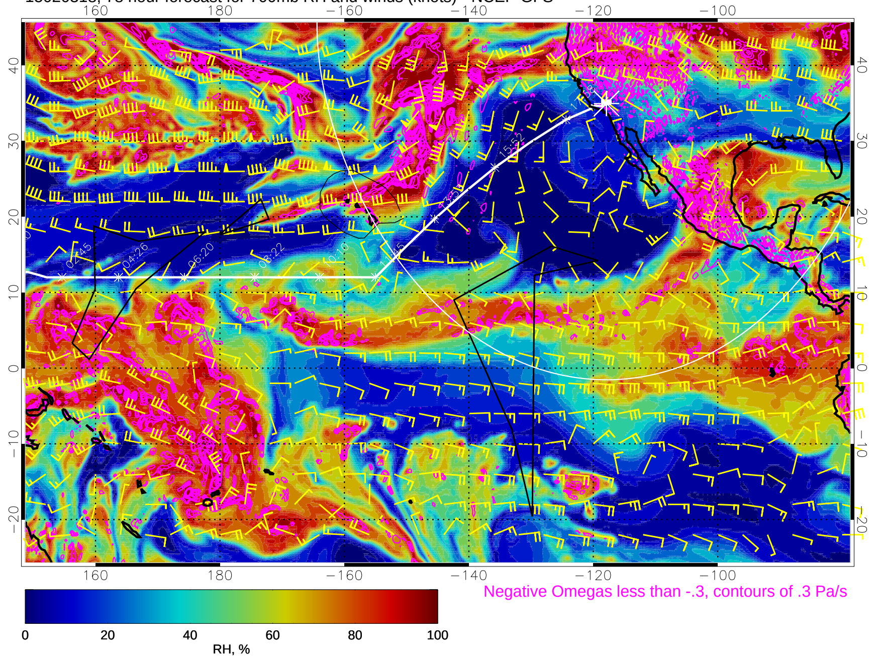
15020318, 78 hour forecast for 700mb RH and winds (knots) - NCEP GFS
