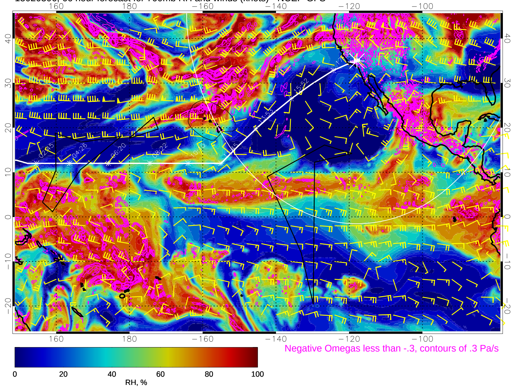
15020306, 66 hour forecast for 700mb RH and winds (knots) - NCEP GFS
