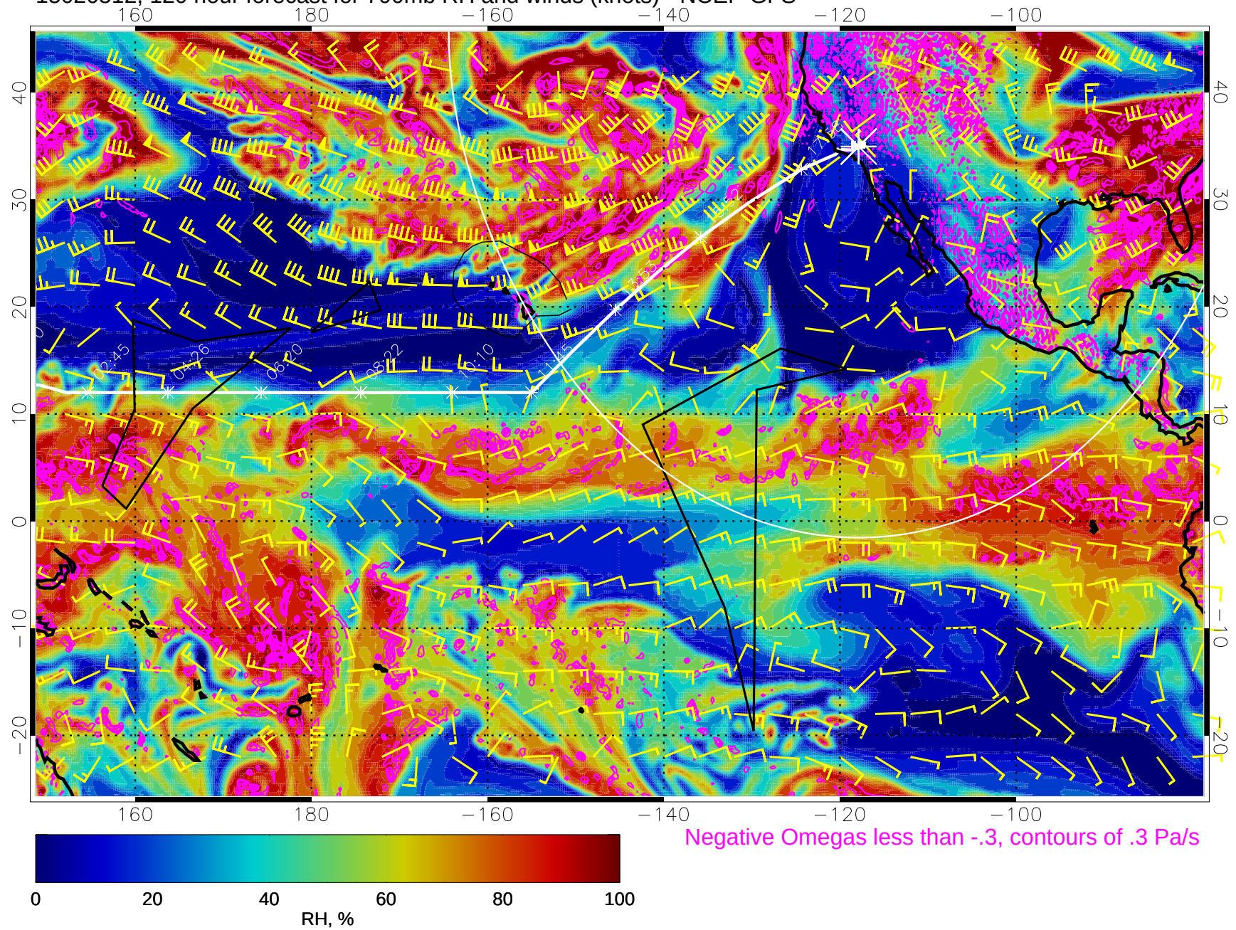
15020512, 120 hour forecast for 700mb RH and winds (knots) - NCEP GFS
