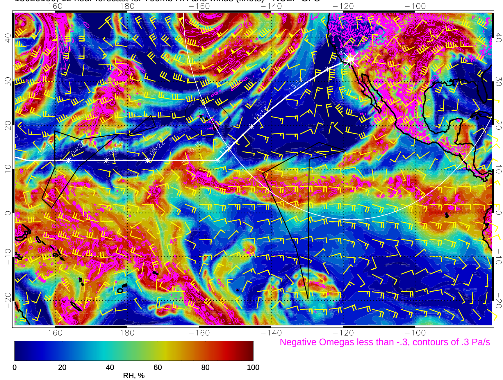
15020100, 12 hour forecast for 700mb RH and winds (knots) - NCEP GFS
