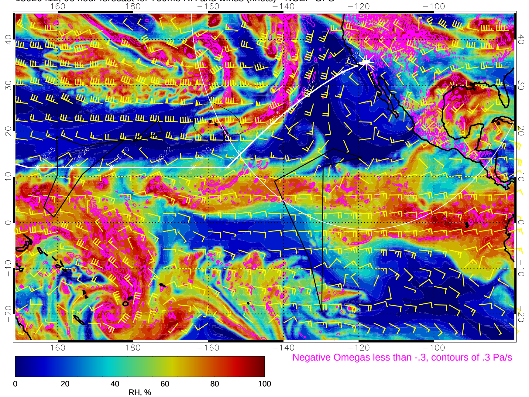
15020412, 96 hour forecast for 700mb RH and winds (knots) - NCEP GFS
