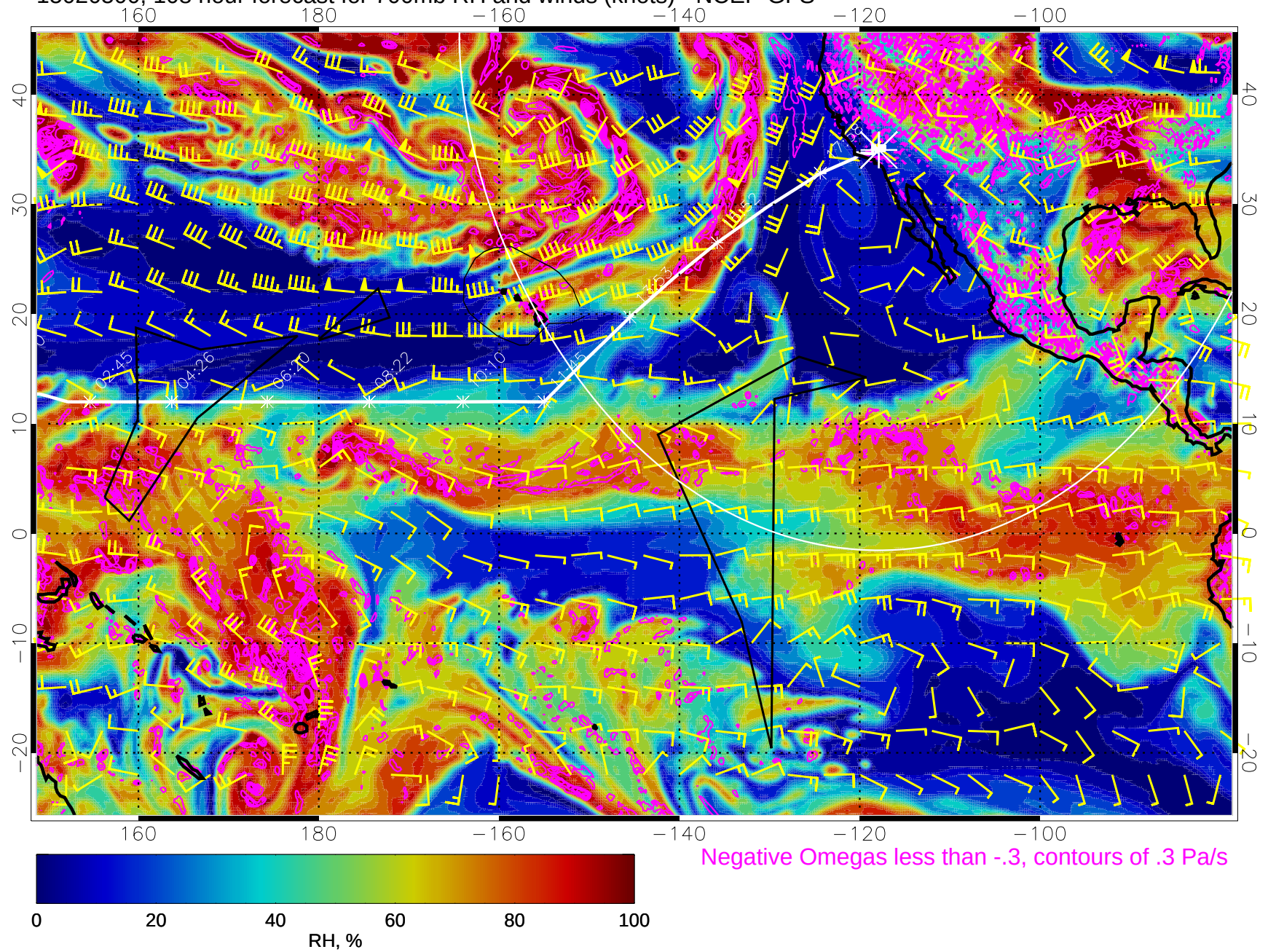
15020500, 108 hour forecast for 700mb RH and winds (knots) - NCEP GFS
