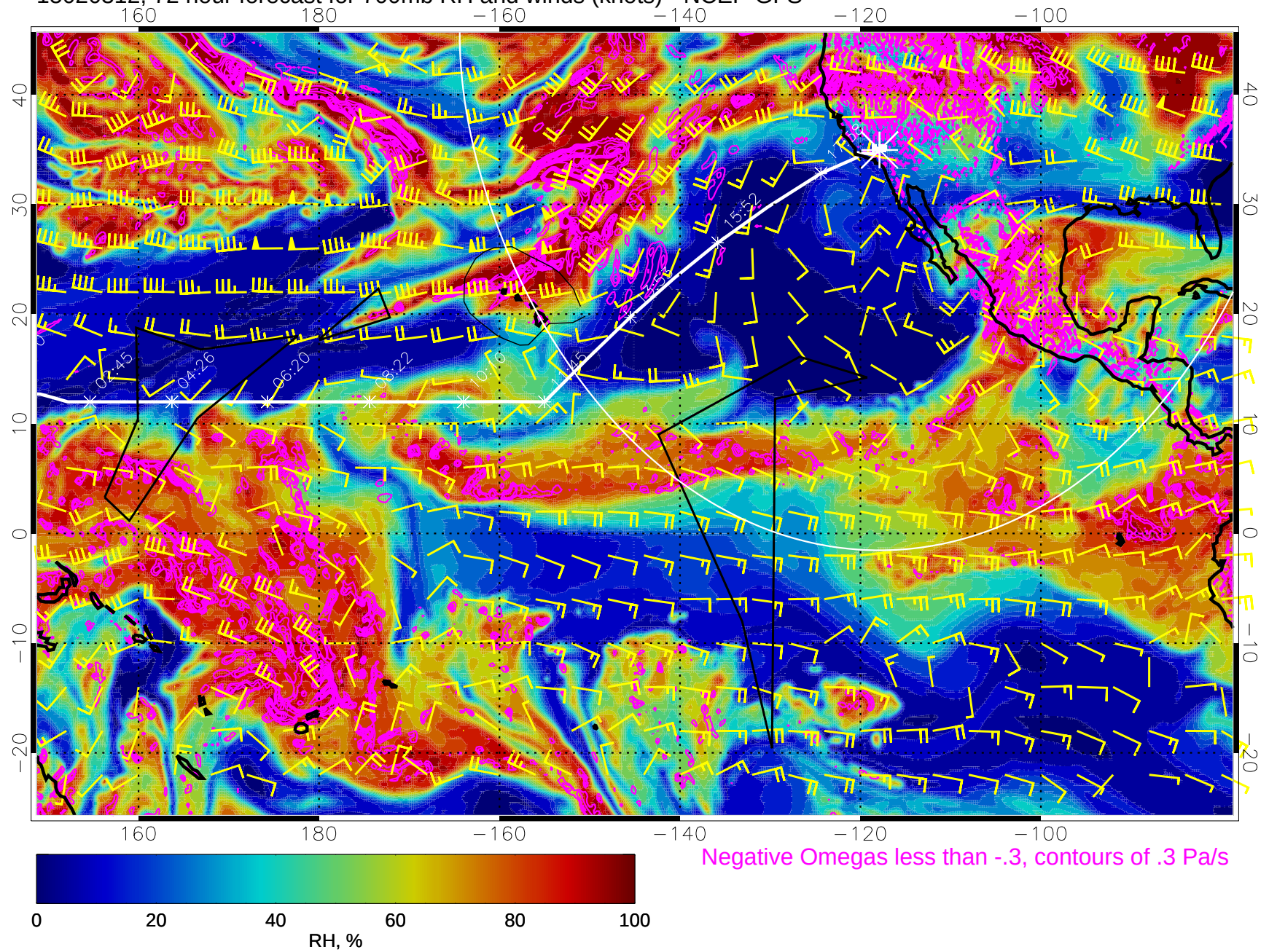
15020312, 72 hour forecast for 700mb RH and winds (knots) - NCEP GFS
