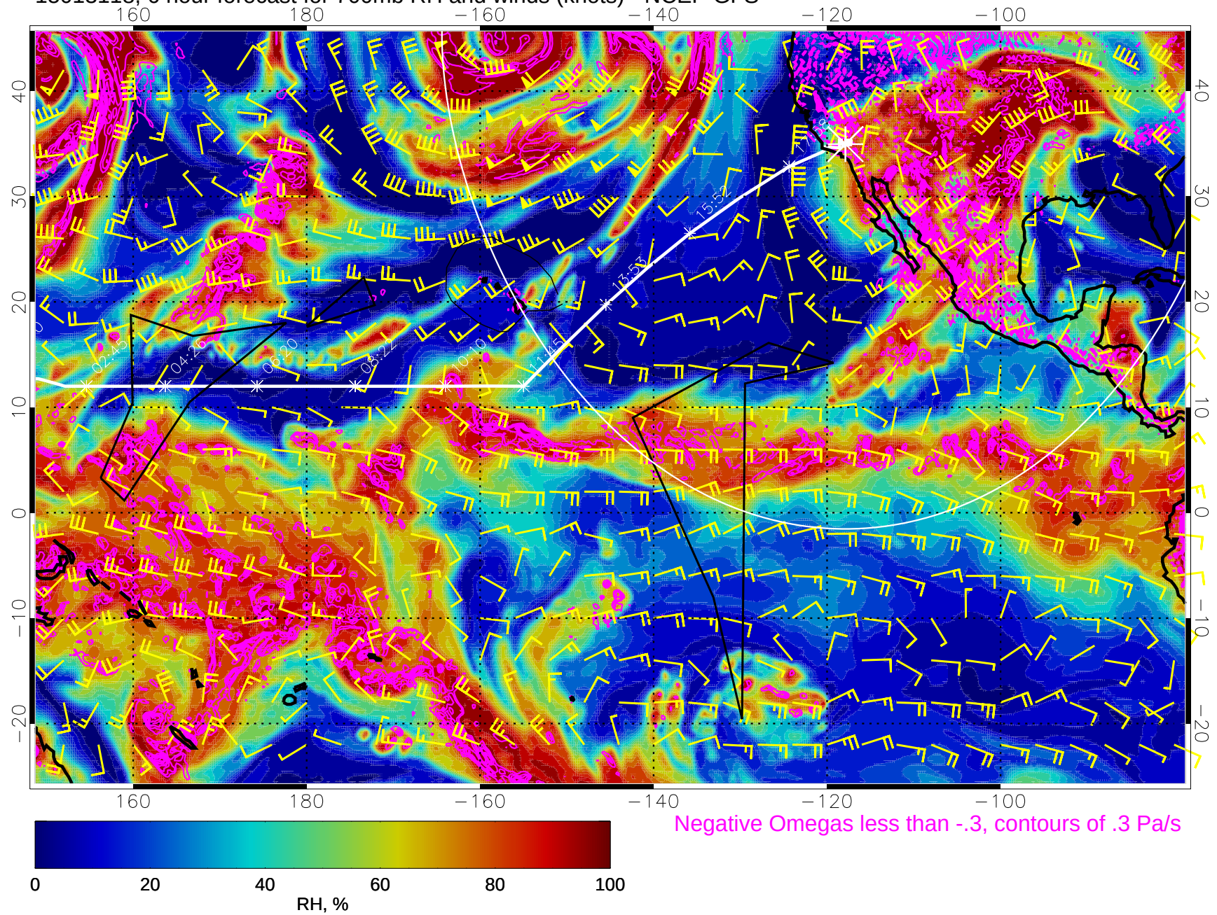
15013118, 6 hour forecast for 700mb RH and winds (knots) - NCEP GFS
