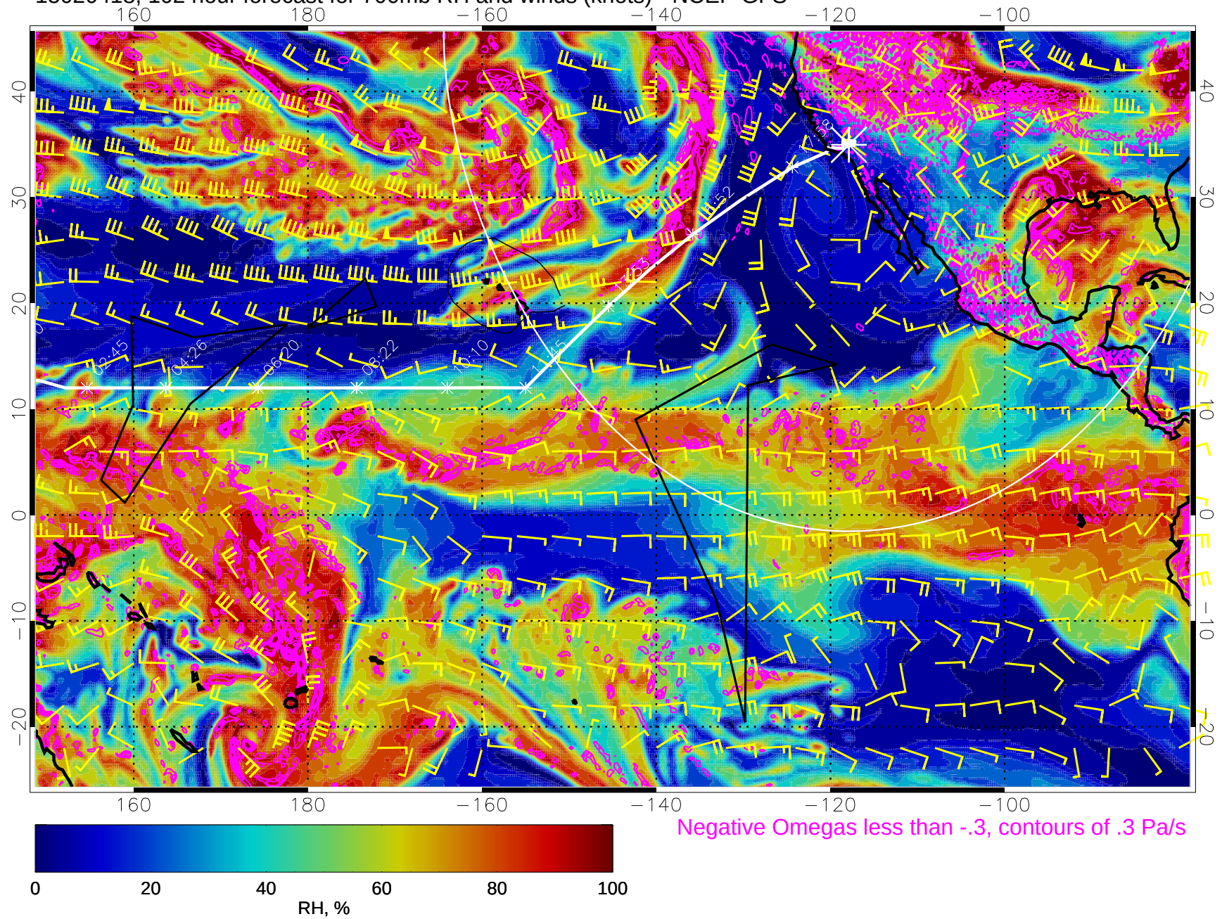
15020418, 102 hour forecast for 700mb RH and winds (knots) - NCEP GFS
