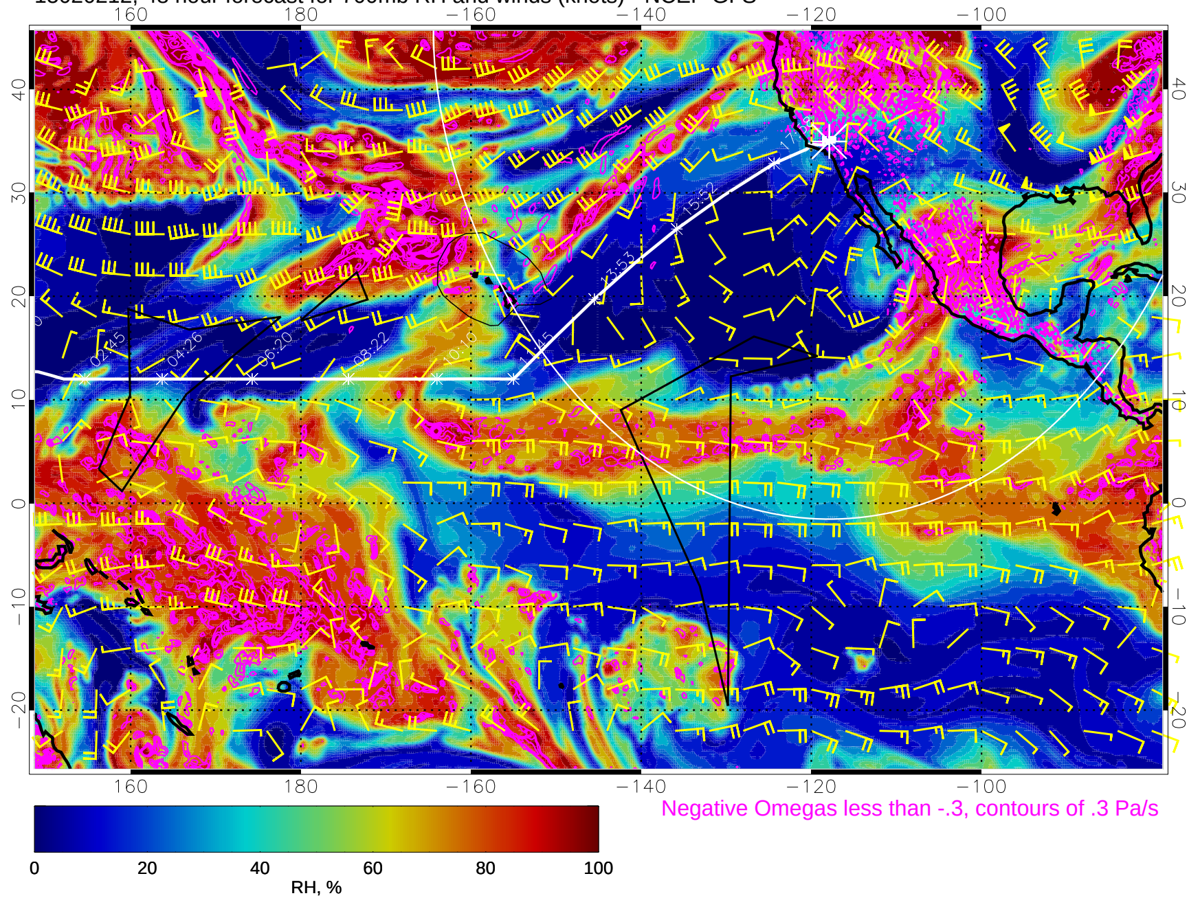
15020212, 48 hour forecast for 700mb RH and winds (knots) - NCEP GFS
