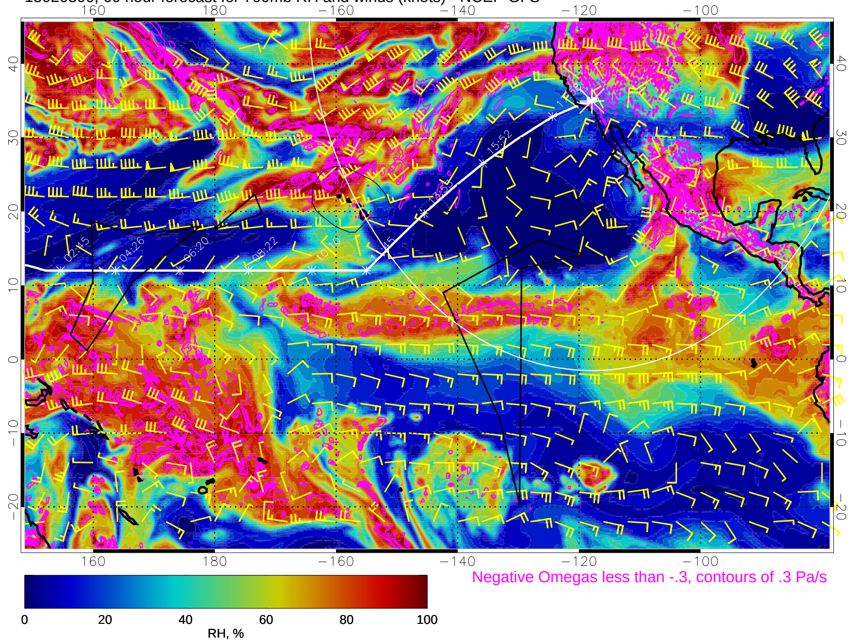
15020300, 60 hour forecast for 700mb RH and winds (knots) - NCEP GFS
