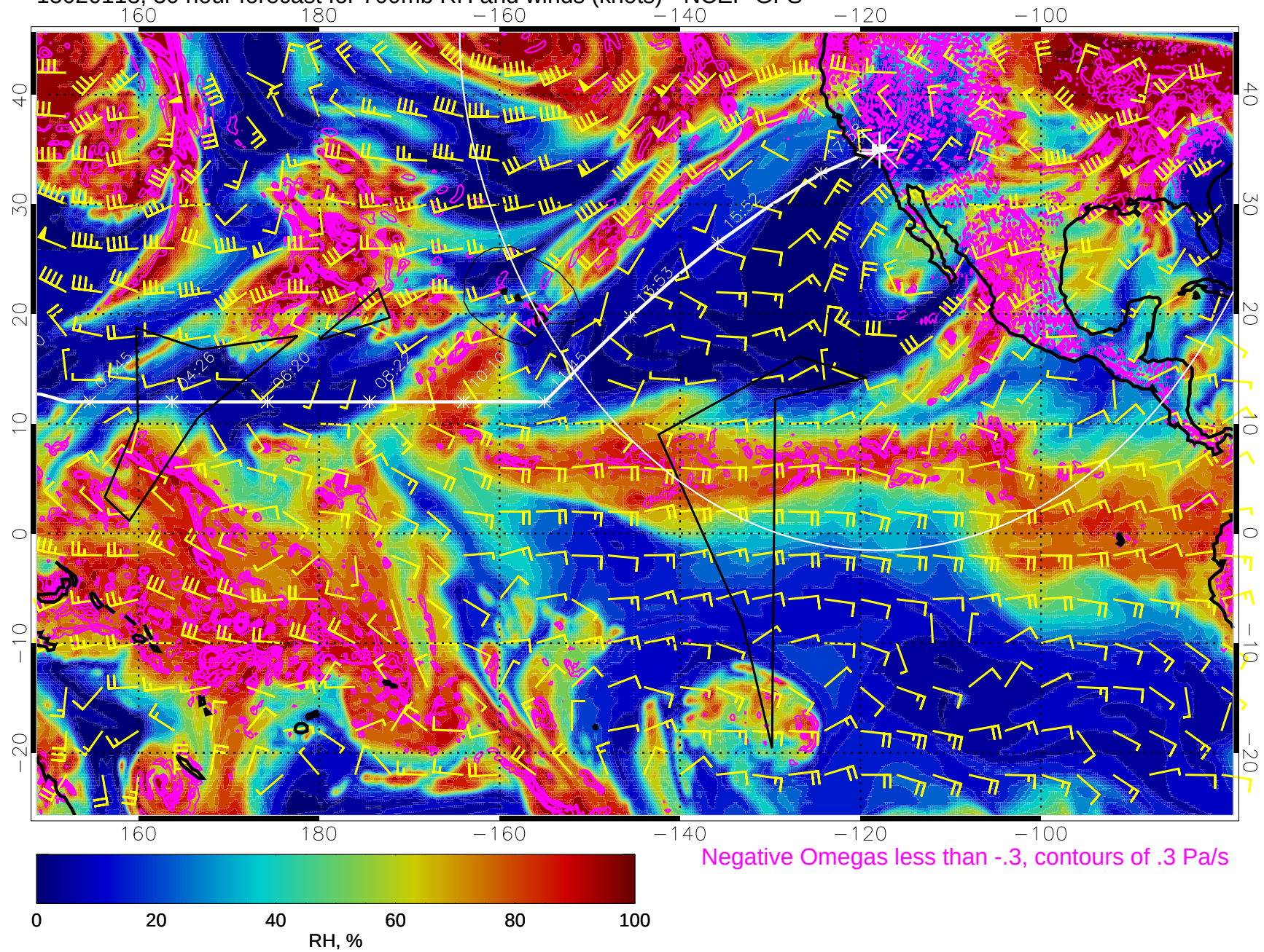
15020118, 30 hour forecast for 700mb RH and winds (knots) - NCEP GFS
