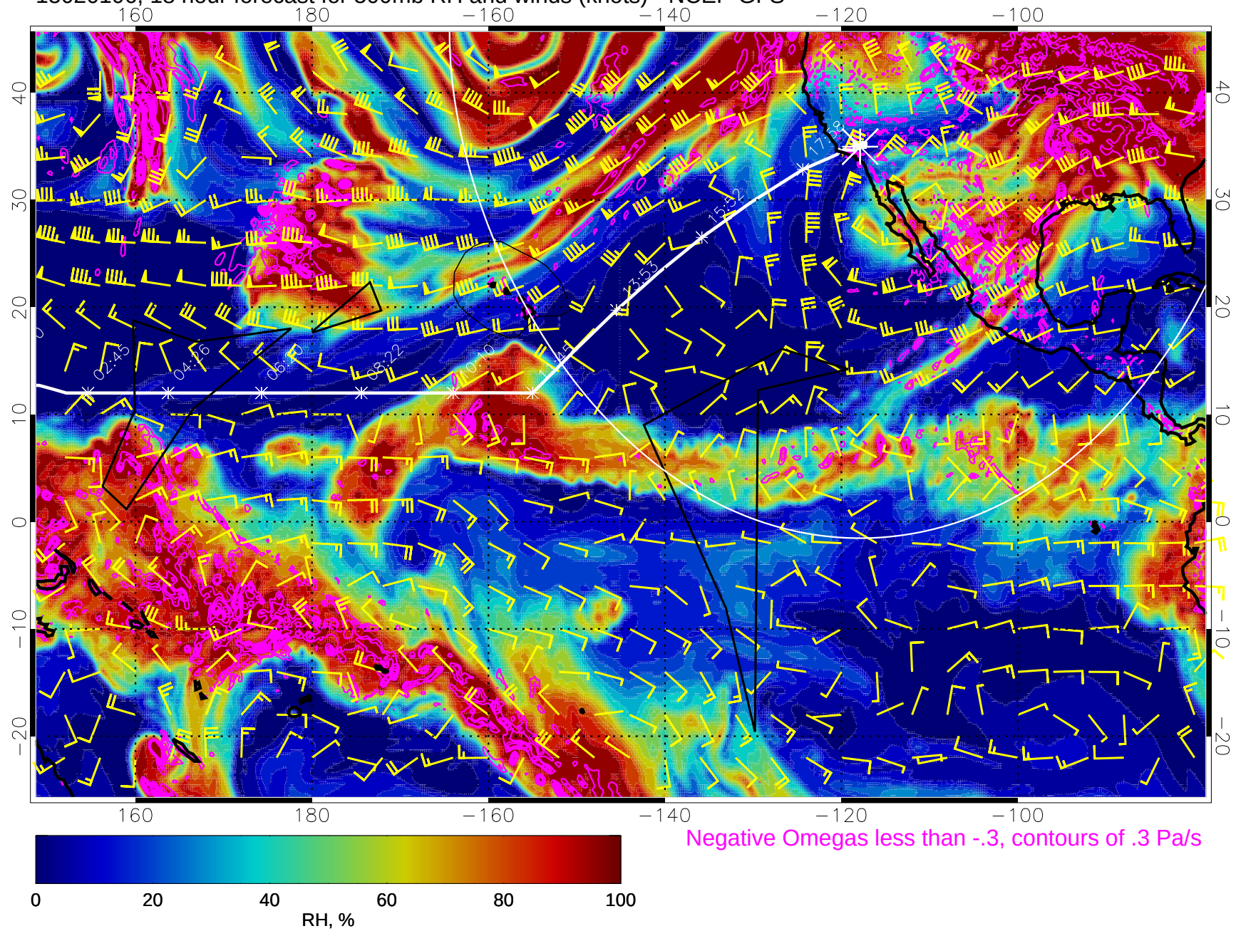
15020106, 18 hour forecast for 500mb RH and winds (knots) - NCEP GFS
