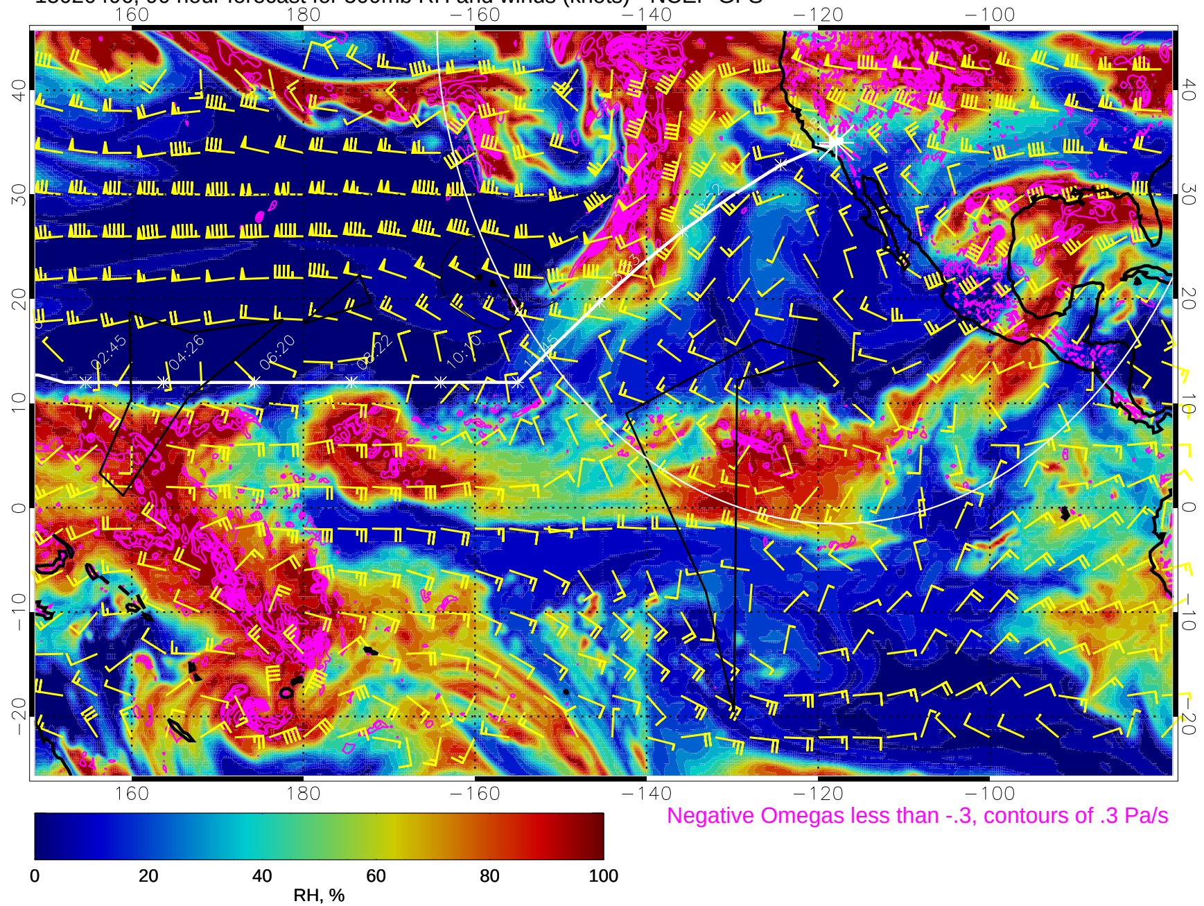
15020406, 90 hour forecast for 500mb RH and winds (knots) - NCEP GFS
