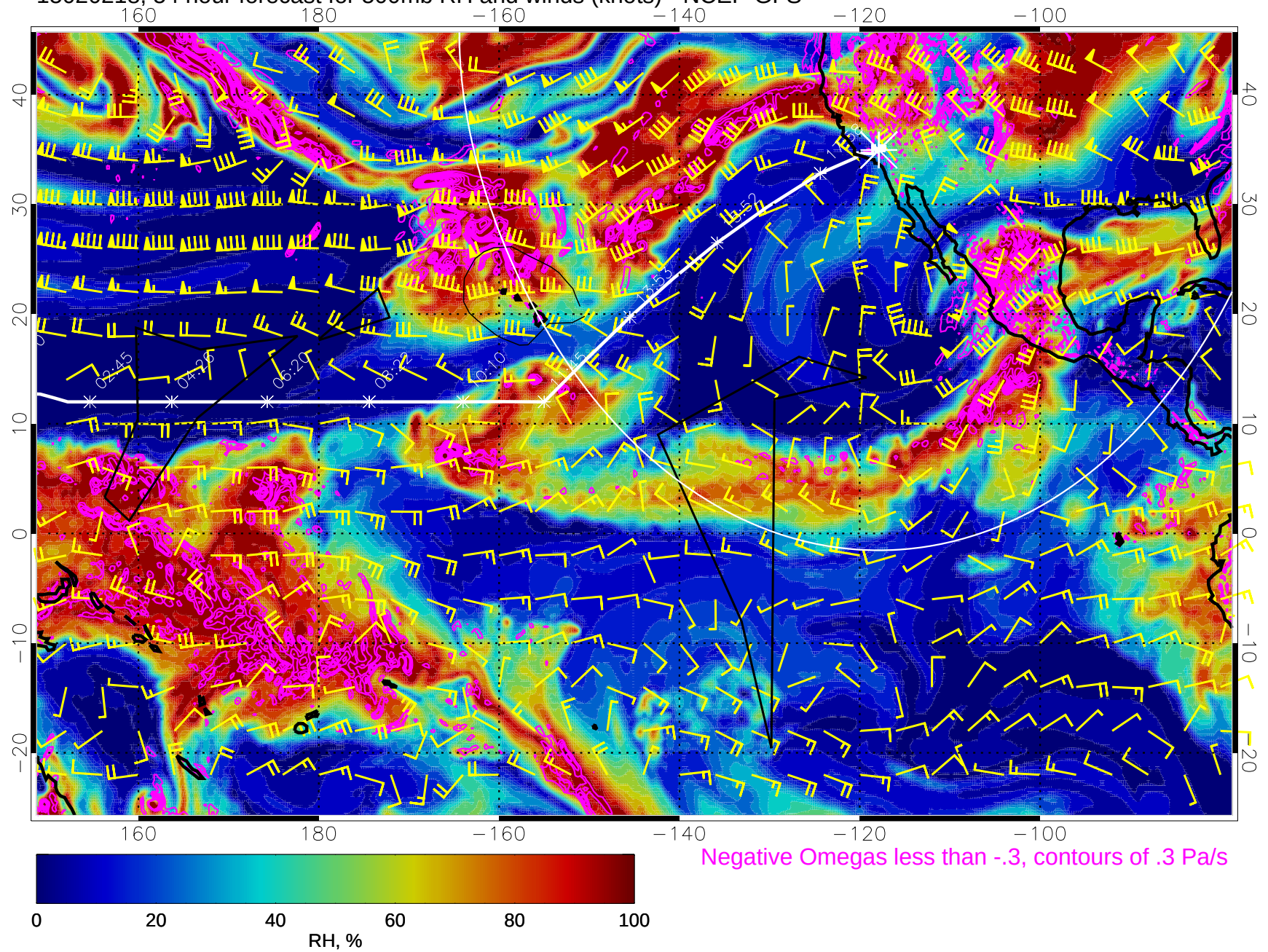
15020218, 54 hour forecast for 500mb RH and winds (knots) - NCEP GFS
