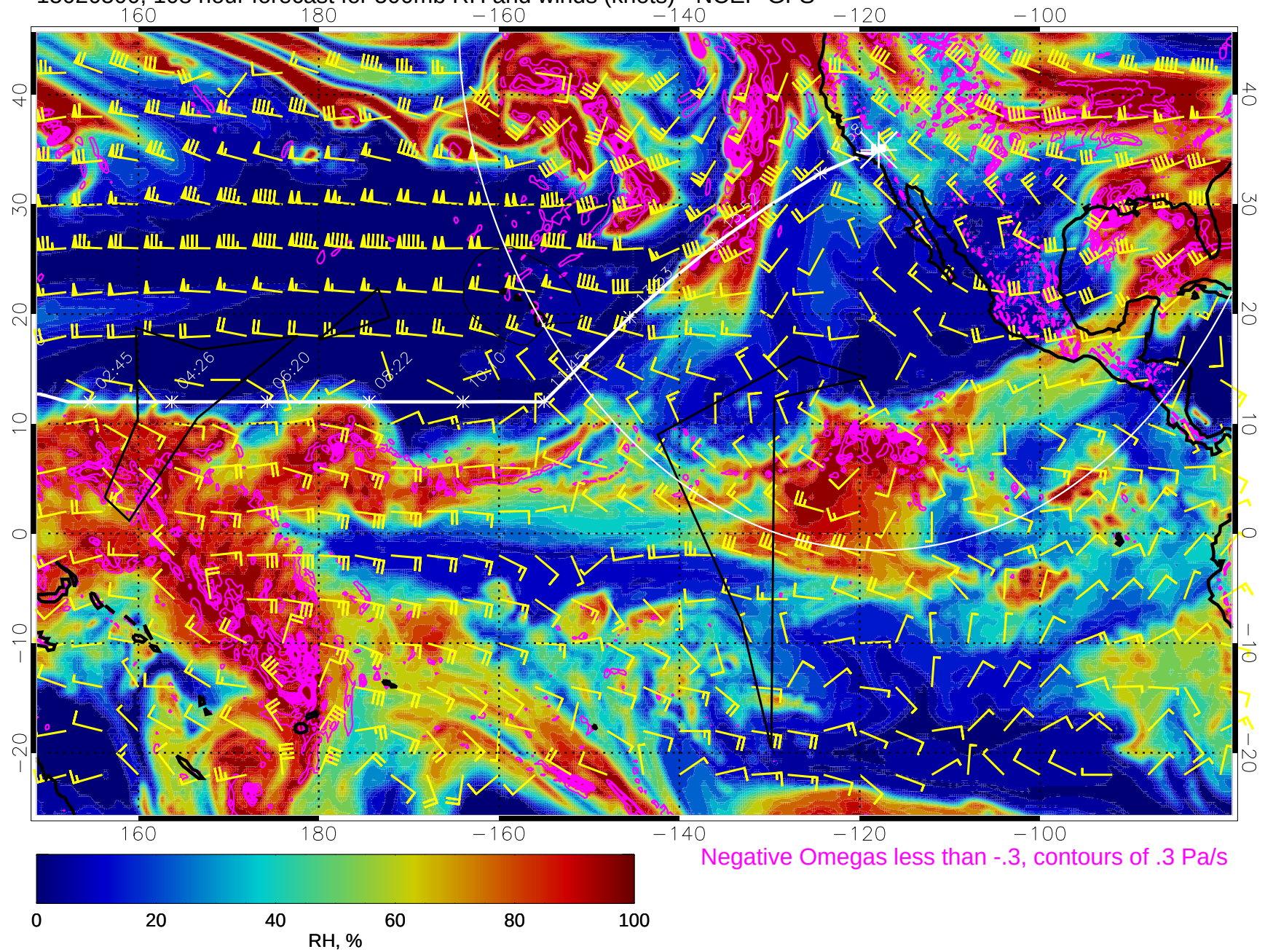
15020500, 108 hour forecast for 500mb RH and winds (knots) - NCEP GFS
