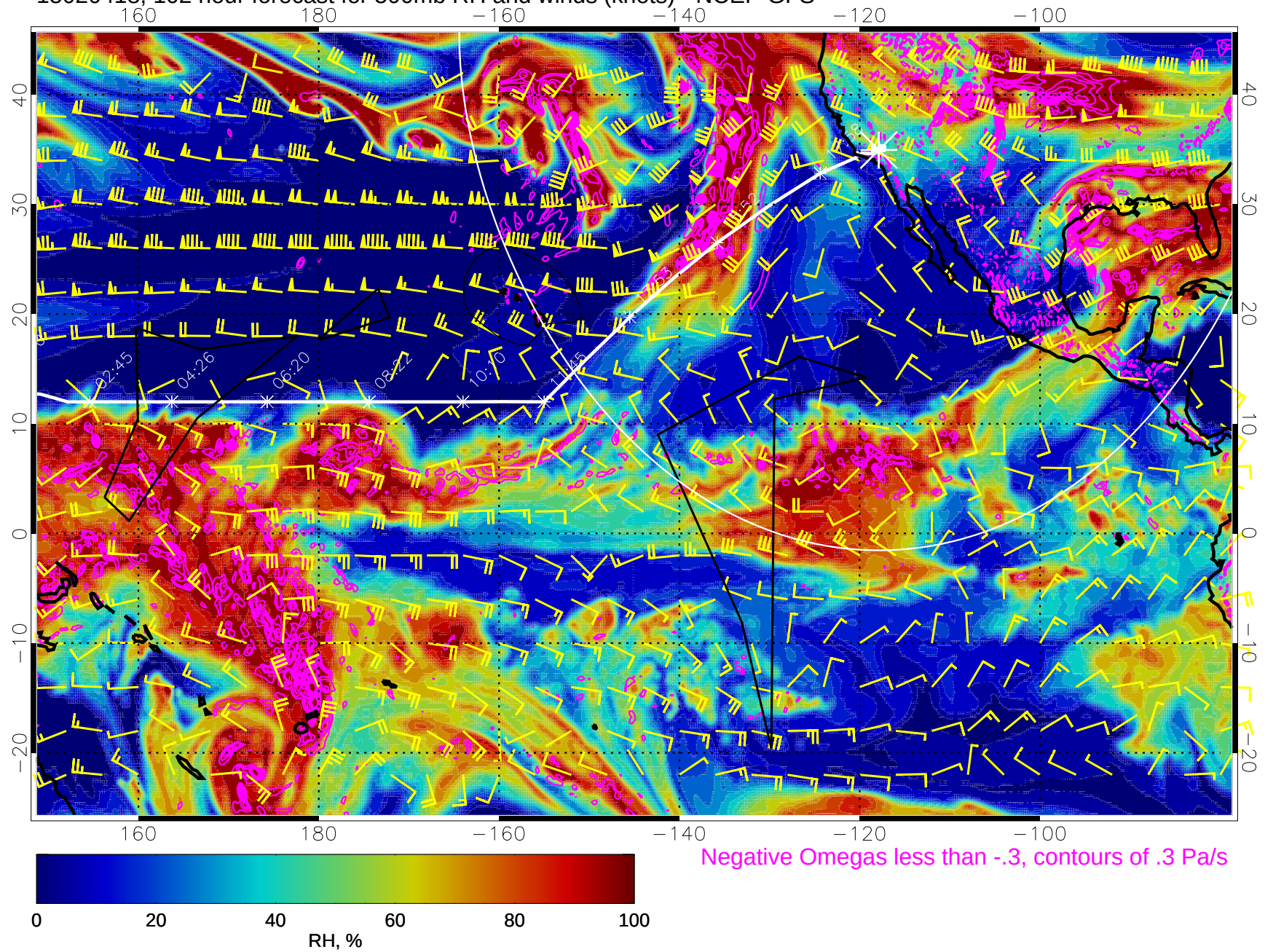
15020418, 102 hour forecast for 500mb RH and winds (knots) - NCEP GFS
