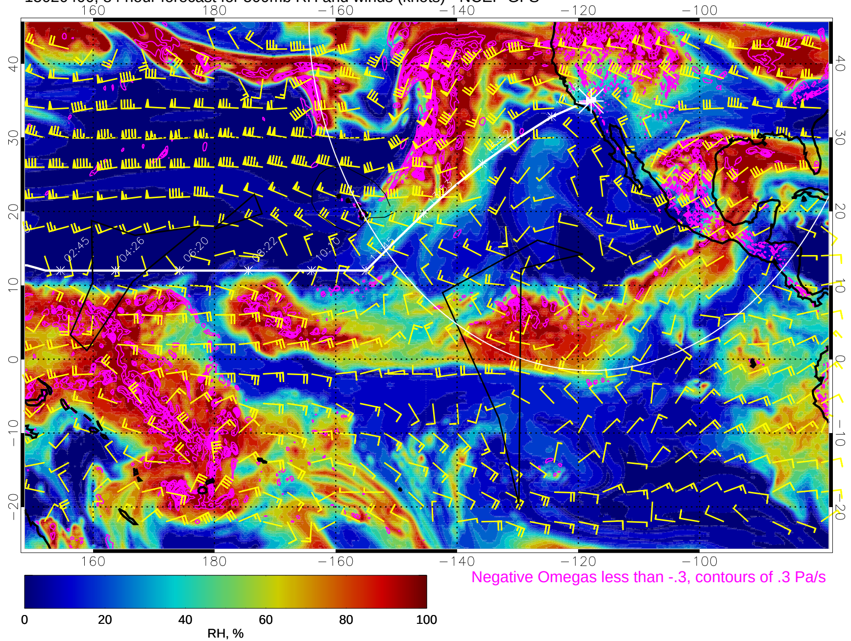
15020400, 84 hour forecast for 500mb RH and winds (knots) - NCEP GFS
