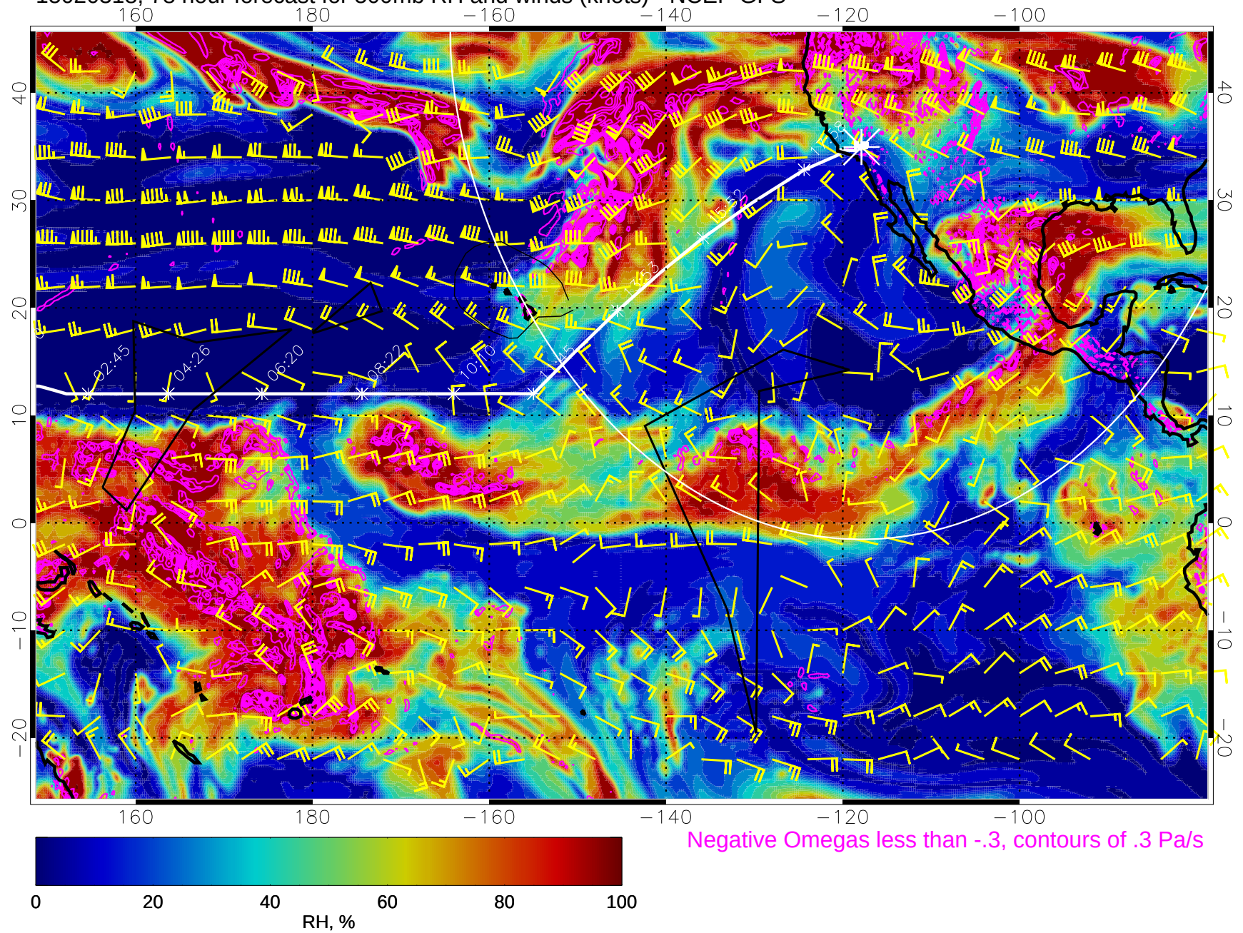
15020318, 78 hour forecast for 500mb RH and winds (knots) - NCEP GFS
