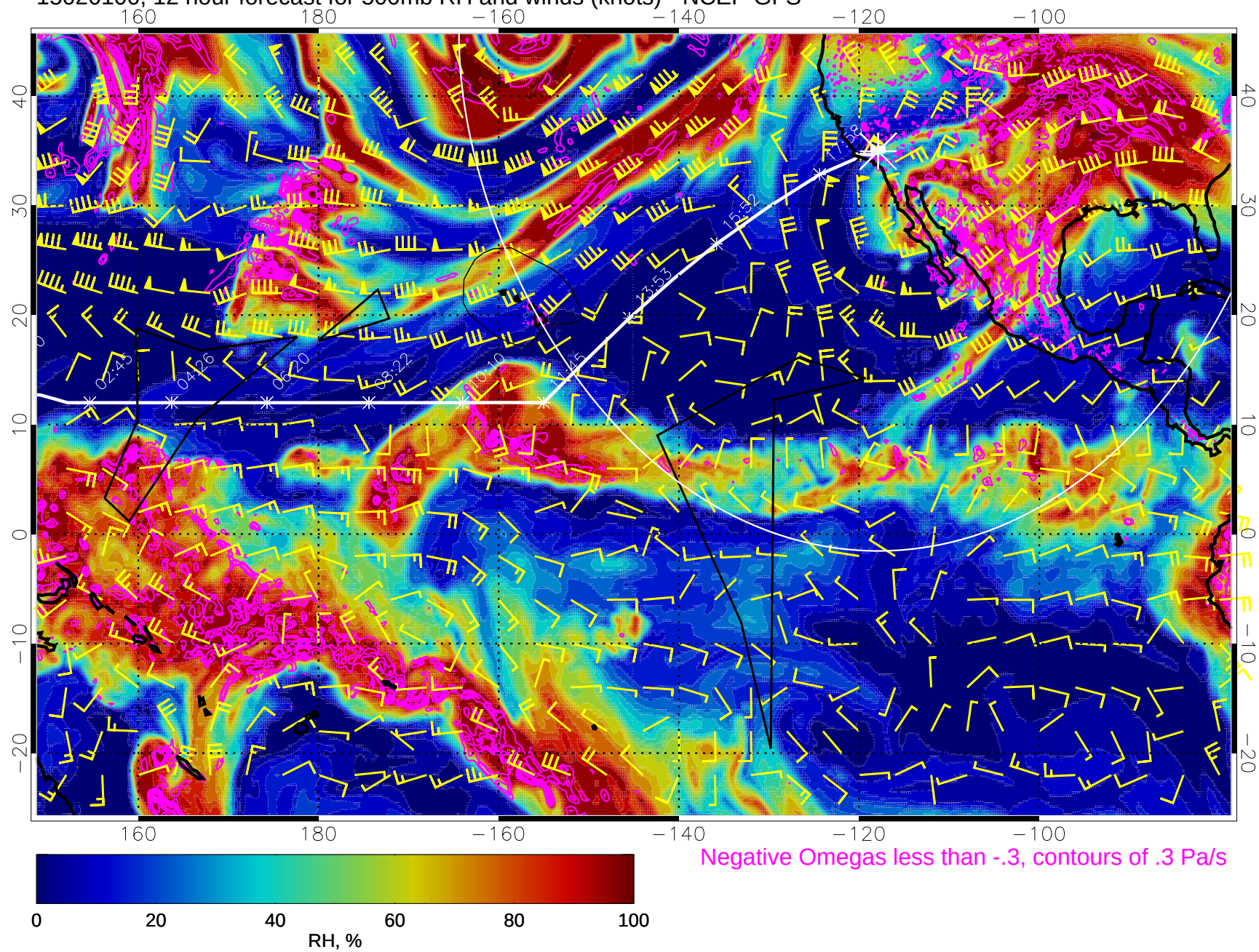
15020100, 12 hour forecast for 500mb RH and winds (knots) - NCEP GFS
