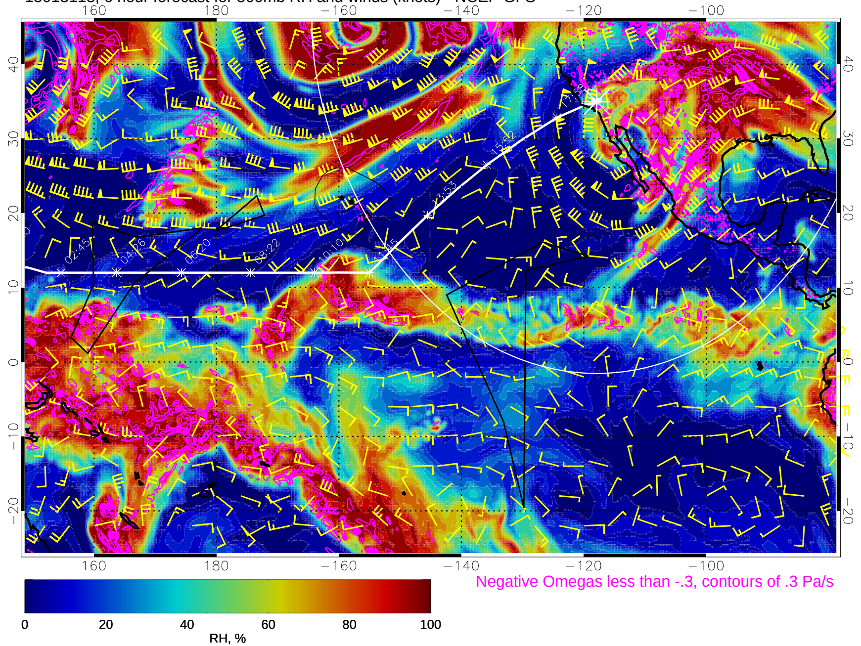
15013118, 6 hour forecast for 500mb RH and winds (knots) - NCEP GFS
