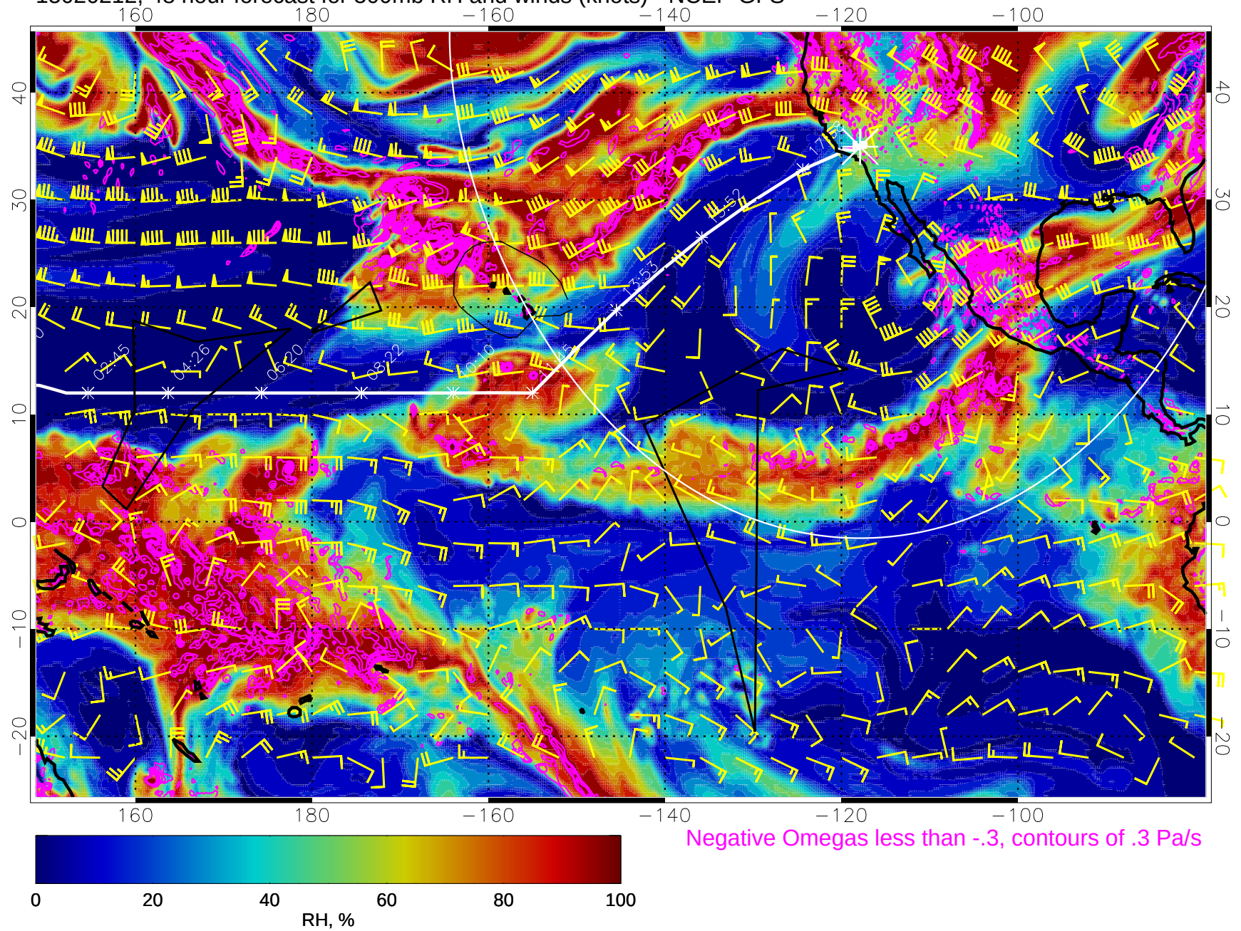
15020212, 48 hour forecast for 500mb RH and winds (knots) - NCEP GFS
