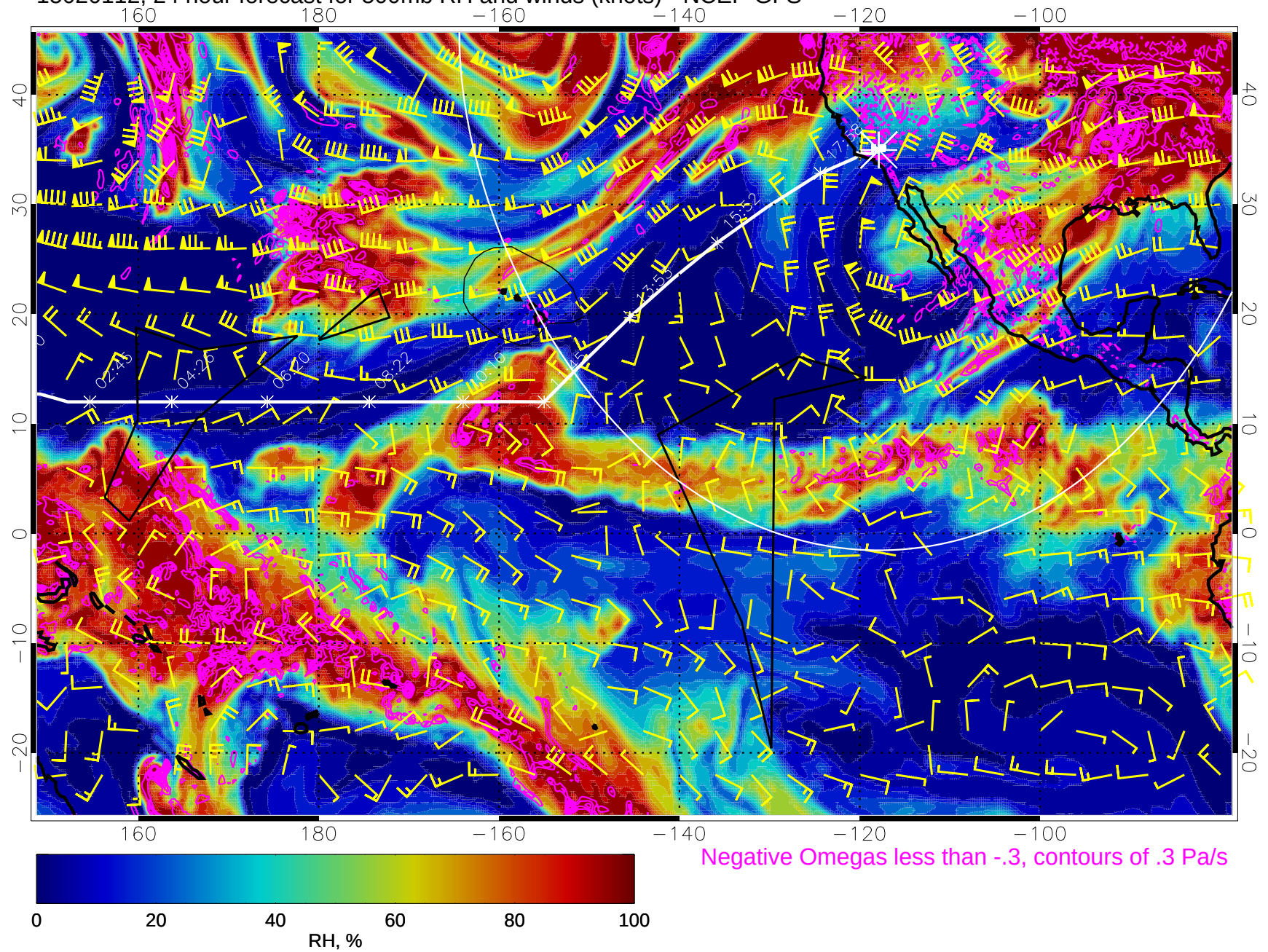
15020112, 24 hour forecast for 500mb RH and winds (knots) - NCEP GFS
