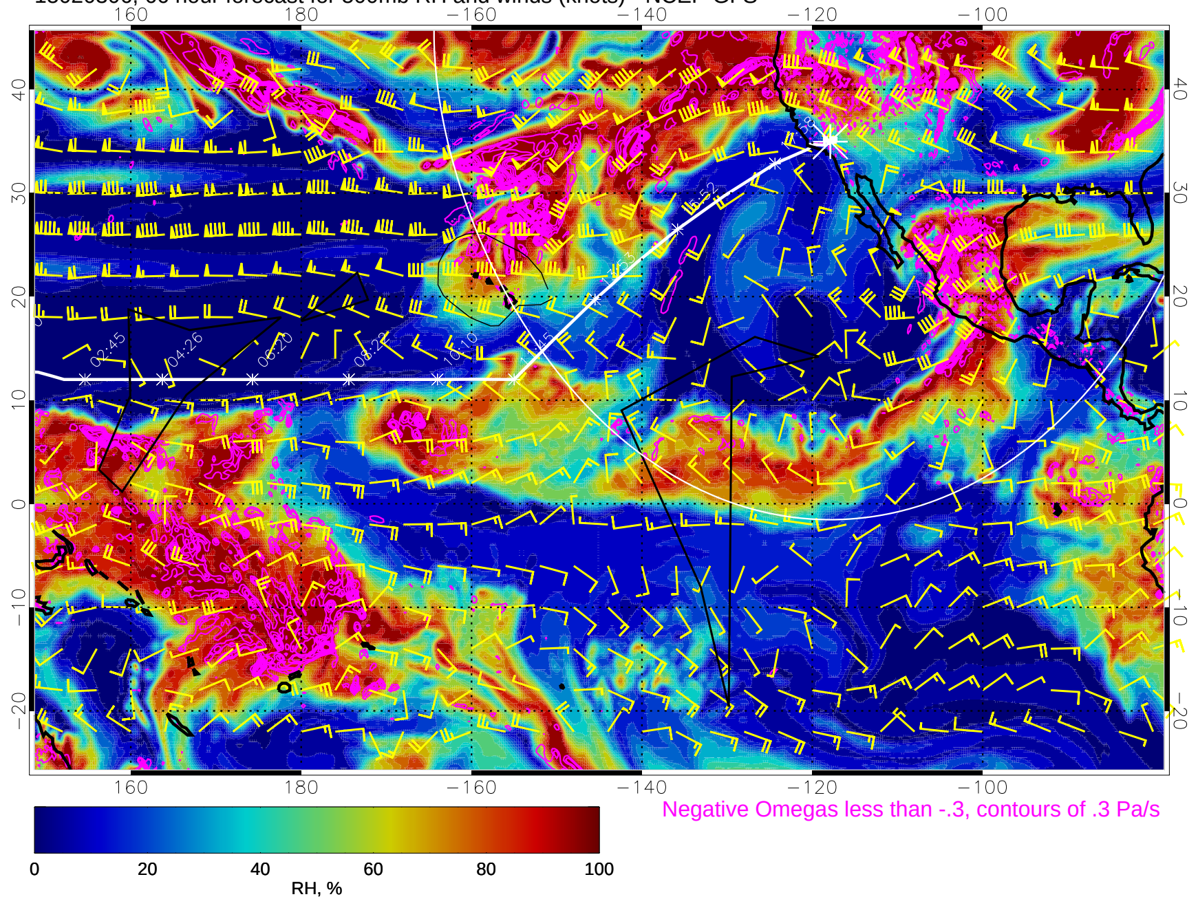
15020306, 66 hour forecast for 500mb RH and winds (knots) - NCEP GFS
