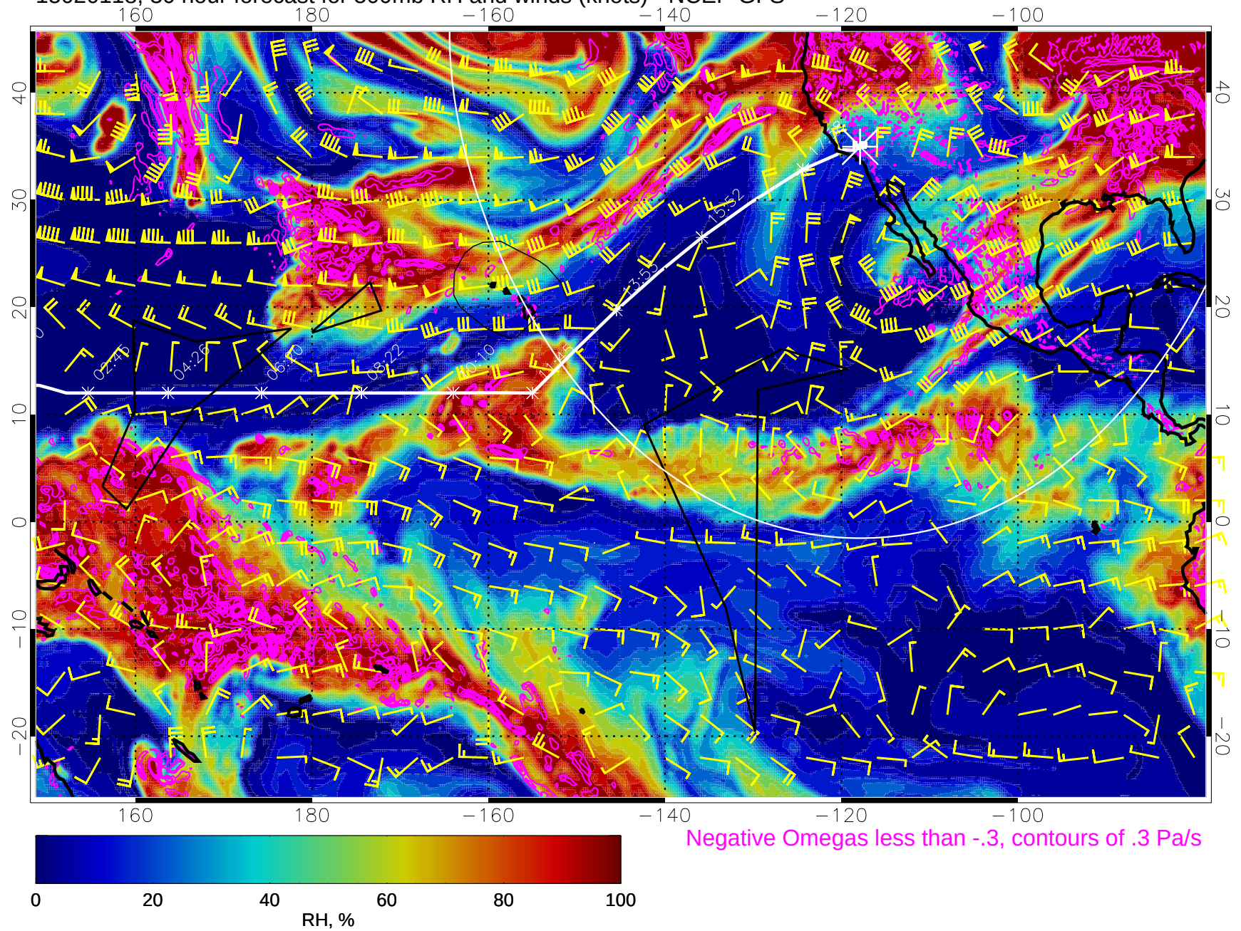
15020118, 30 hour forecast for 500mb RH and winds (knots) - NCEP GFS
