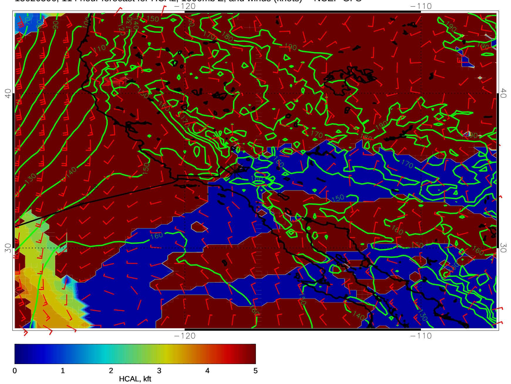
15020506, 114 hour forecast for HCAL, 1000mb Z, and winds (knots) -- NCEP GFS
