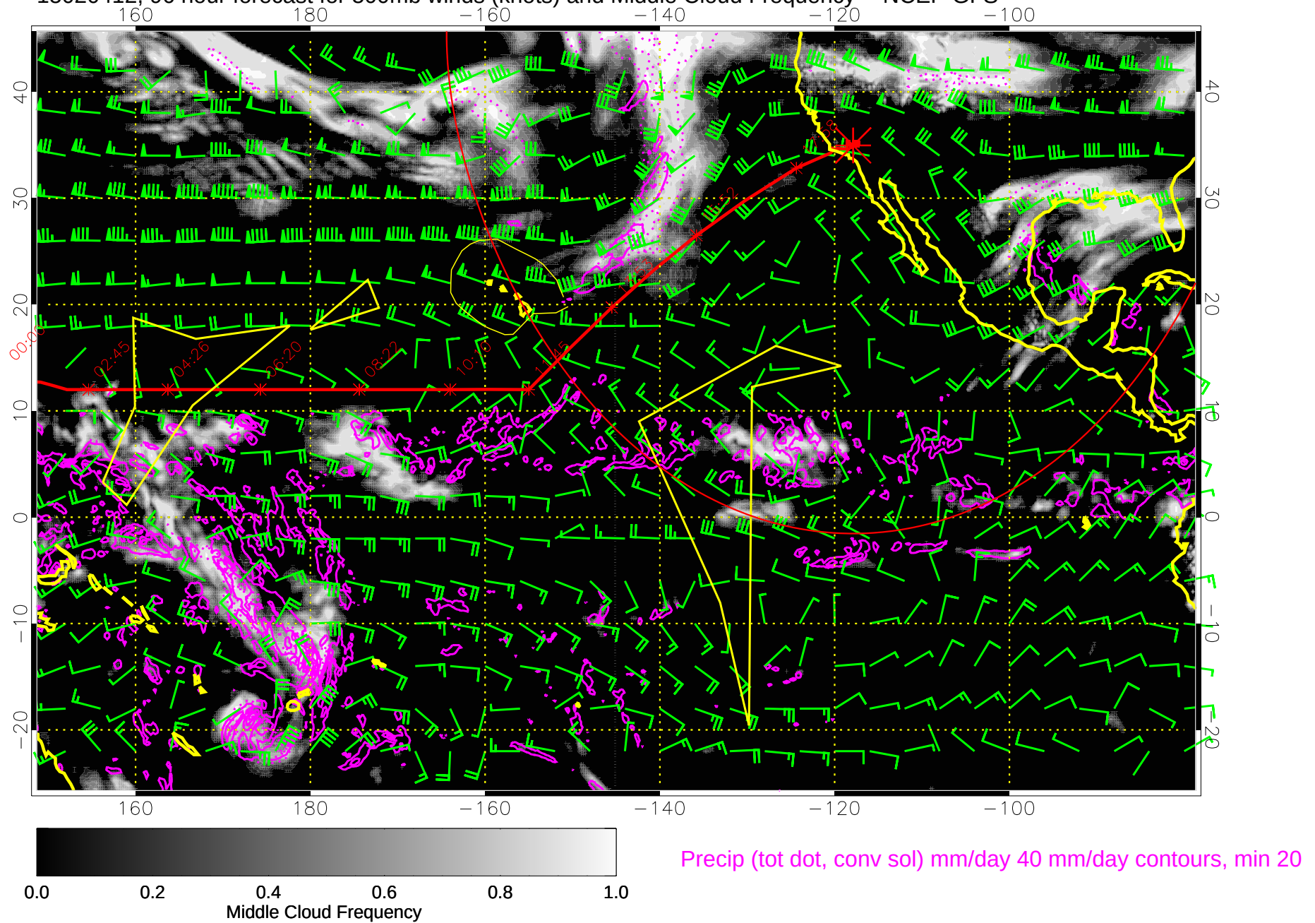
15020412, 96 hour forecast for 500mb winds (knots) and Middle Cloud Frequency -- NCEP GFS
