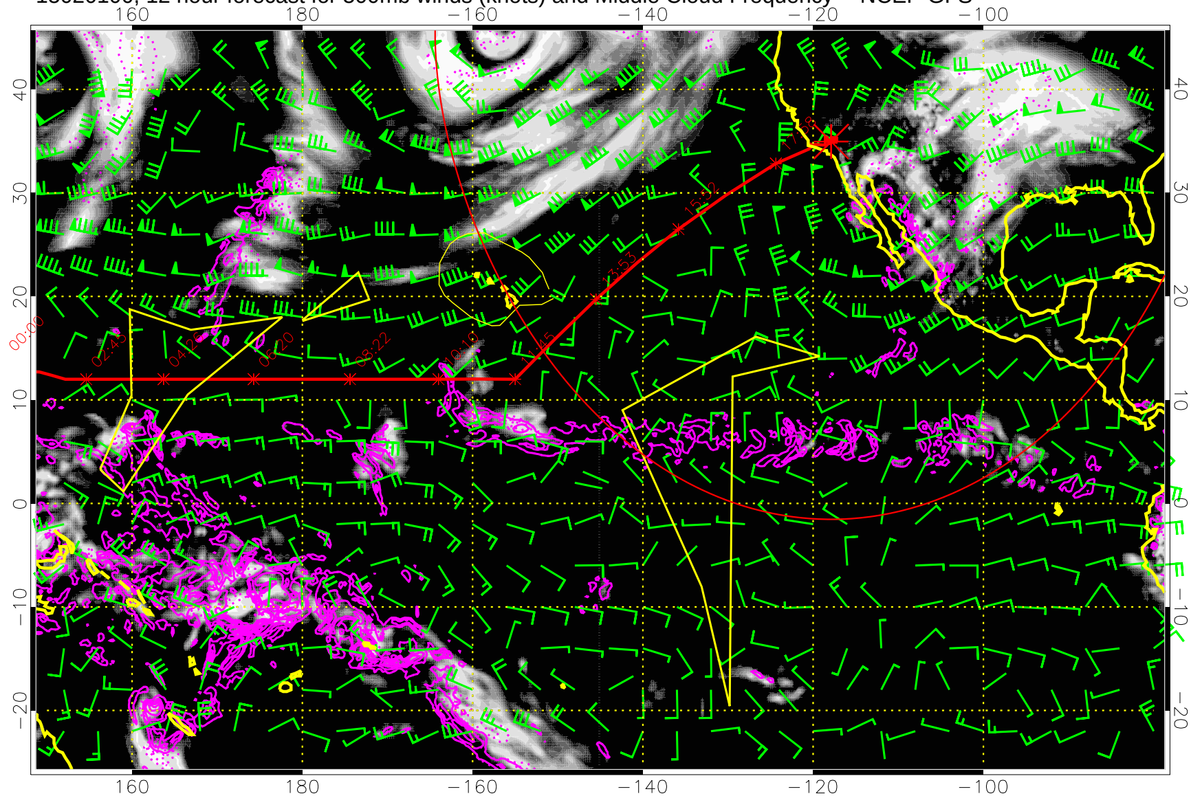
15020100, 12 hour forecast for 500mb winds (knots) and Middle Cloud Frequency -- NCEP GFS
