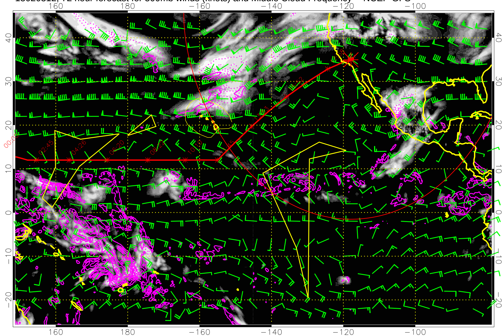
15020312, 72 hour forecast for 500mb winds (knots) and Middle Cloud Frequency -- NCEP GFS
