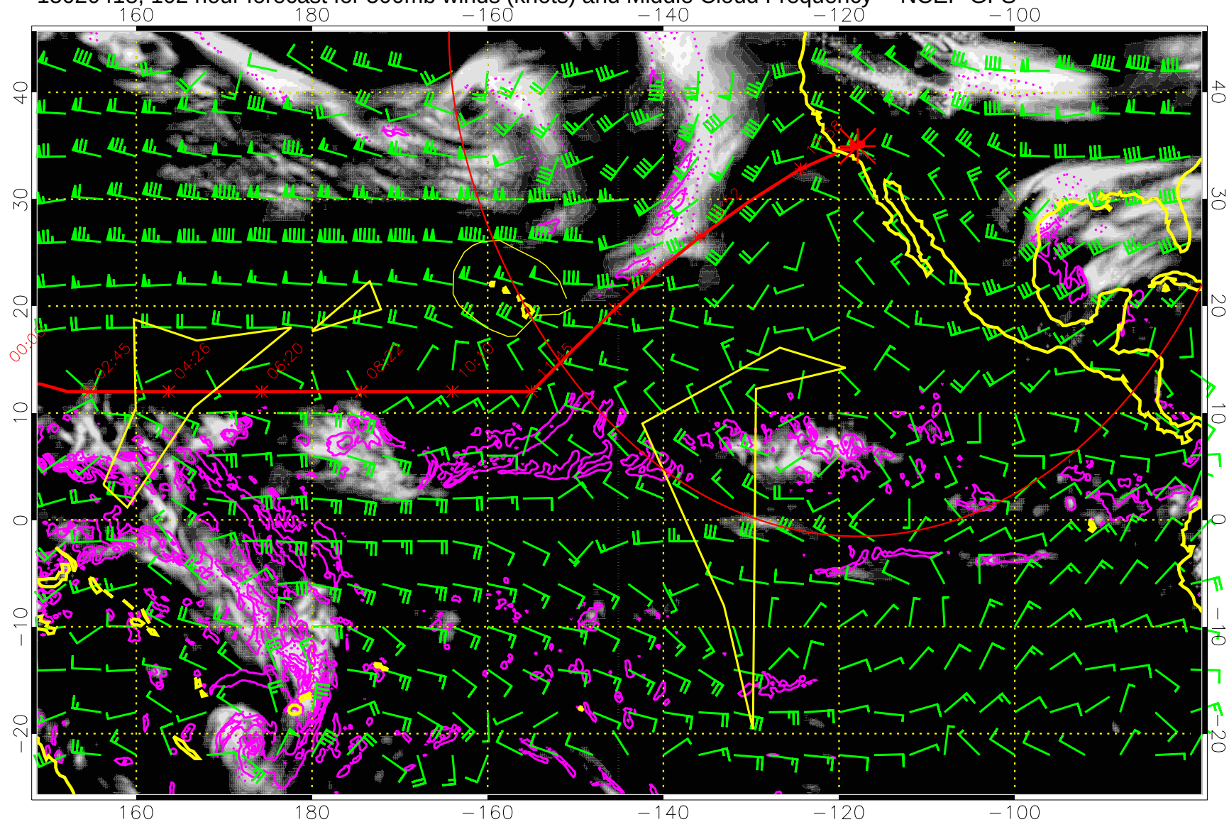
15020418, 102 hour forecast for 500mb winds (knots) and Middle Cloud Frequency -- NCEP GFS
