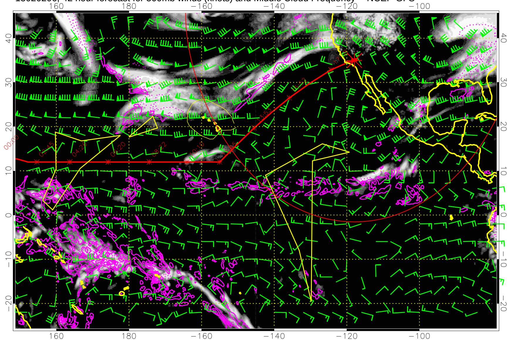
15020206, 42 hour forecast for 500mb winds (knots) and Middle Cloud Frequency -- NCEP GFS
