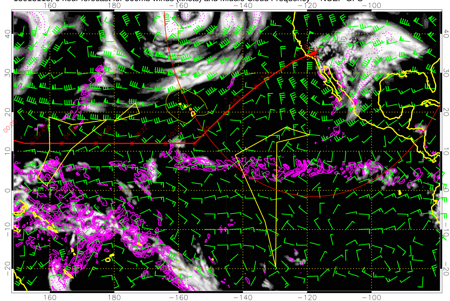
15013118, 6 hour forecast for 500mb winds (knots) and Middle Cloud Frequency -- NCEP GFS
