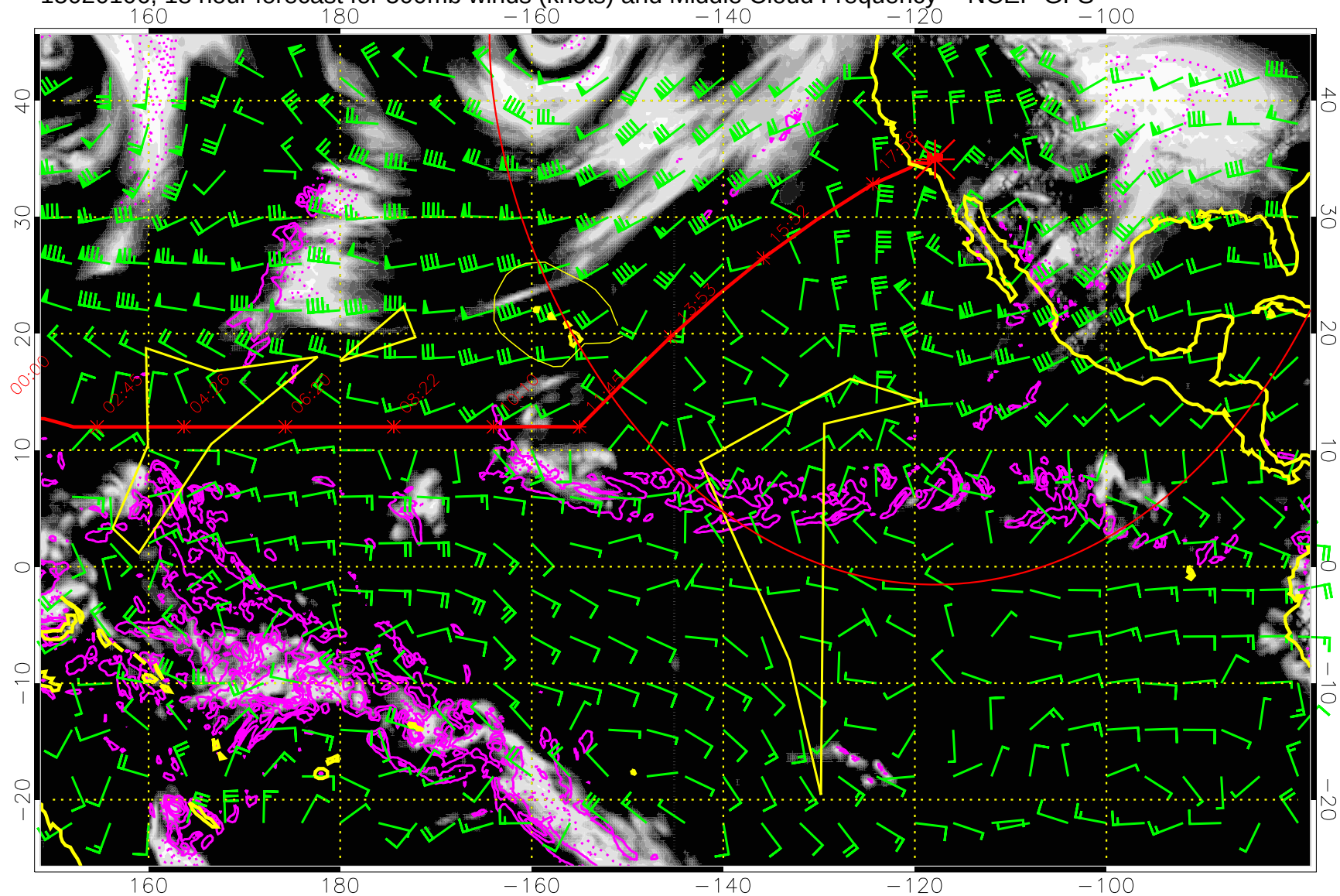
15020106, 18 hour forecast for 500mb winds (knots) and Middle Cloud Frequency -- NCEP GFS
