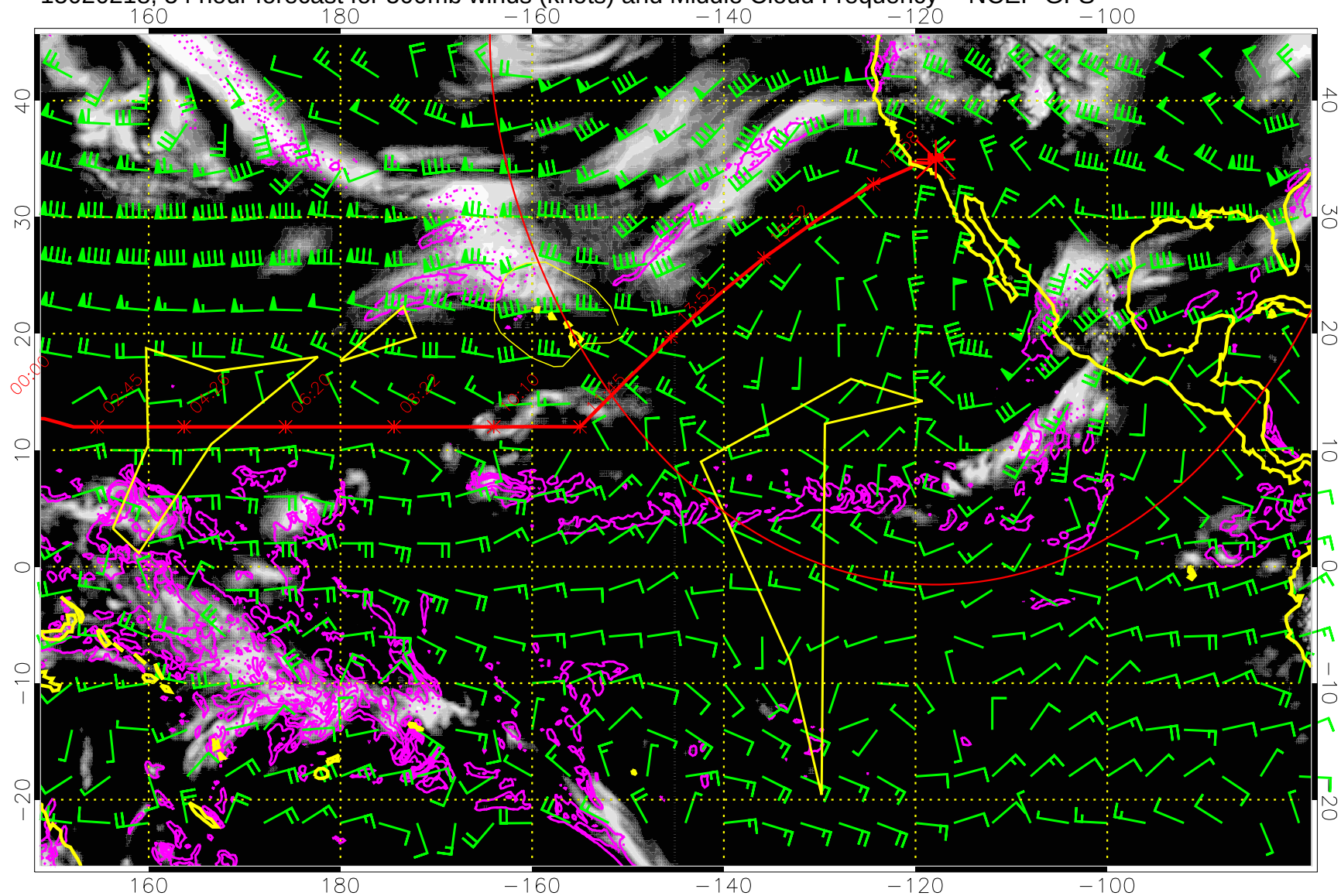
15020218, 54 hour forecast for 500mb winds (knots) and Middle Cloud Frequency -- NCEP GFS
