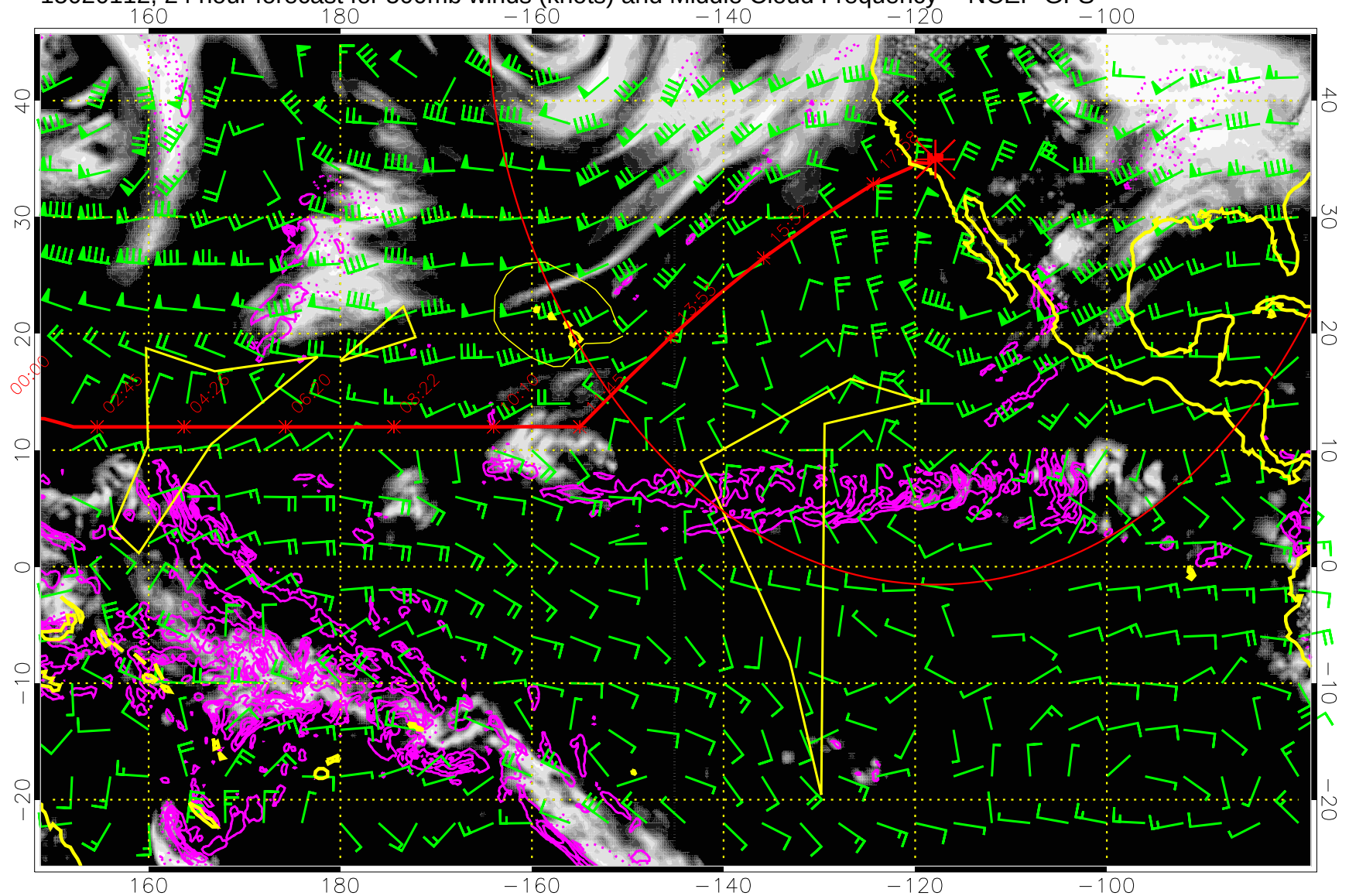
15020112, 24 hour forecast for 500mb winds (knots) and Middle Cloud Frequency -- NCEP GFS
