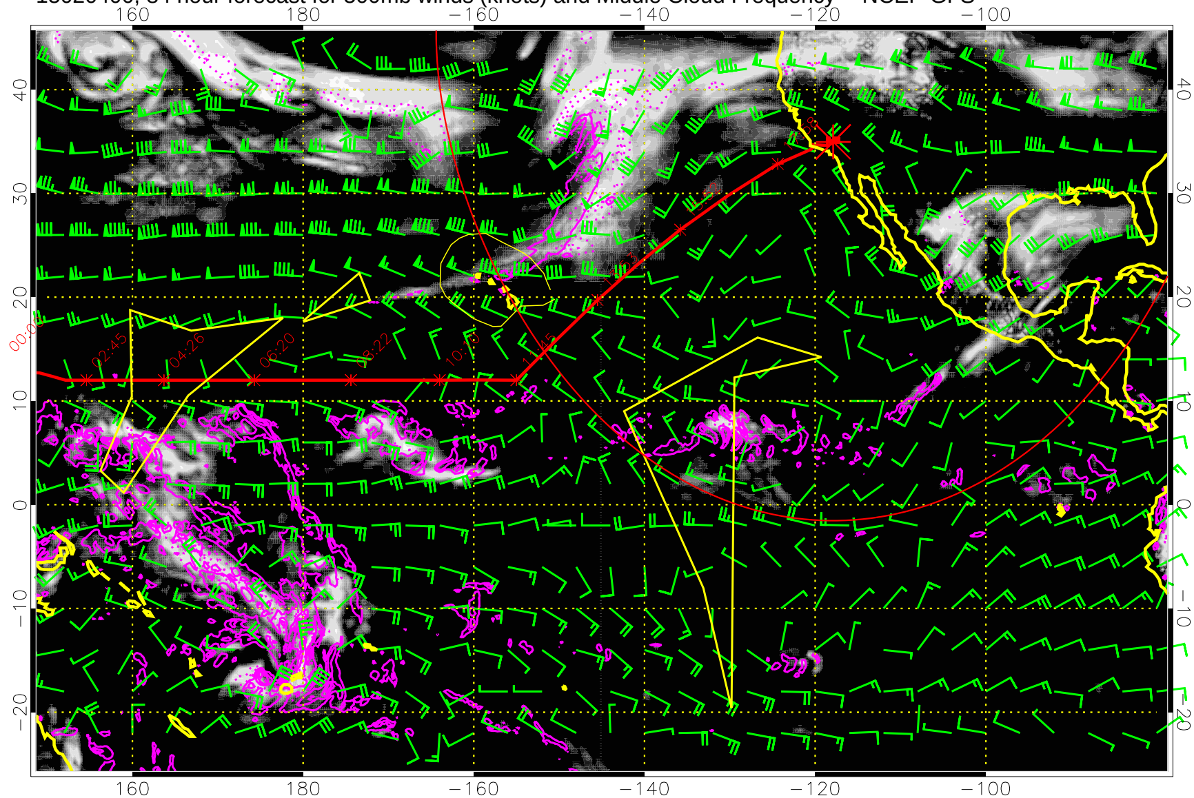
15020400, 84 hour forecast for 500mb winds (knots) and Middle Cloud Frequency -- NCEP GFS
