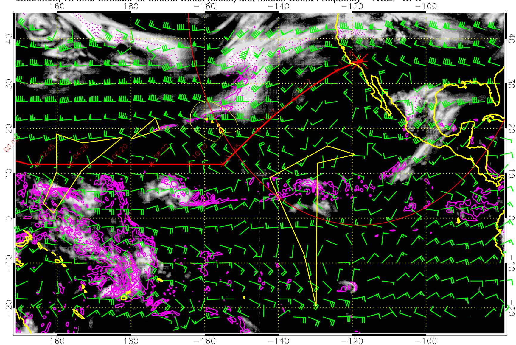
15020318, 78 hour forecast for 500mb winds (knots) and Middle Cloud Frequency -- NCEP GFS
