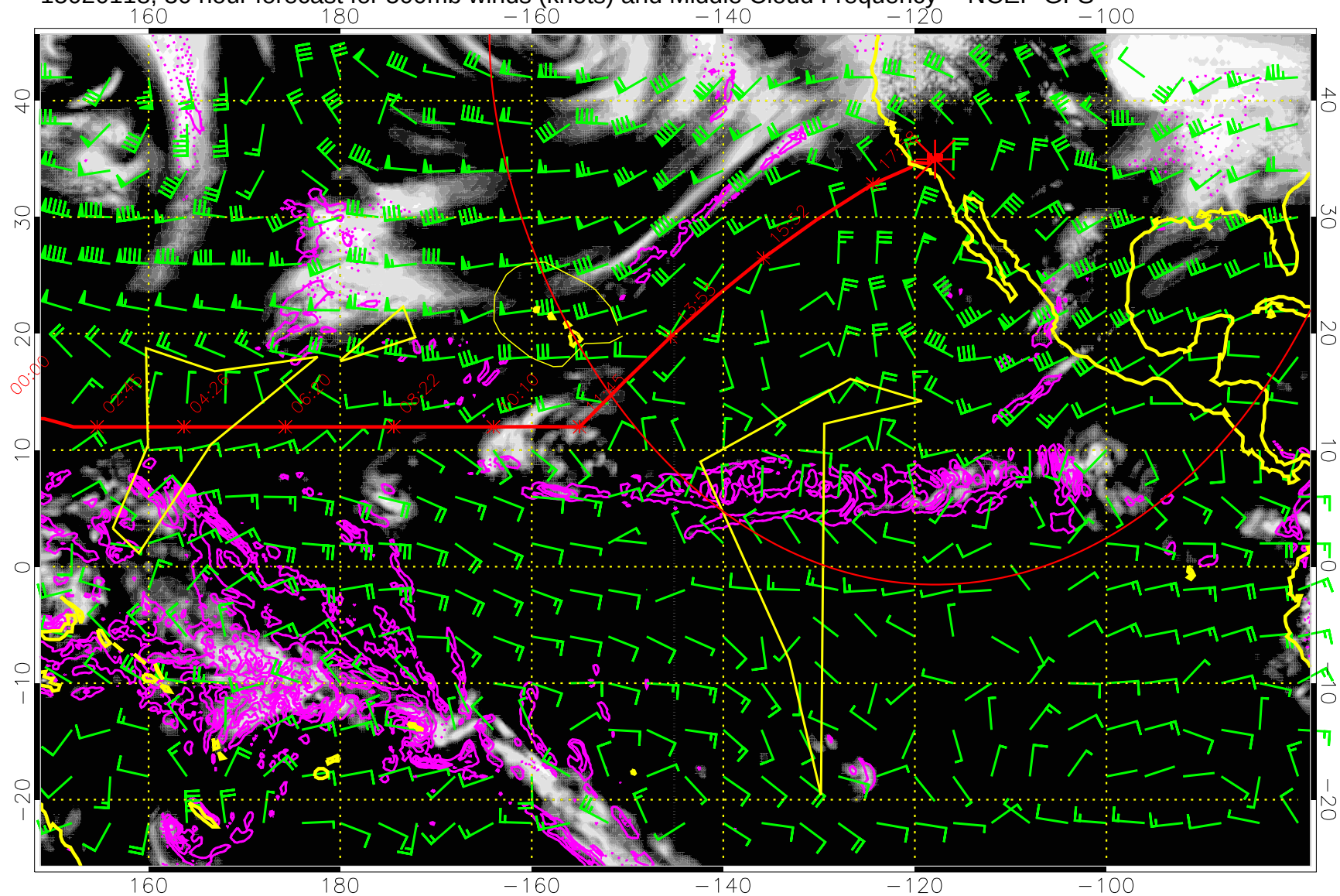
15020118, 30 hour forecast for 500mb winds (knots) and Middle Cloud Frequency -- NCEP GFS
