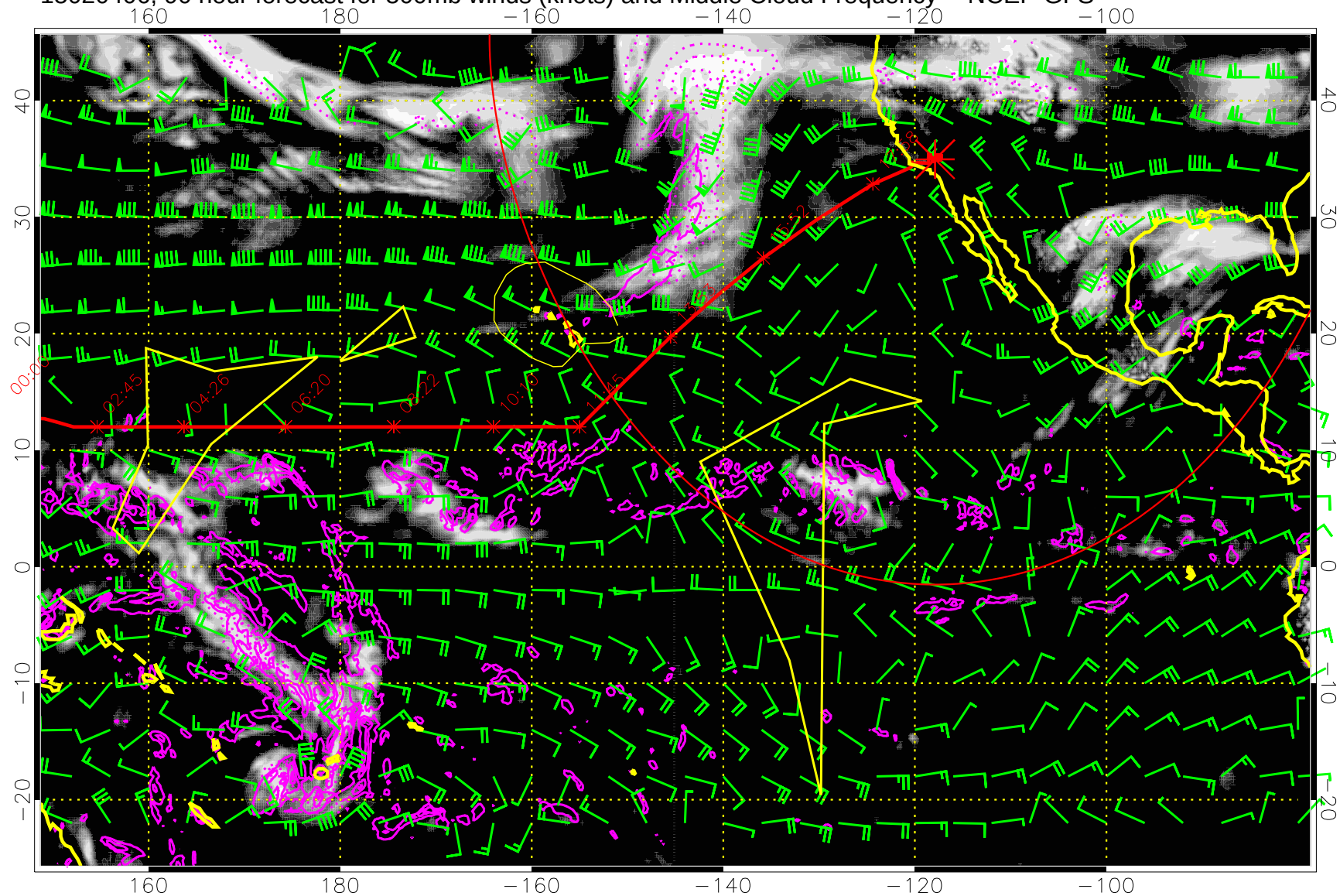
15020406, 90 hour forecast for 500mb winds (knots) and Middle Cloud Frequency -- NCEP GFS
