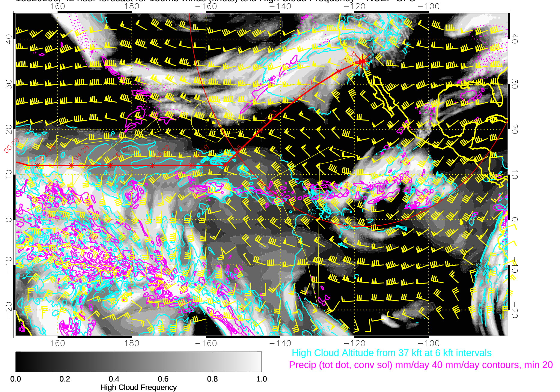
15020206, 42 hour forecast for 150mb winds (knots) and High Cloud Frequency -- NCEP GFS
