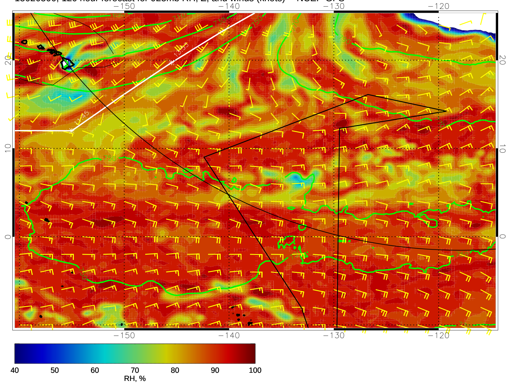
15020500, 120 hour forecast for 925mb RH, Z, and winds (knots) -- NCEP GFS
