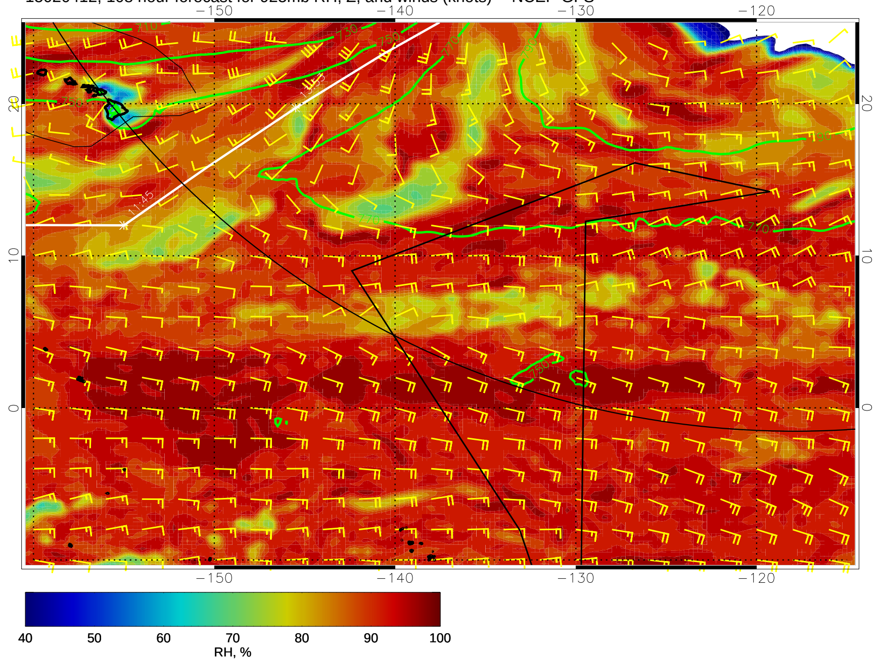
15020412, 108 hour forecast for 925mb RH, Z, and winds (knots) -- NCEP GFS
