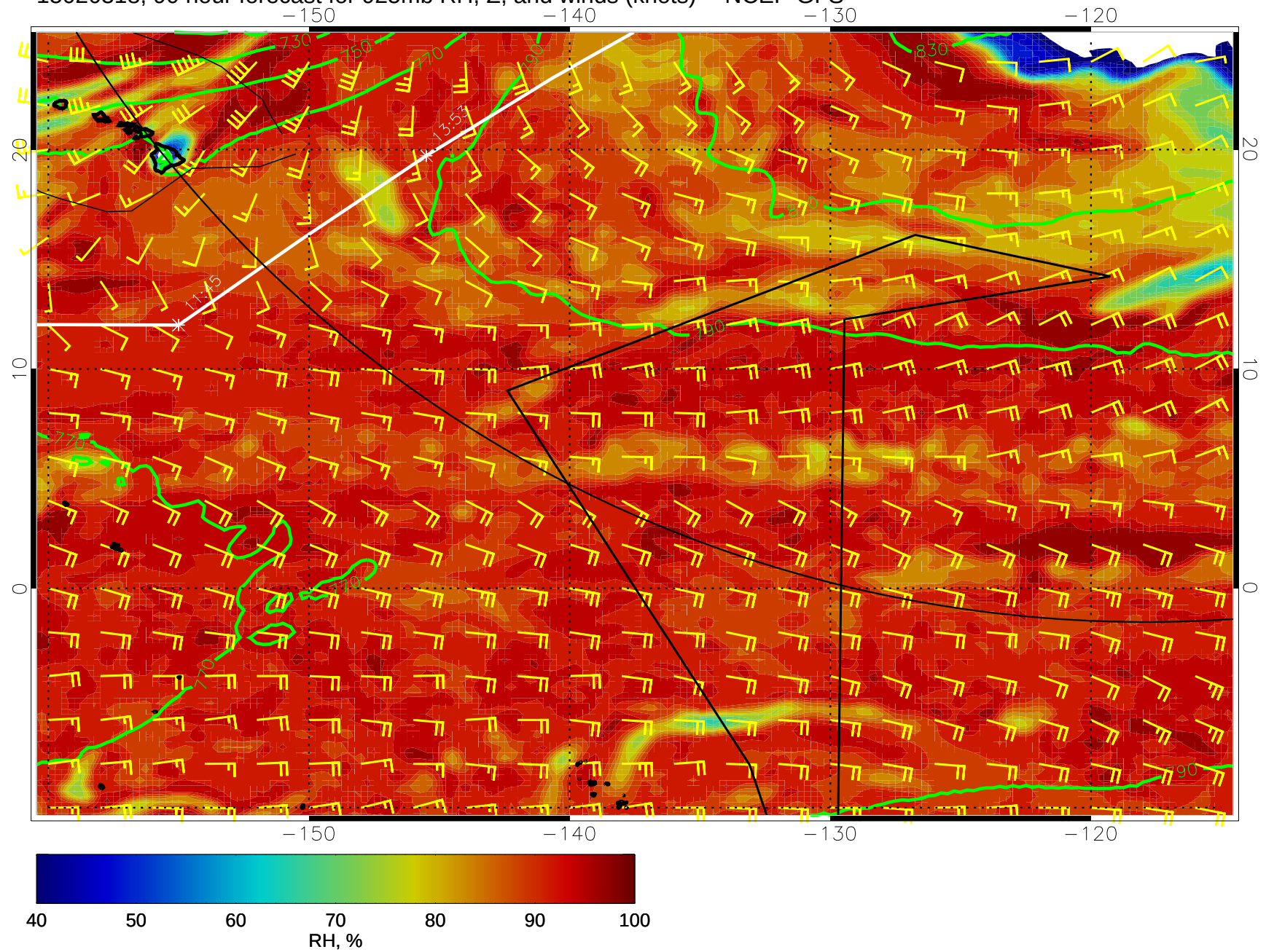
15020318, 90 hour forecast for 925mb RH, Z, and winds (knots) -- NCEP GFS
