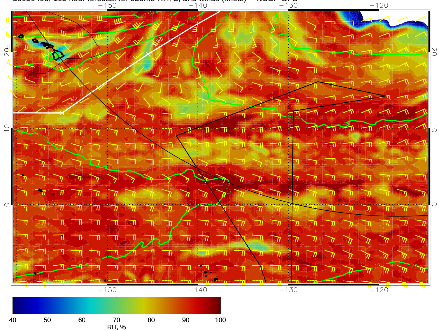
15020406, 102 hour forecast for 925mb RH, Z, and winds (knots) -- NCEP GFS
