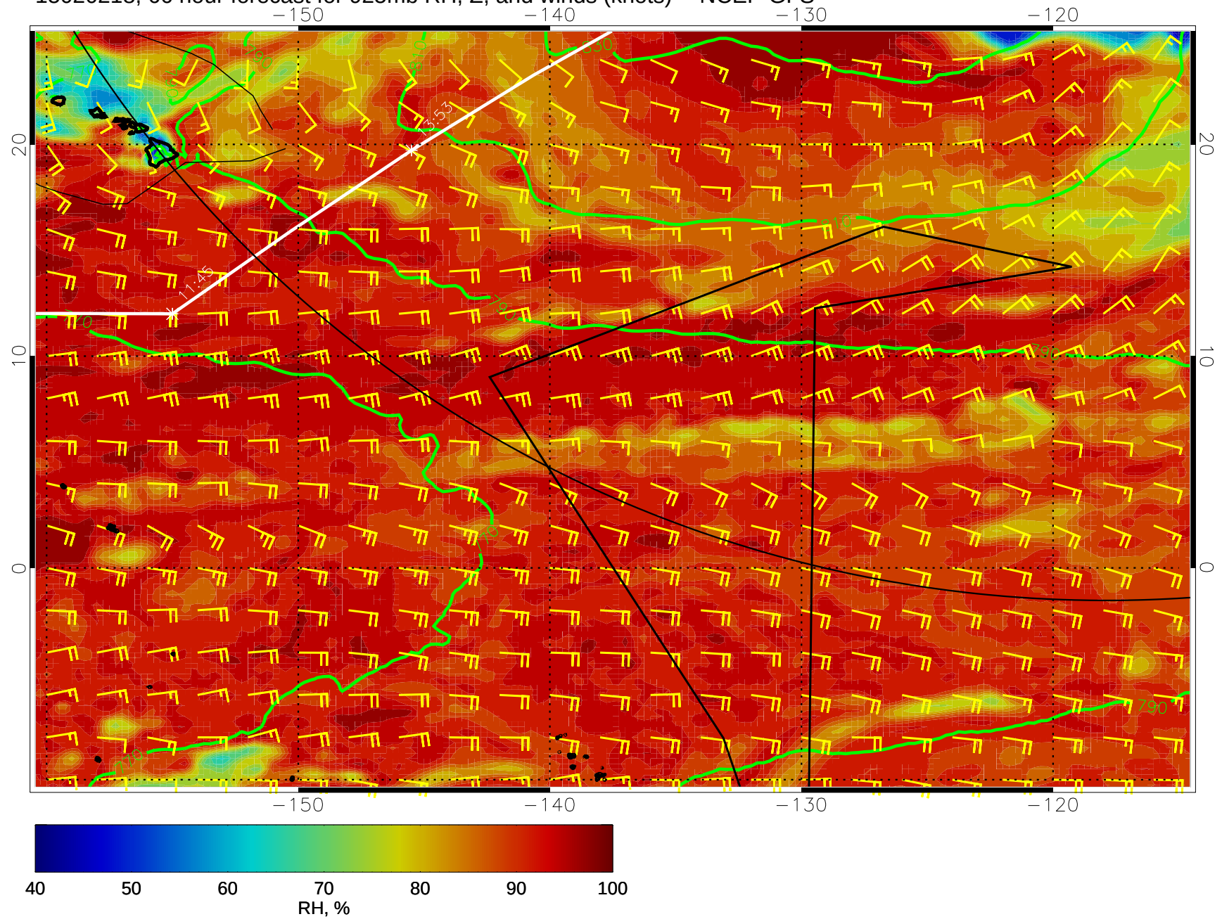
15020218, 66 hour forecast for 925mb RH, Z, and winds (knots) -- NCEP GFS
