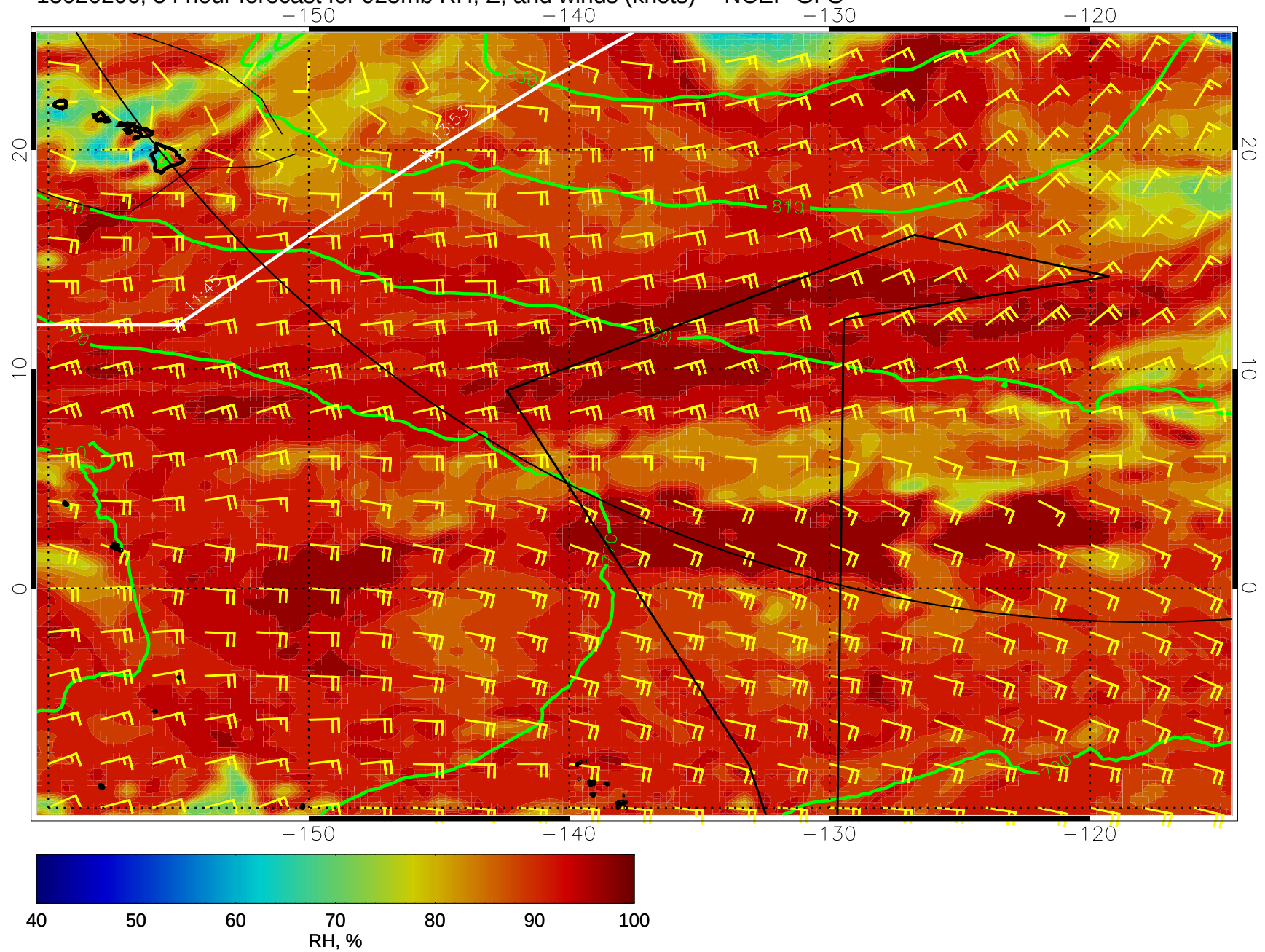
15020206, 54 hour forecast for 925mb RH, Z, and winds (knots) -- NCEP GFS
