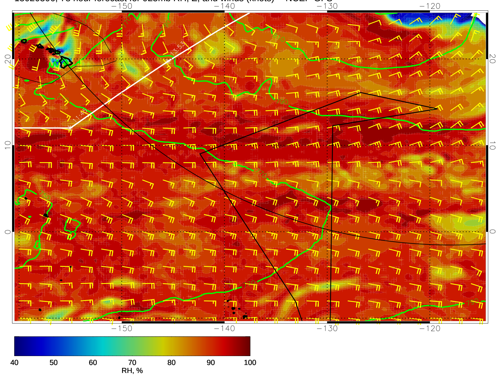
15020306, 78 hour forecast for 925mb RH, Z, and winds (knots) -- NCEP GFS
