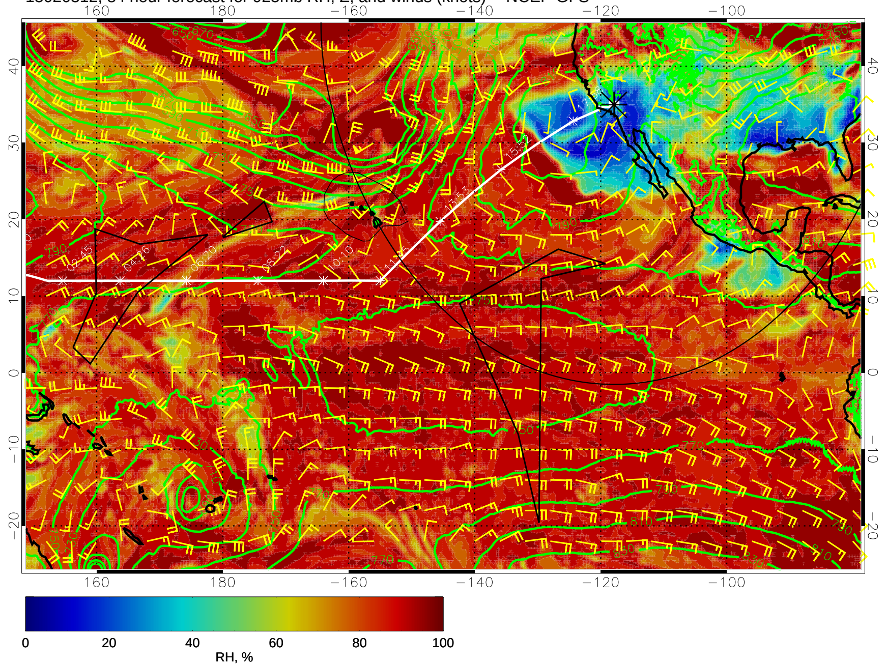
15020312, 84 hour forecast for 925mb RH, Z, and winds (knots) -- NCEP GFS
