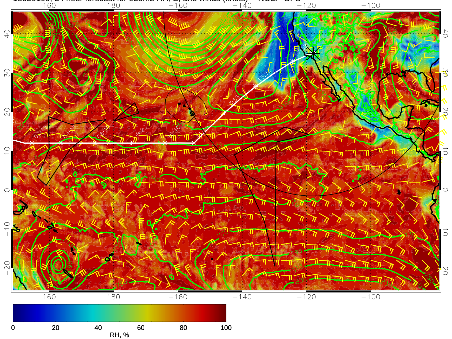
15020100, 24 hour forecast for 925mb RH, Z, and winds (knots) -- NCEP GFS
