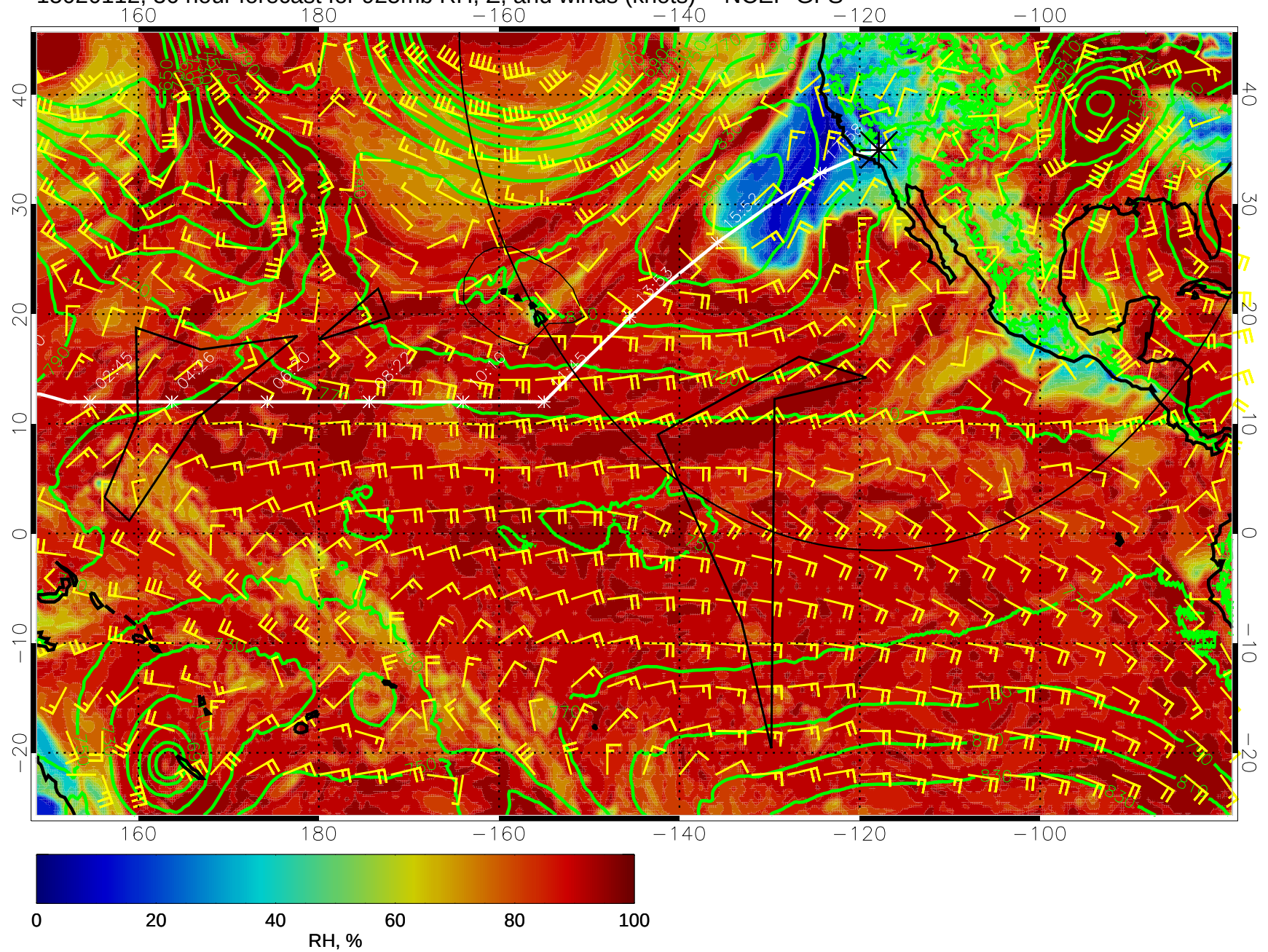
15020112, 36 hour forecast for 925mb RH, Z, and winds (knots) -- NCEP GFS
