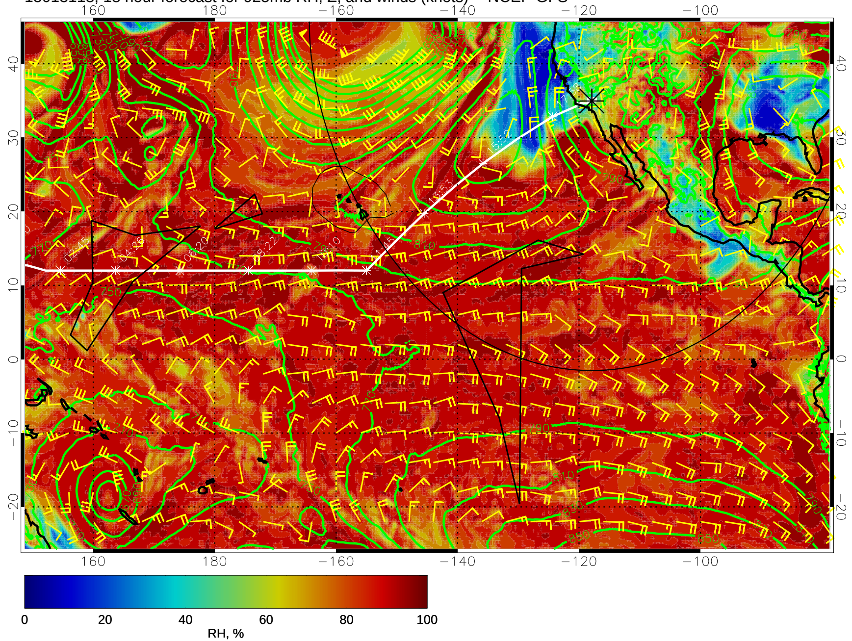
15013118, 18 hour forecast for 925mb RH, Z, and winds (knots) -- NCEP GFS
