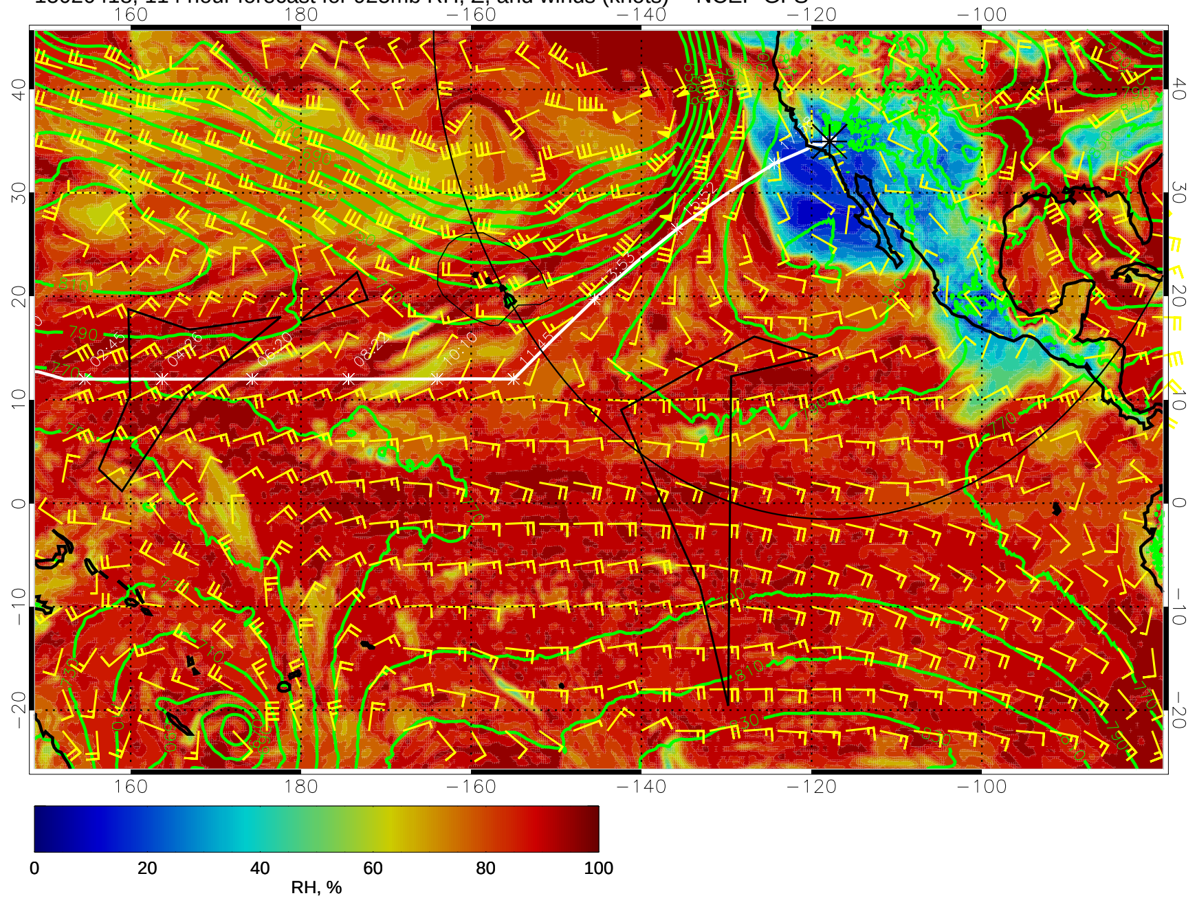
15020418, 114 hour forecast for 925mb RH, Z, and winds (knots) -- NCEP GFS
