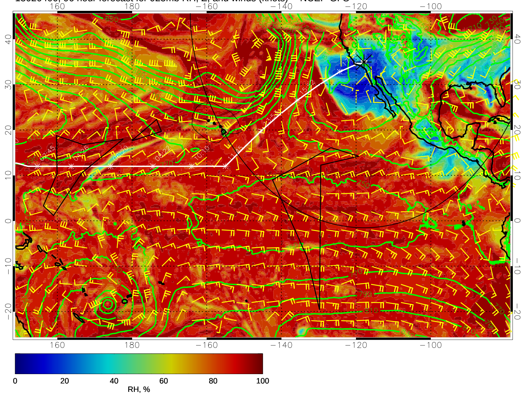
15020400, 96 hour forecast for 925mb RH, Z, and winds (knots) -- NCEP GFS
