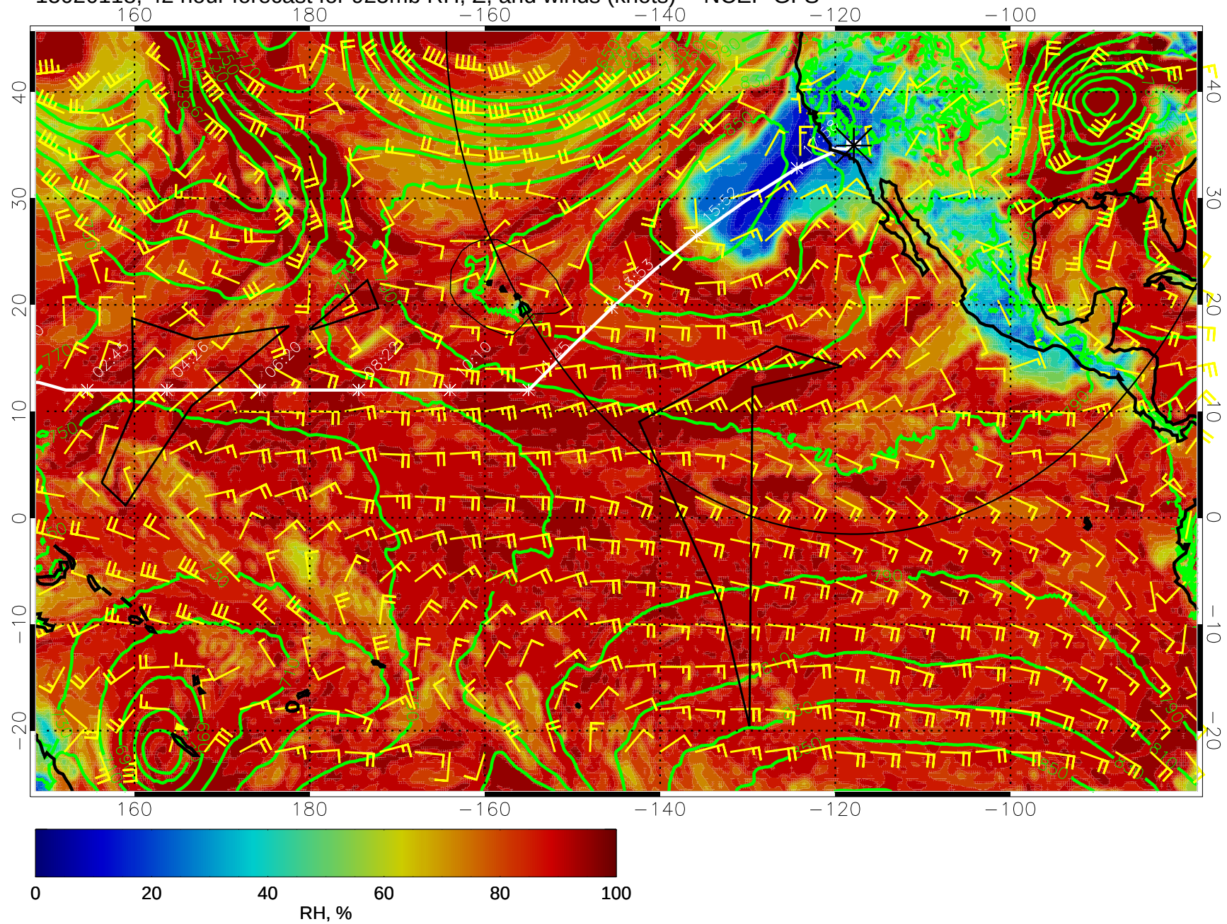
15020118, 42 hour forecast for 925mb RH, Z, and winds (knots) -- NCEP GFS
