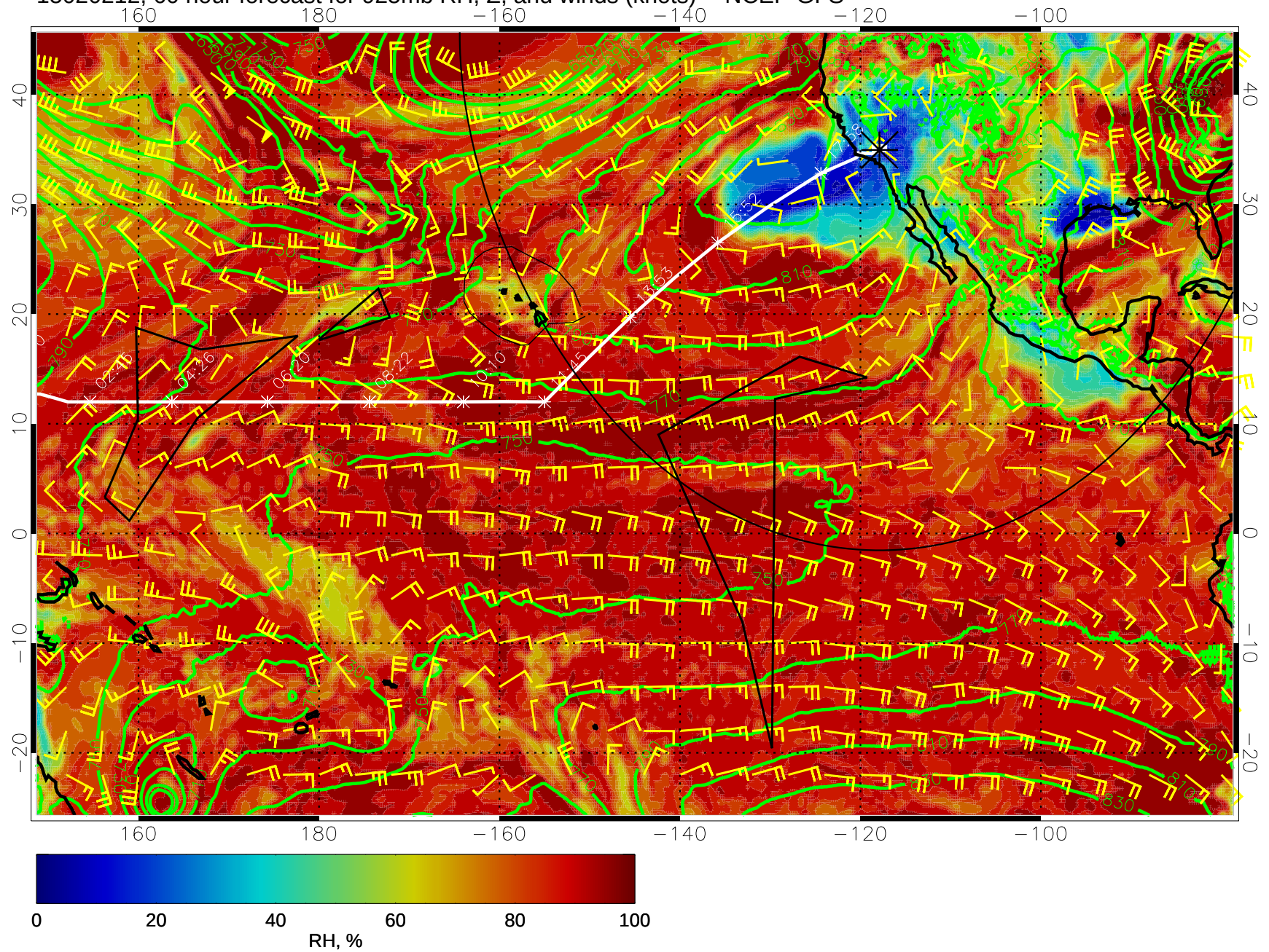
15020212, 60 hour forecast for 925mb RH, Z, and winds (knots) -- NCEP GFS
