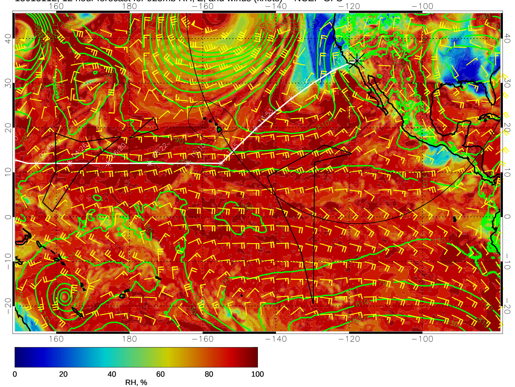
15013112, 12 hour forecast for 925mb RH, Z, and winds (knots) -- NCEP GFS
