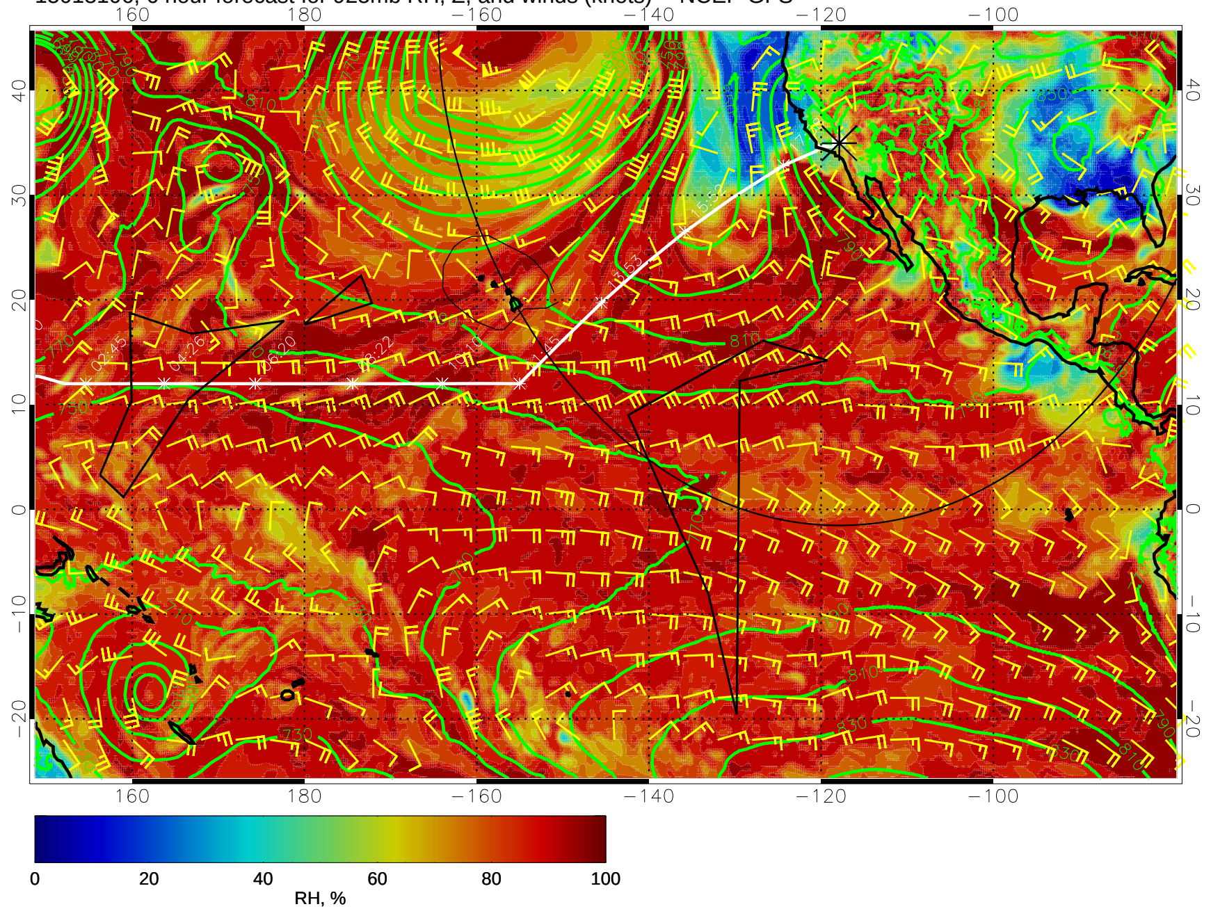
15013106, 6 hour forecast for 925mb RH, Z, and winds (knots) -- NCEP GFS
