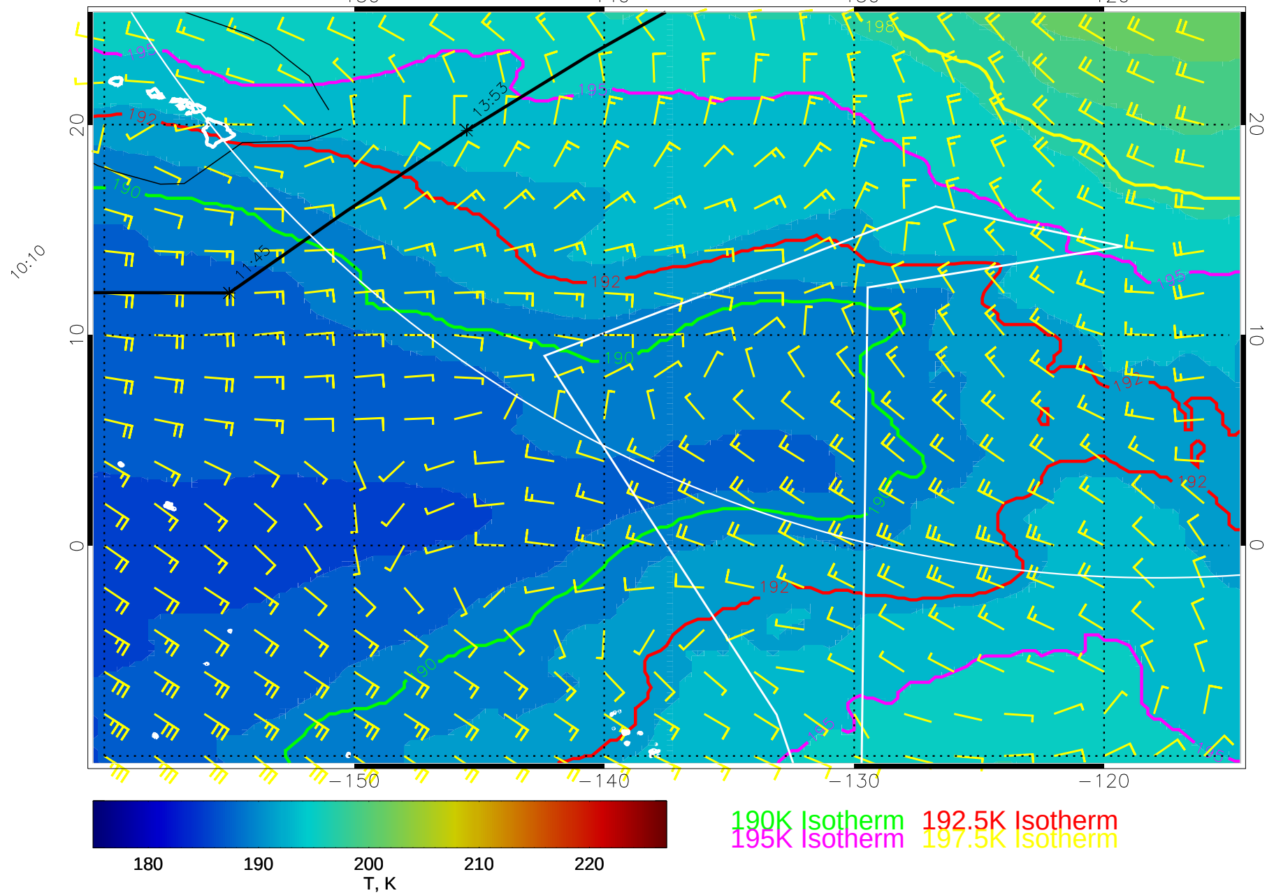
15020500, 120 hour forecast for 70mb T and winds (knots) -- NCEP GFS
