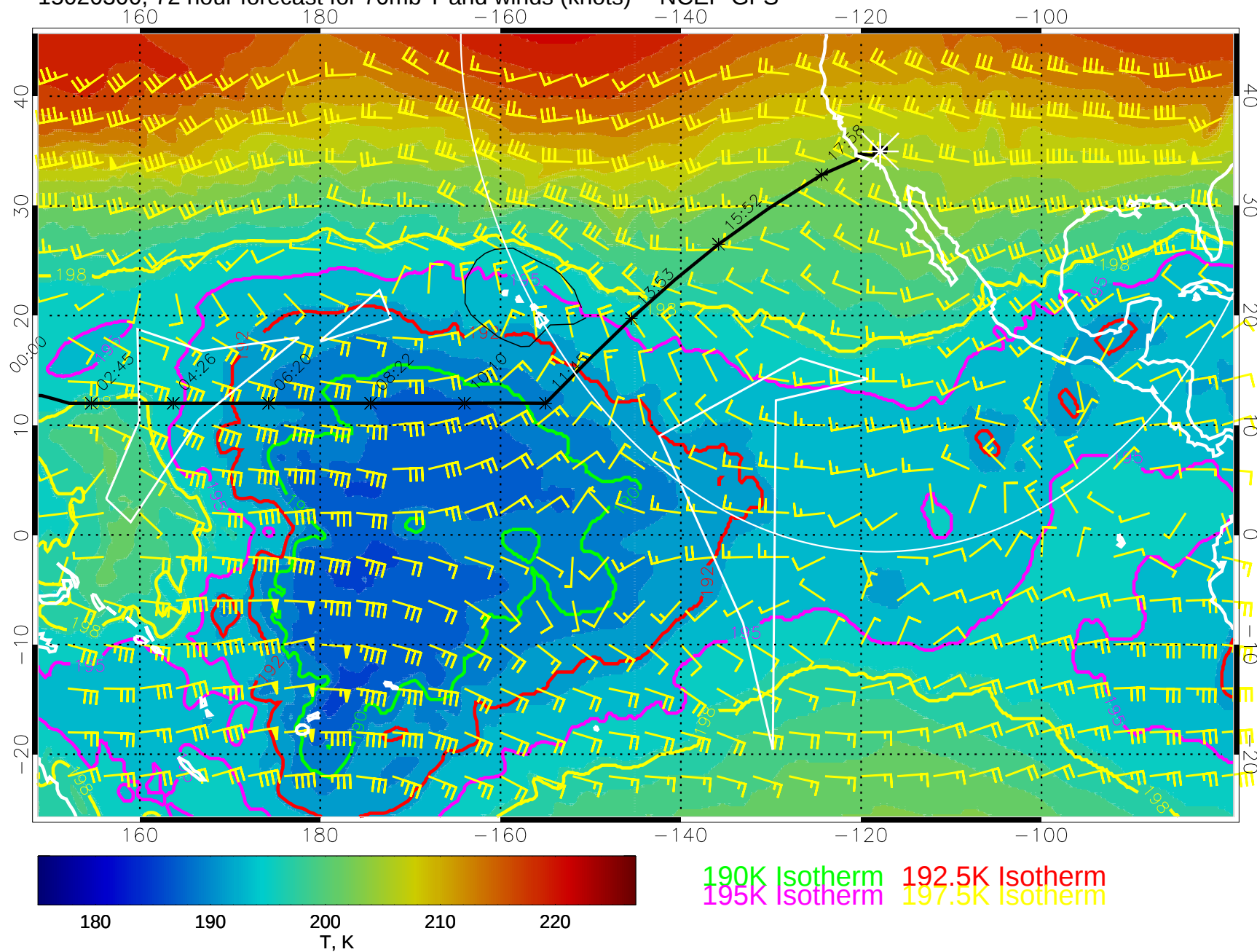
15020300, 72 hour forecast for 70mb T and winds (knots) -- NCEP GFS
