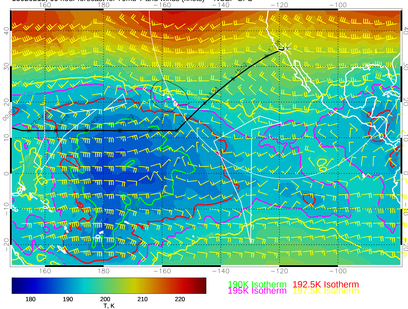
15020212, 60 hour forecast for 70mb T and winds (knots) -- NCEP GFS
