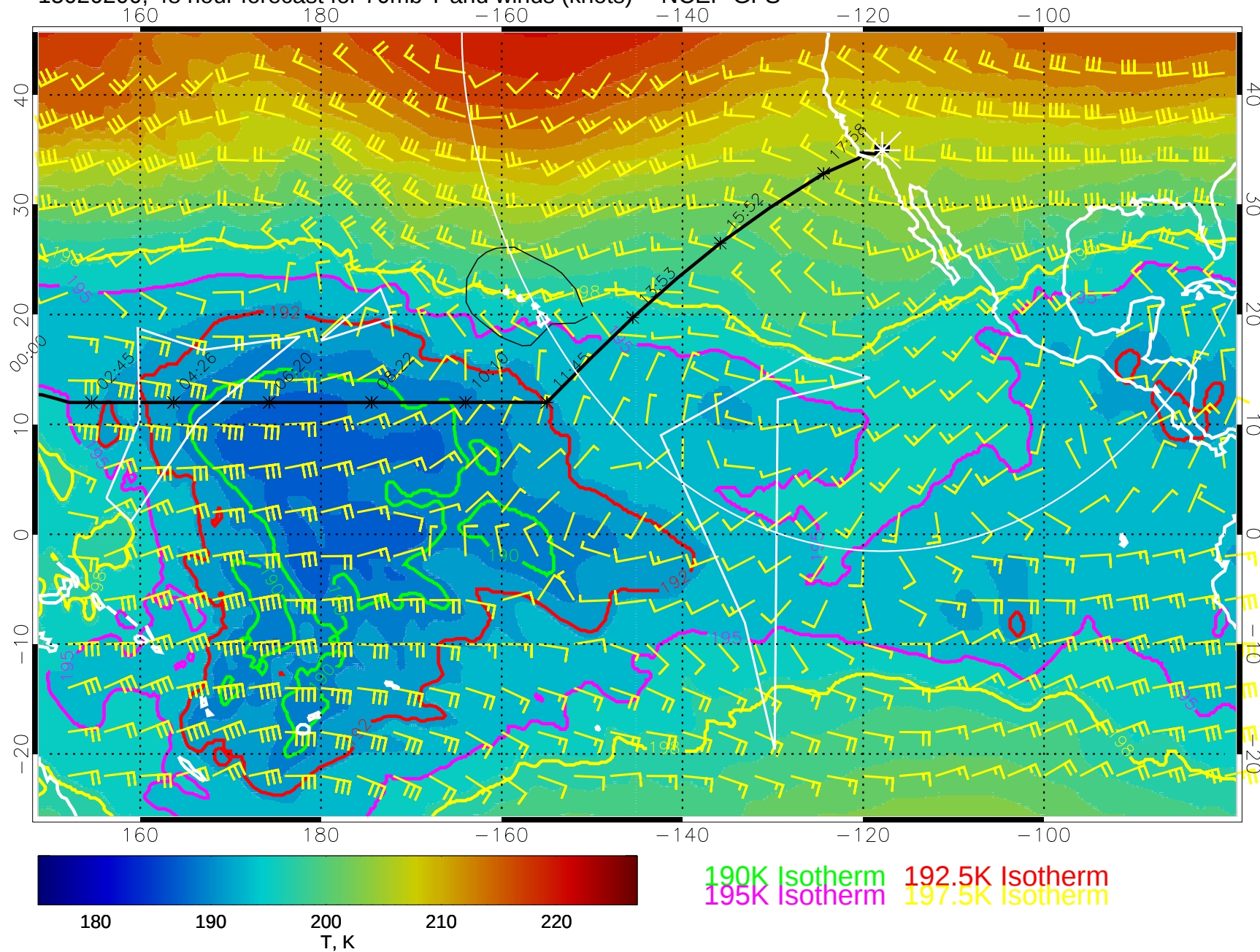
15020200, 48 hour forecast for 70mb T and winds (knots) -- NCEP GFS
