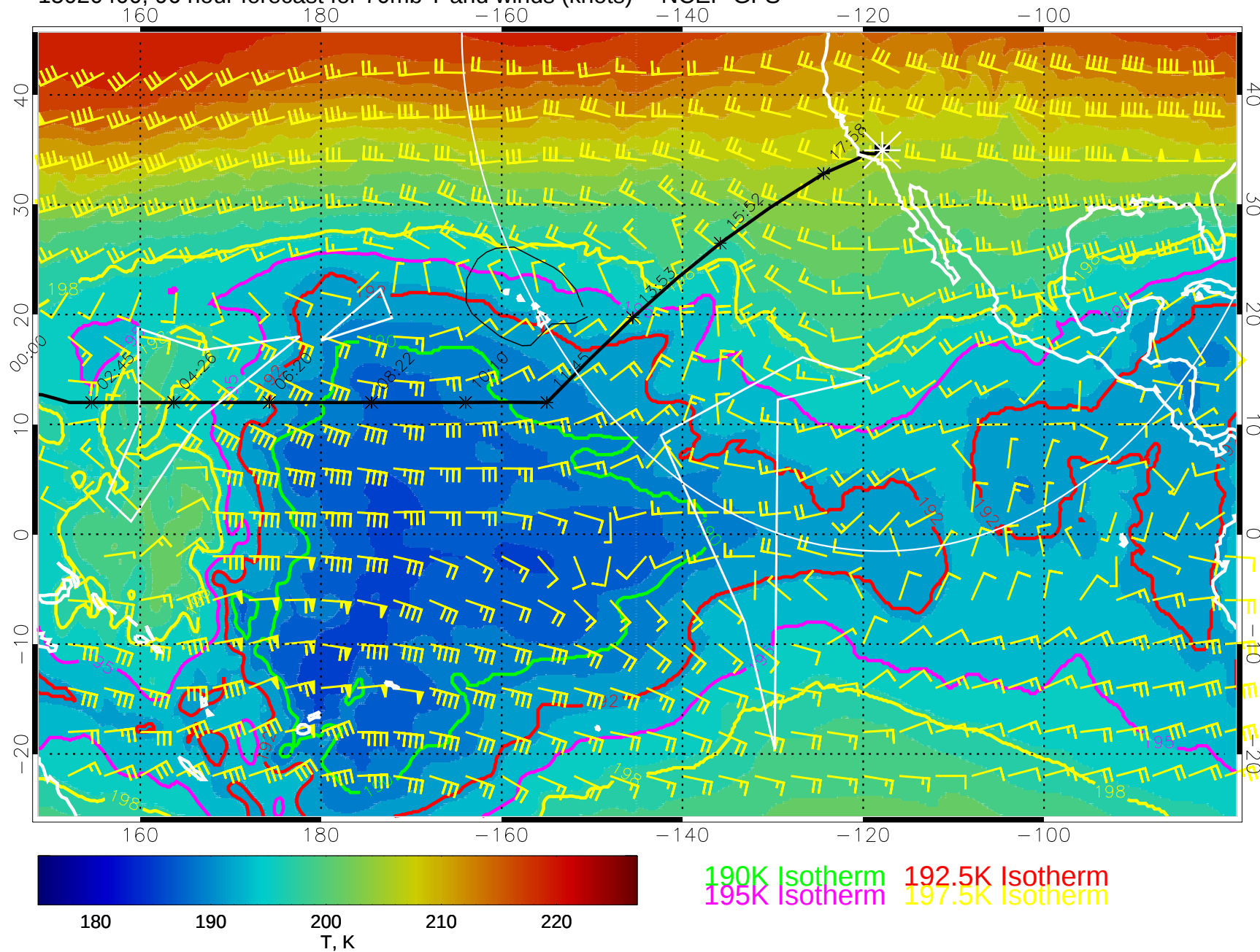
15020400, 96 hour forecast for 70mb T and winds (knots) -- NCEP GFS
