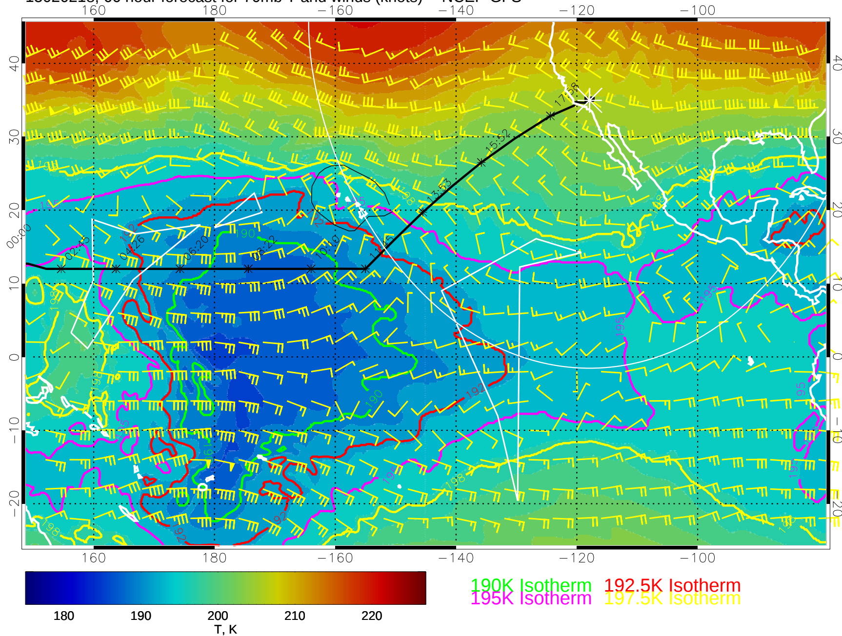
15020218, 66 hour forecast for 70mb T and winds (knots) -- NCEP GFS
