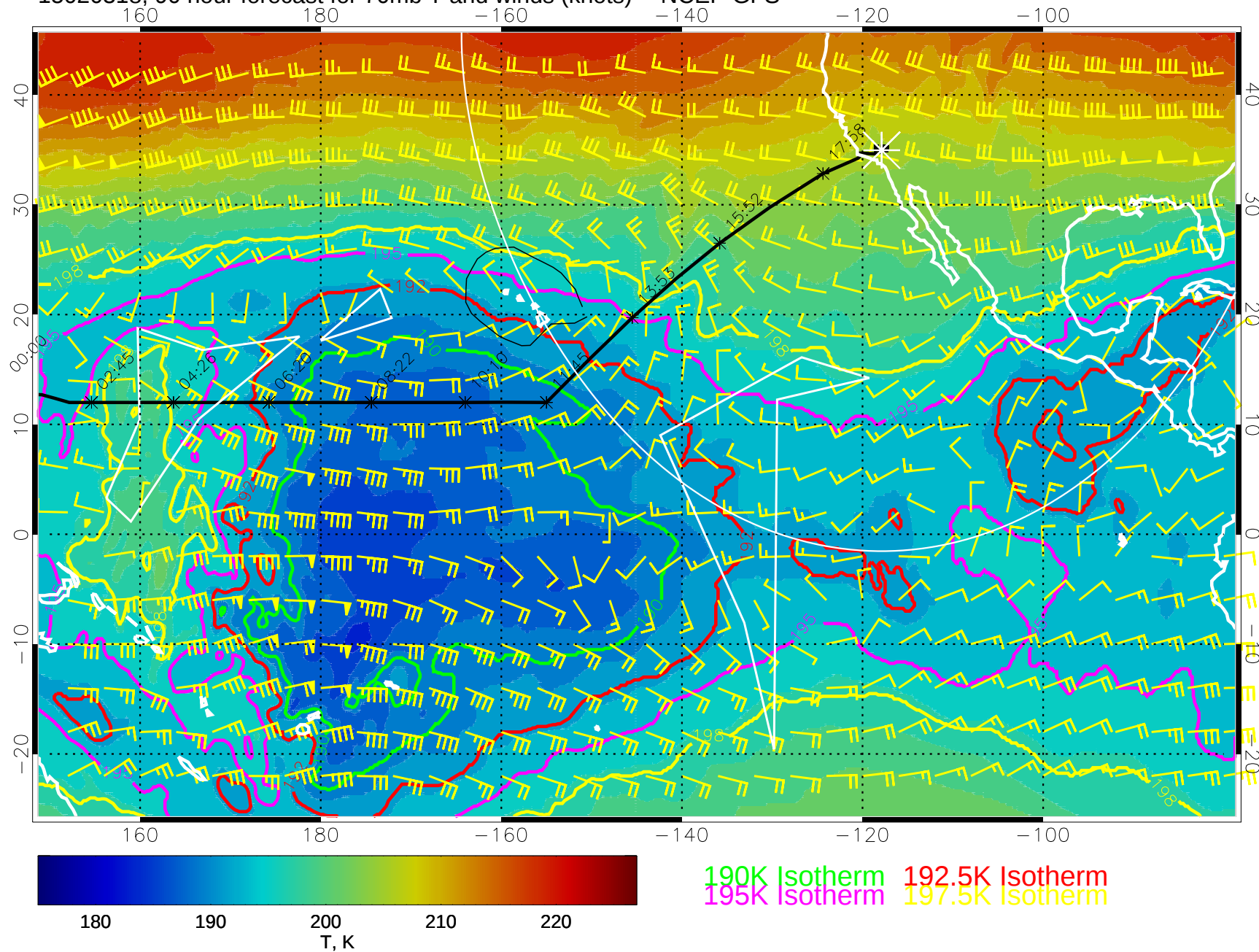
15020318, 90 hour forecast for 70mb T and winds (knots) -- NCEP GFS
