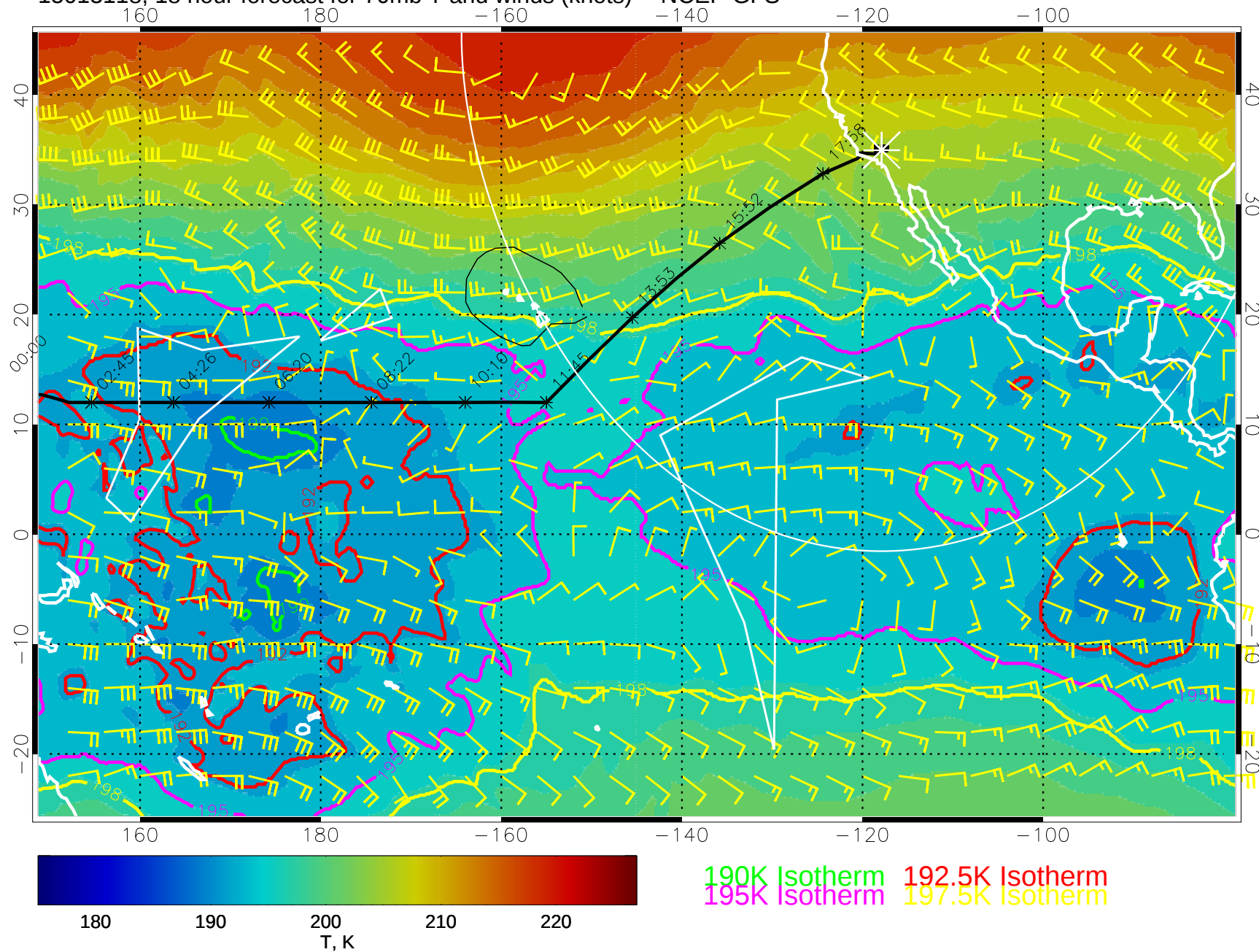
15013118, 18 hour forecast for 70mb T and winds (knots) -- NCEP GFS
