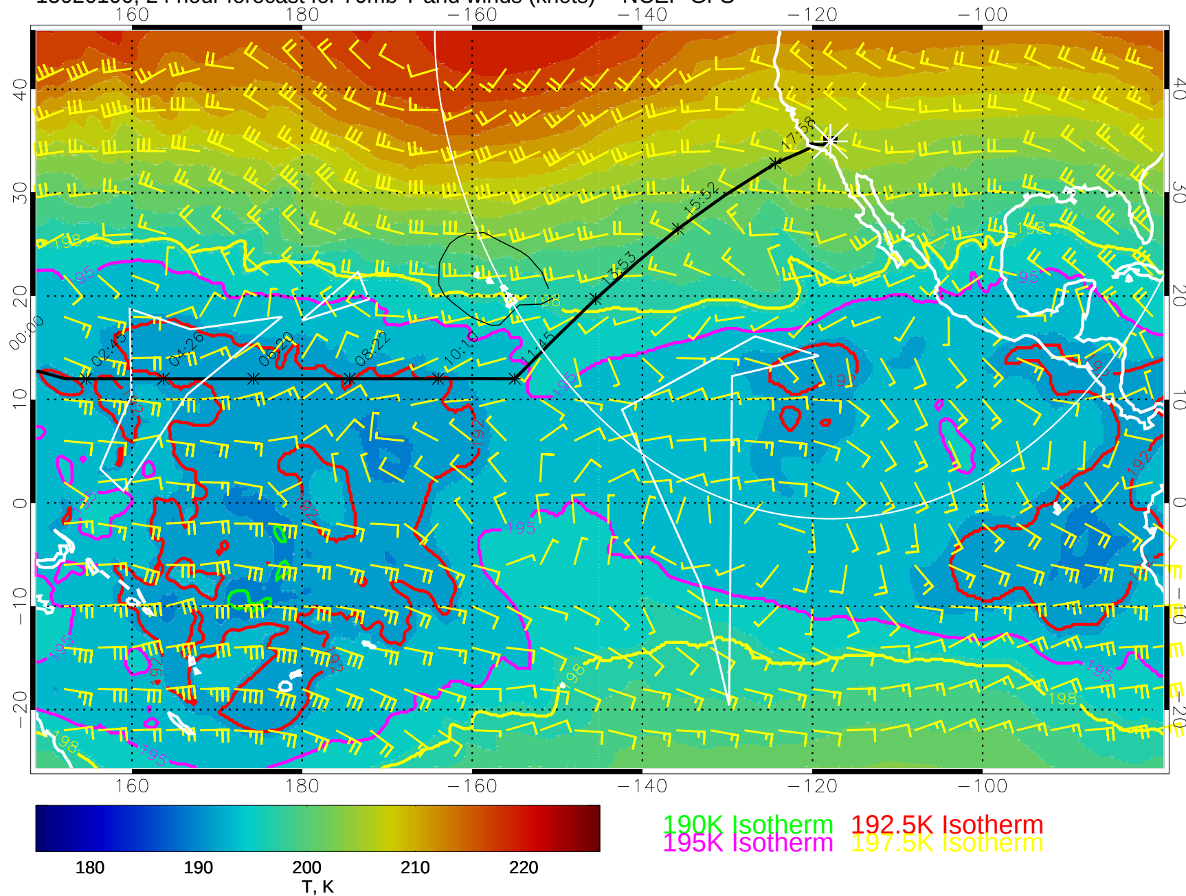
15020100, 24 hour forecast for 70mb T and winds (knots) -- NCEP GFS
