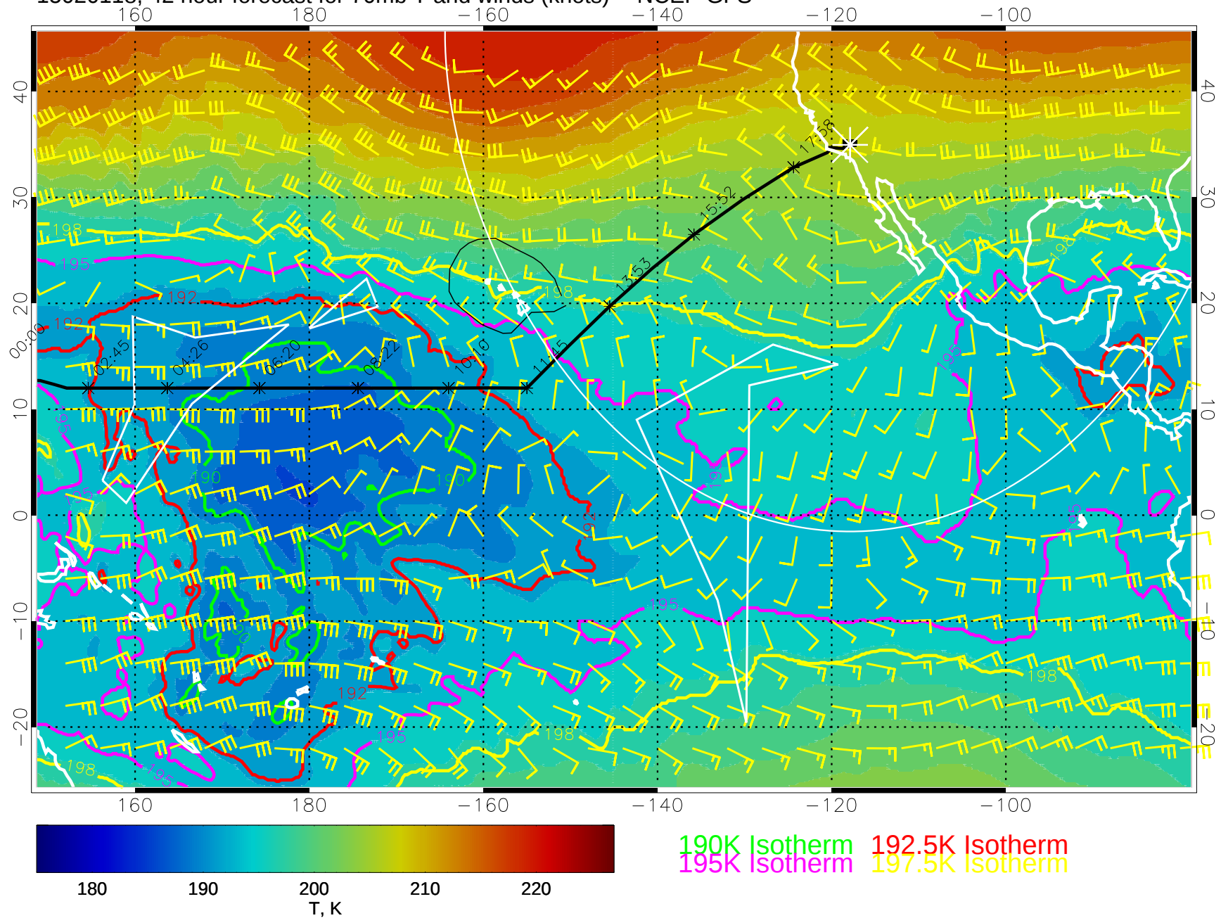
15020118, 42 hour forecast for 70mb T and winds (knots) -- NCEP GFS
