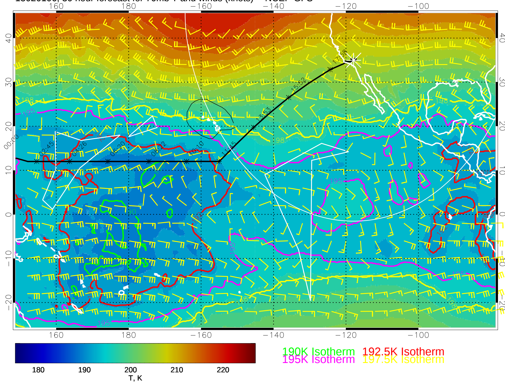
15020106, 30 hour forecast for 70mb T and winds (knots) -- NCEP GFS
