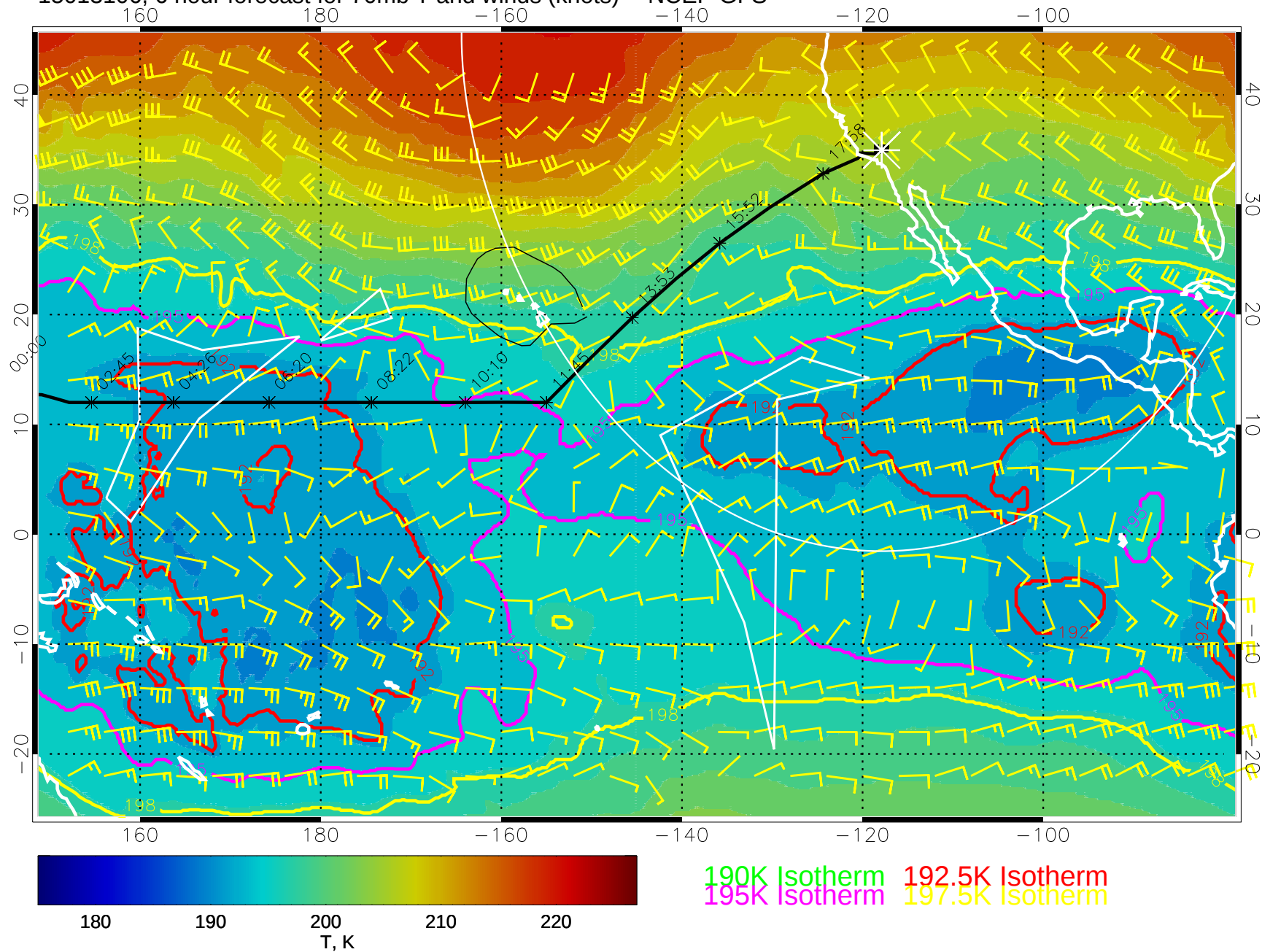
15013106, 6 hour forecast for 70mb T and winds (knots) -- NCEP GFS
