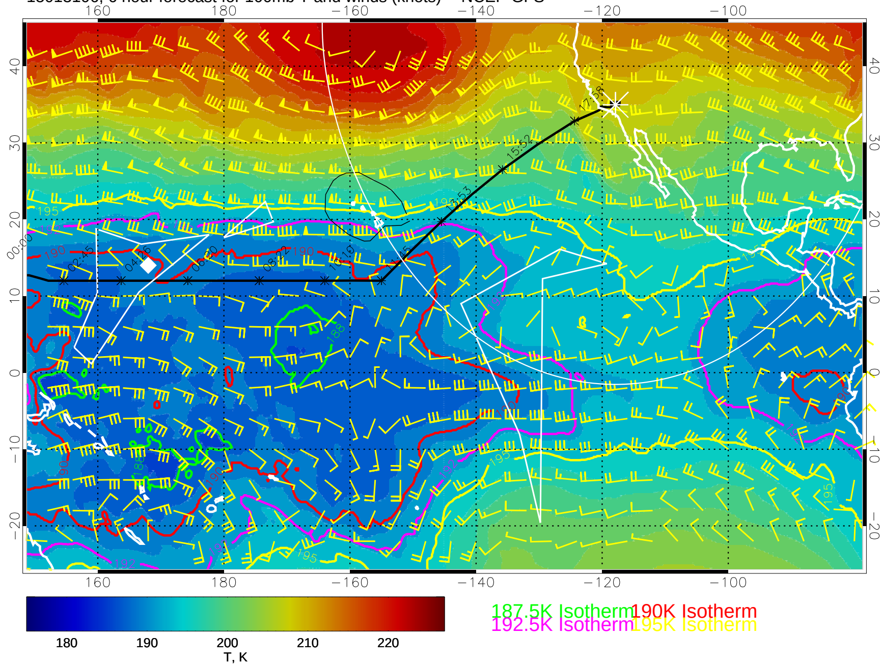
15013106, 6 hour forecast for 100mb T and winds (knots) -- NCEP GFS
