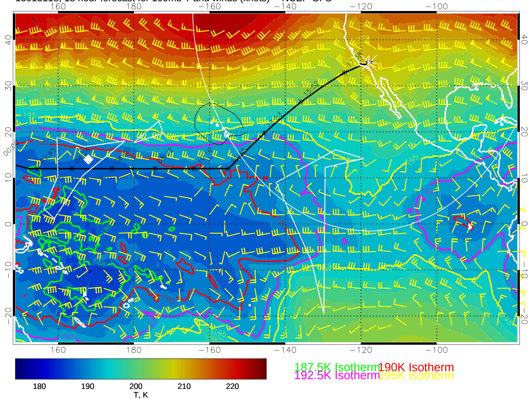
15013118, 18 hour forecast for 100mb T and winds (knots) -- NCEP GFS
