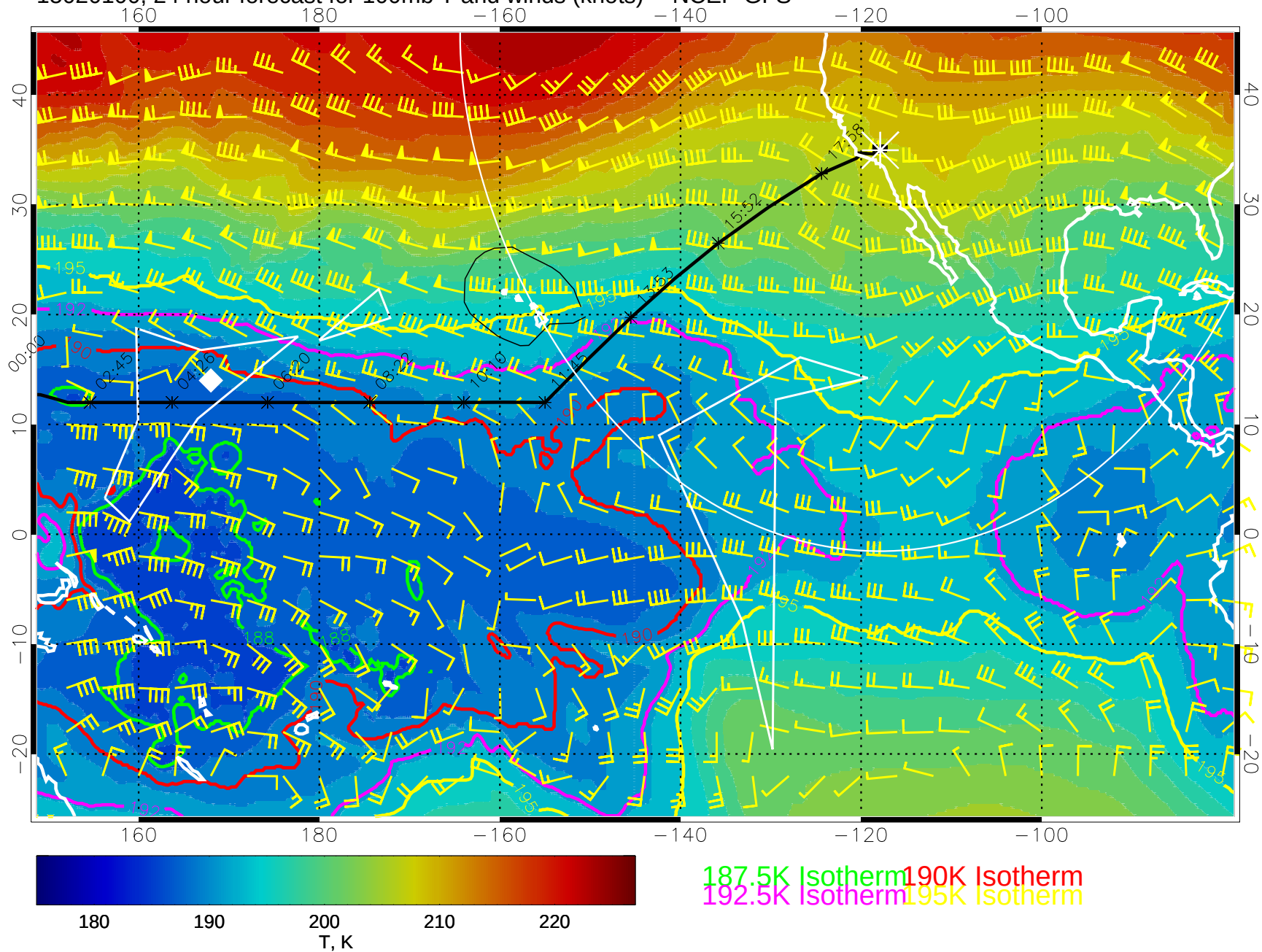
15020100, 24 hour forecast for 100mb T and winds (knots) -- NCEP GFS
