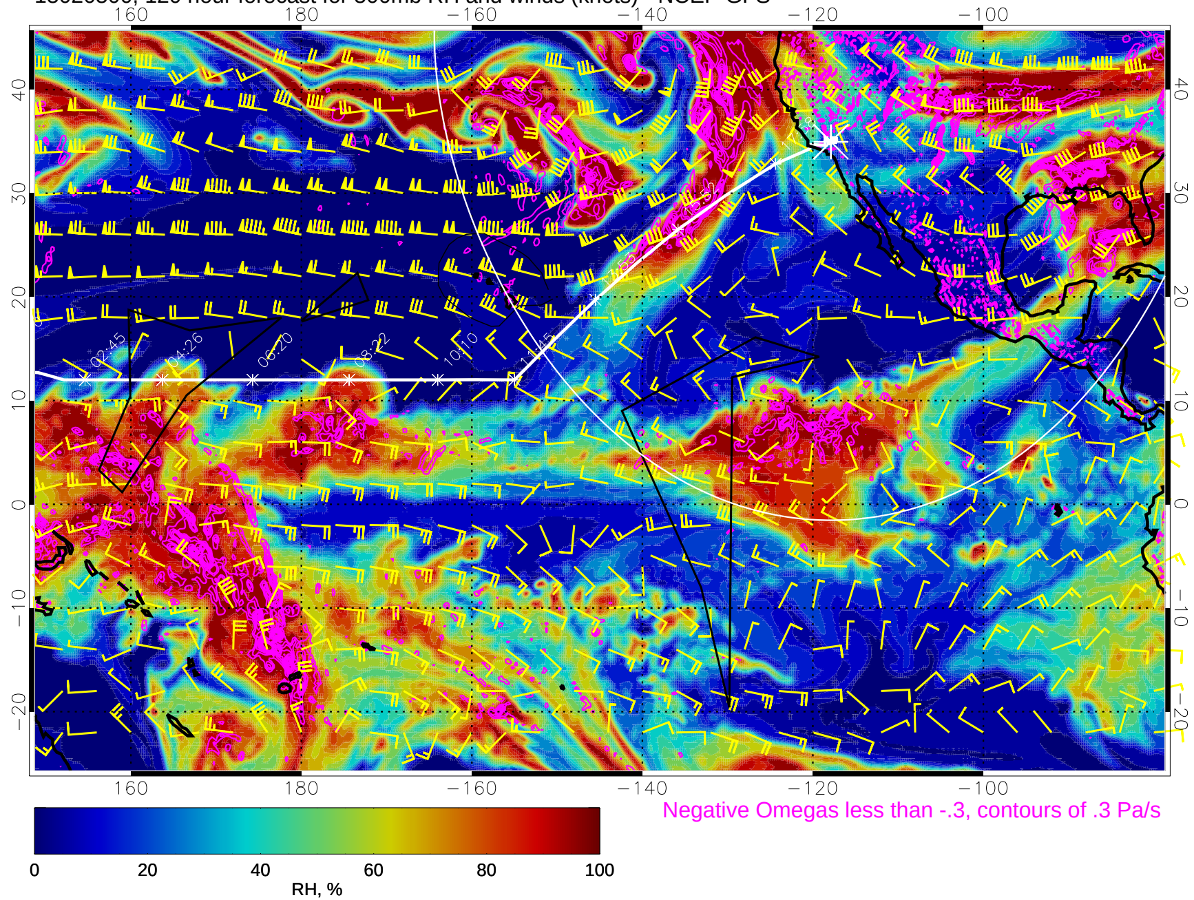
15020500, 120 hour forecast for 500mb RH and winds (knots) - NCEP GFS
