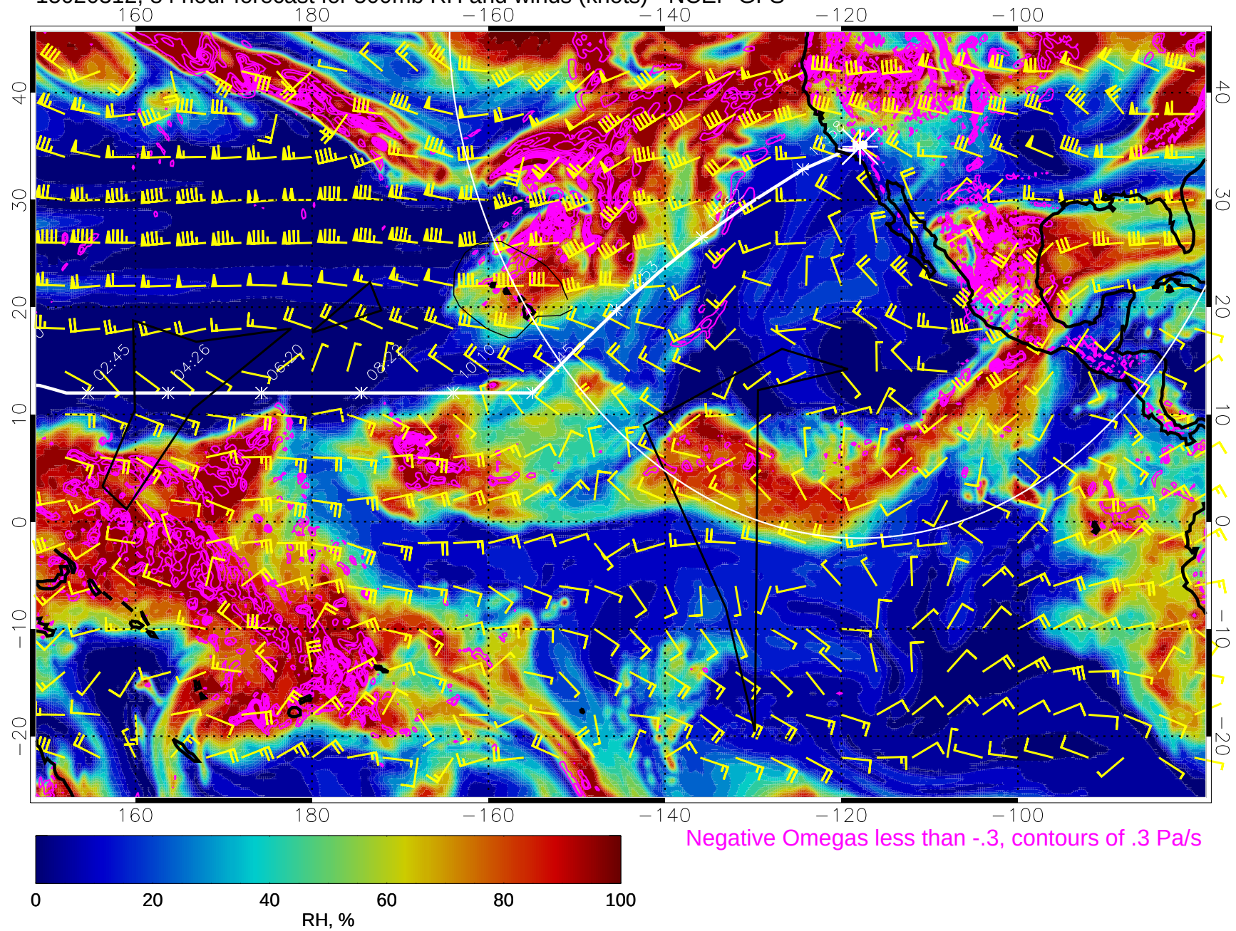
15020312, 84 hour forecast for 500mb RH and winds (knots) - NCEP GFS
