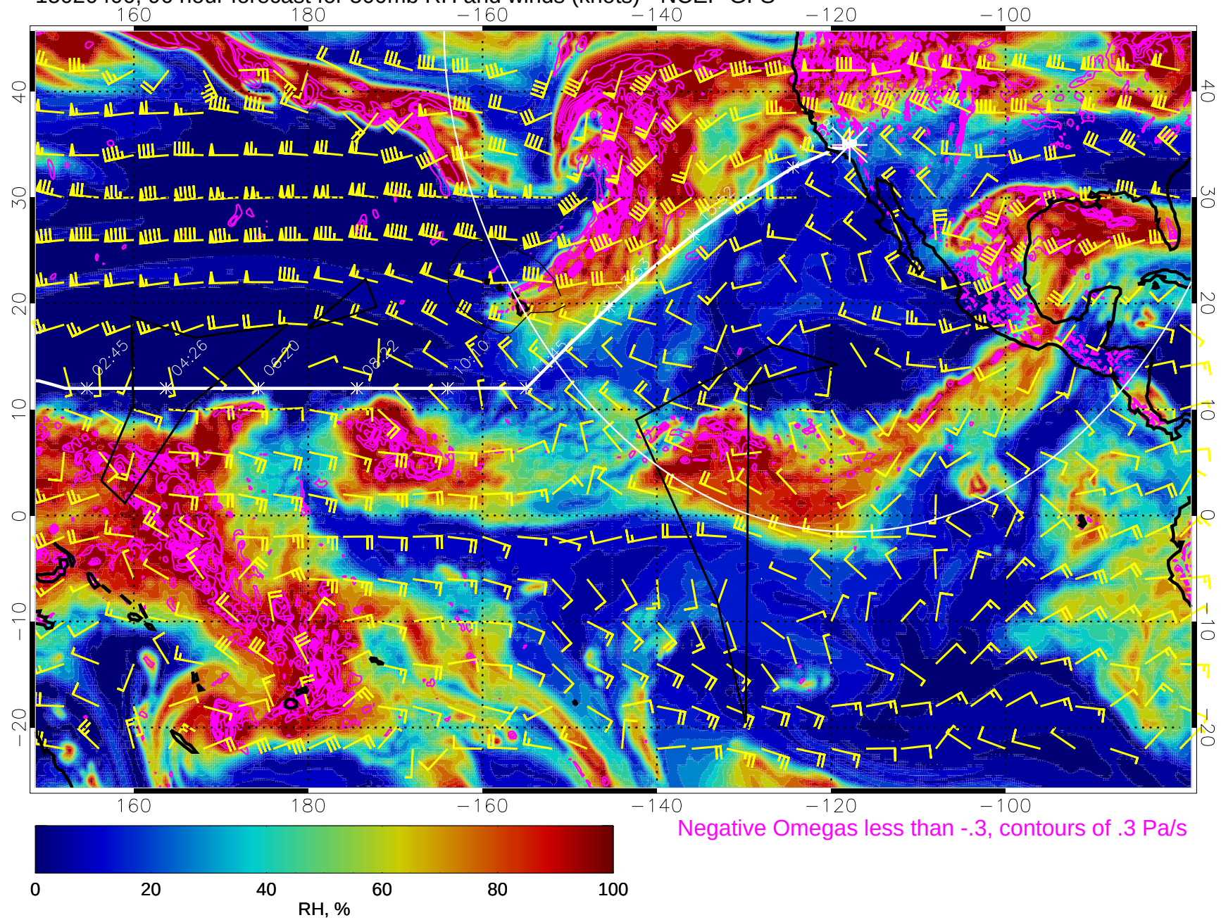
15020400, 96 hour forecast for 500mb RH and winds (knots) - NCEP GFS
