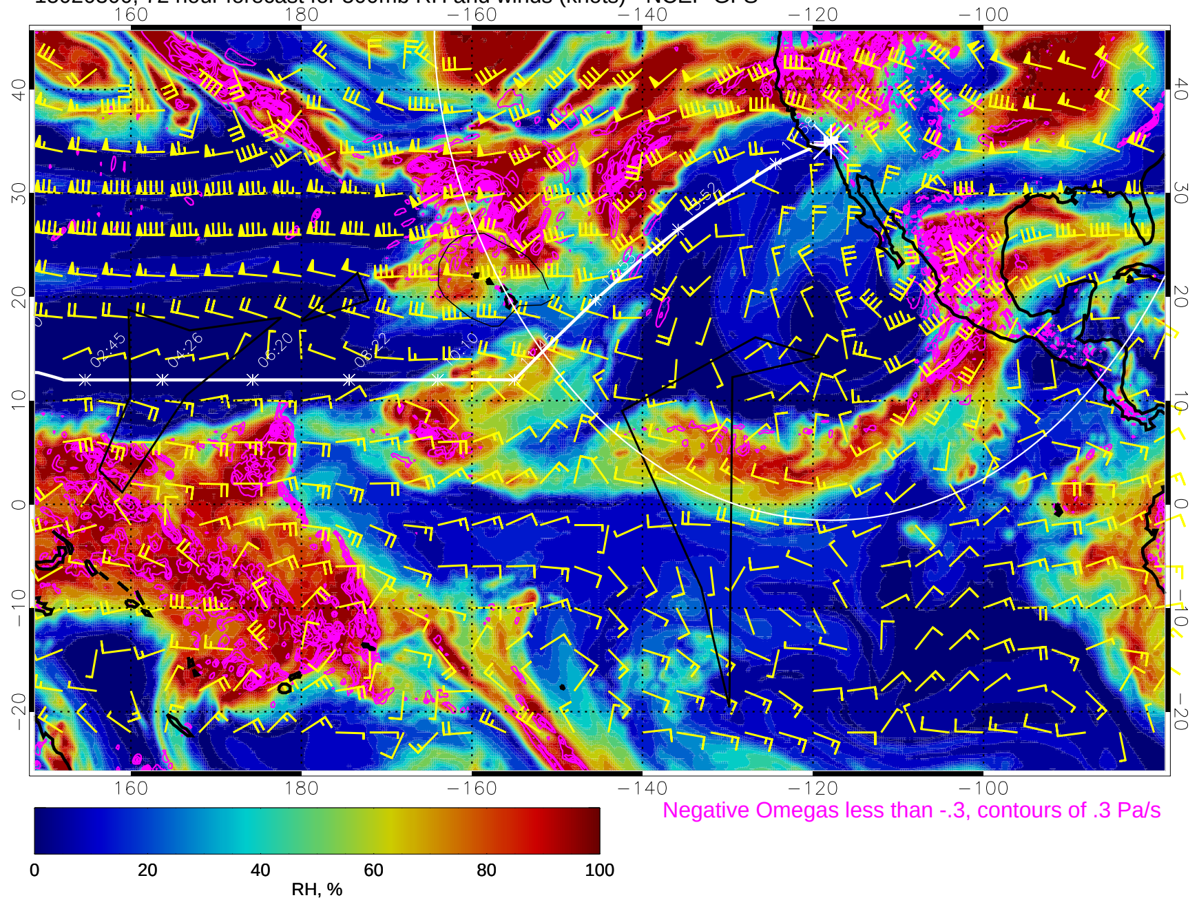
15020300, 72 hour forecast for 500mb RH and winds (knots) - NCEP GFS
