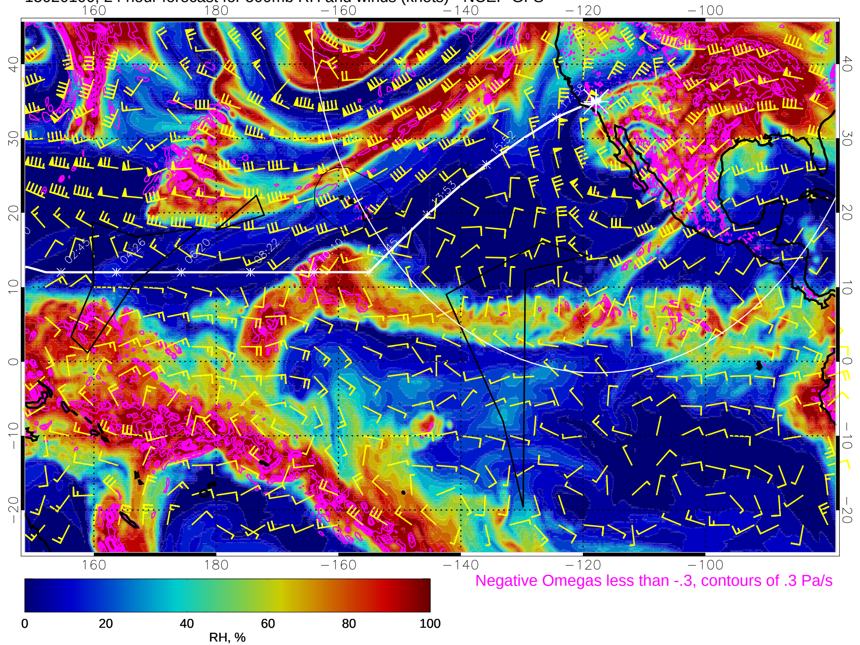
15020100, 24 hour forecast for 500mb RH and winds (knots) - NCEP GFS
