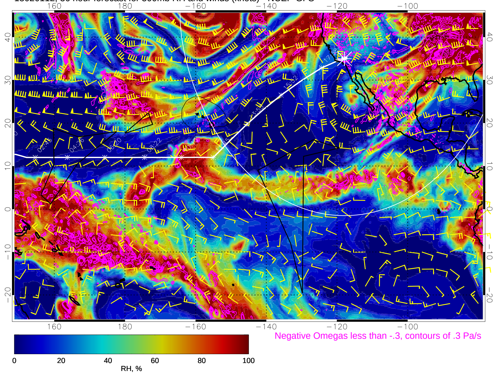
15020112, 36 hour forecast for 500mb RH and winds (knots) - NCEP GFS
