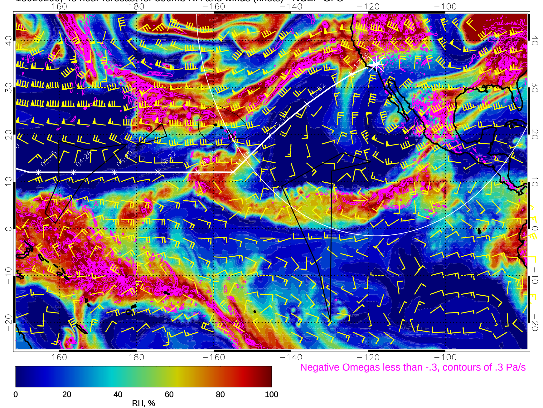
15020200, 48 hour forecast for 500mb RH and winds (knots) - NCEP GFS
