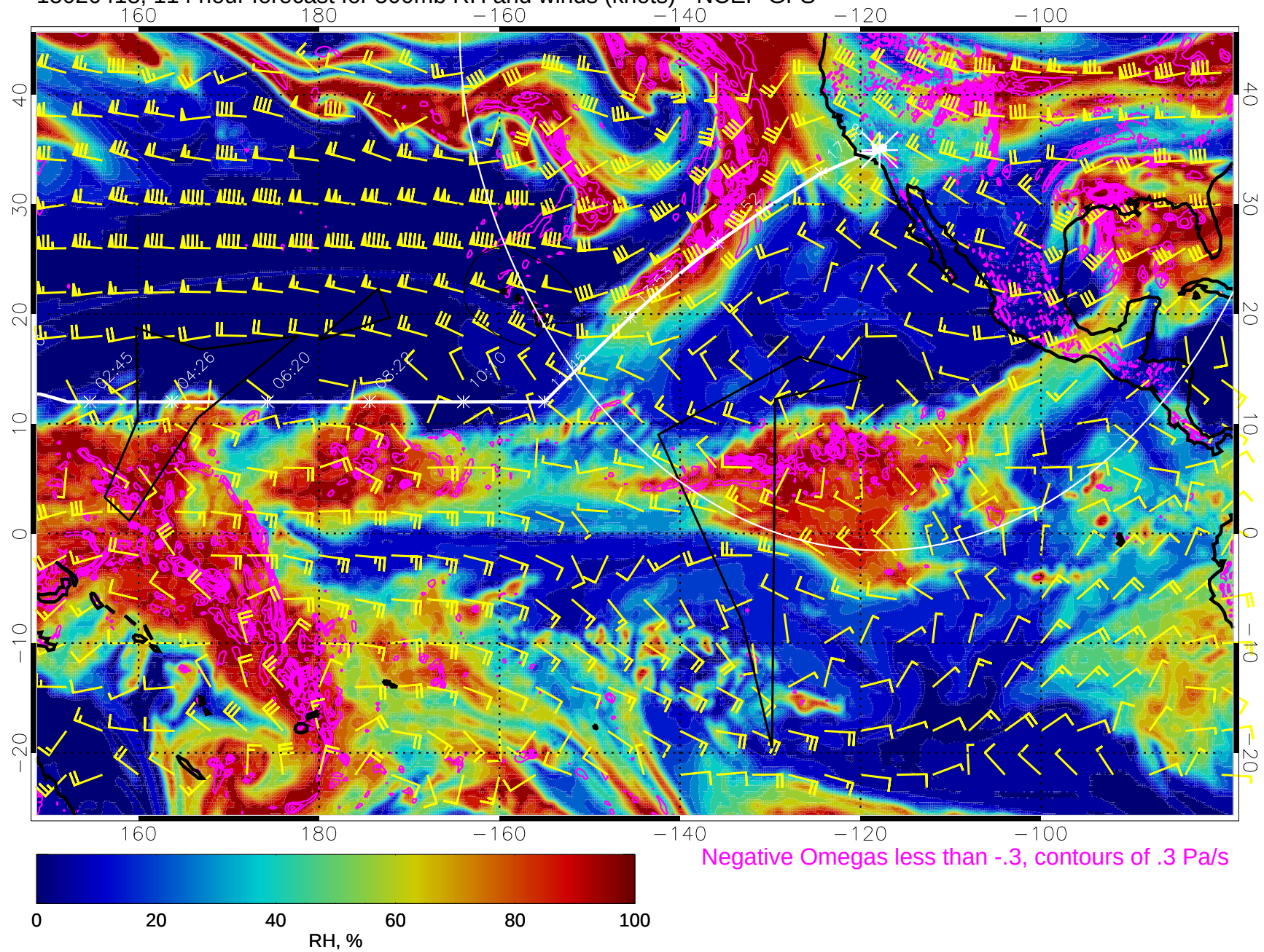
15020418, 114 hour forecast for 500mb RH and winds (knots) - NCEP GFS
