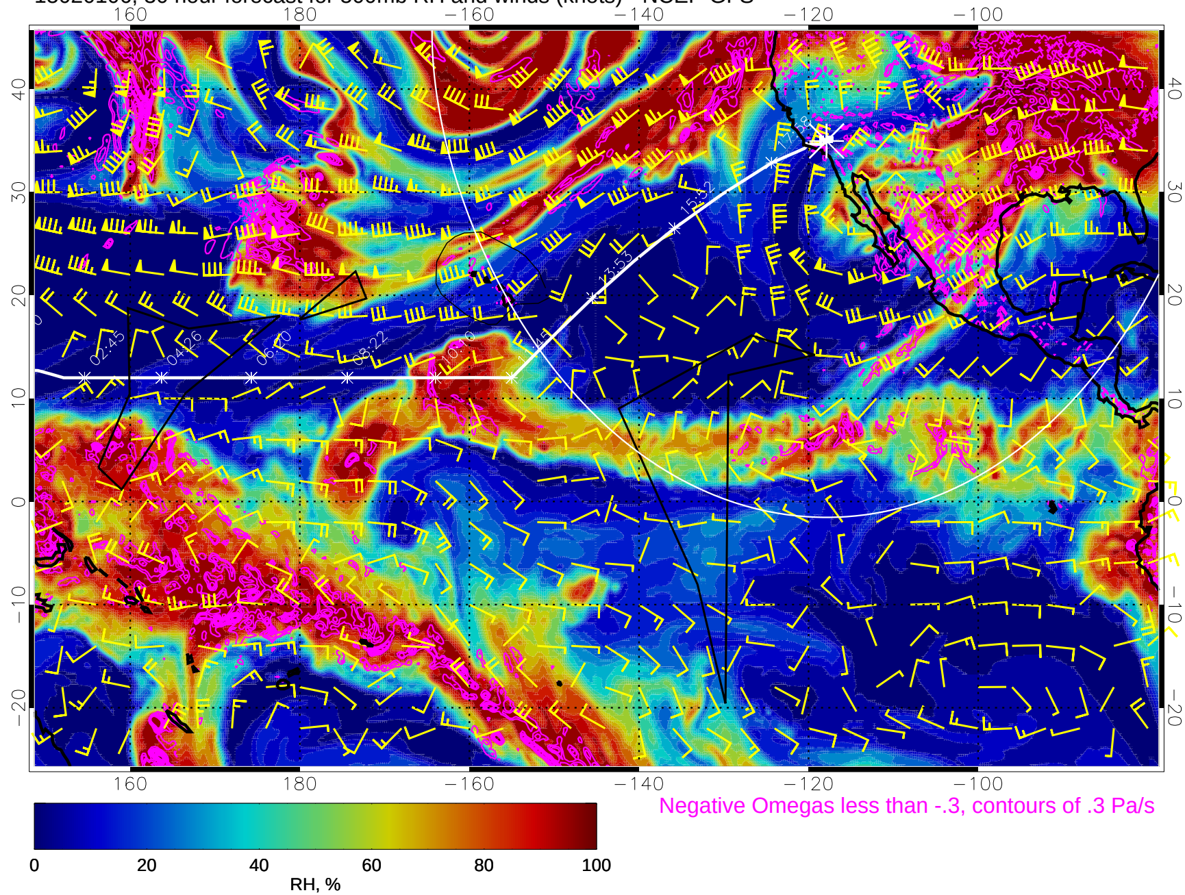
15020106, 30 hour forecast for 500mb RH and winds (knots) - NCEP GFS
