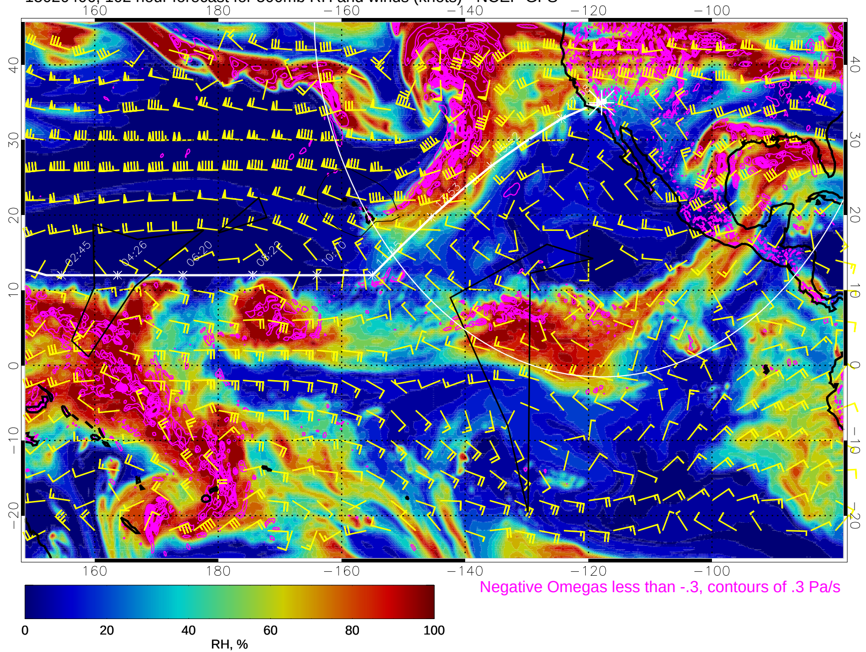
15020406, 102 hour forecast for 500mb RH and winds (knots) - NCEP GFS
