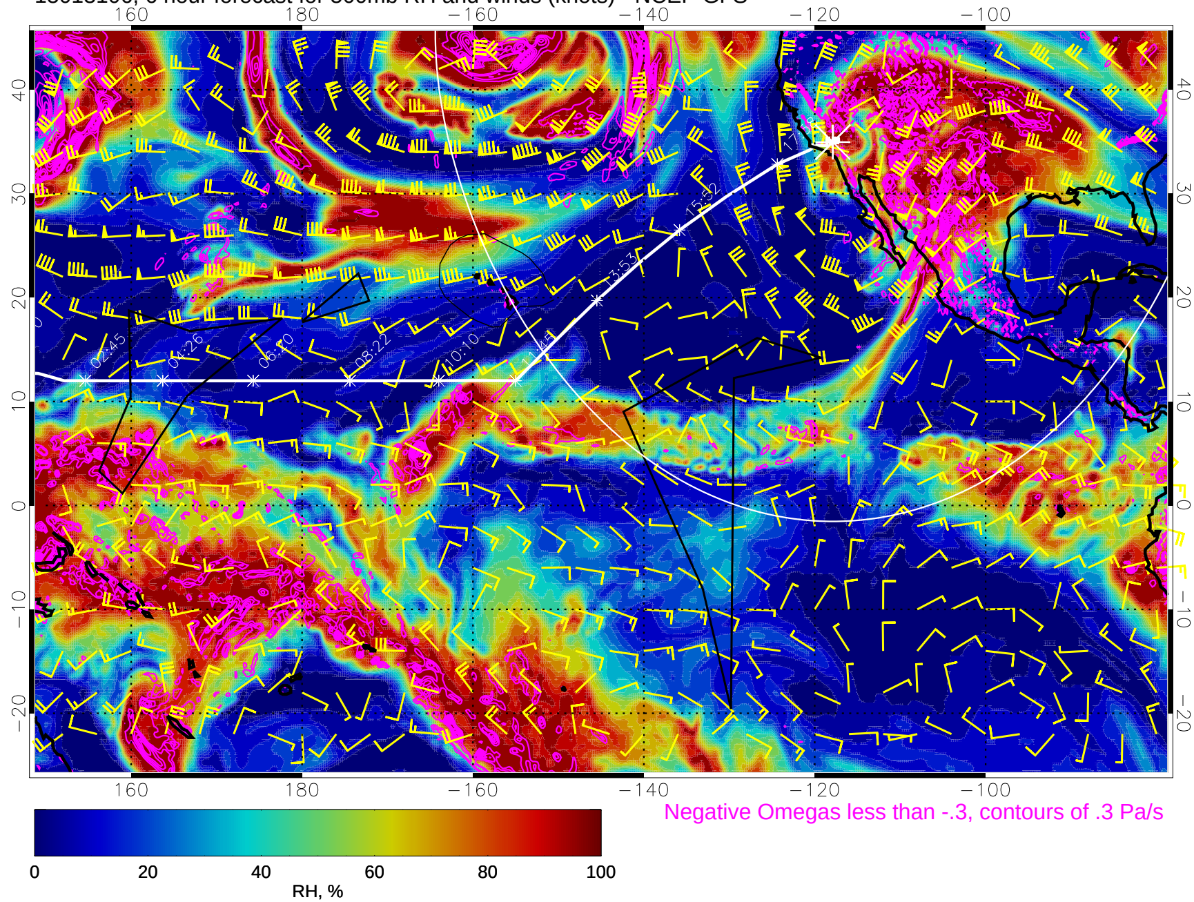
15013106, 6 hour forecast for 500mb RH and winds (knots) - NCEP GFS
