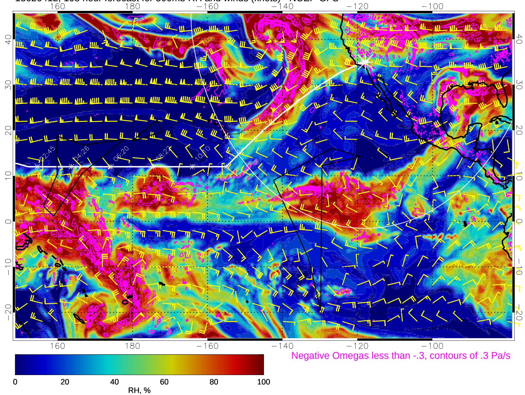
15020412, 108 hour forecast for 500mb RH and winds (knots) - NCEP GFS
