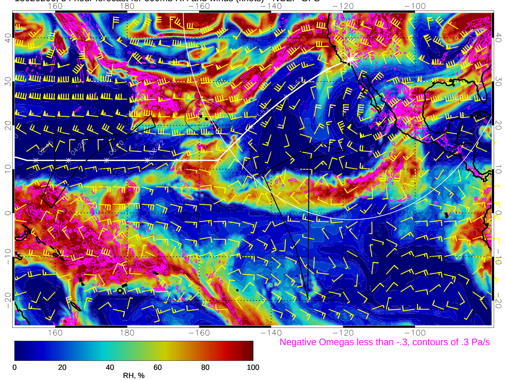
15020206, 54 hour forecast for 500mb RH and winds (knots) - NCEP GFS
