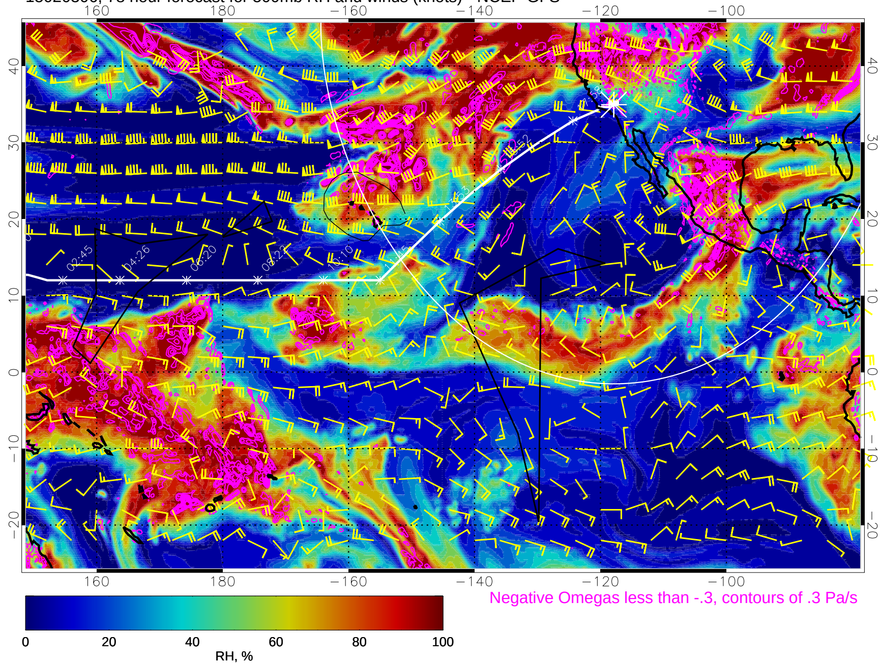
15020306, 78 hour forecast for 500mb RH and winds (knots) - NCEP GFS
