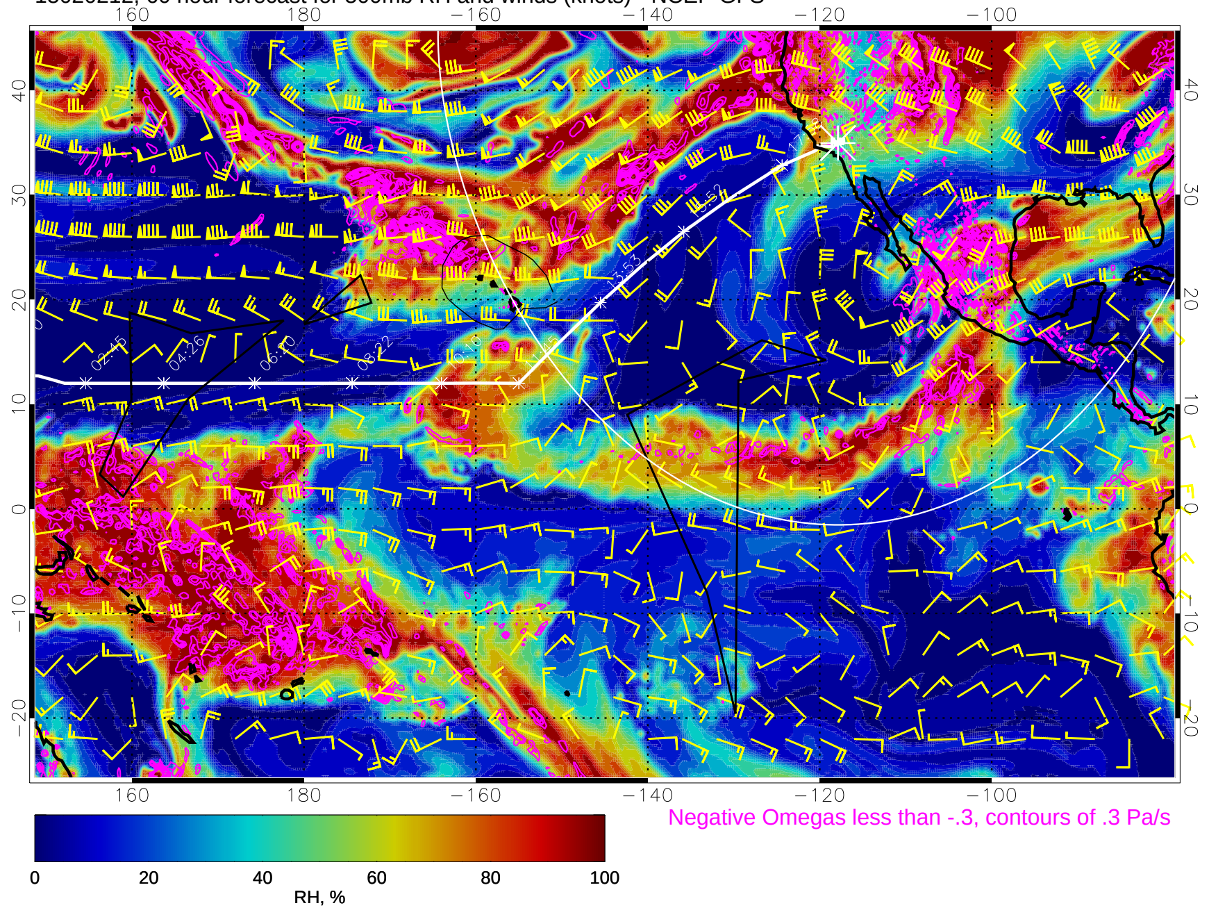
15020212, 60 hour forecast for 500mb RH and winds (knots) - NCEP GFS
