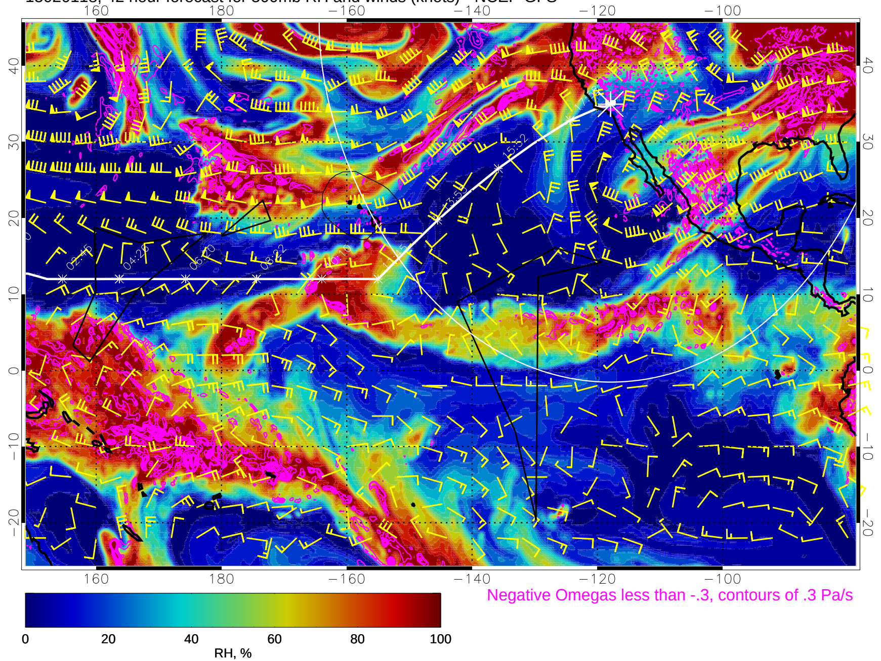
15020118, 42 hour forecast for 500mb RH and winds (knots) - NCEP GFS
