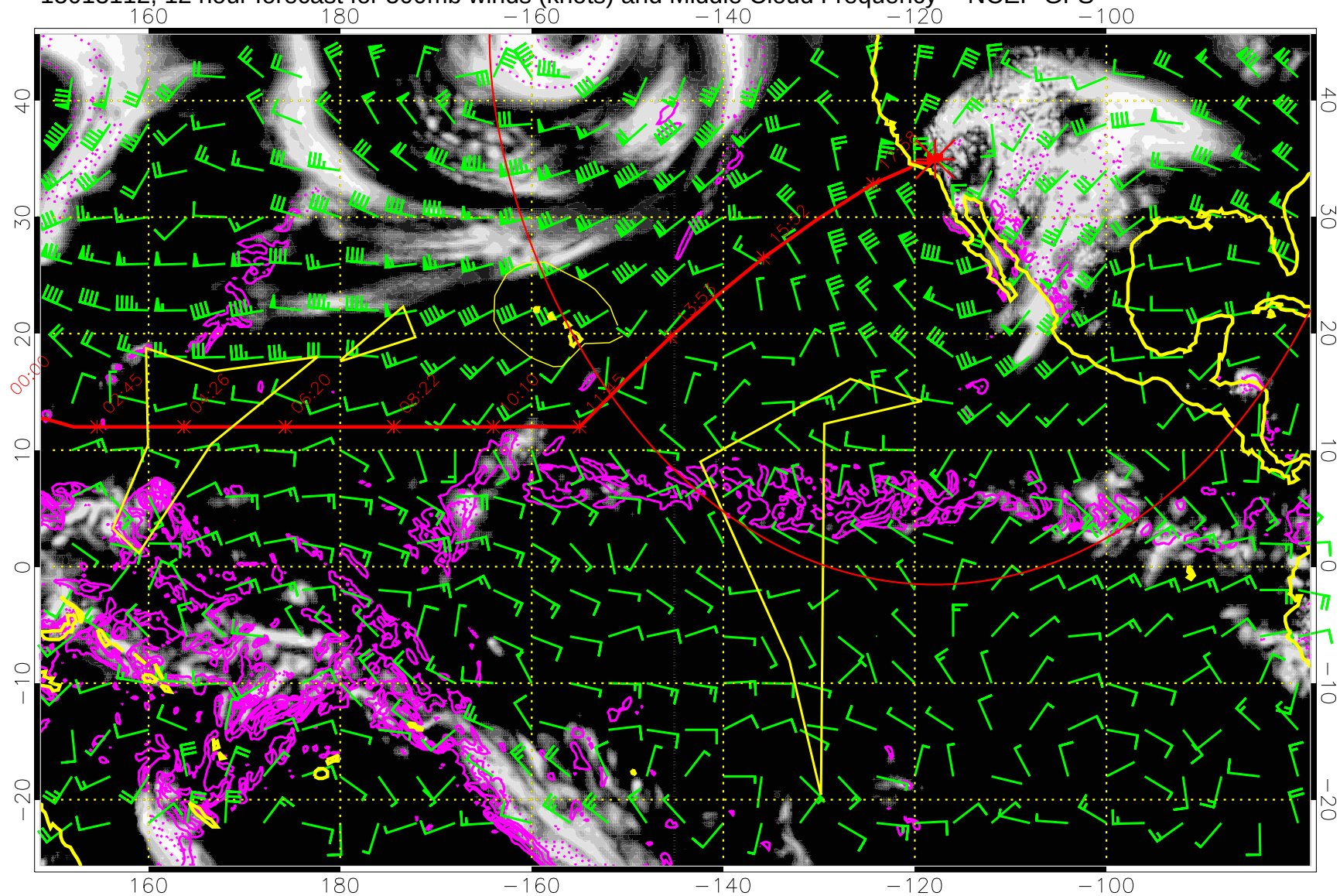
15013112, 12 hour forecast for 500mb winds (knots) and Middle Cloud Frequency -- NCEP GFS
