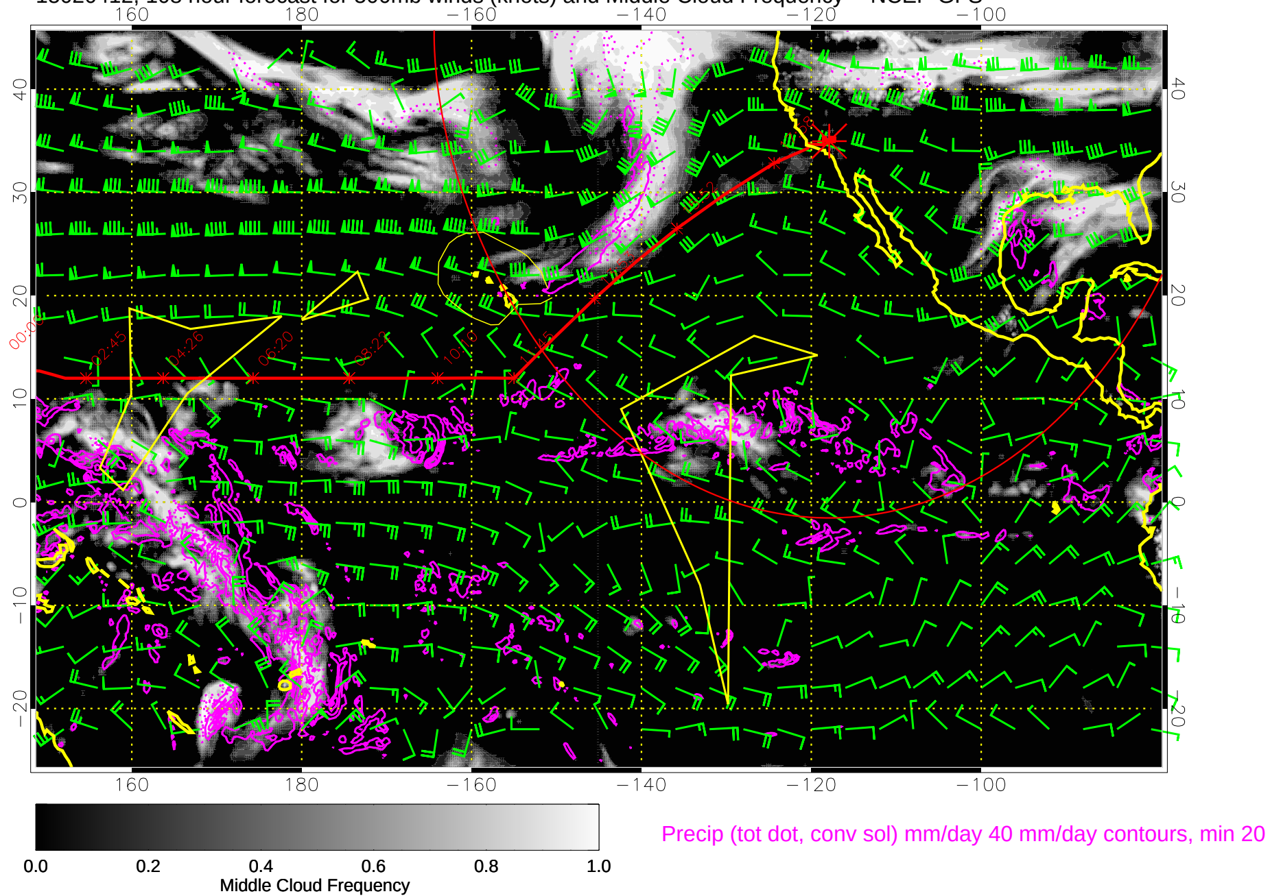
15020412, 108 hour forecast for 500mb winds (knots) and Middle Cloud Frequency -- NCEP GFS
