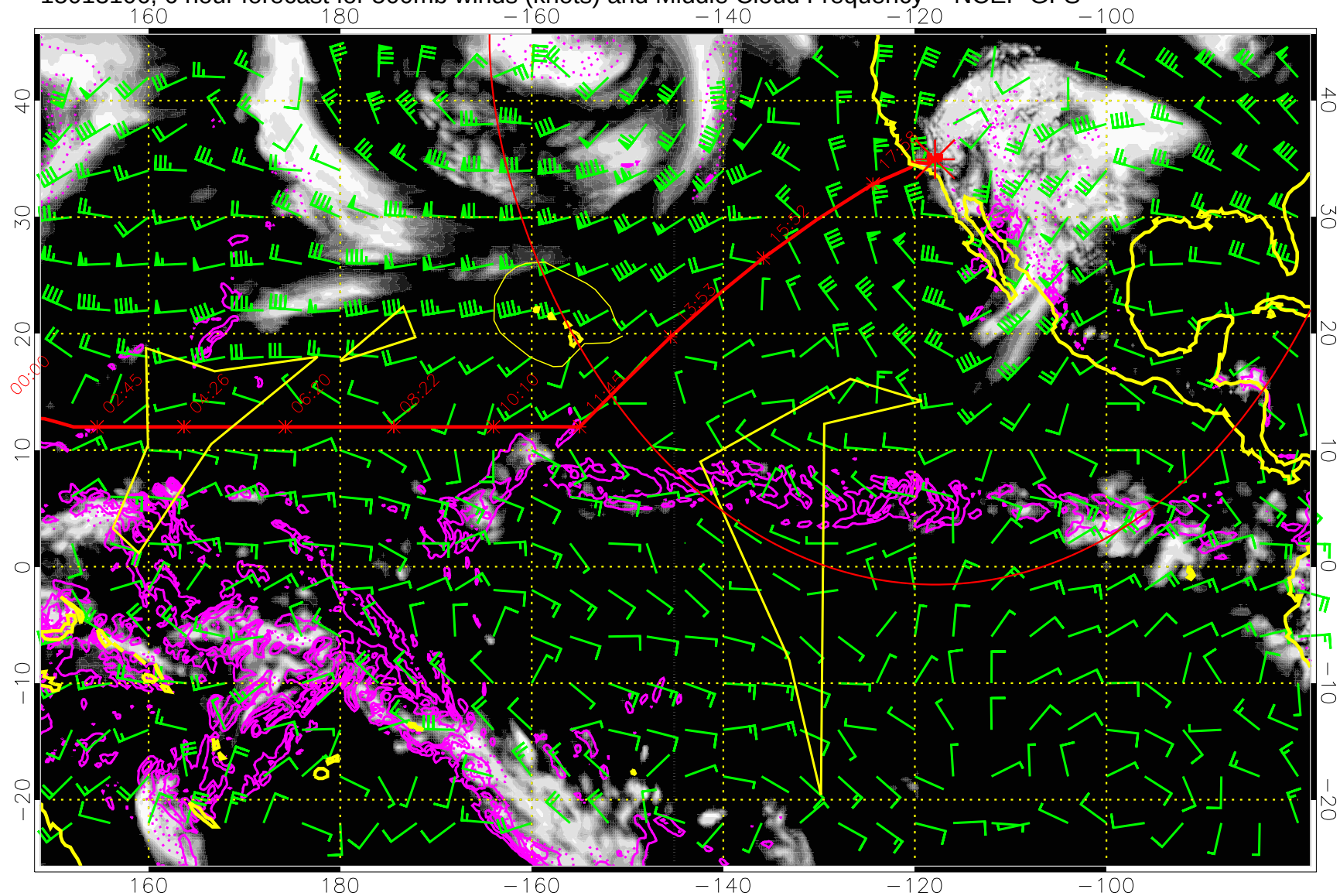
15013106, 6 hour forecast for 500mb winds (knots) and Middle Cloud Frequency -- NCEP GFS
