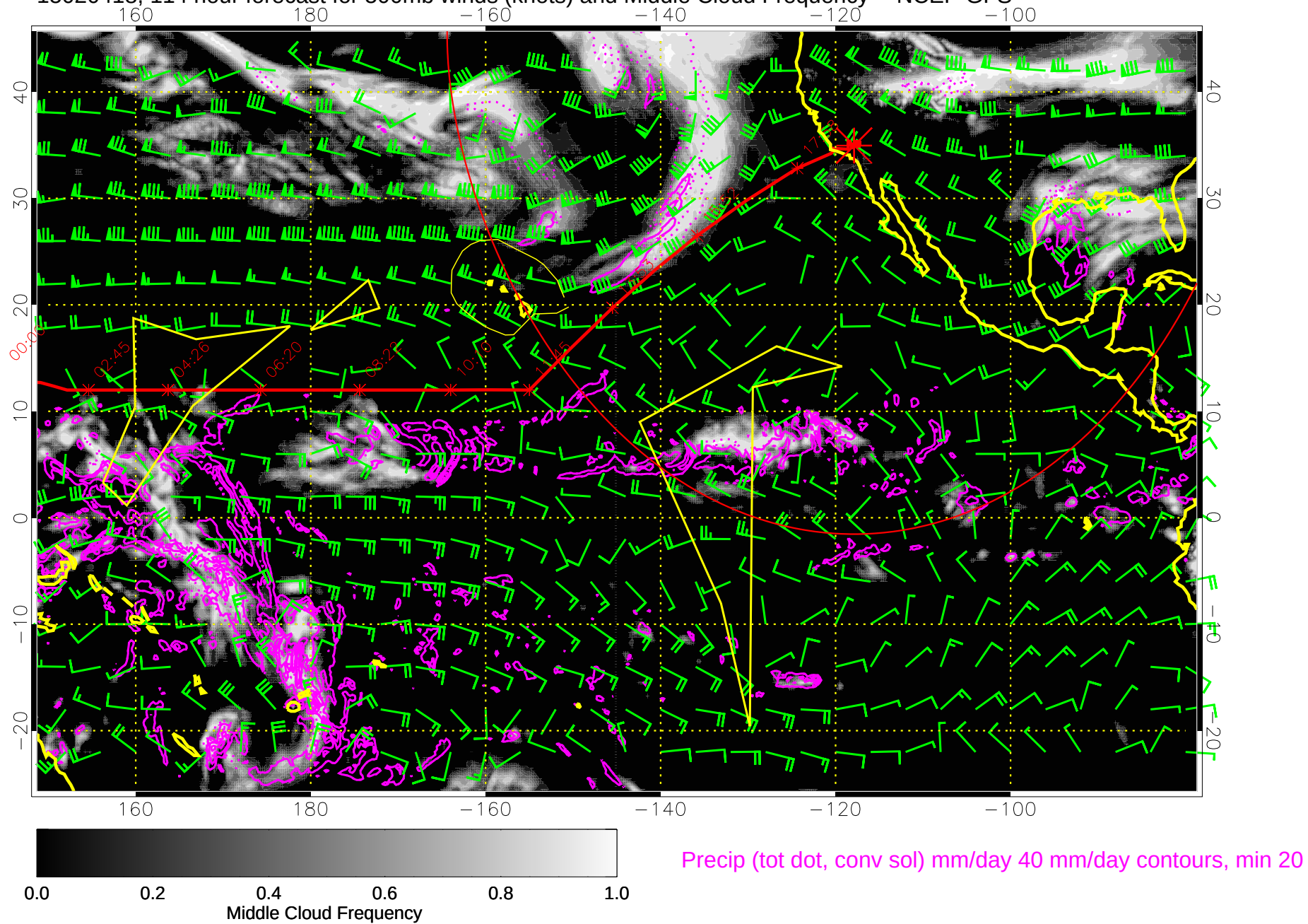
15020418, 114 hour forecast for 500mb winds (knots) and Middle Cloud Frequency -- NCEP GFS
