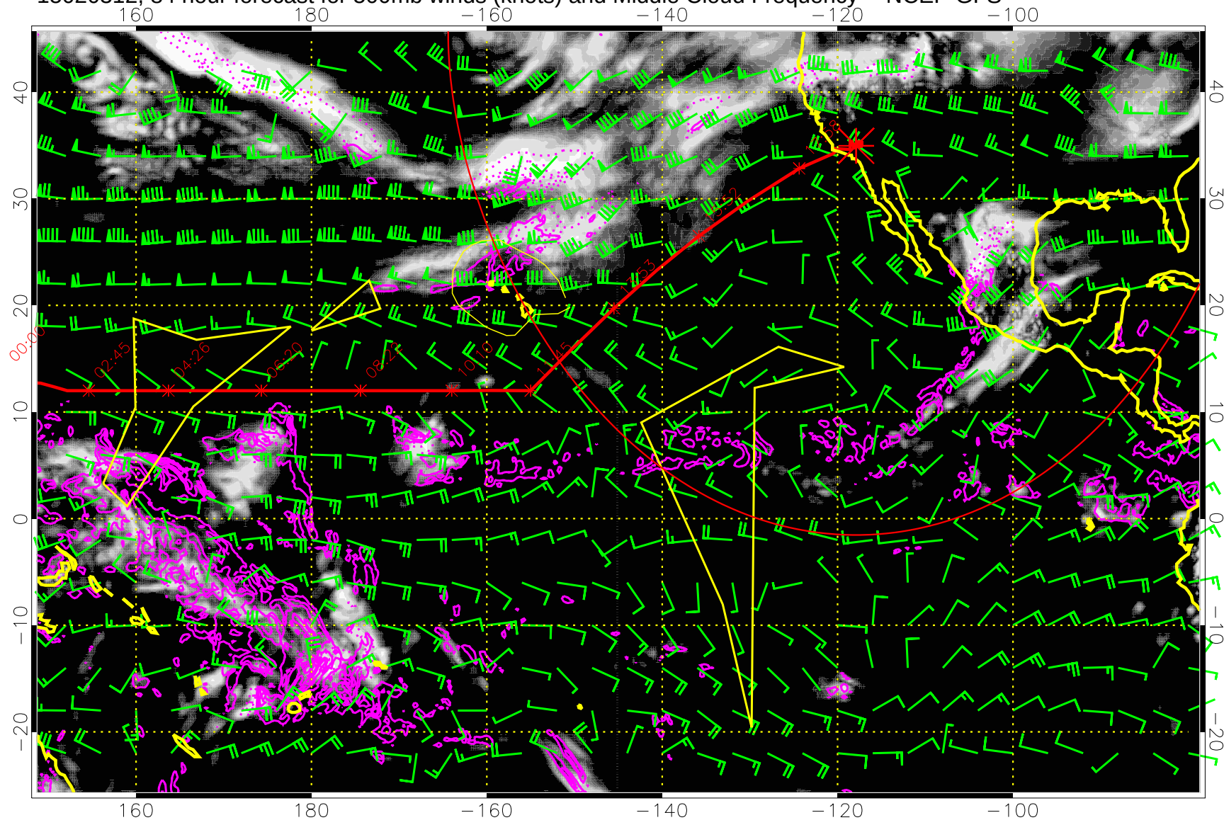
15020312, 84 hour forecast for 500mb winds (knots) and Middle Cloud Frequency -- NCEP GFS
