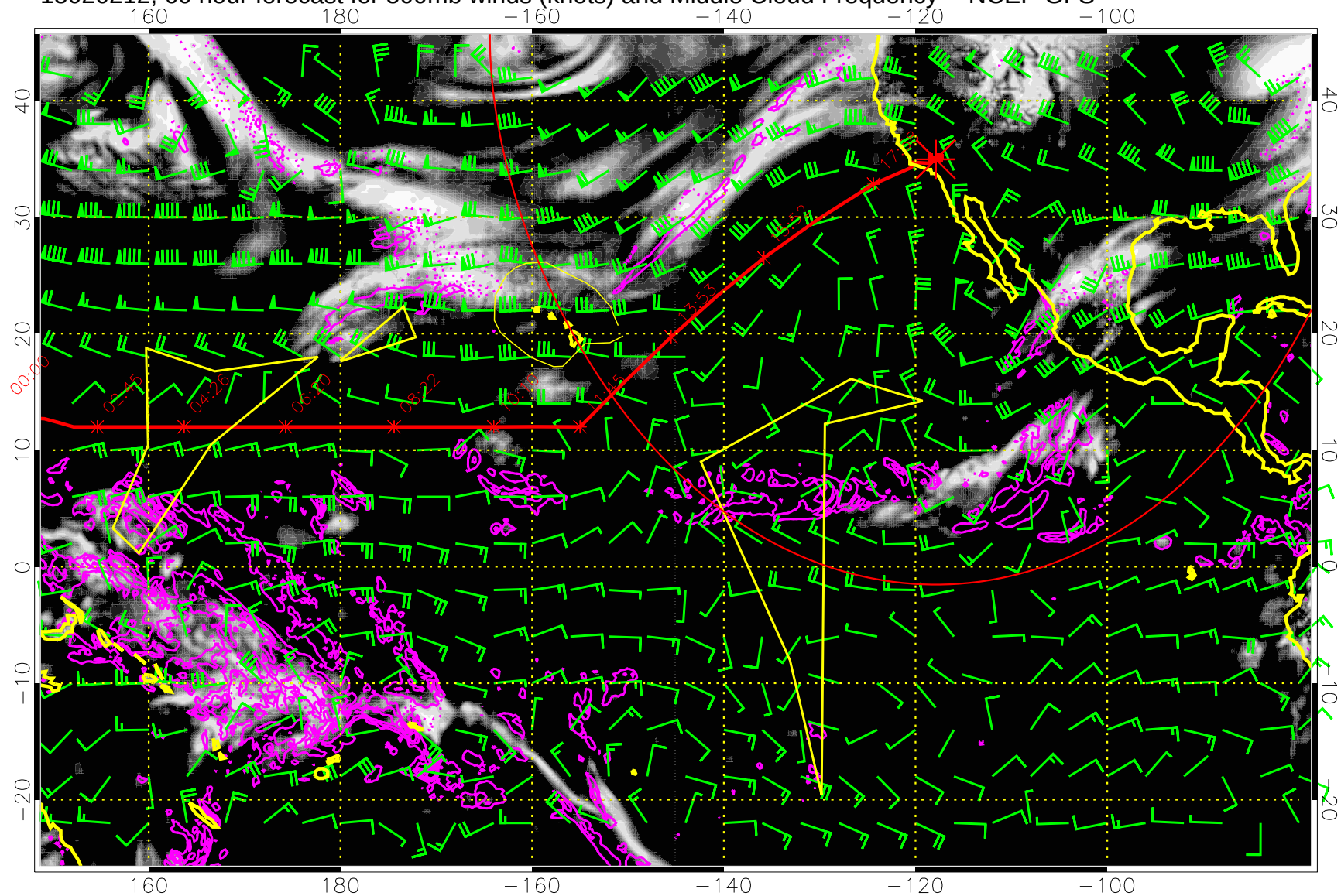
15020212, 60 hour forecast for 500mb winds (knots) and Middle Cloud Frequency -- NCEP GFS
