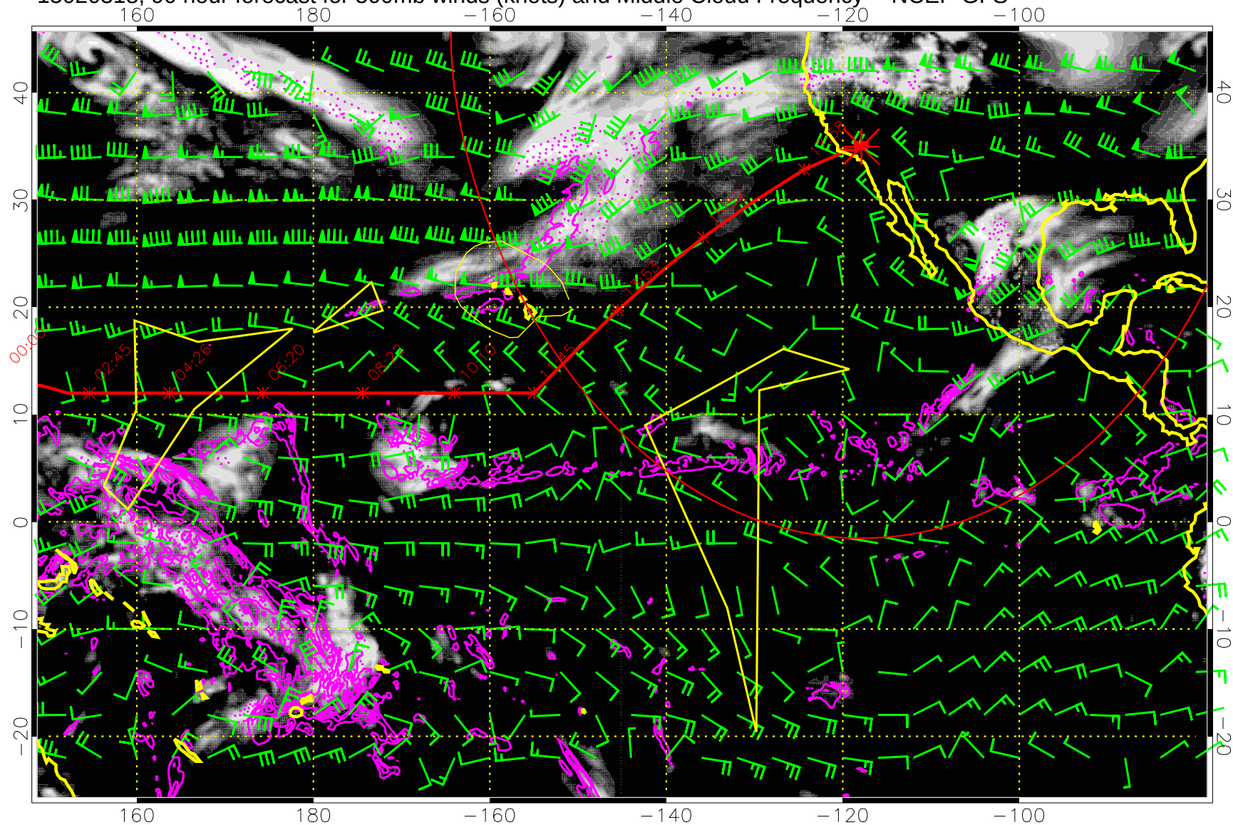
15020318, 90 hour forecast for 500mb winds (knots) and Middle Cloud Frequency -- NCEP GFS
