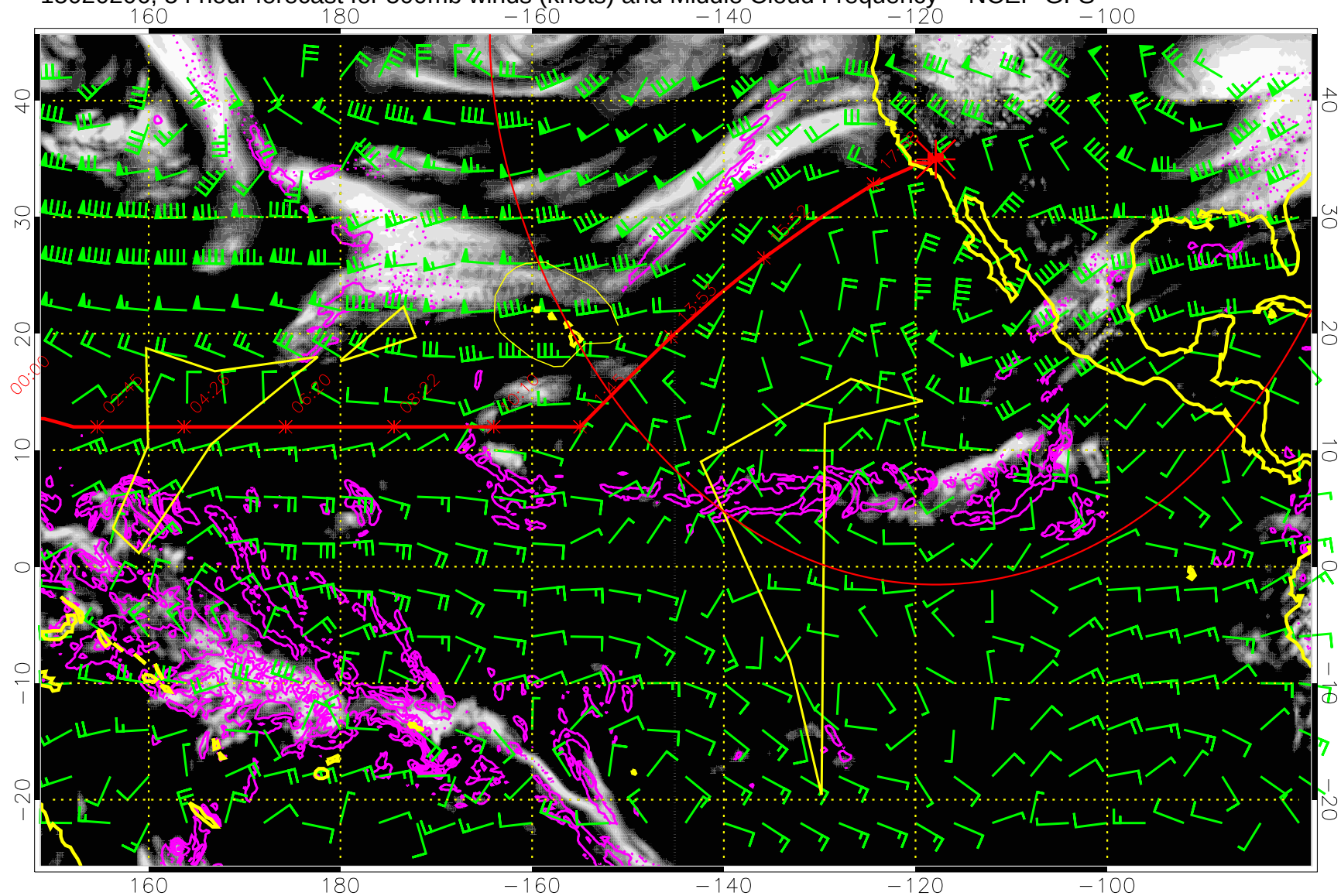
15020206, 54 hour forecast for 500mb winds (knots) and Middle Cloud Frequency -- NCEP GFS
