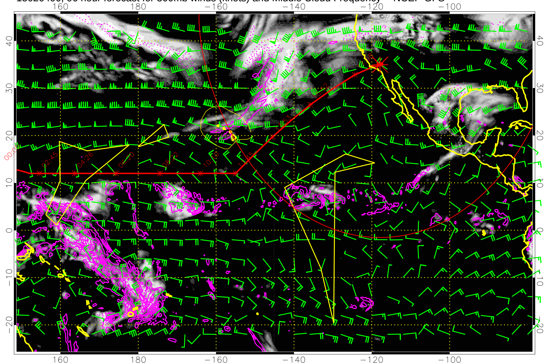
15020400, 96 hour forecast for 500mb winds (knots) and Middle Cloud Frequency -- NCEP GFS
