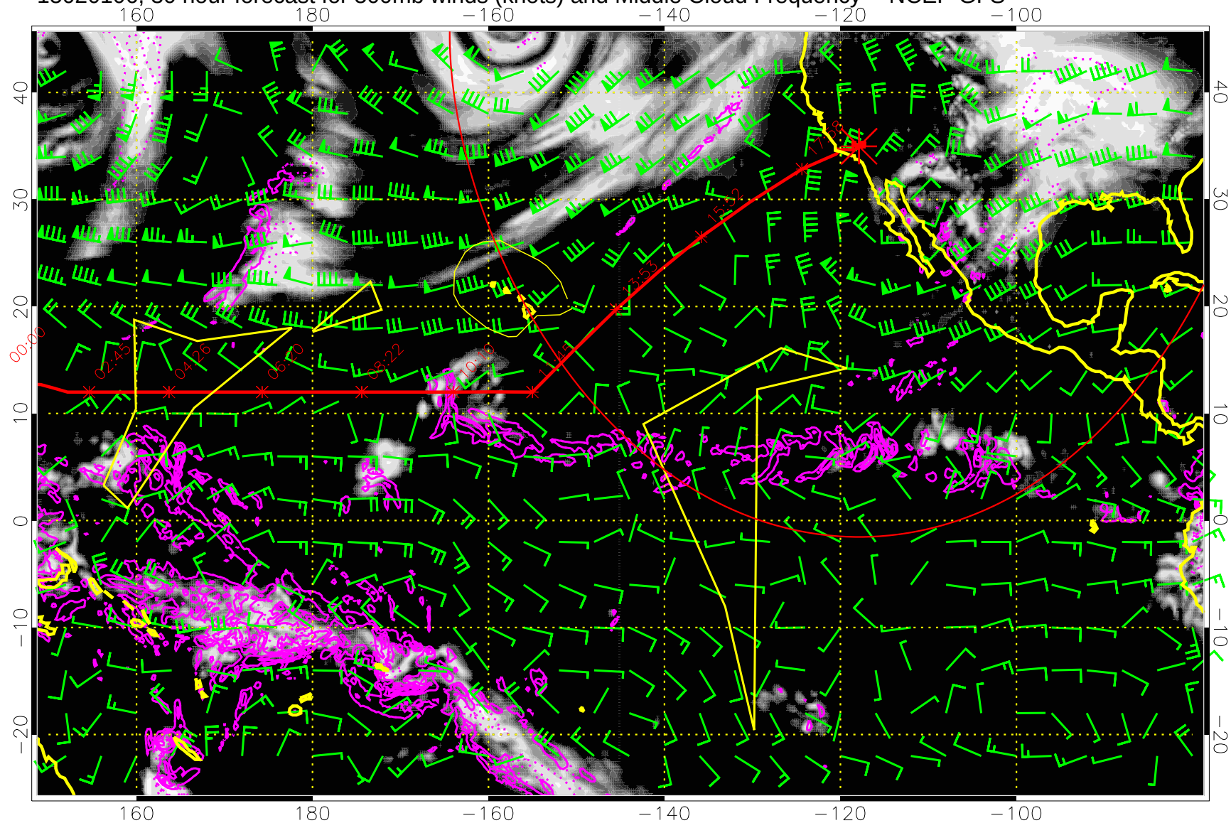
15020106, 30 hour forecast for 500mb winds (knots) and Middle Cloud Frequency -- NCEP GFS
