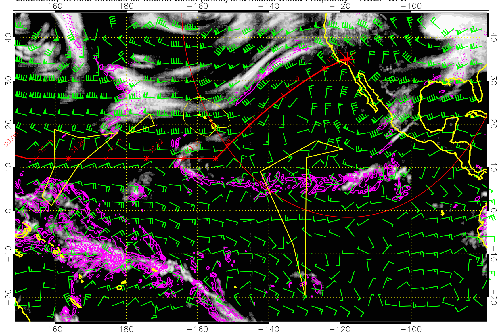
15020200, 48 hour forecast for 500mb winds (knots) and Middle Cloud Frequency -- NCEP GFS
