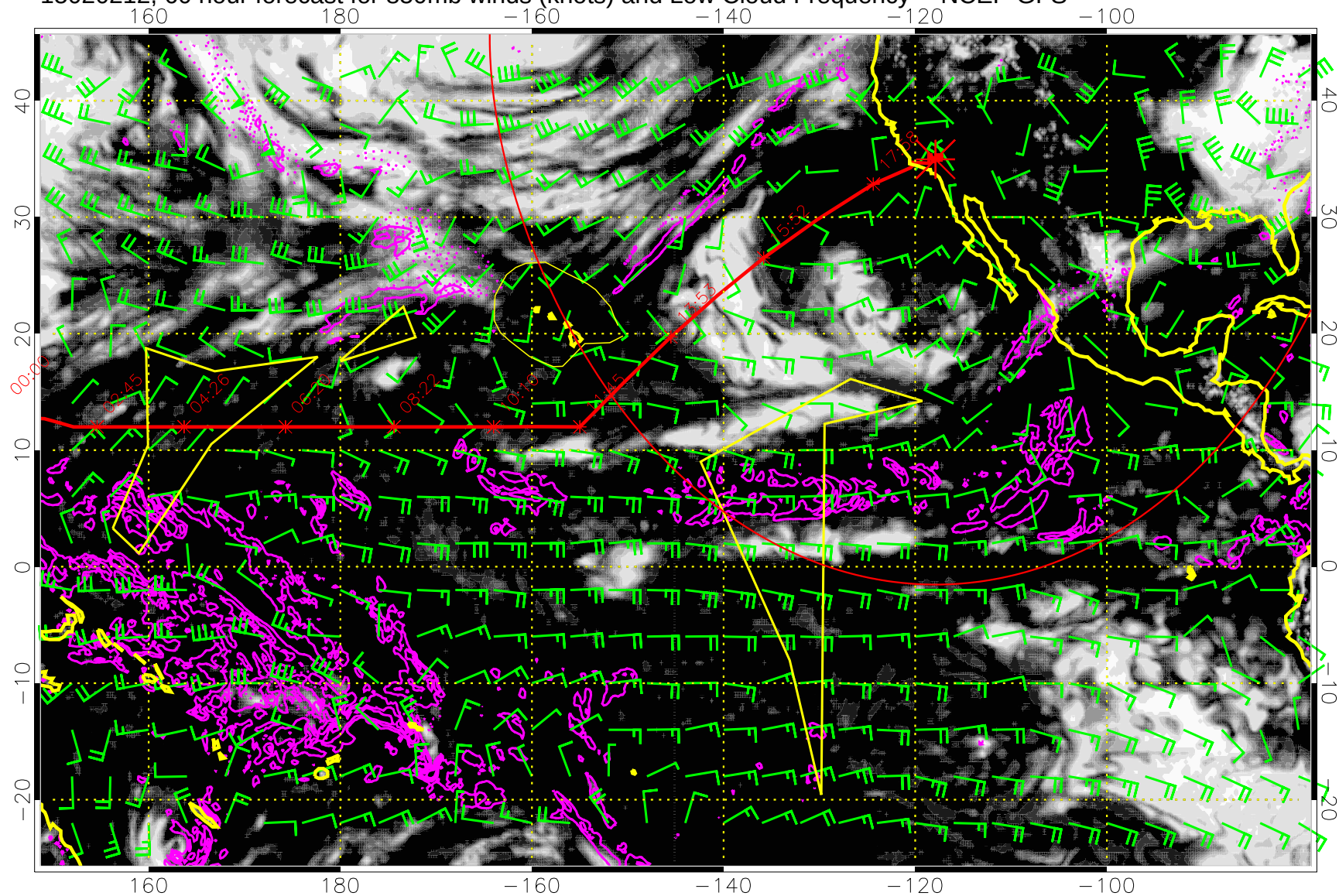
15020212, 60 hour forecast for 850mb winds (knots) and Low Cloud Frequency -- NCEP GFS
