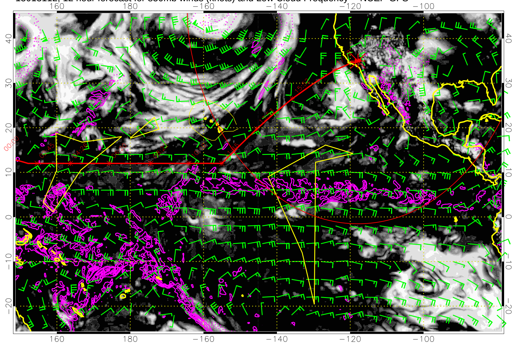
15013112, 12 hour forecast for 850mb winds (knots) and Low Cloud Frequency -- NCEP GFS
