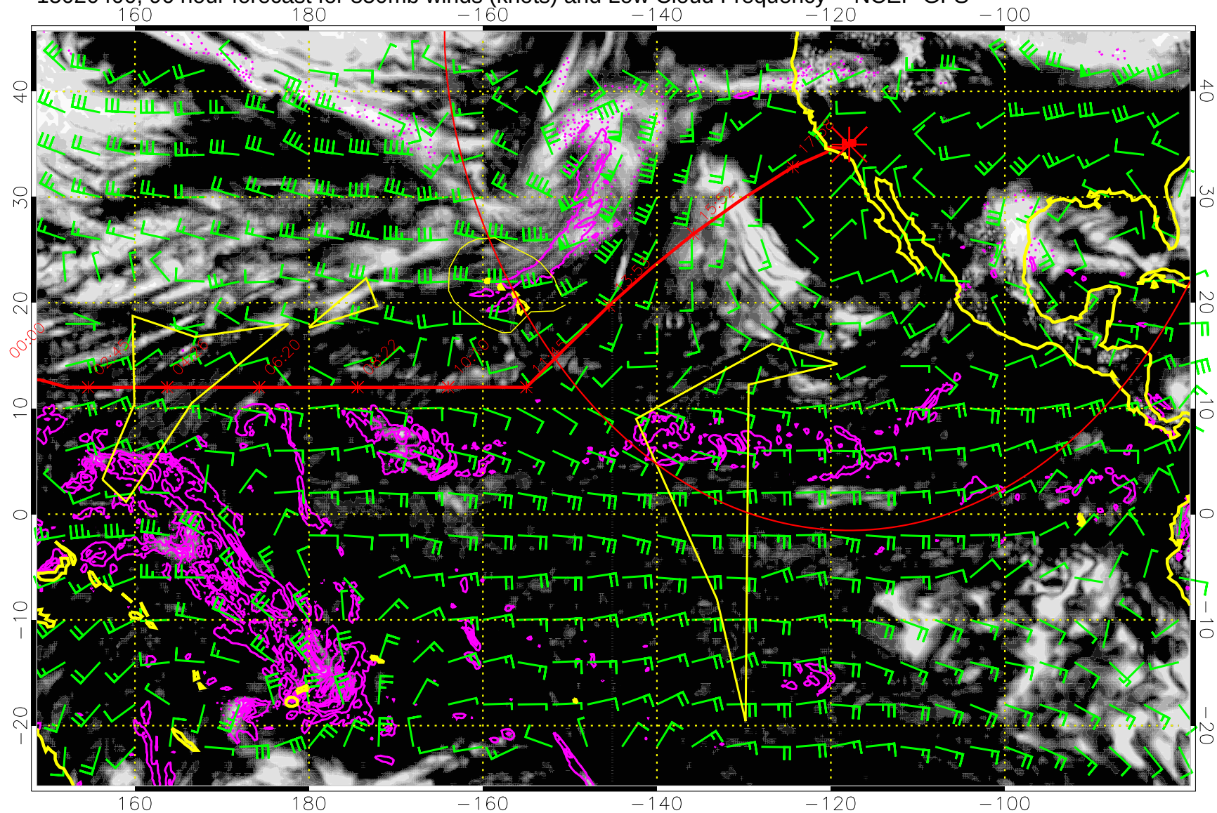
15020400, 96 hour forecast for 850mb winds (knots) and Low Cloud Frequency -- NCEP GFS
