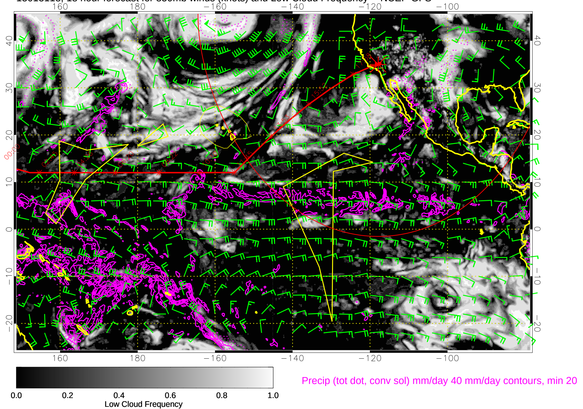
15013118, 18 hour forecast for 850mb winds (knots) and Low Cloud Frequency -- NCEP GFS
