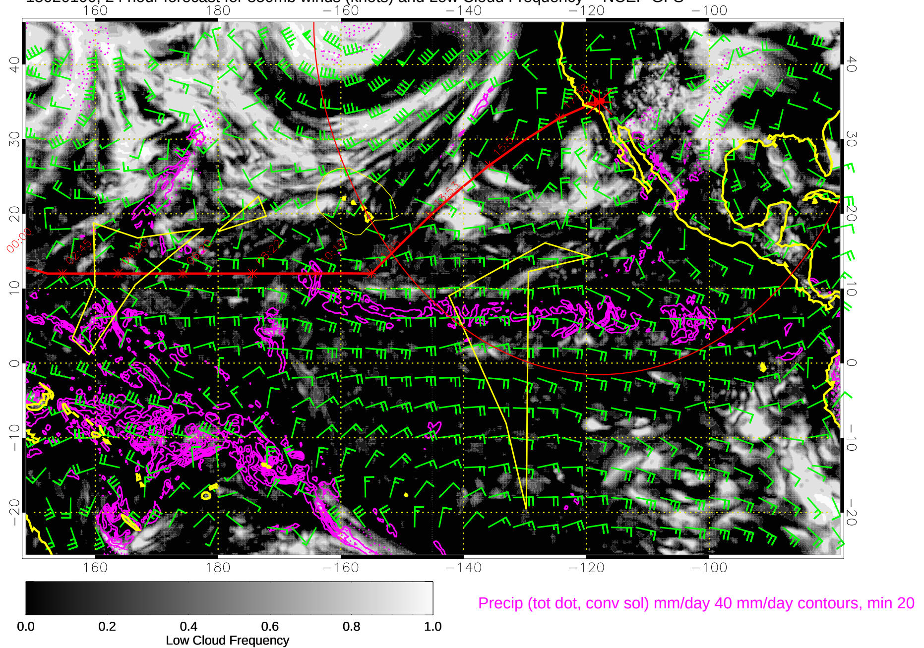
15020100, 24 hour forecast for 850mb winds (knots) and Low Cloud Frequency -- NCEP GFS
