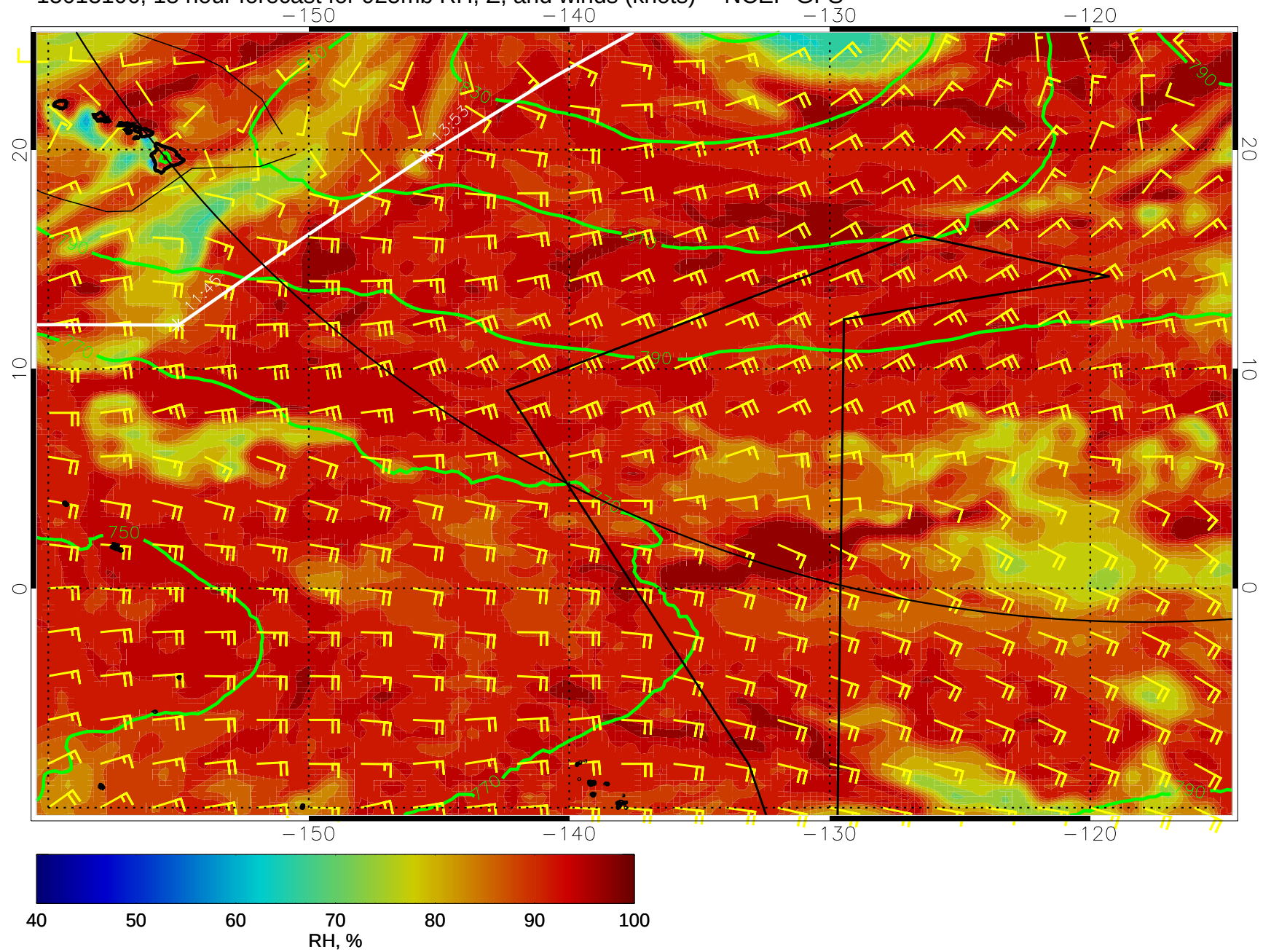
15013106, 18 hour forecast for 925mb RH, Z, and winds (knots) -- NCEP GFS
