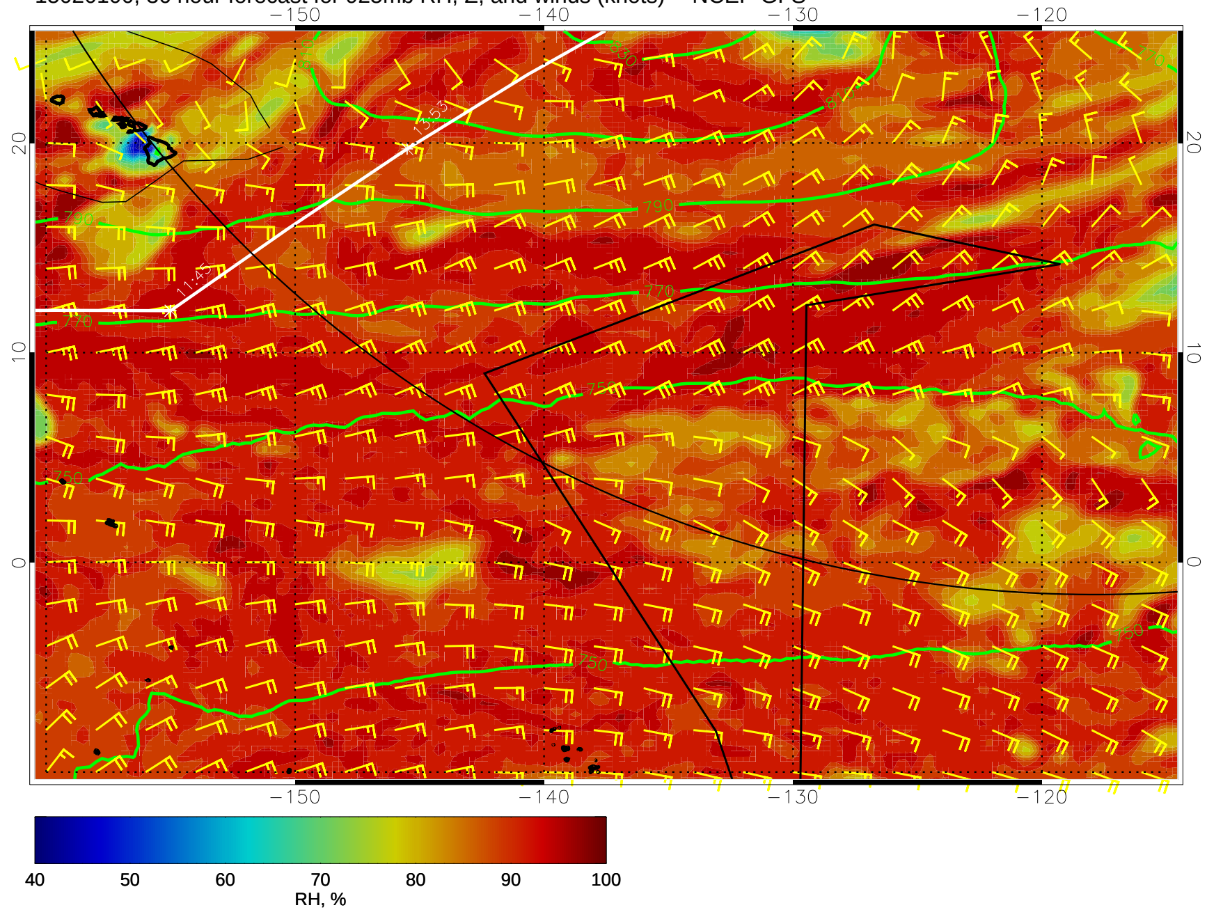
15020100, 36 hour forecast for 925mb RH, Z, and winds (knots) -- NCEP GFS
