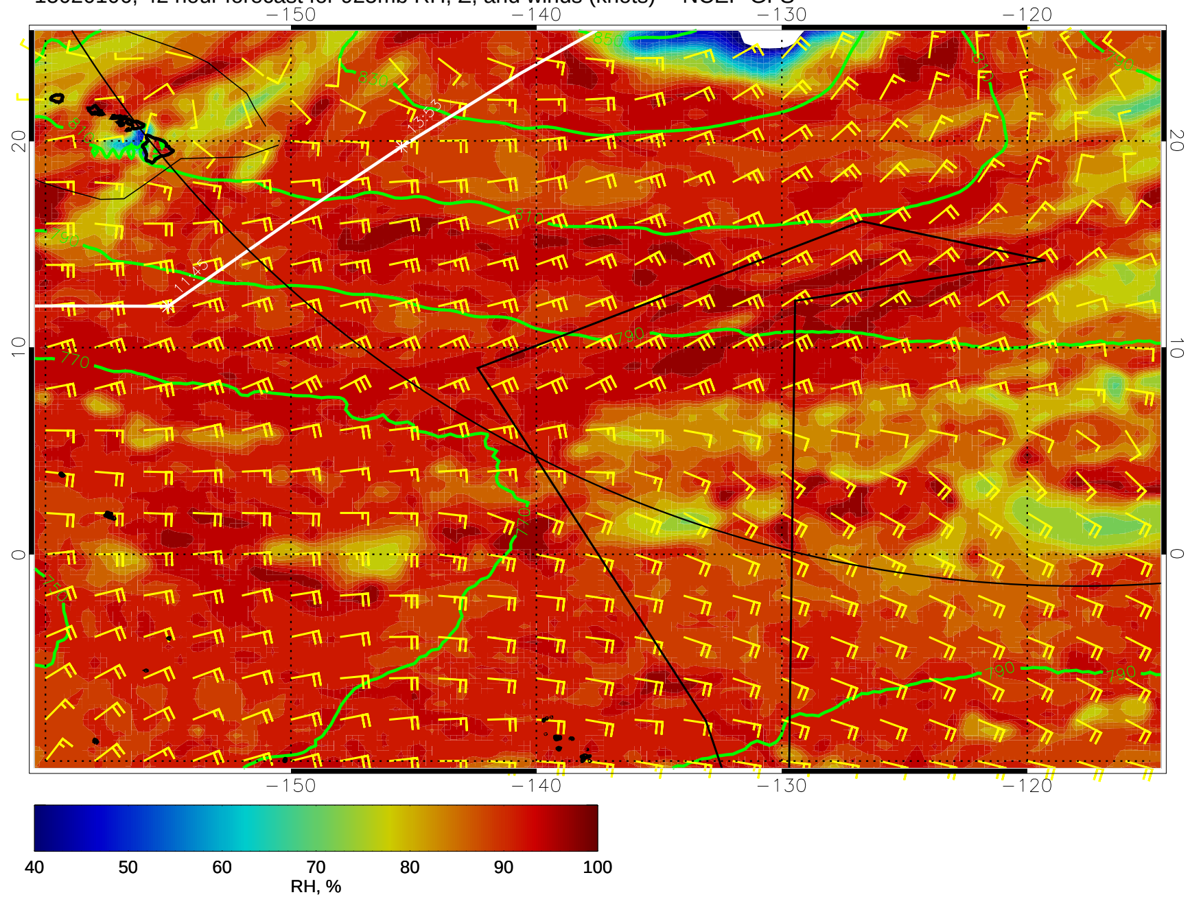
15020106, 42 hour forecast for 925mb RH, Z, and winds (knots) -- NCEP GFS
