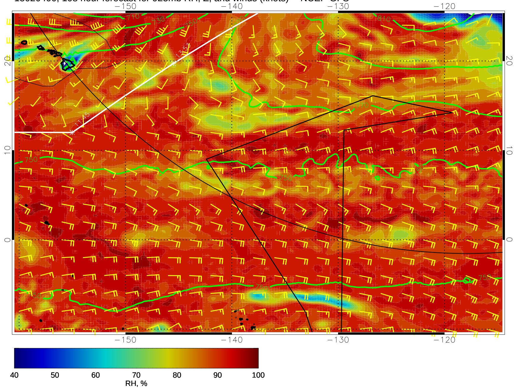
15020400, 108 hour forecast for 925mb RH, Z, and winds (knots) -- NCEP GFS
