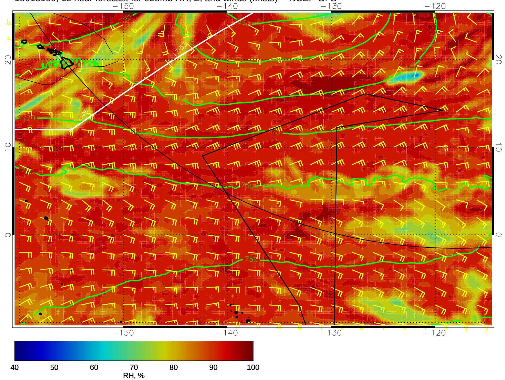
15013100, 12 hour forecast for 925mb RH, Z, and winds (knots) -- NCEP GFS
