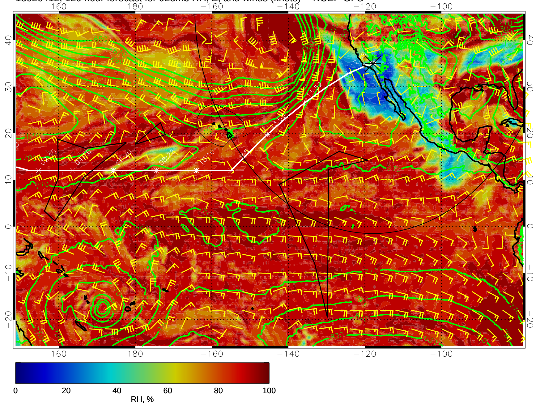
15020412, 120 hour forecast for 925mb RH, Z, and winds (knots) -- NCEP GFS
