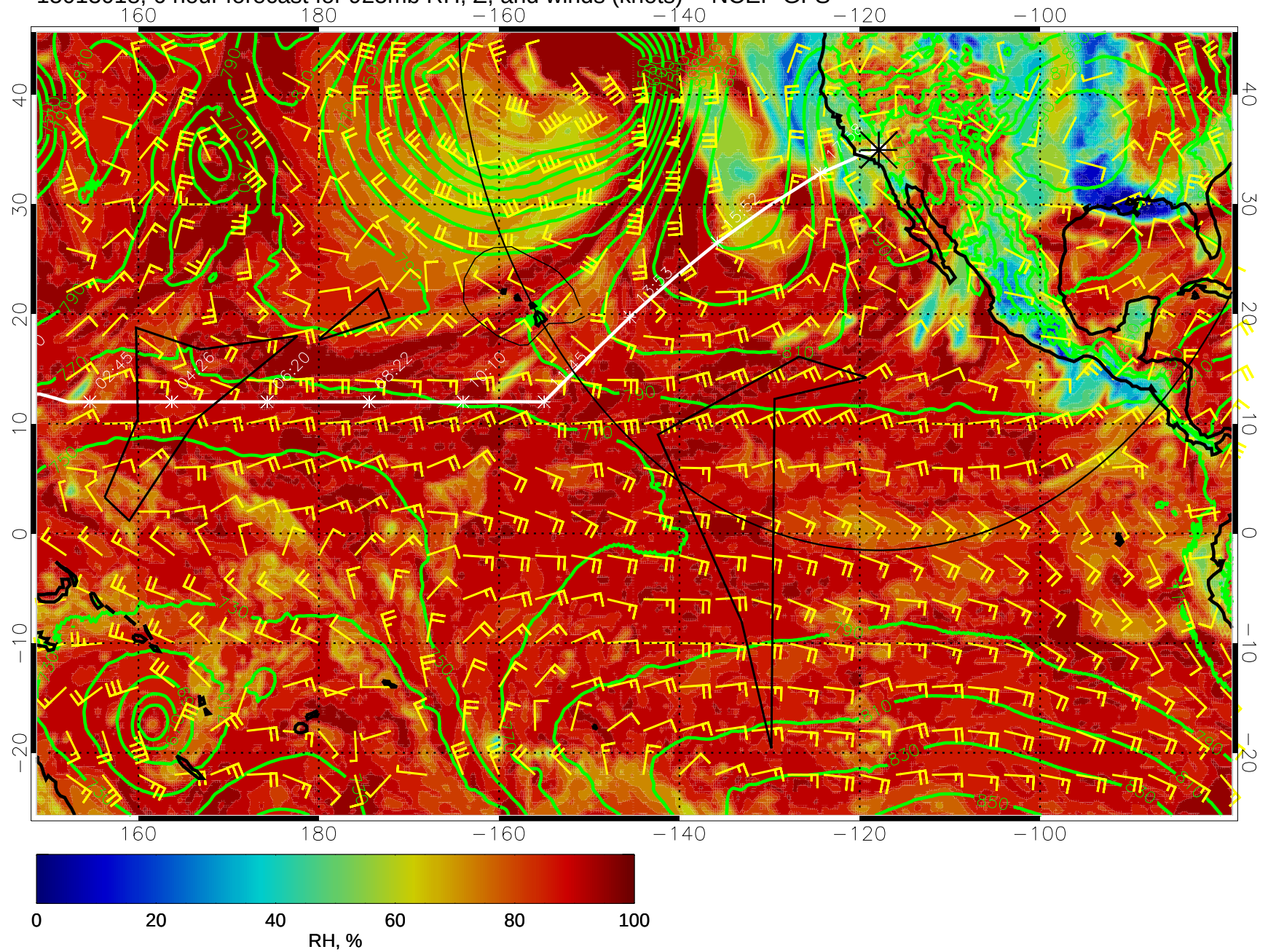
15013018, 6 hour forecast for 925mb RH, Z, and winds (knots) -- NCEP GFS
