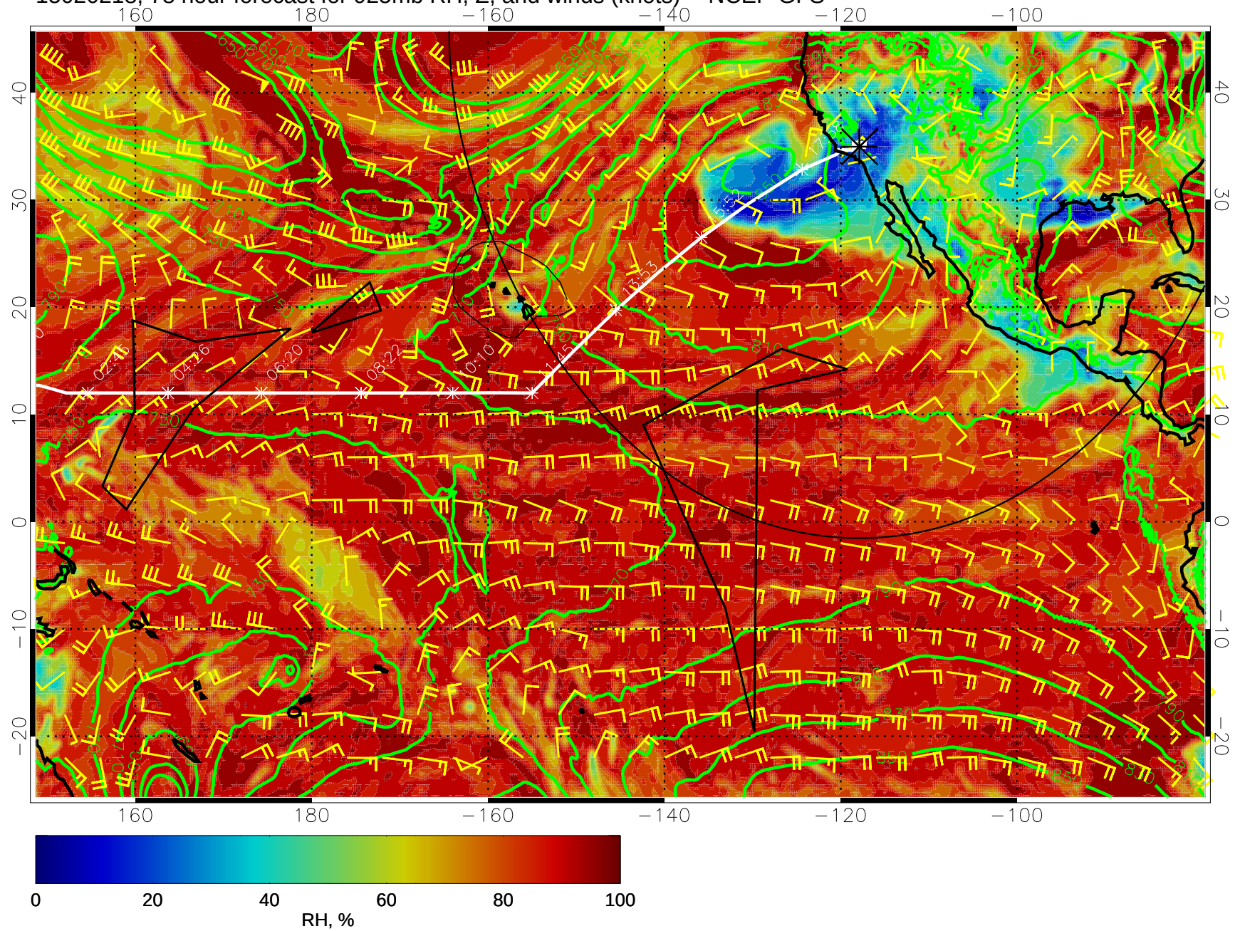
15020218, 78 hour forecast for 925mb RH, Z, and winds (knots) -- NCEP GFS
