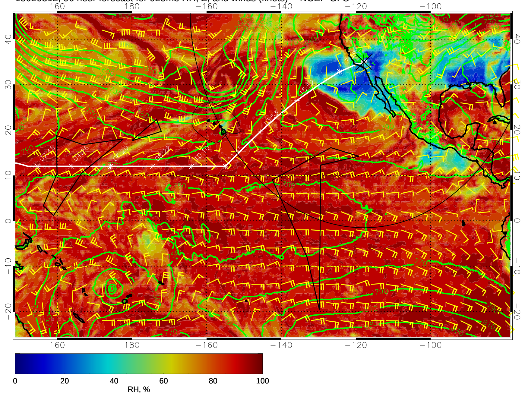
15020312, 96 hour forecast for 925mb RH, Z, and winds (knots) -- NCEP GFS
