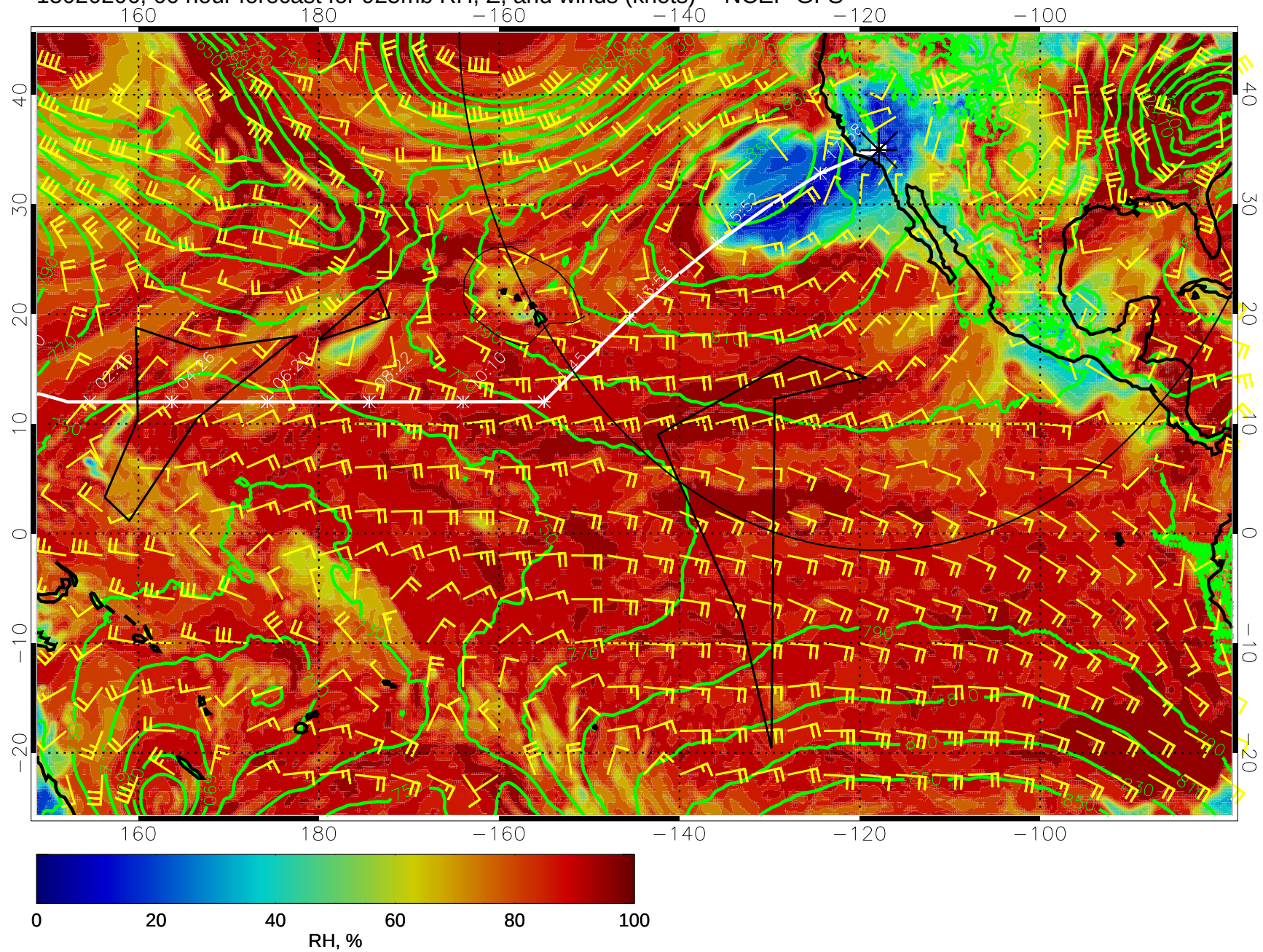
15020206, 66 hour forecast for 925mb RH, Z, and winds (knots) -- NCEP GFS
