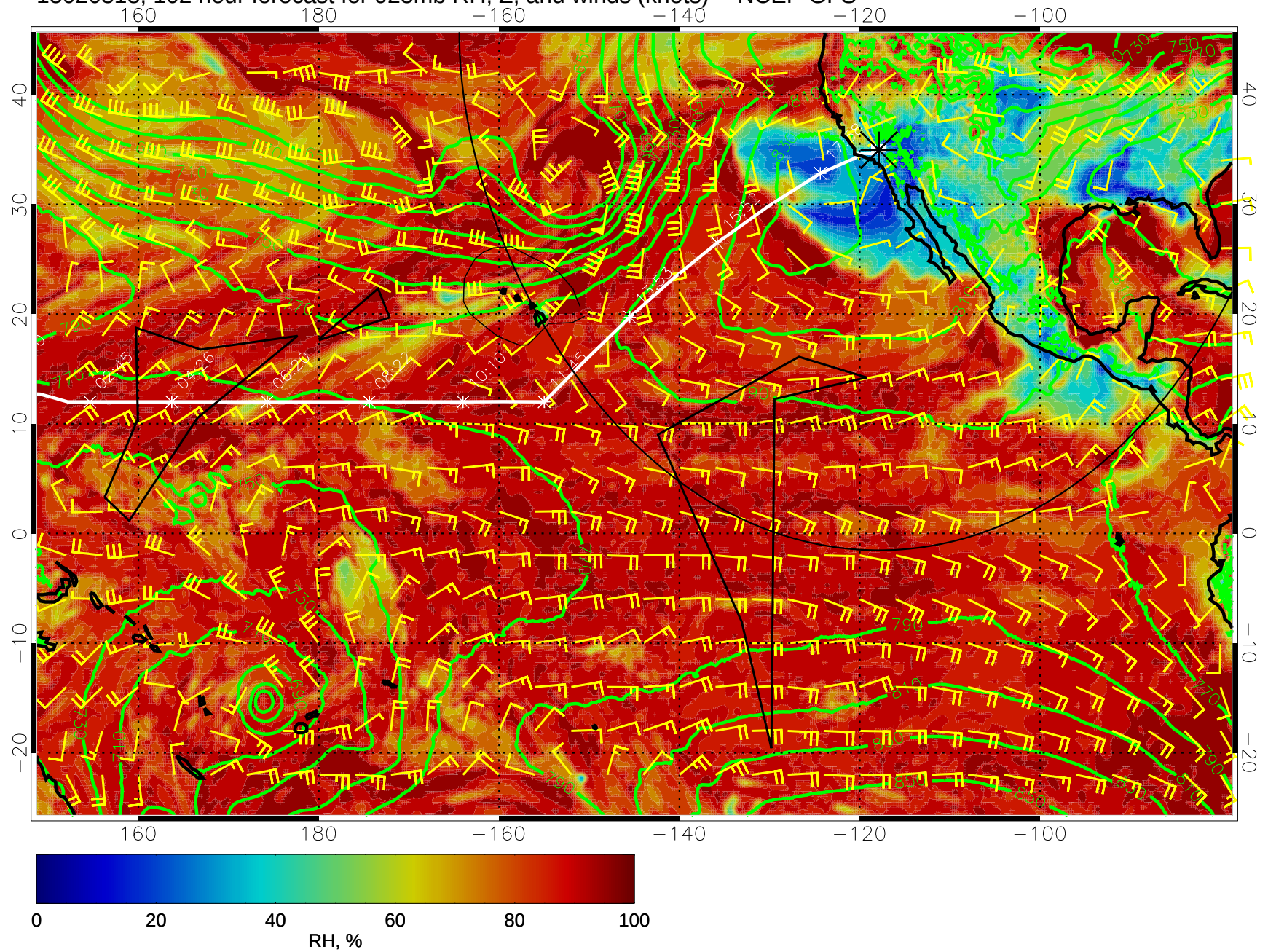
15020318, 102 hour forecast for 925mb RH, Z, and winds (knots) -- NCEP GFS
