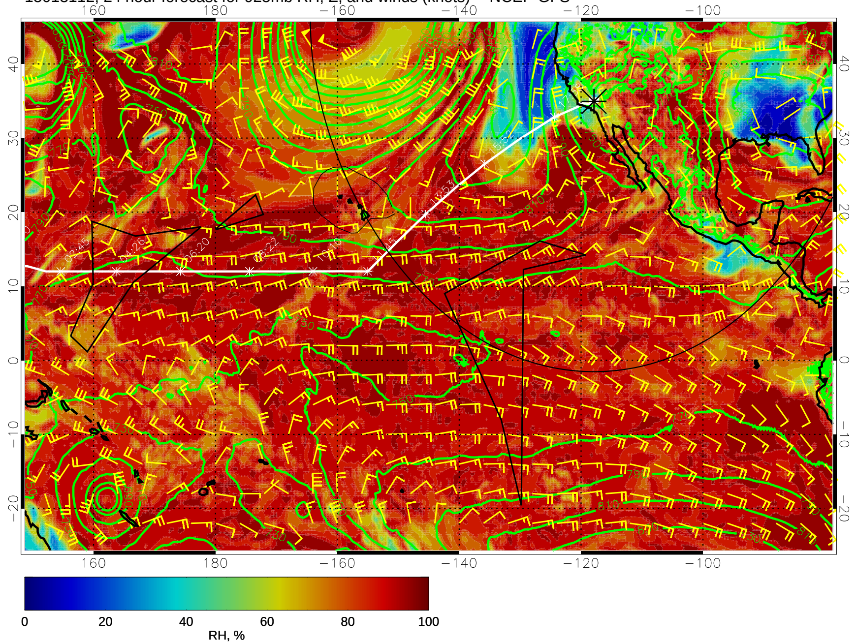
15013112, 24 hour forecast for 925mb RH, Z, and winds (knots) -- NCEP GFS
