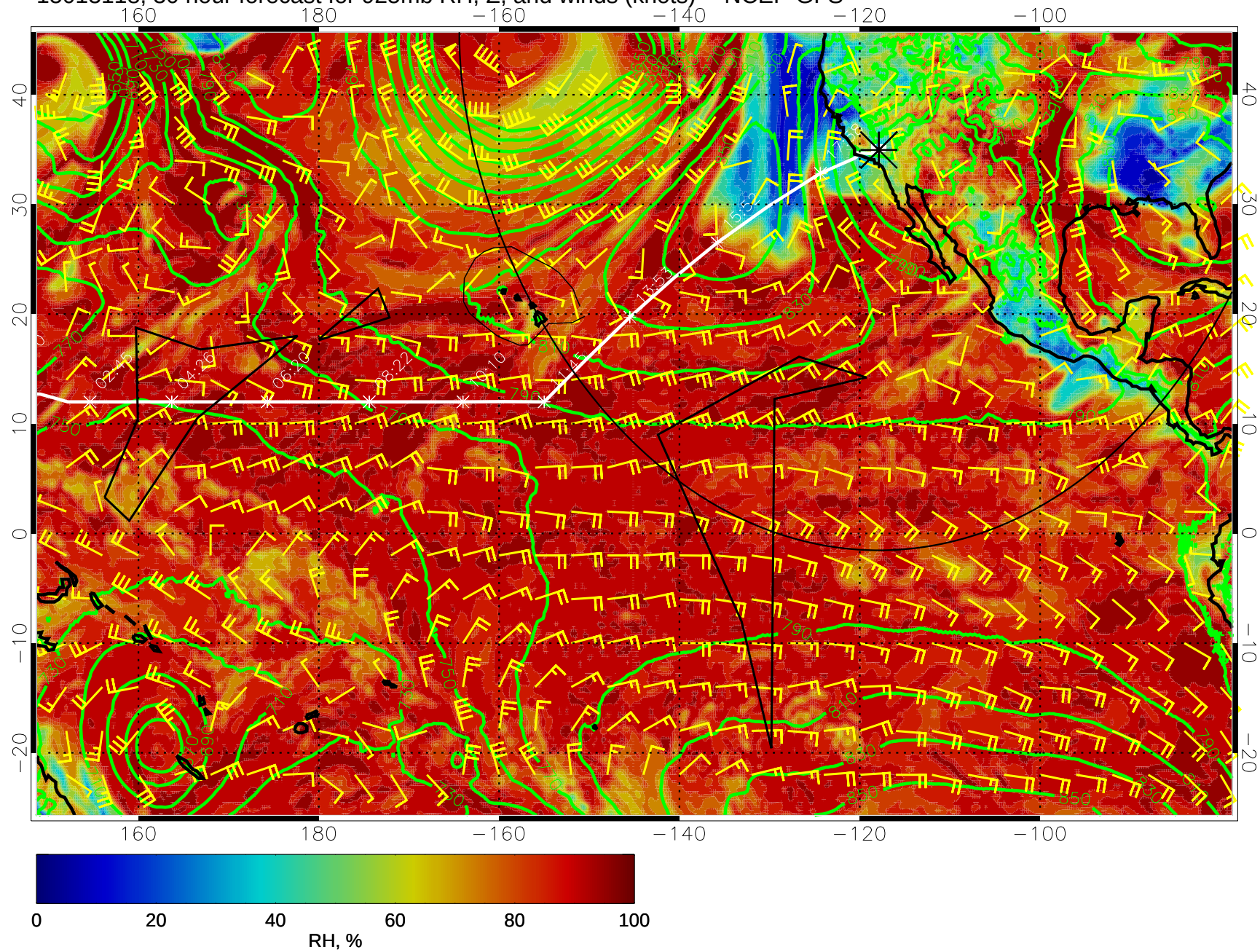
15013118, 30 hour forecast for 925mb RH, Z, and winds (knots) -- NCEP GFS
