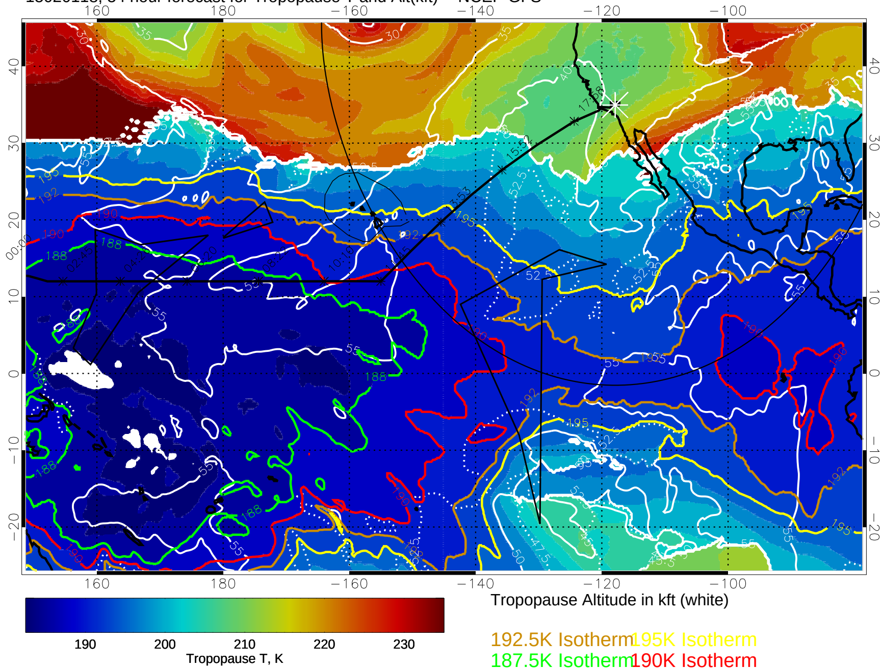
15020118, 54 hour forecast for Tropopause T and Alt(kft) -- NCEP GFS
