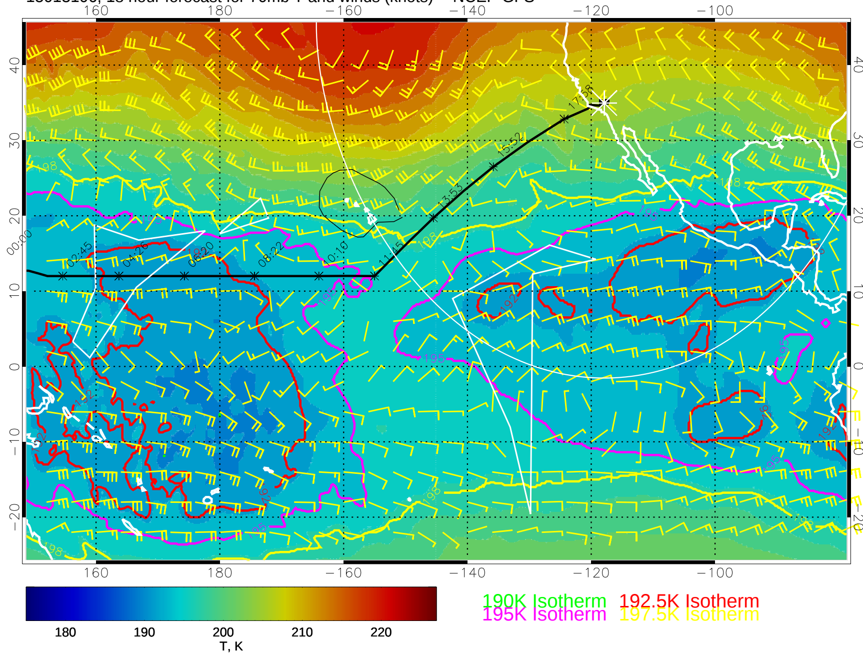
15013106, 18 hour forecast for 70mb T and winds (knots) -- NCEP GFS
