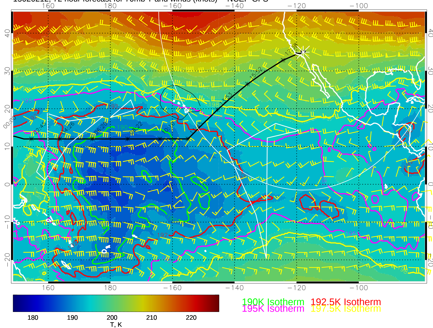
15020212, 72 hour forecast for 70mb T and winds (knots) -- NCEP GFS
