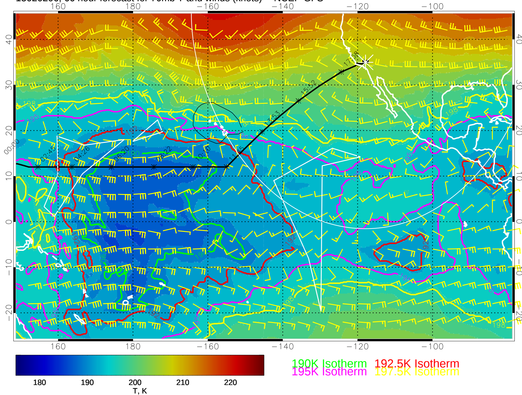
15020206, 66 hour forecast for 70mb T and winds (knots) -- NCEP GFS
