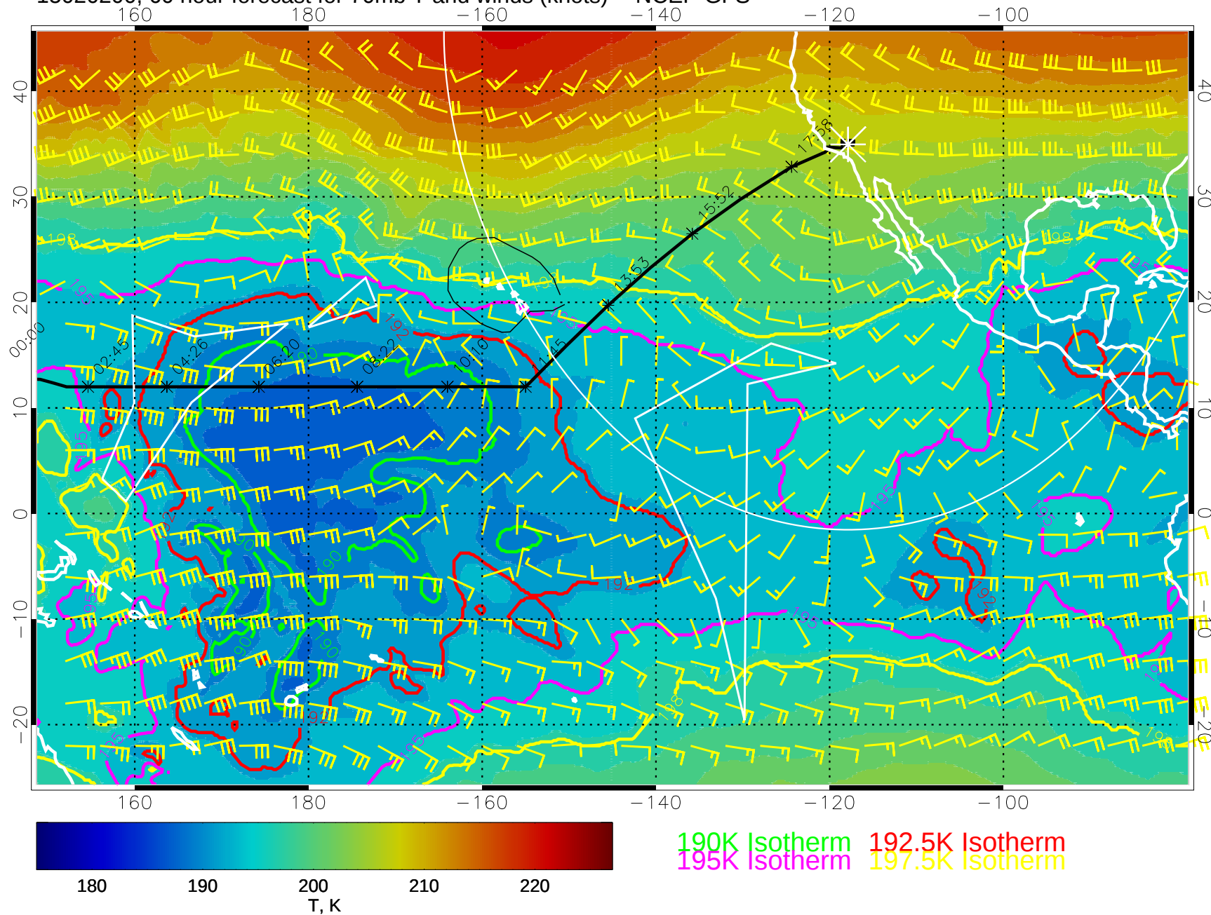
15020200, 60 hour forecast for 70mb T and winds (knots) -- NCEP GFS
