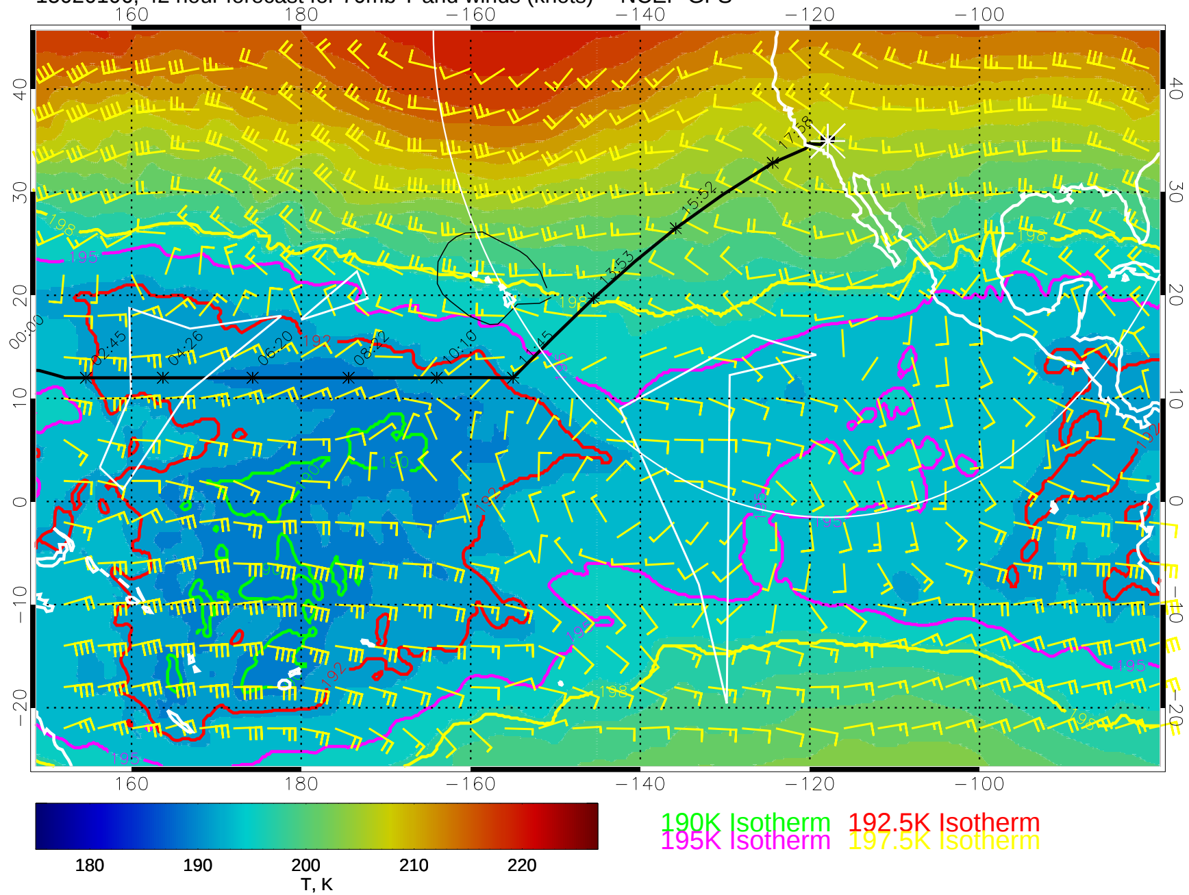
15020106, 42 hour forecast for 70mb T and winds (knots) -- NCEP GFS
