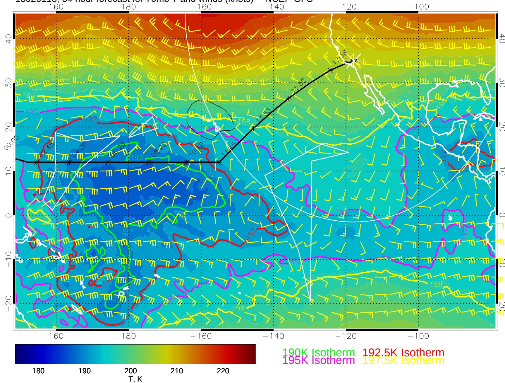
15020118, 54 hour forecast for 70mb T and winds (knots) -- NCEP GFS
