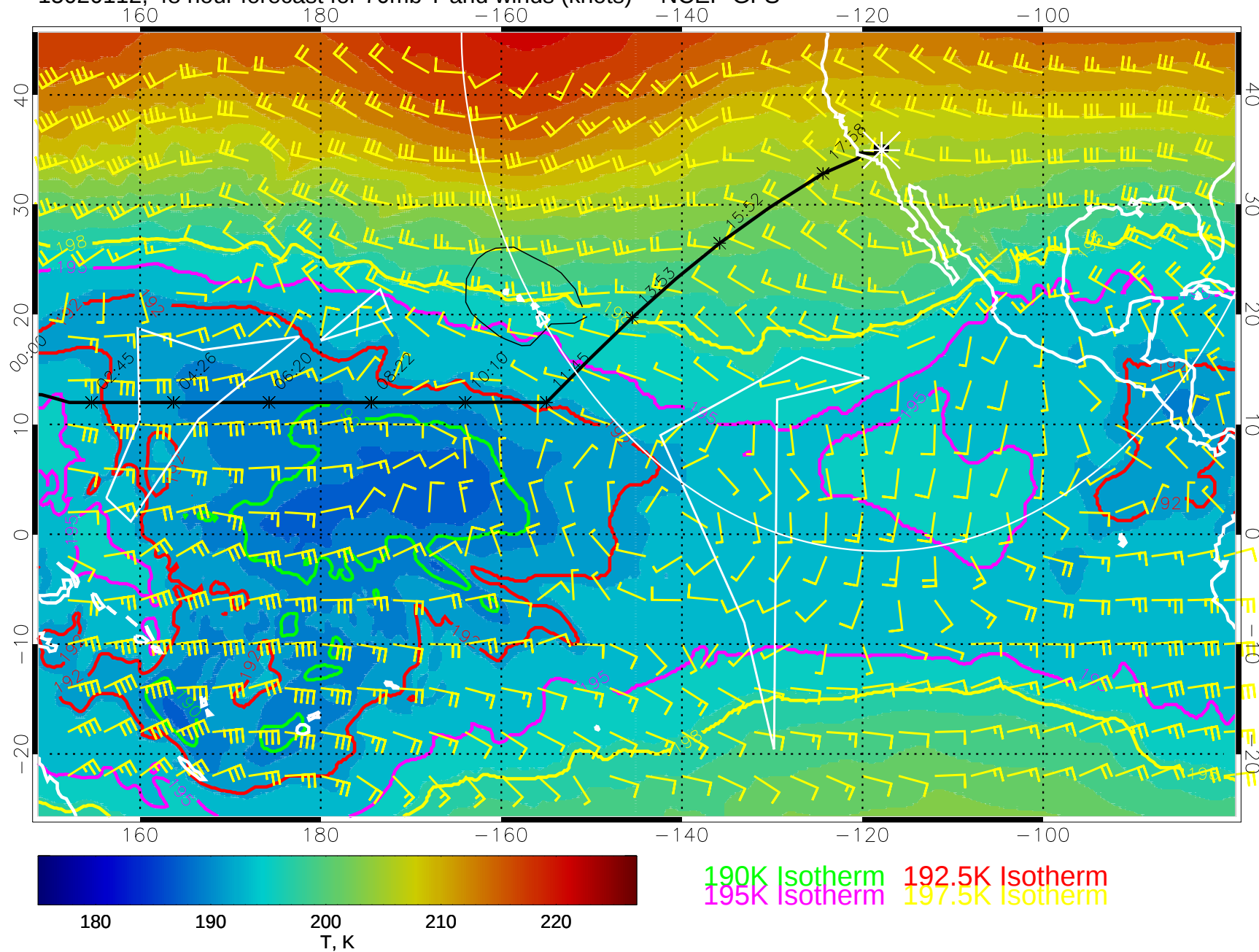
15020112, 48 hour forecast for 70mb T and winds (knots) -- NCEP GFS
