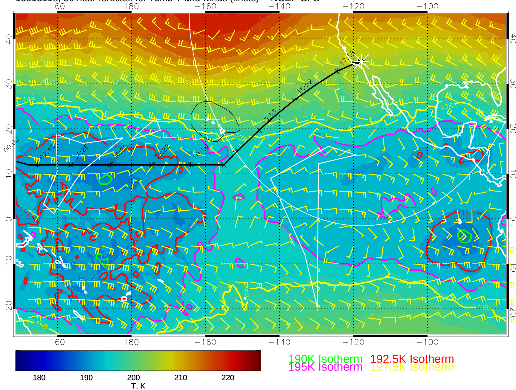
15013118, 30 hour forecast for 70mb T and winds (knots) -- NCEP GFS
