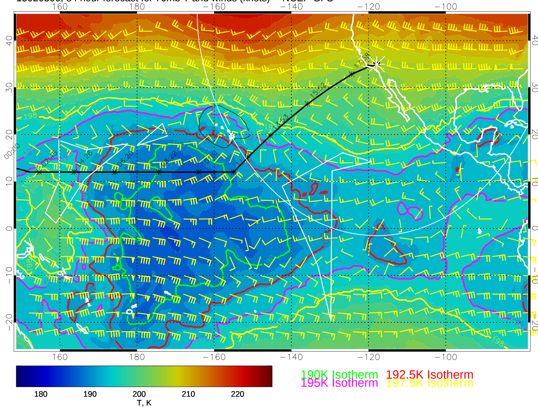
15020300, 84 hour forecast for 70mb T and winds (knots) -- NCEP GFS
