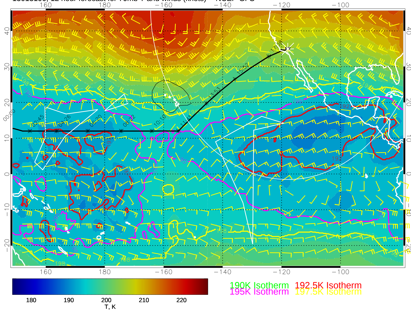
15013100, 12 hour forecast for 70mb T and winds (knots) -- NCEP GFS
