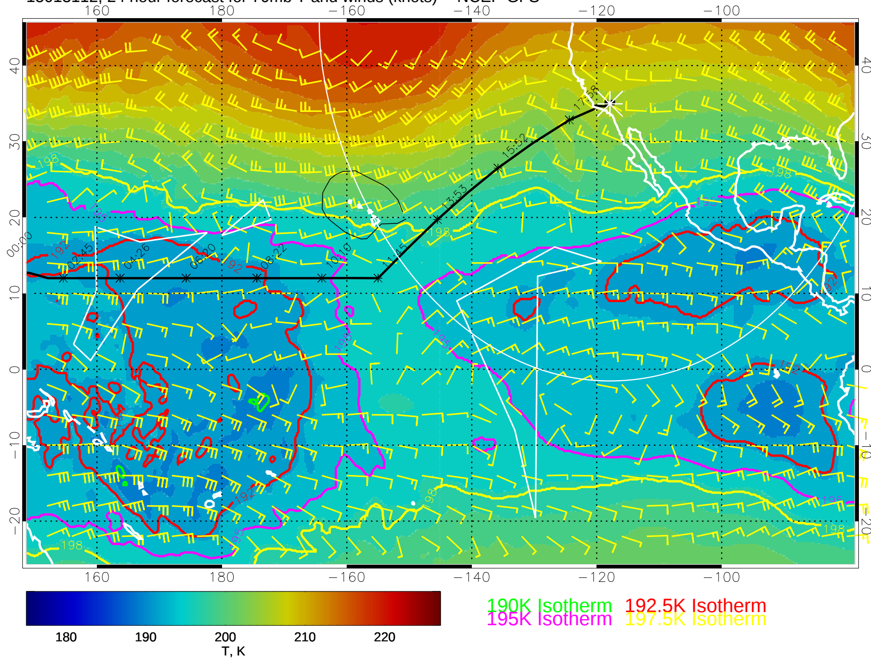
15013112, 24 hour forecast for 70mb T and winds (knots) -- NCEP GFS
