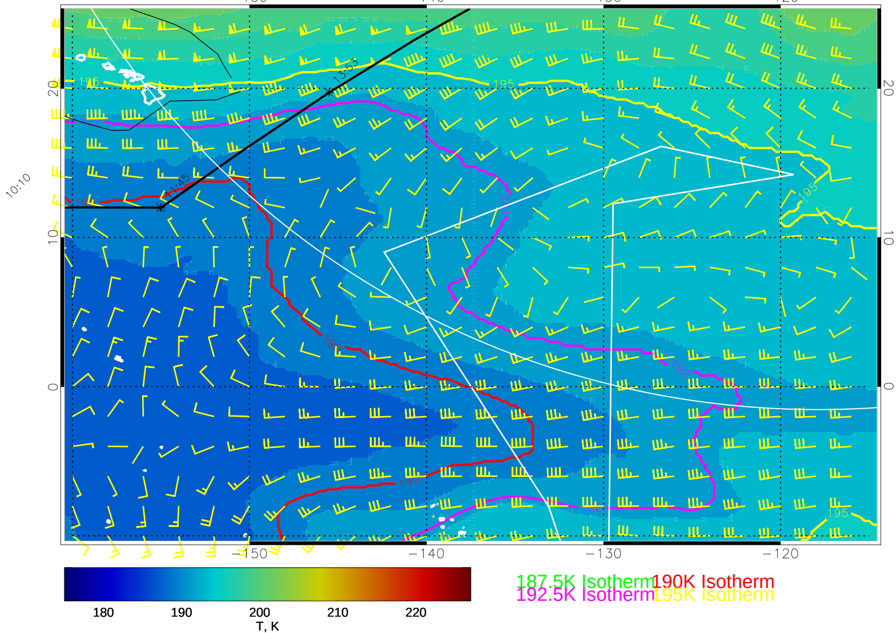
15013106, 18 hour forecast for 100mb T and winds (knots) -- NCEP GFS
