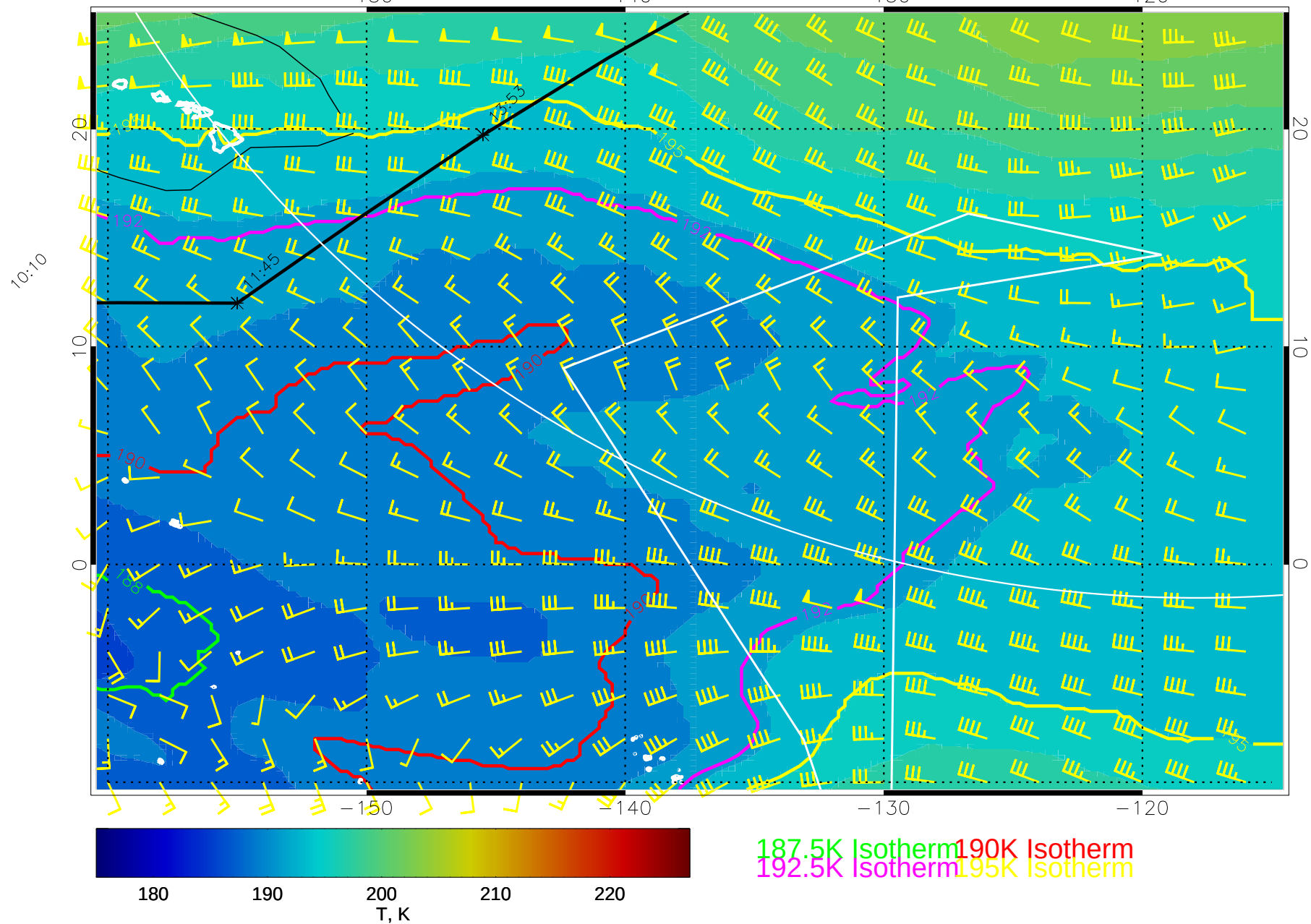
15020112, 48 hour forecast for 100mb T and winds (knots) -- NCEP GFS
