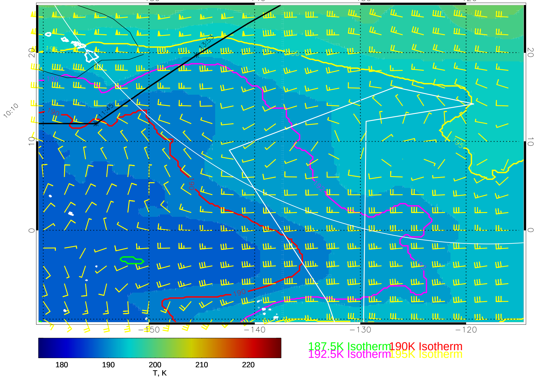
15013112, 24 hour forecast for 100mb T and winds (knots) -- NCEP GFS
