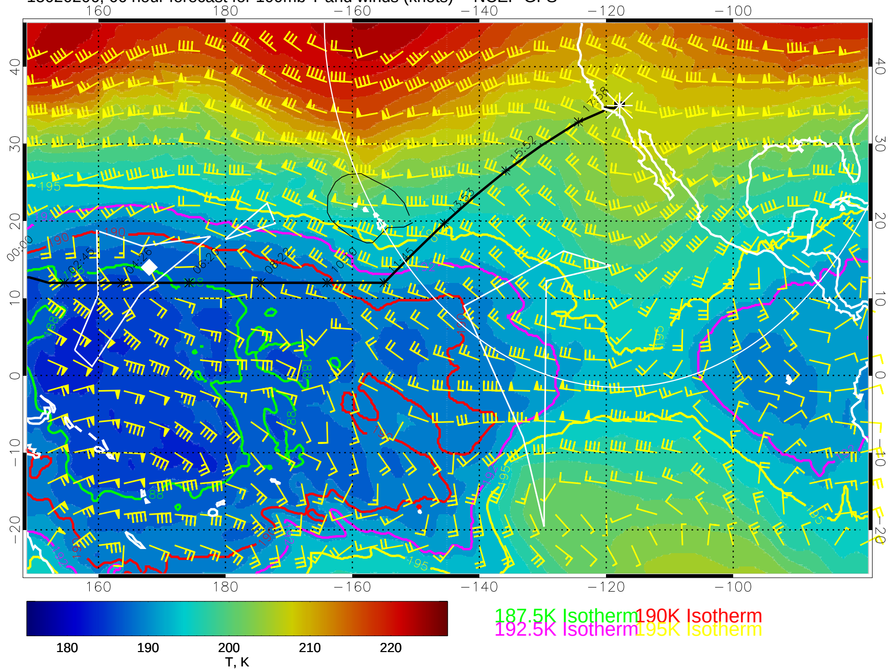
15020206, 66 hour forecast for 100mb T and winds (knots) -- NCEP GFS
