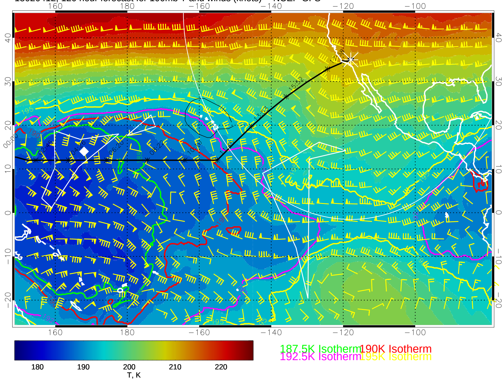
15020412, 120 hour forecast for 100mb T and winds (knots) -- NCEP GFS
