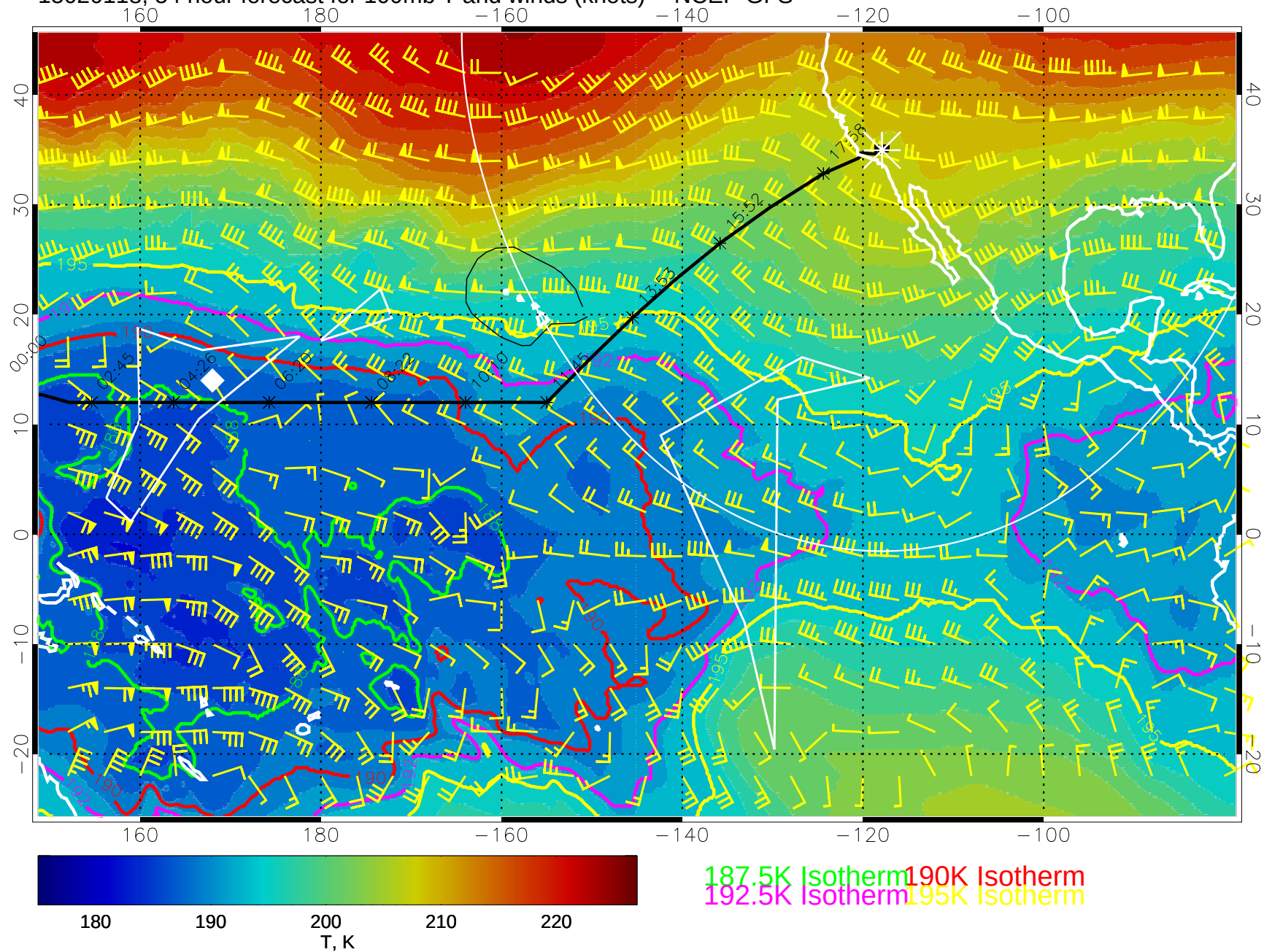
15020118, 54 hour forecast for 100mb T and winds (knots) -- NCEP GFS
