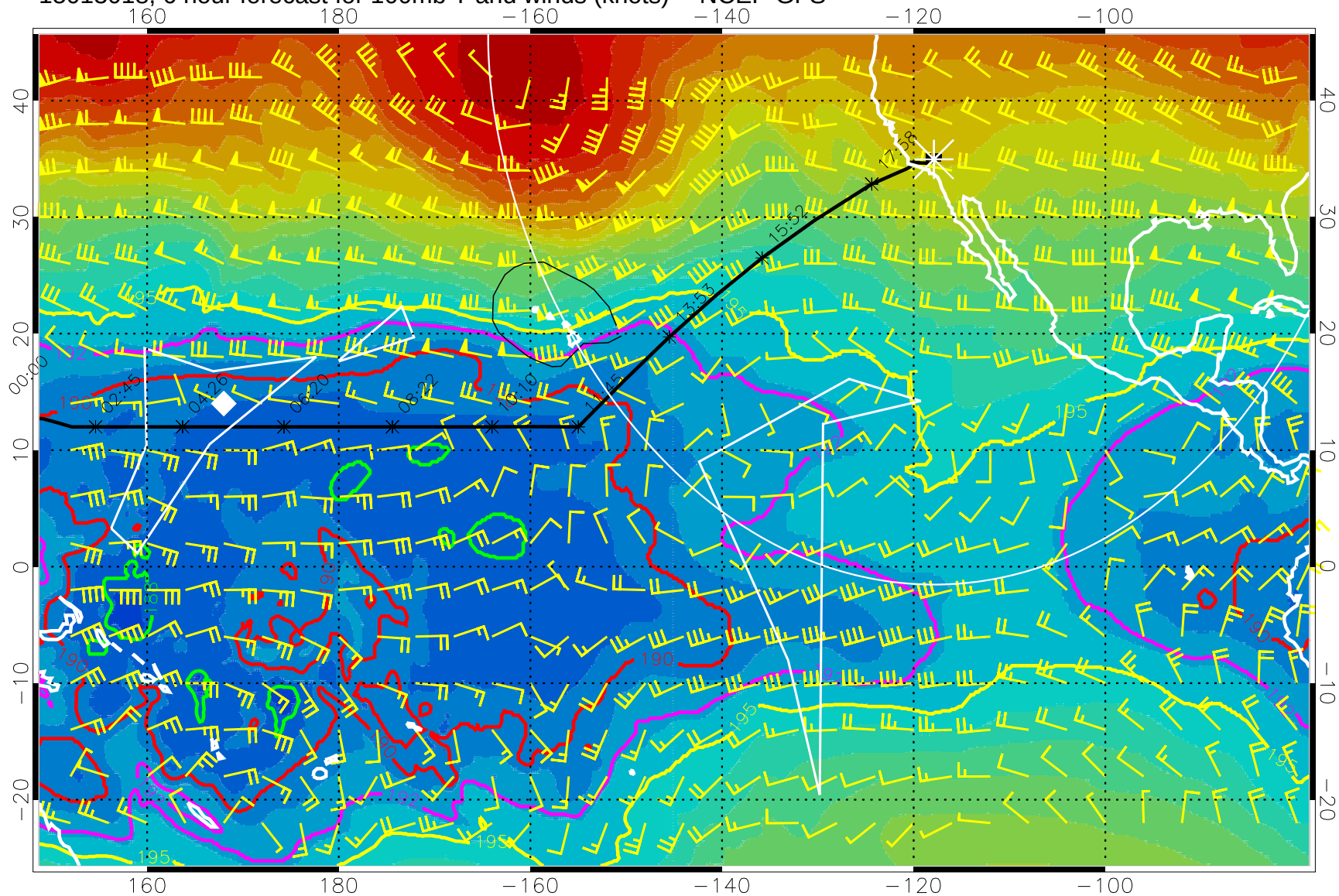
15013018, 6 hour forecast for 100mb T and winds (knots) -- NCEP GFS
