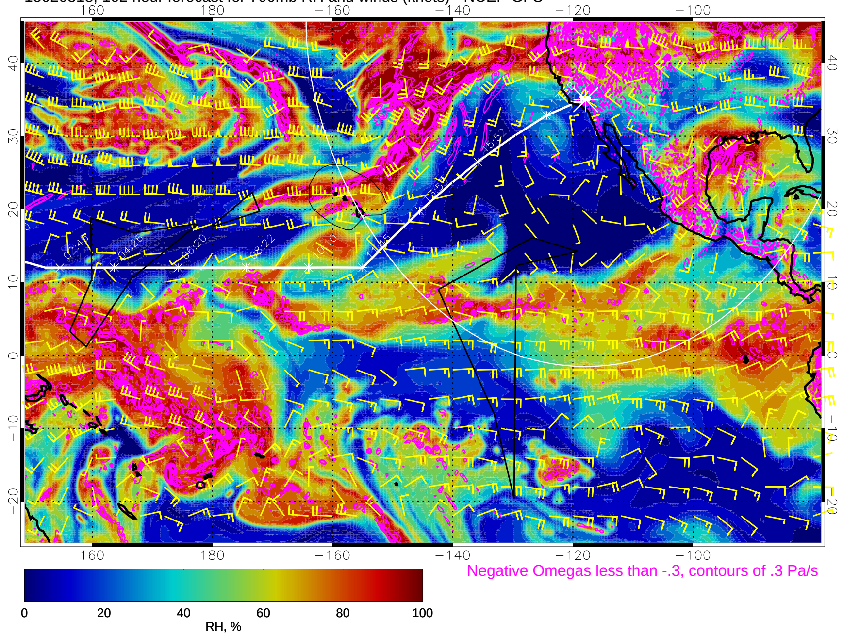
15020318, 102 hour forecast for 700mb RH and winds (knots) - NCEP GFS
