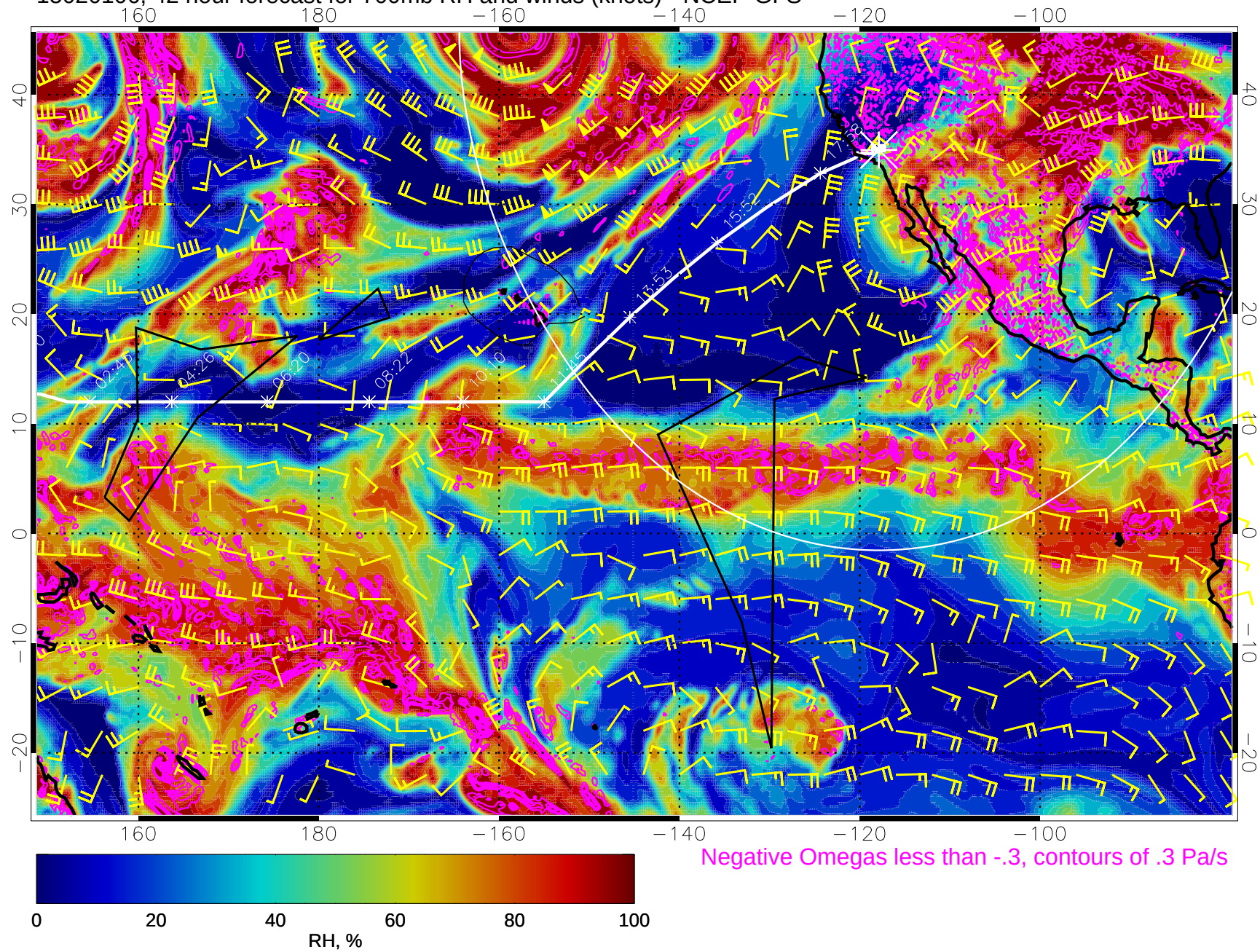
15020106, 42 hour forecast for 700mb RH and winds (knots) - NCEP GFS
