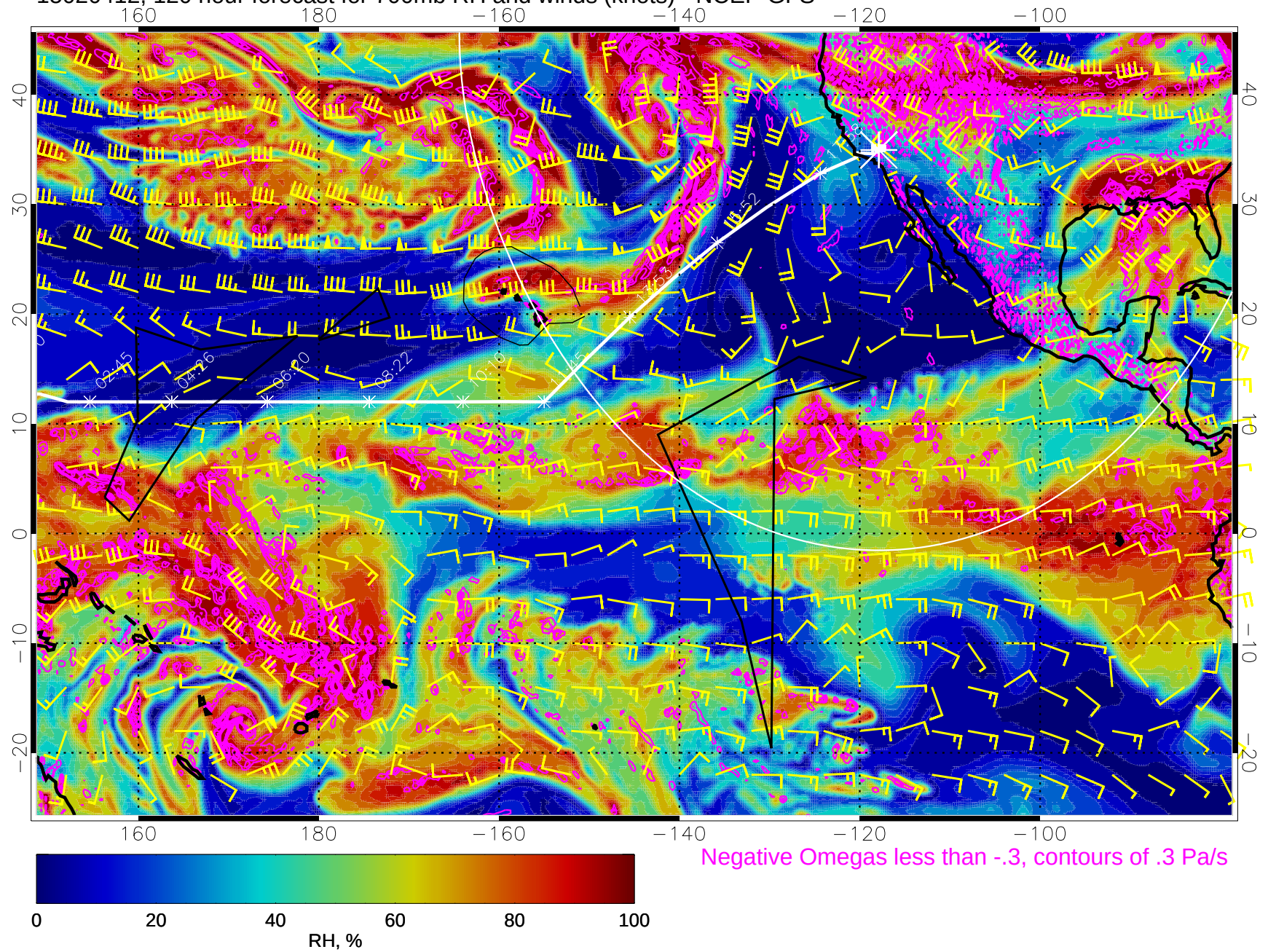
15020412, 120 hour forecast for 700mb RH and winds (knots) - NCEP GFS
