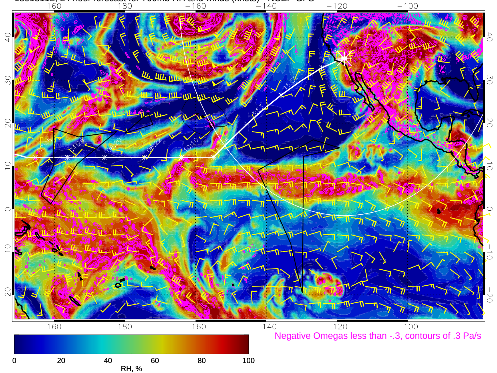
15013112, 24 hour forecast for 700mb RH and winds (knots) - NCEP GFS
