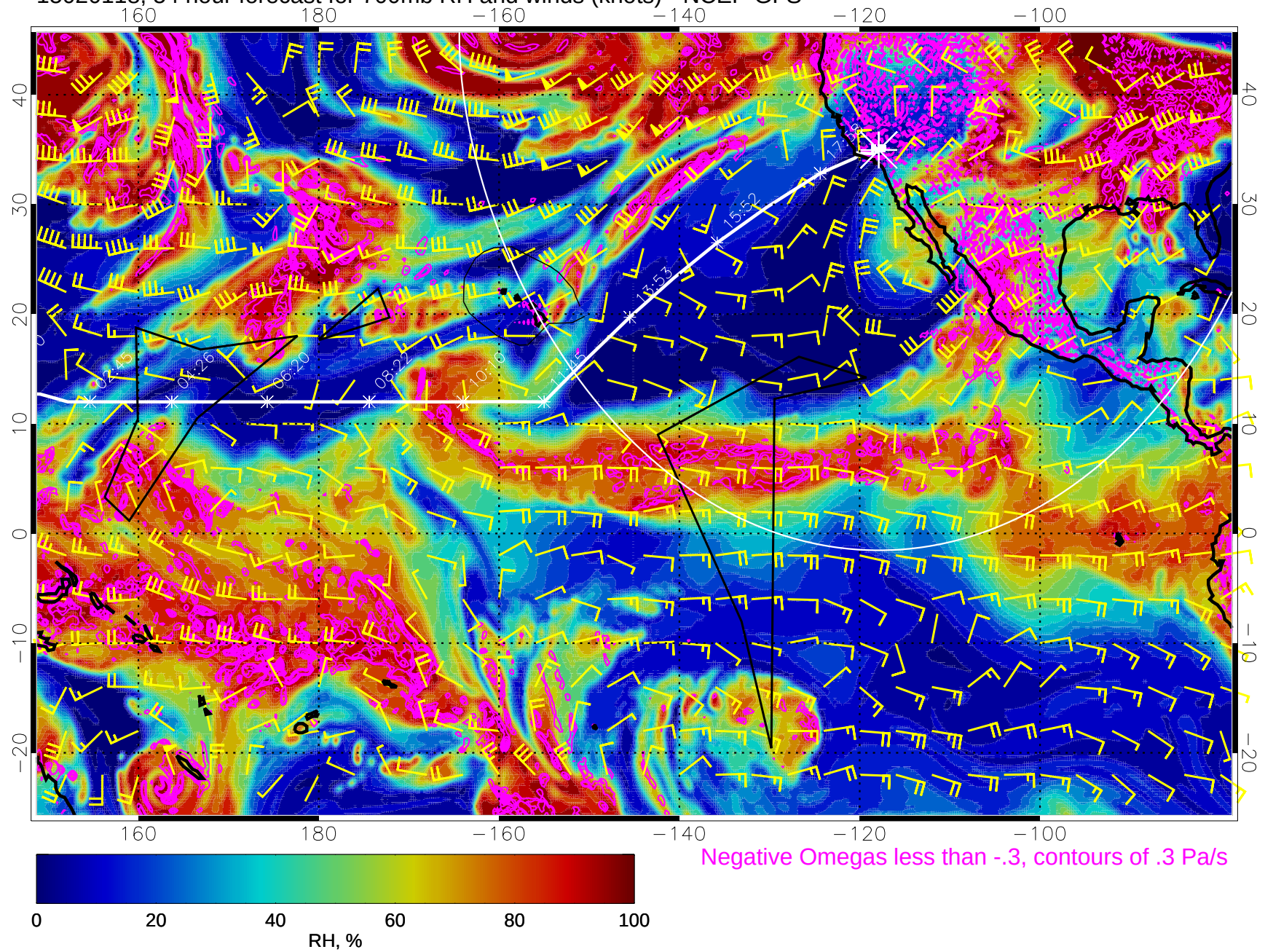
15020118, 54 hour forecast for 700mb RH and winds (knots) - NCEP GFS
