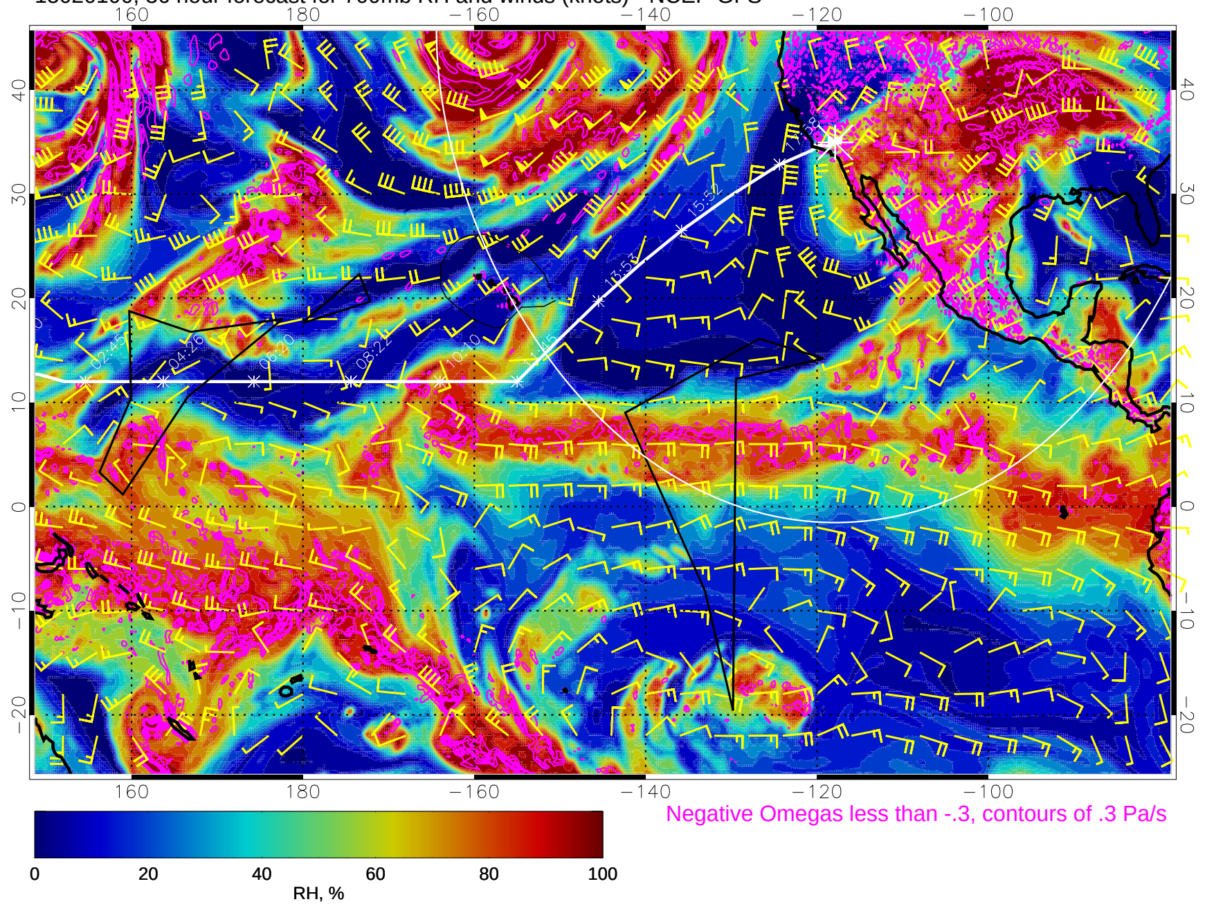
15020100, 36 hour forecast for 700mb RH and winds (knots) - NCEP GFS
