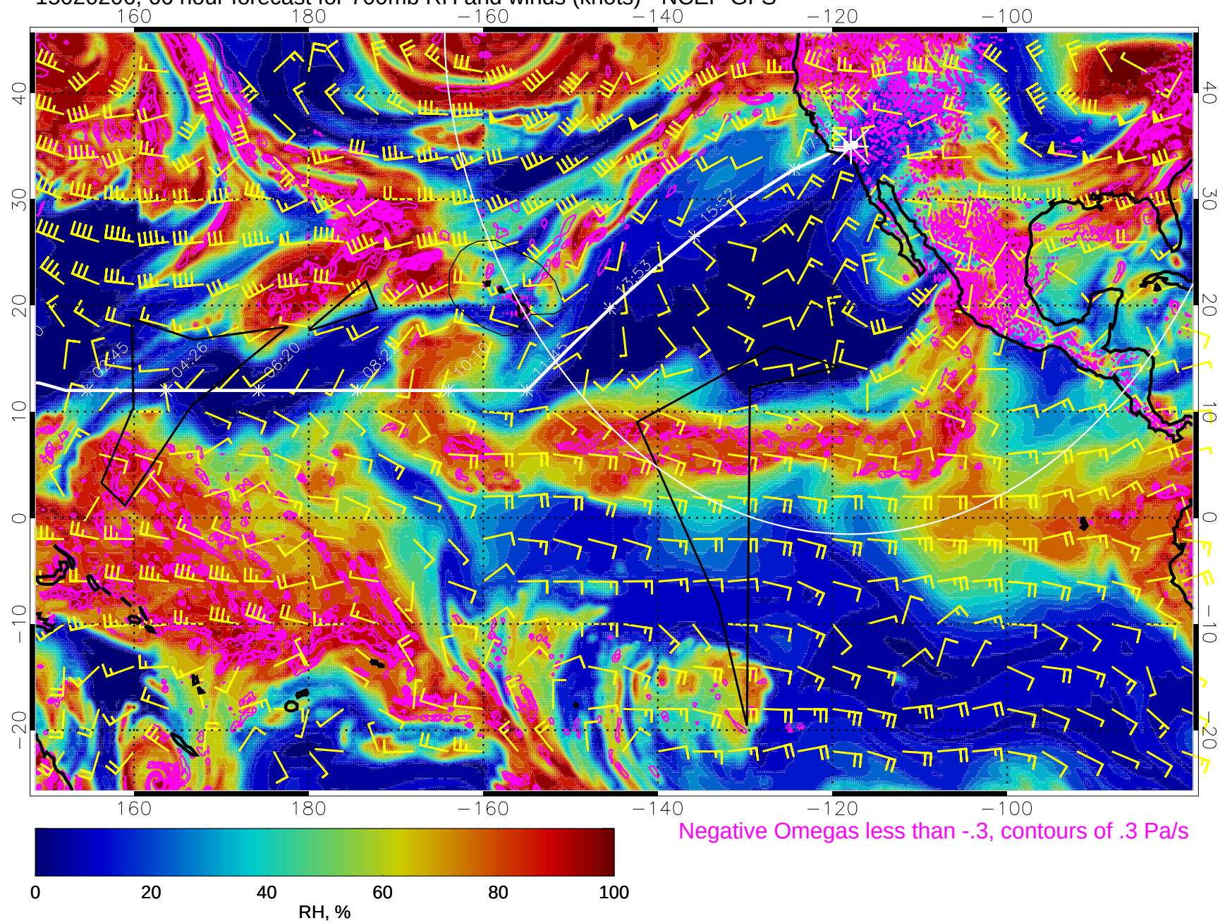
15020206, 66 hour forecast for 700mb RH and winds (knots) - NCEP GFS
