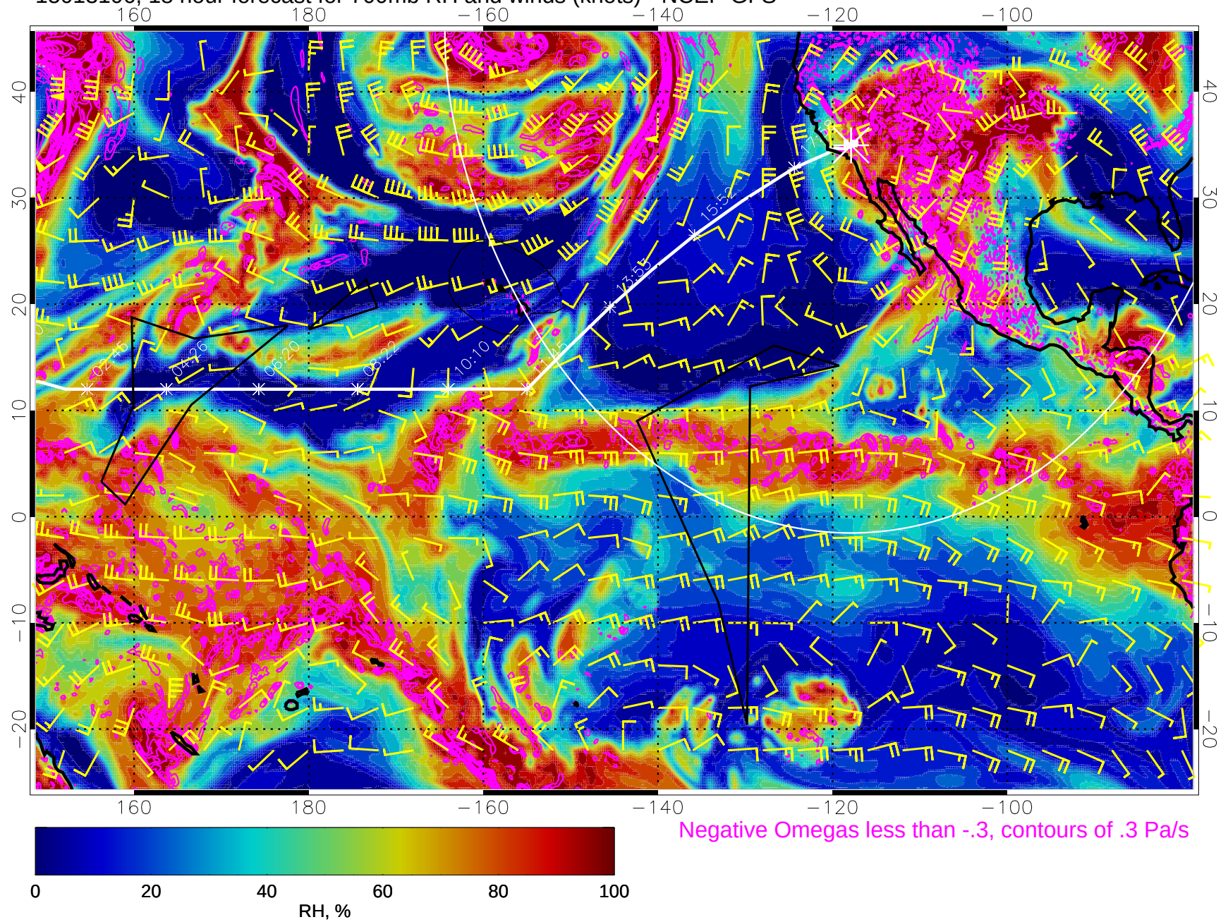
15013106, 18 hour forecast for 700mb RH and winds (knots) - NCEP GFS
