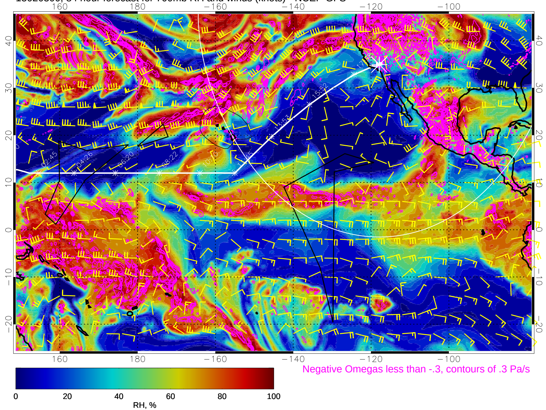
15020300, 84 hour forecast for 700mb RH and winds (knots) - NCEP GFS
