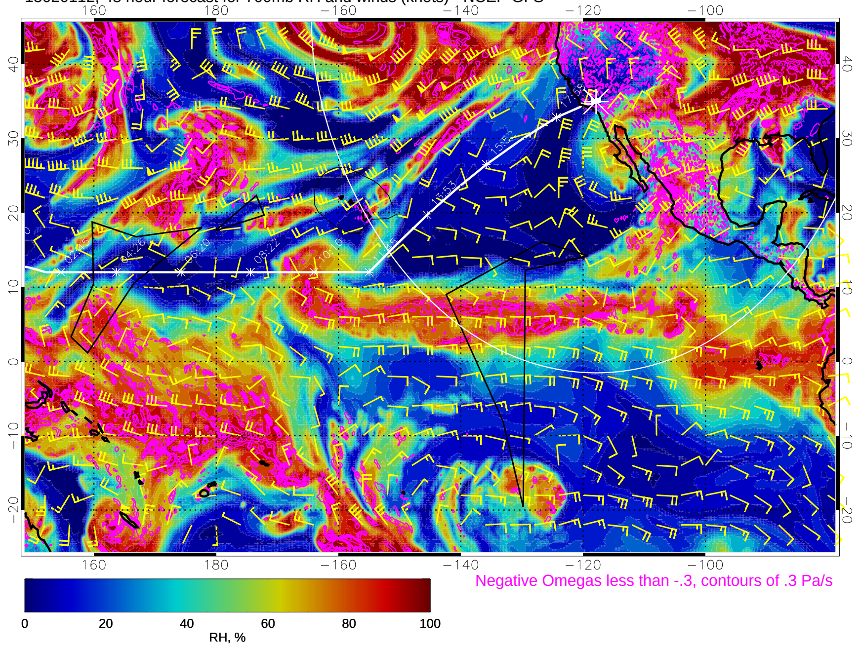
15020112, 48 hour forecast for 700mb RH and winds (knots) - NCEP GFS
