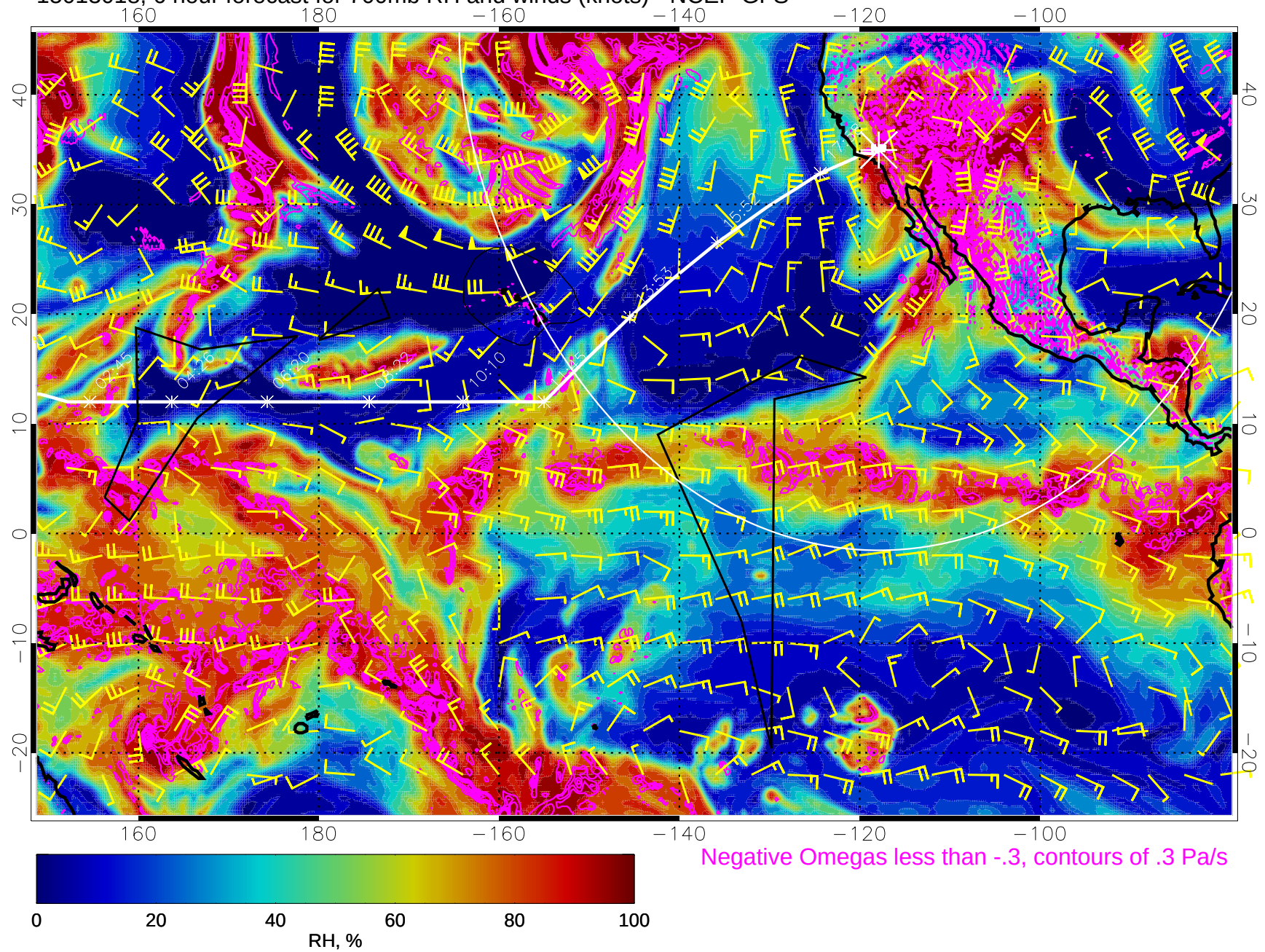
15013018, 6 hour forecast for 700mb RH and winds (knots) - NCEP GFS
