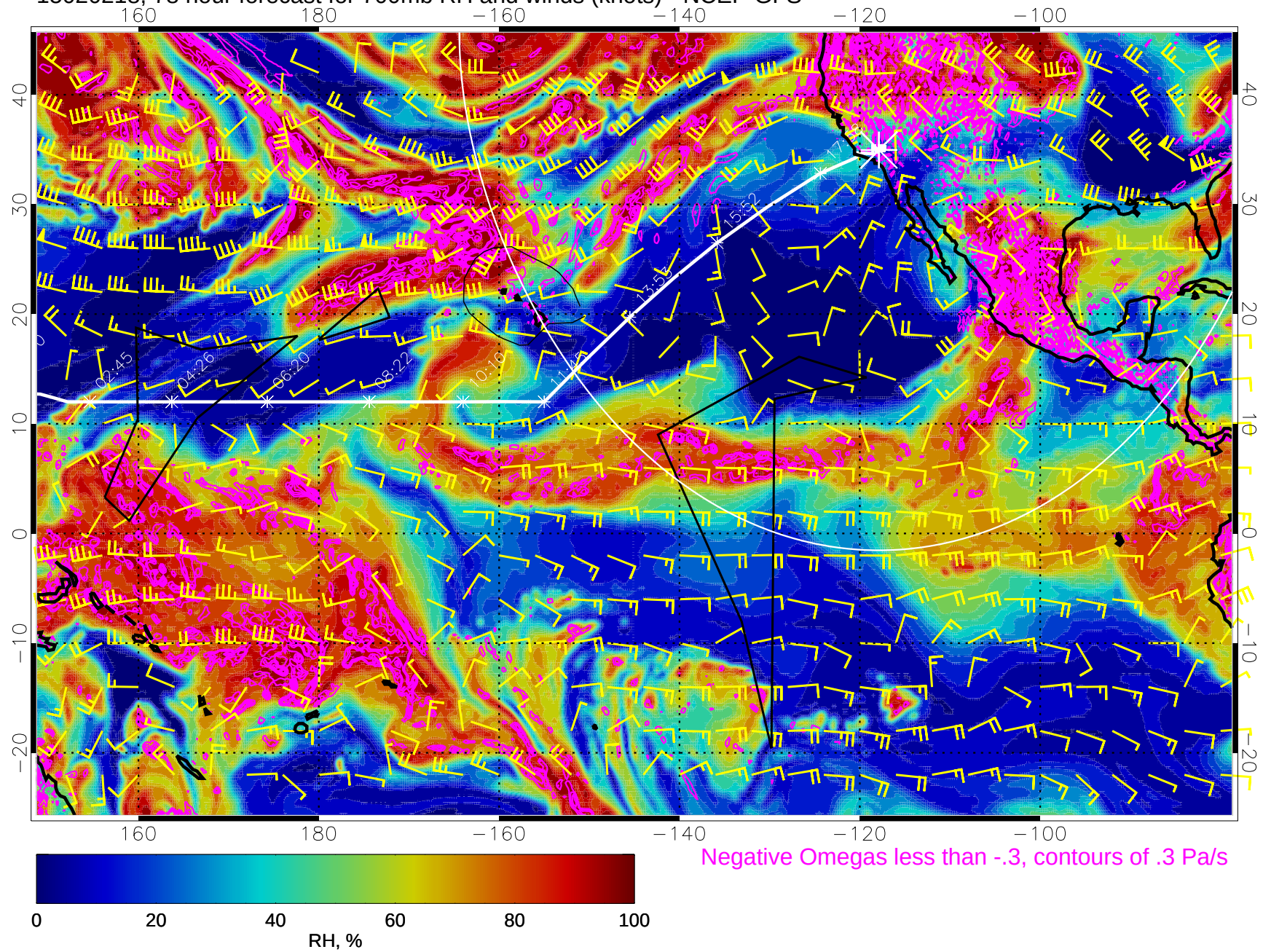
15020218, 78 hour forecast for 700mb RH and winds (knots) - NCEP GFS
