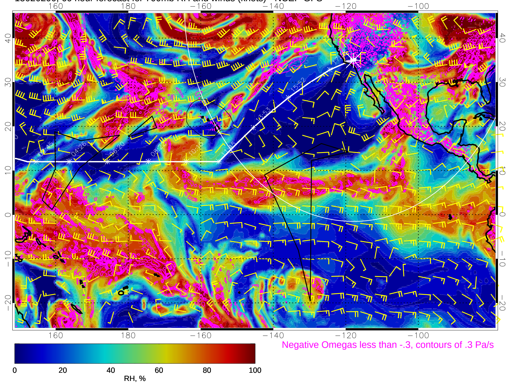
15020200, 60 hour forecast for 700mb RH and winds (knots) - NCEP GFS
