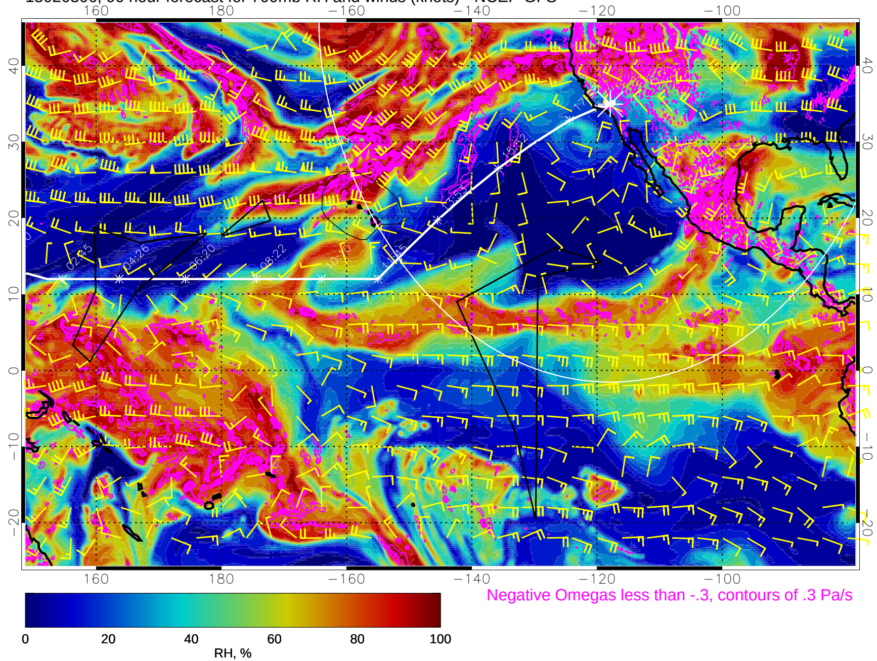
15020306, 90 hour forecast for 700mb RH and winds (knots) - NCEP GFS
