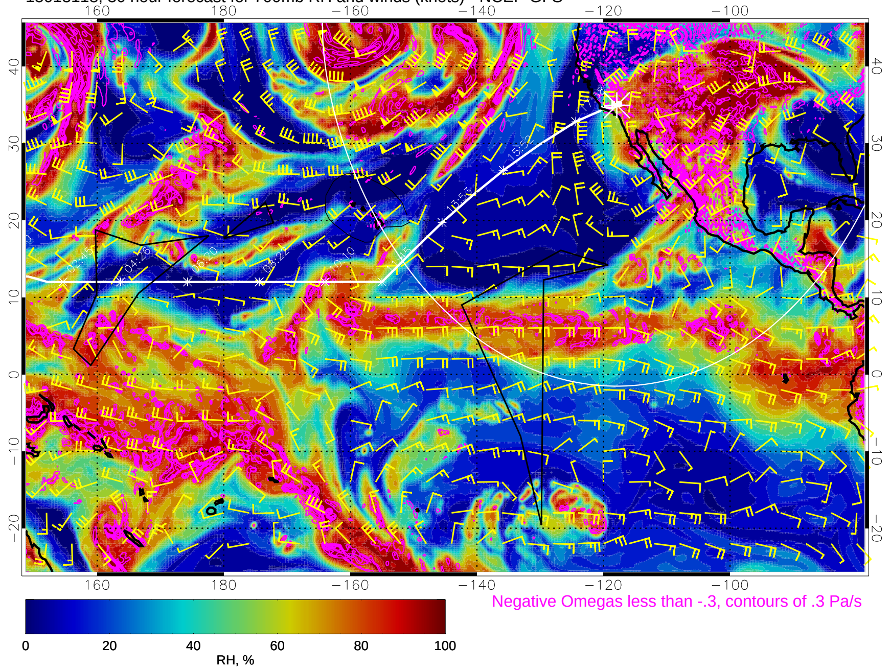
15013118, 30 hour forecast for 700mb RH and winds (knots) - NCEP GFS
