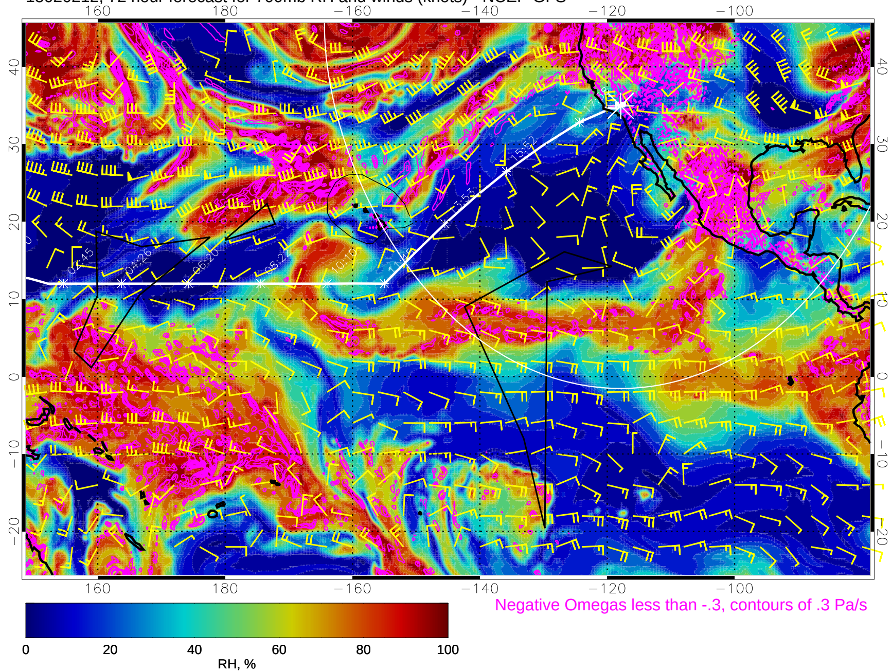
15020212, 72 hour forecast for 700mb RH and winds (knots) - NCEP GFS
