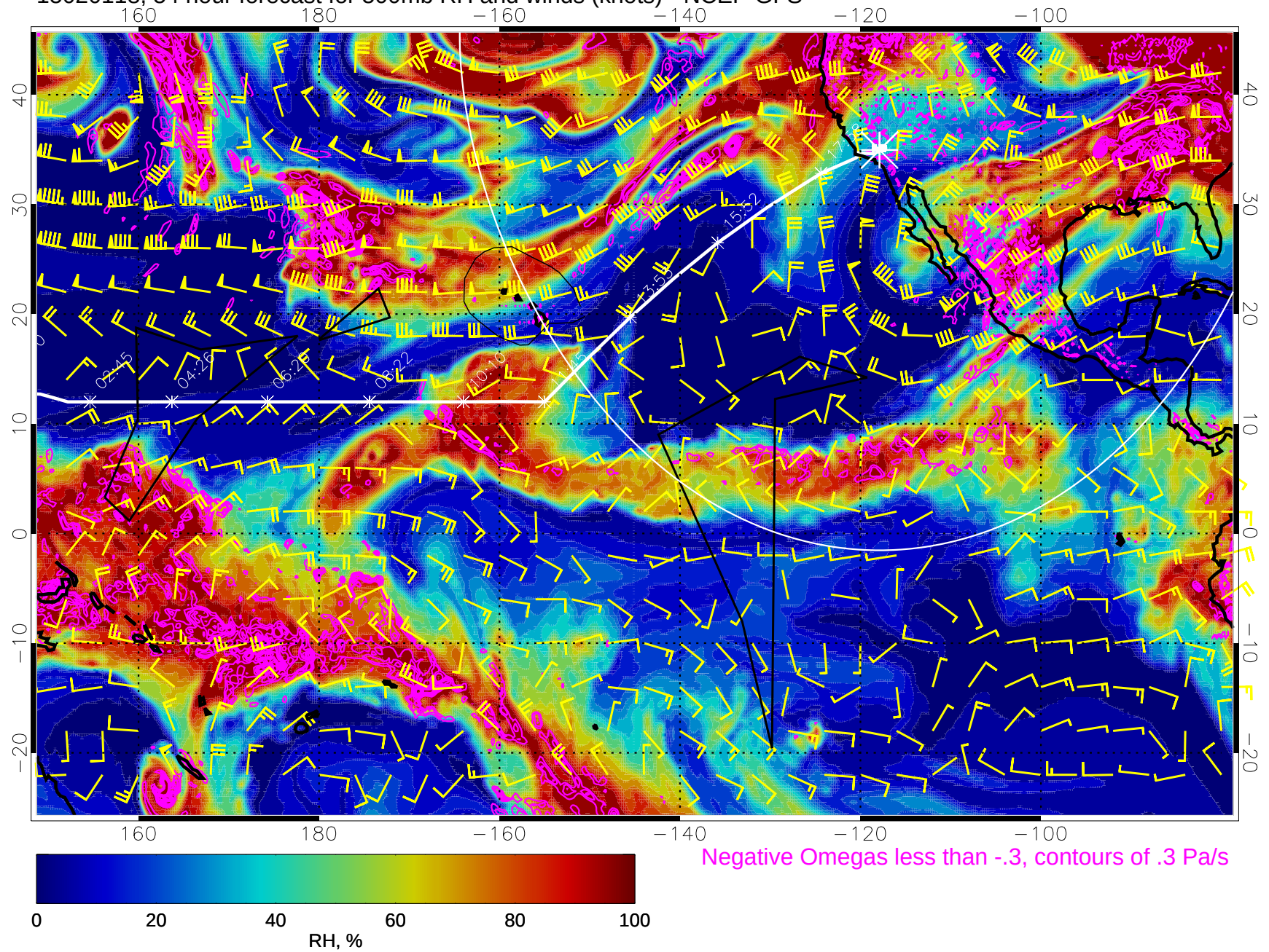
15020118, 54 hour forecast for 500mb RH and winds (knots) - NCEP GFS
