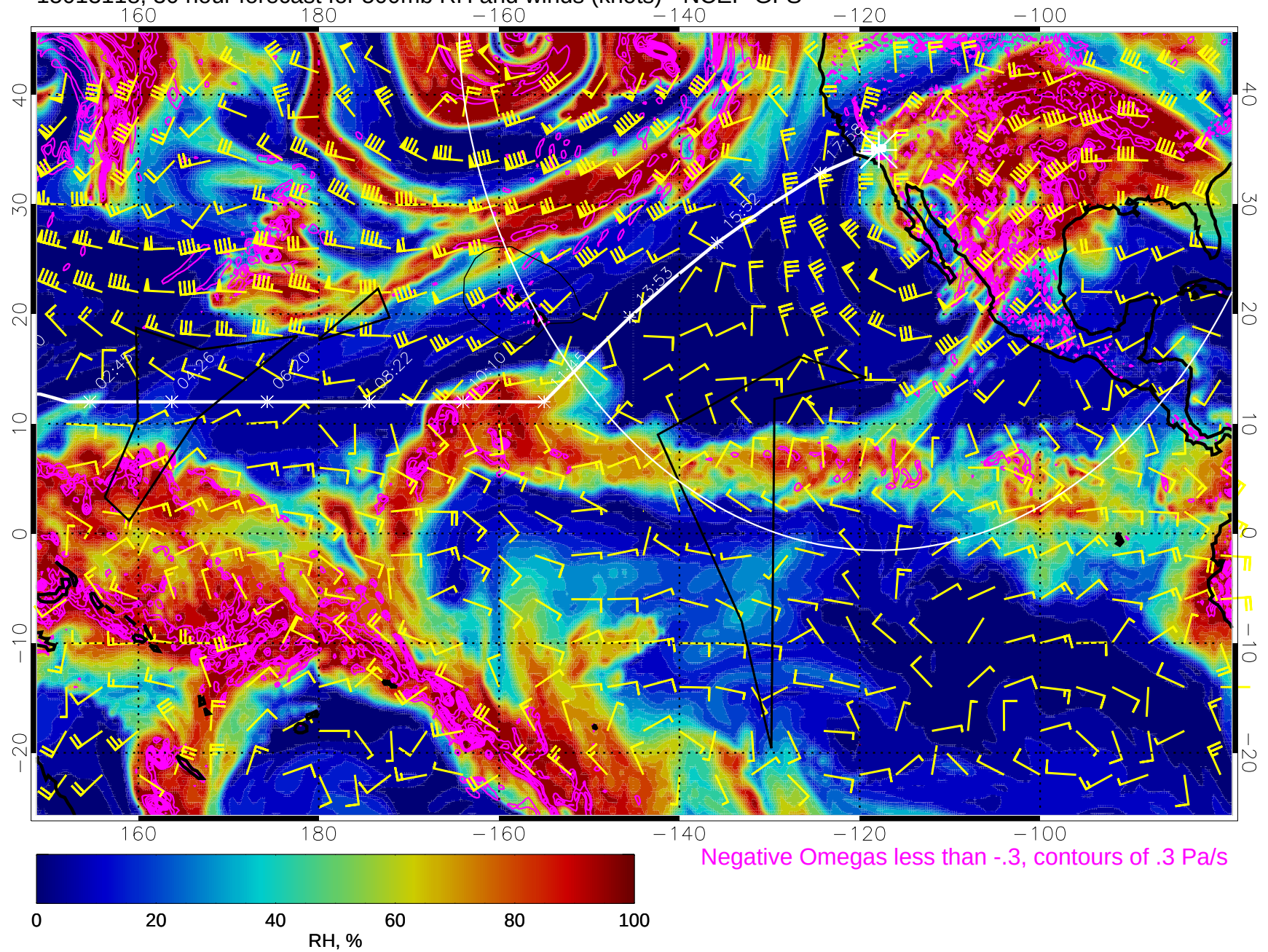
15013118, 30 hour forecast for 500mb RH and winds (knots) - NCEP GFS
