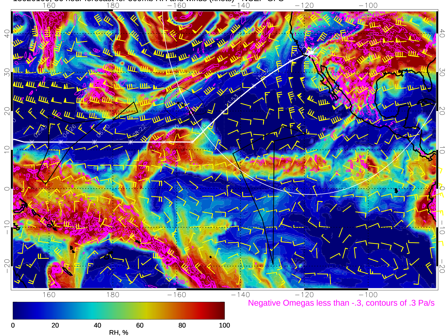
15020100, 36 hour forecast for 500mb RH and winds (knots) - NCEP GFS
