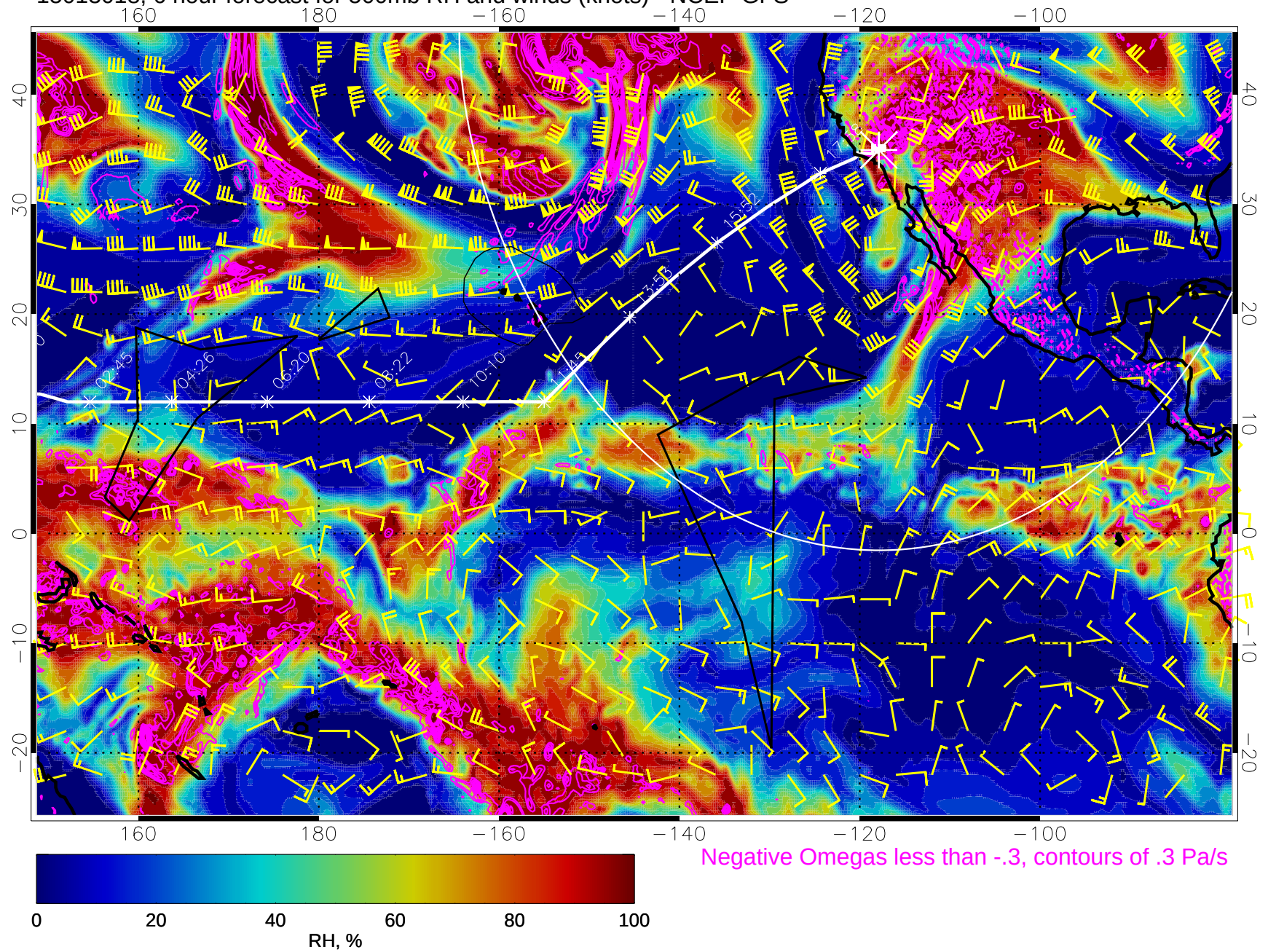
15013018, 6 hour forecast for 500mb RH and winds (knots) - NCEP GFS
