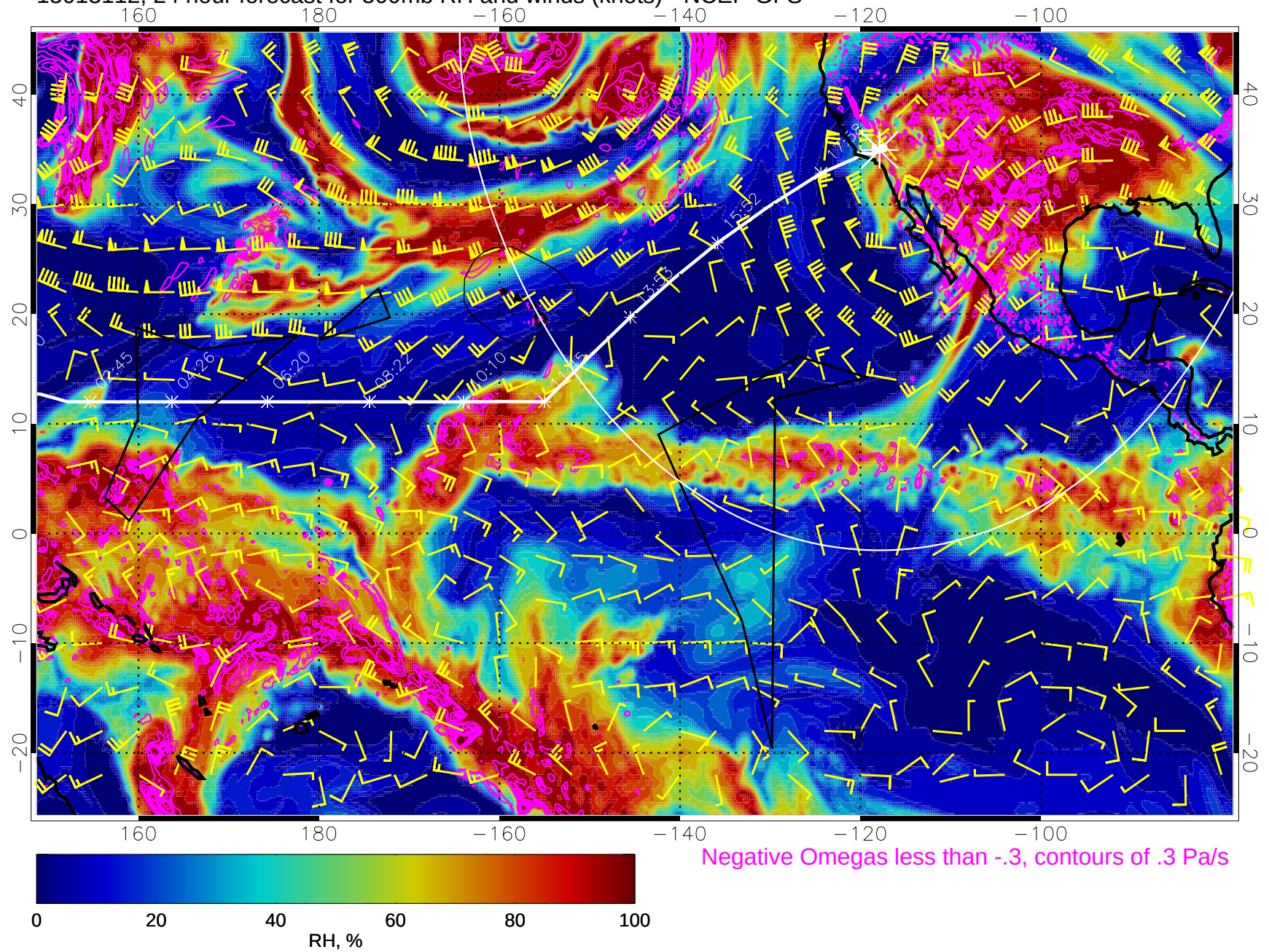
15013112, 24 hour forecast for 500mb RH and winds (knots) - NCEP GFS
