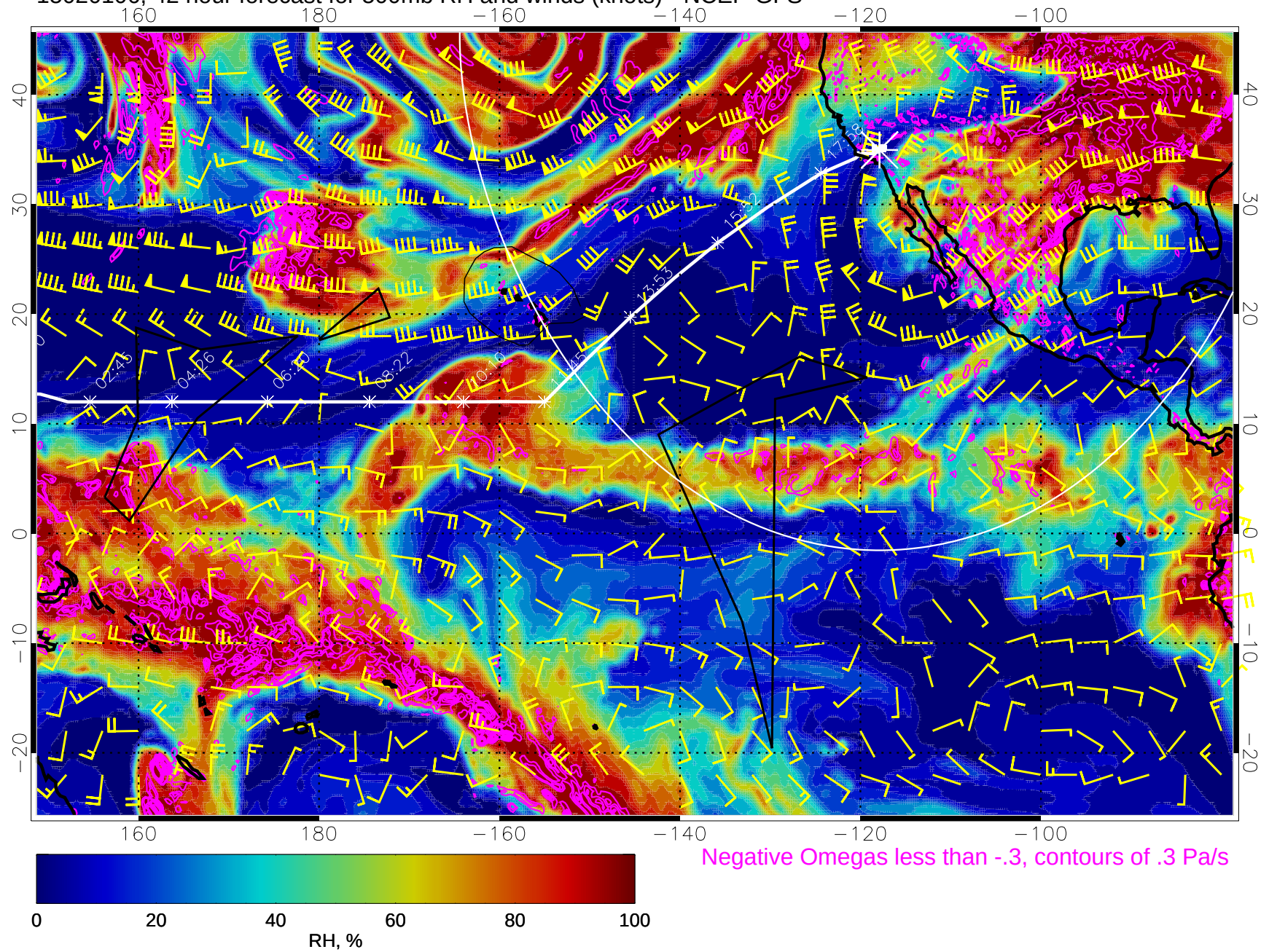
15020106, 42 hour forecast for 500mb RH and winds (knots) - NCEP GFS
