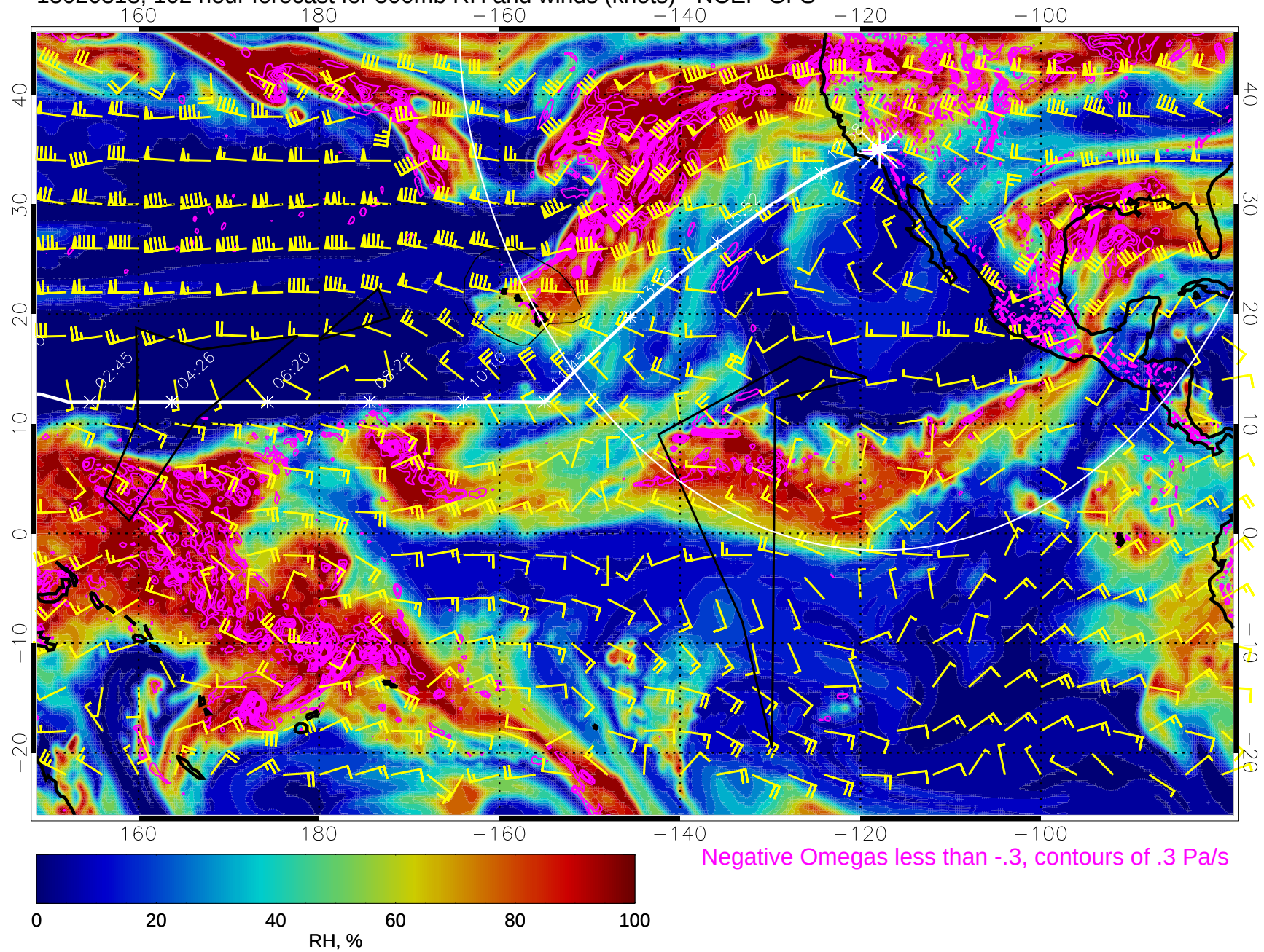
15020318, 102 hour forecast for 500mb RH and winds (knots) - NCEP GFS
