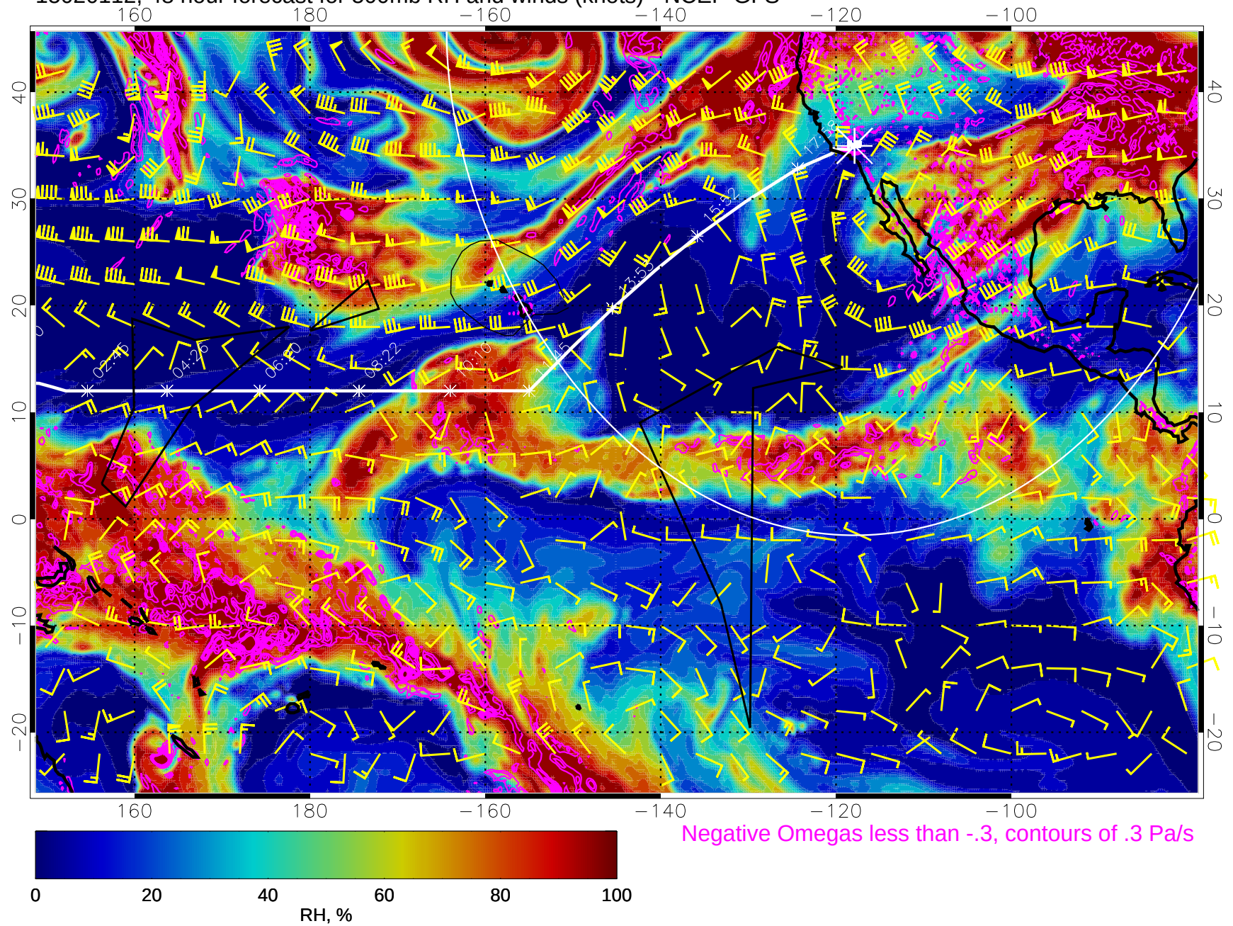
15020112, 48 hour forecast for 500mb RH and winds (knots) - NCEP GFS
