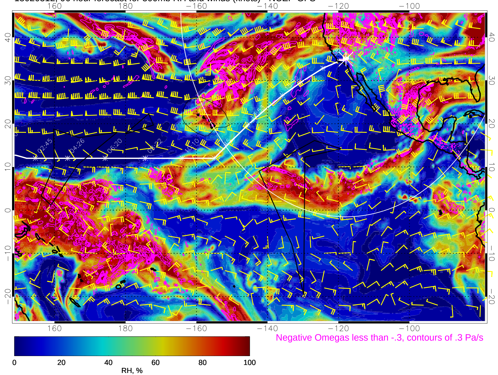
15020312, 96 hour forecast for 500mb RH and winds (knots) - NCEP GFS
