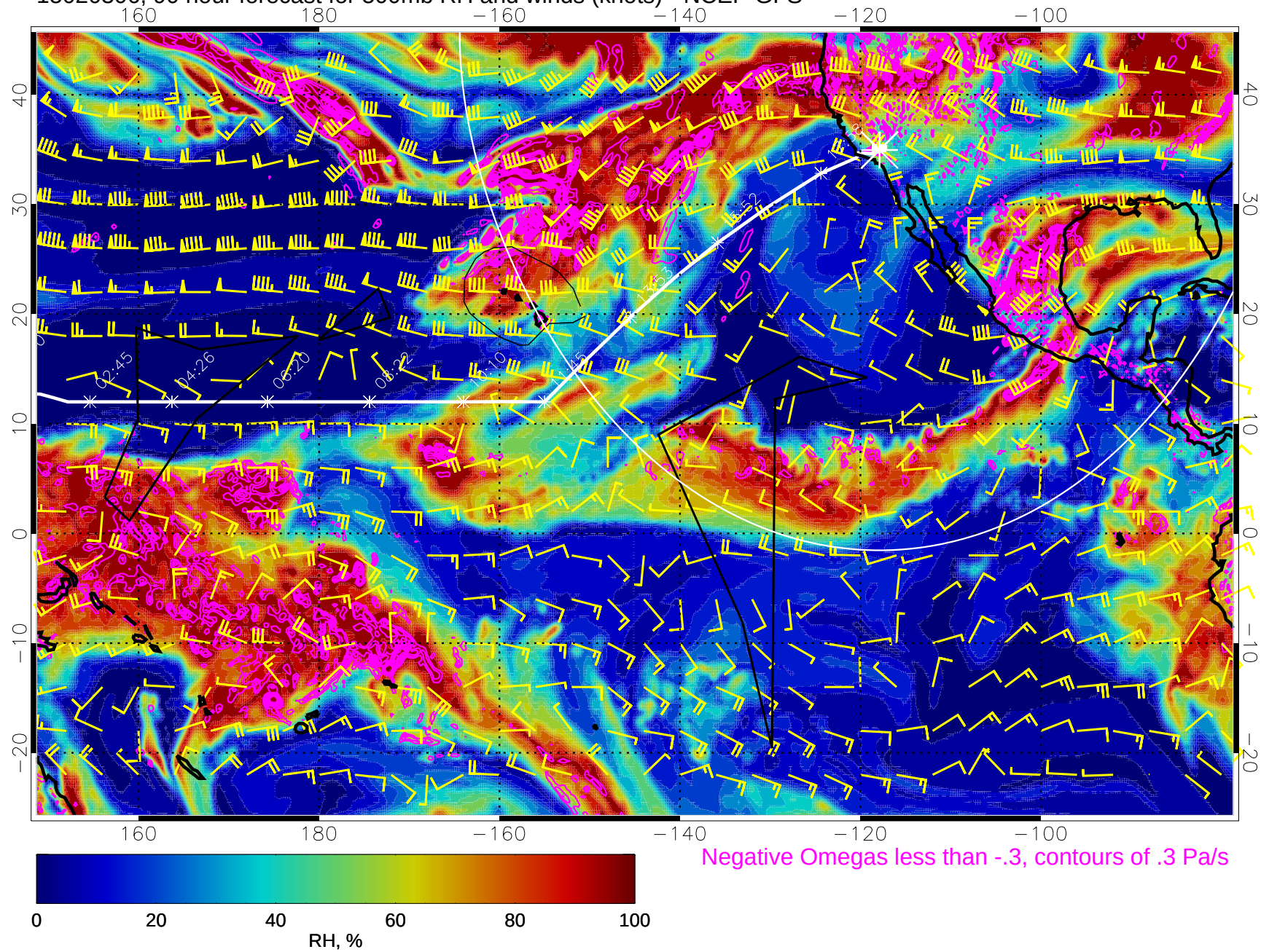
15020306, 90 hour forecast for 500mb RH and winds (knots) - NCEP GFS
