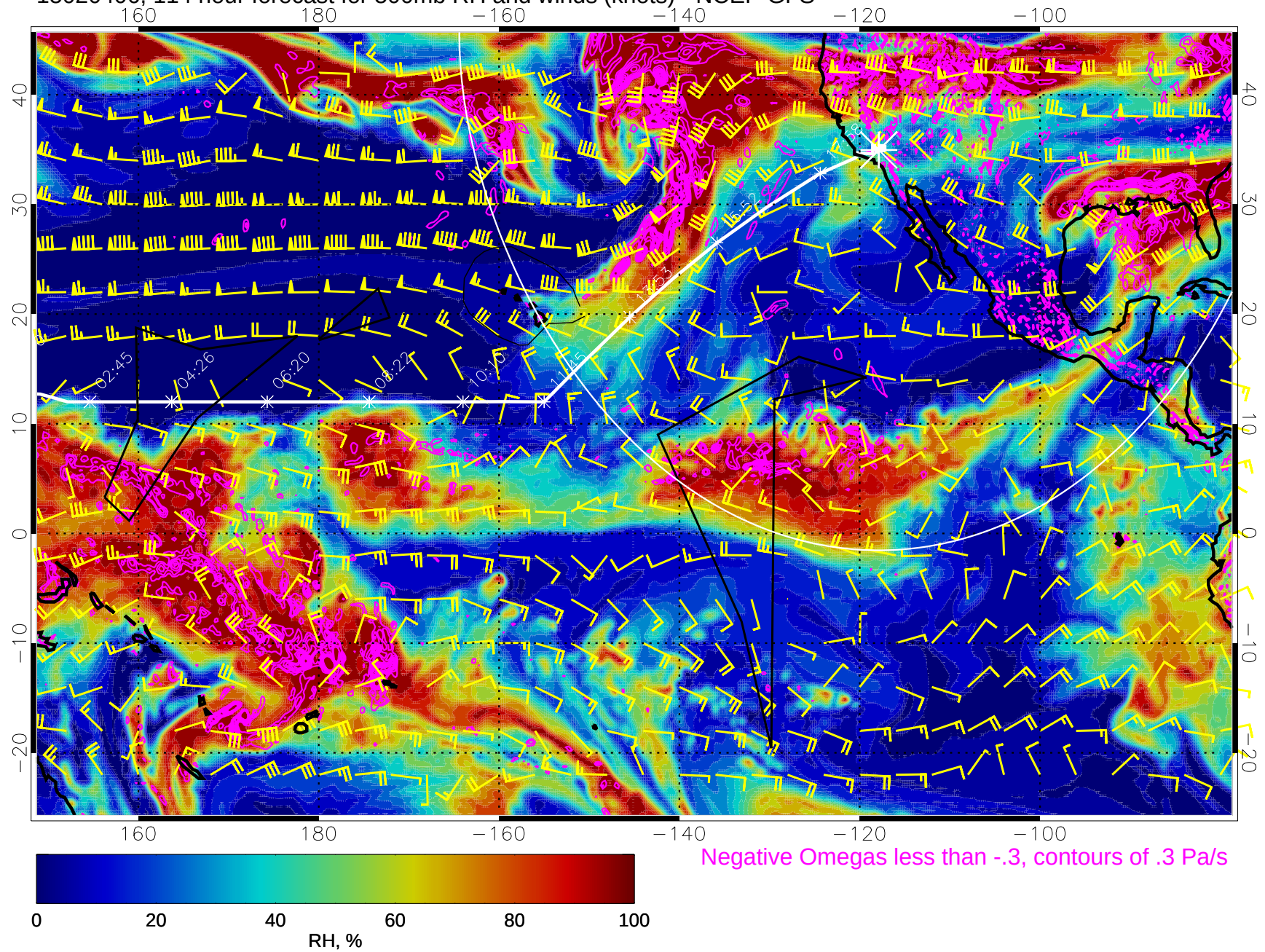
15020406, 114 hour forecast for 500mb RH and winds (knots) - NCEP GFS
