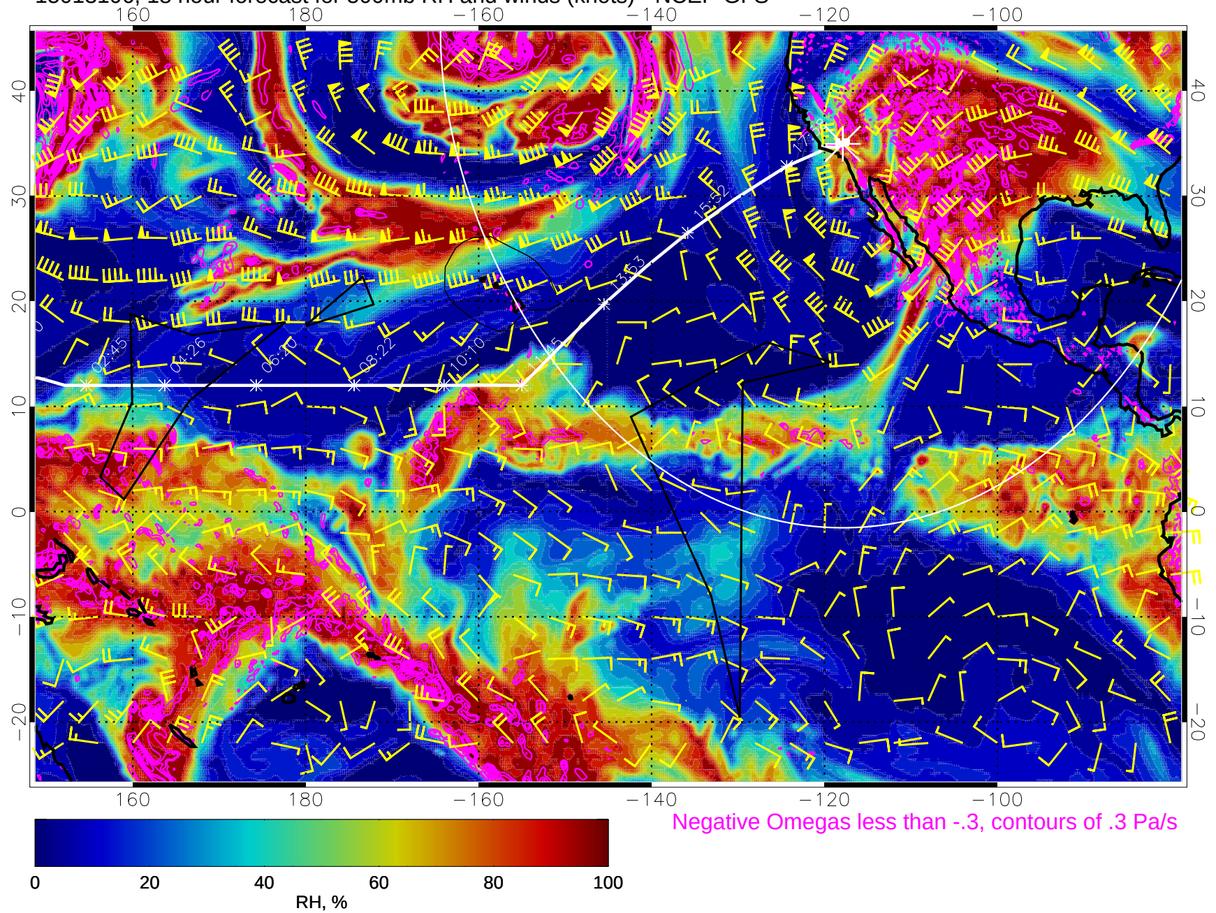
15013106, 18 hour forecast for 500mb RH and winds (knots) - NCEP GFS
