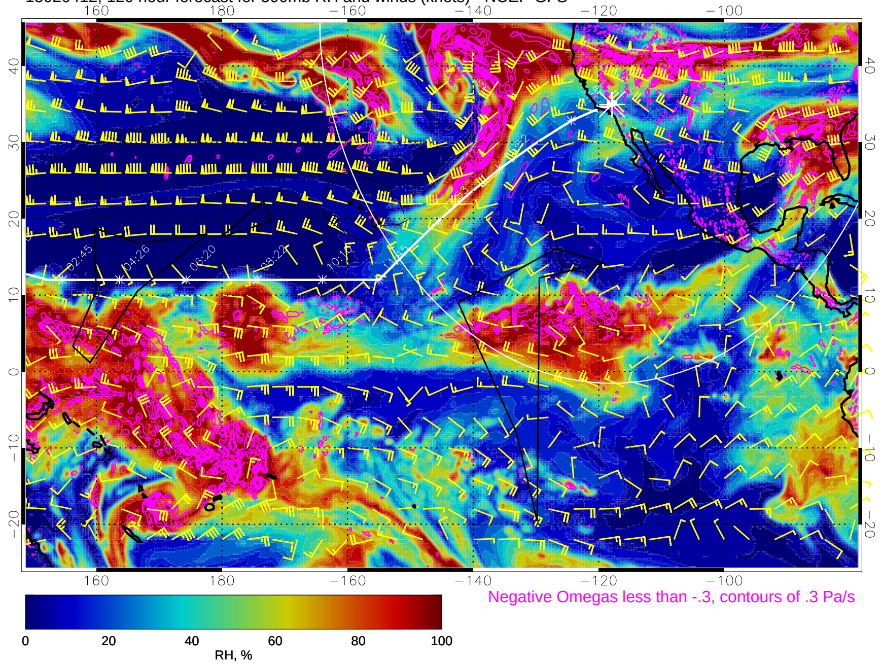
15020412, 120 hour forecast for 500mb RH and winds (knots) - NCEP GFS
