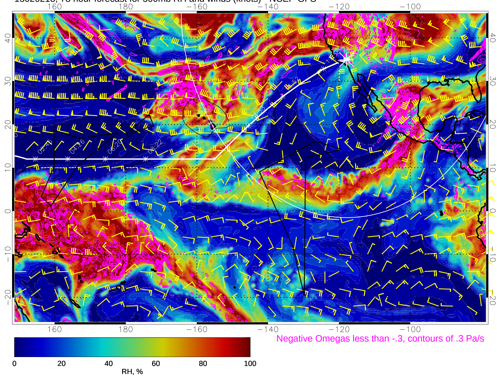
15020218, 78 hour forecast for 500mb RH and winds (knots) - NCEP GFS
