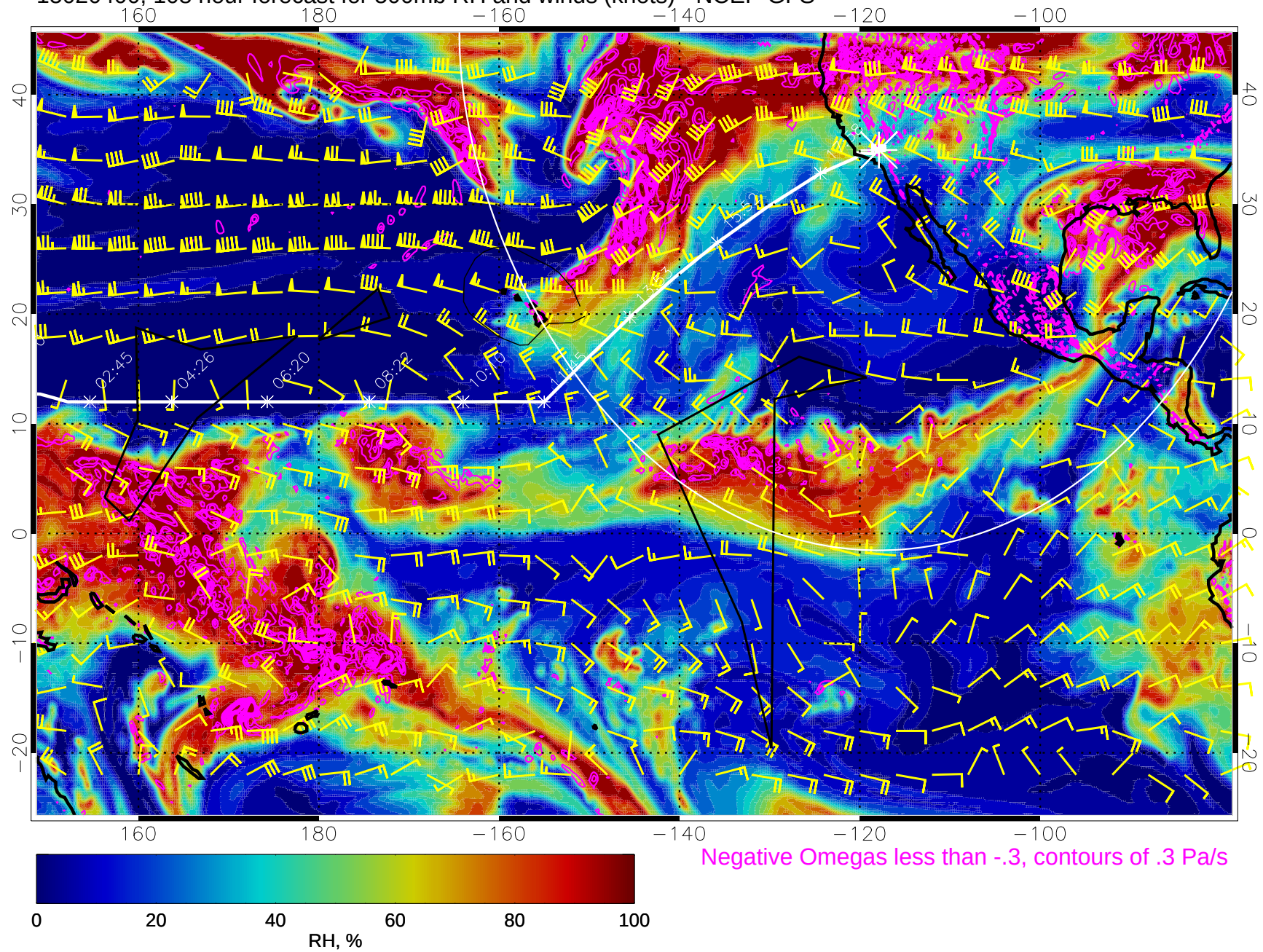
15020400, 108 hour forecast for 500mb RH and winds (knots) - NCEP GFS
