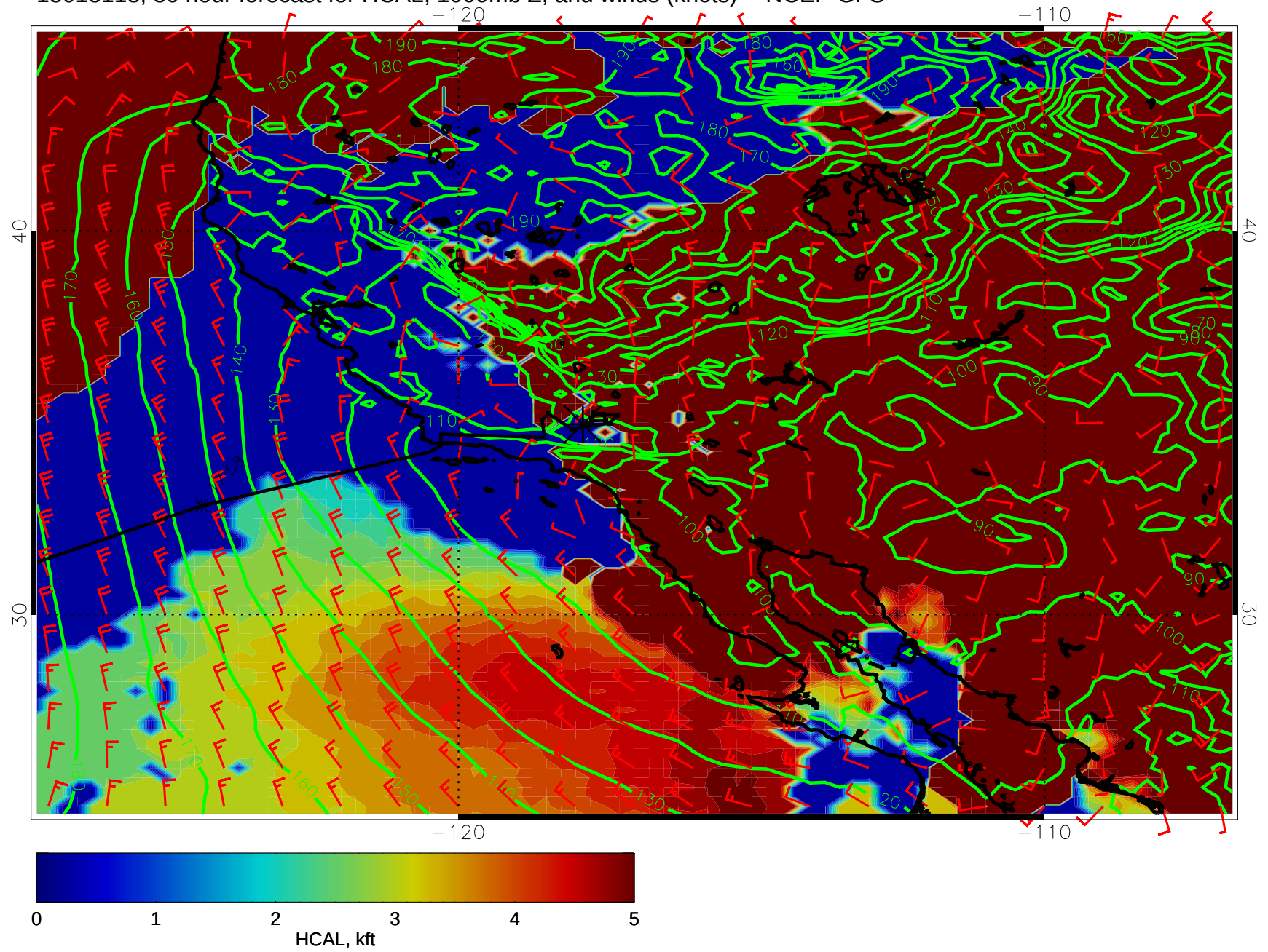
15013118, 30 hour forecast for HCAL, 1000mb Z, and winds (knots) -- NCEP GFS
