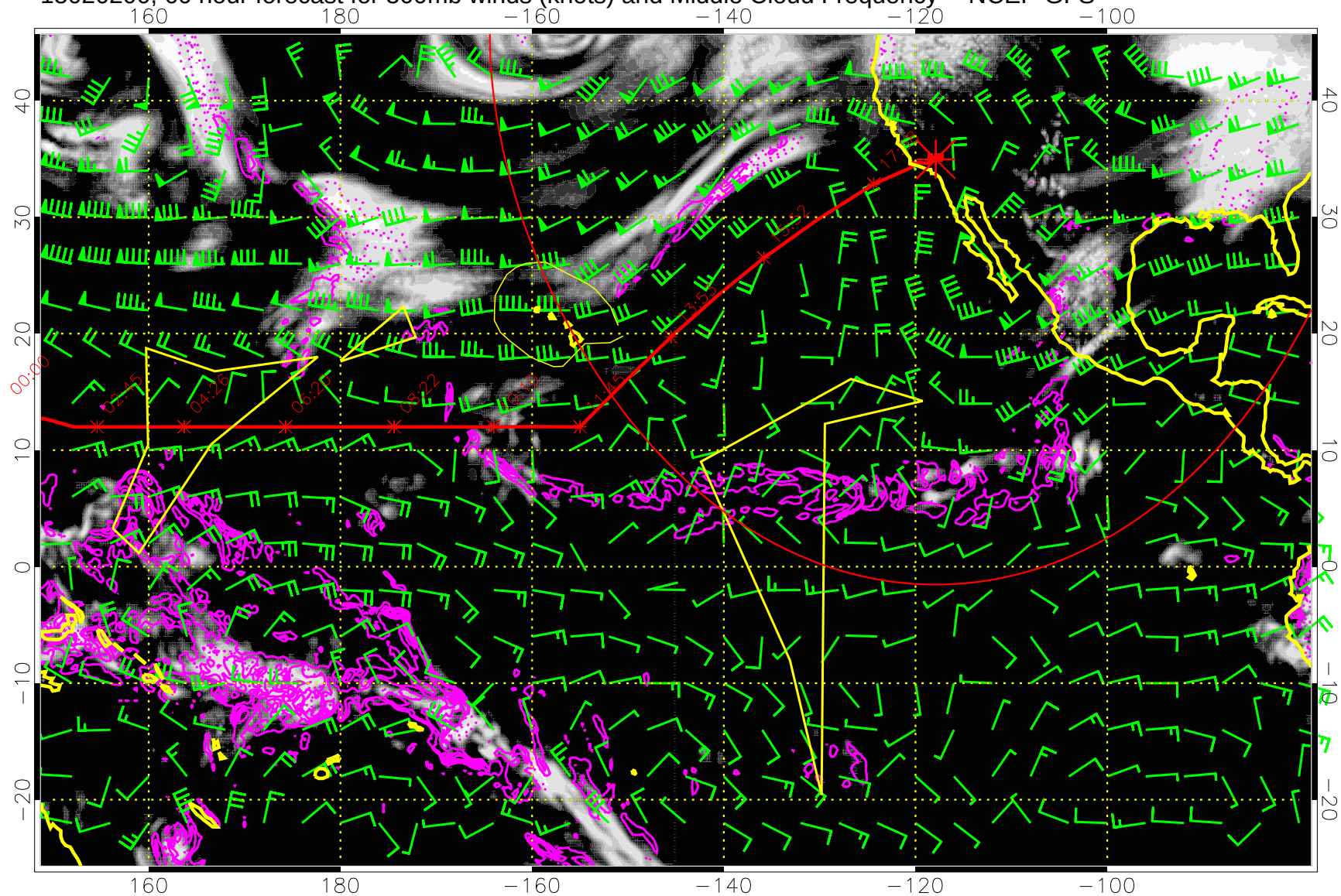
15020200, 60 hour forecast for 500mb winds (knots) and Middle Cloud Frequency -- NCEP GFS
