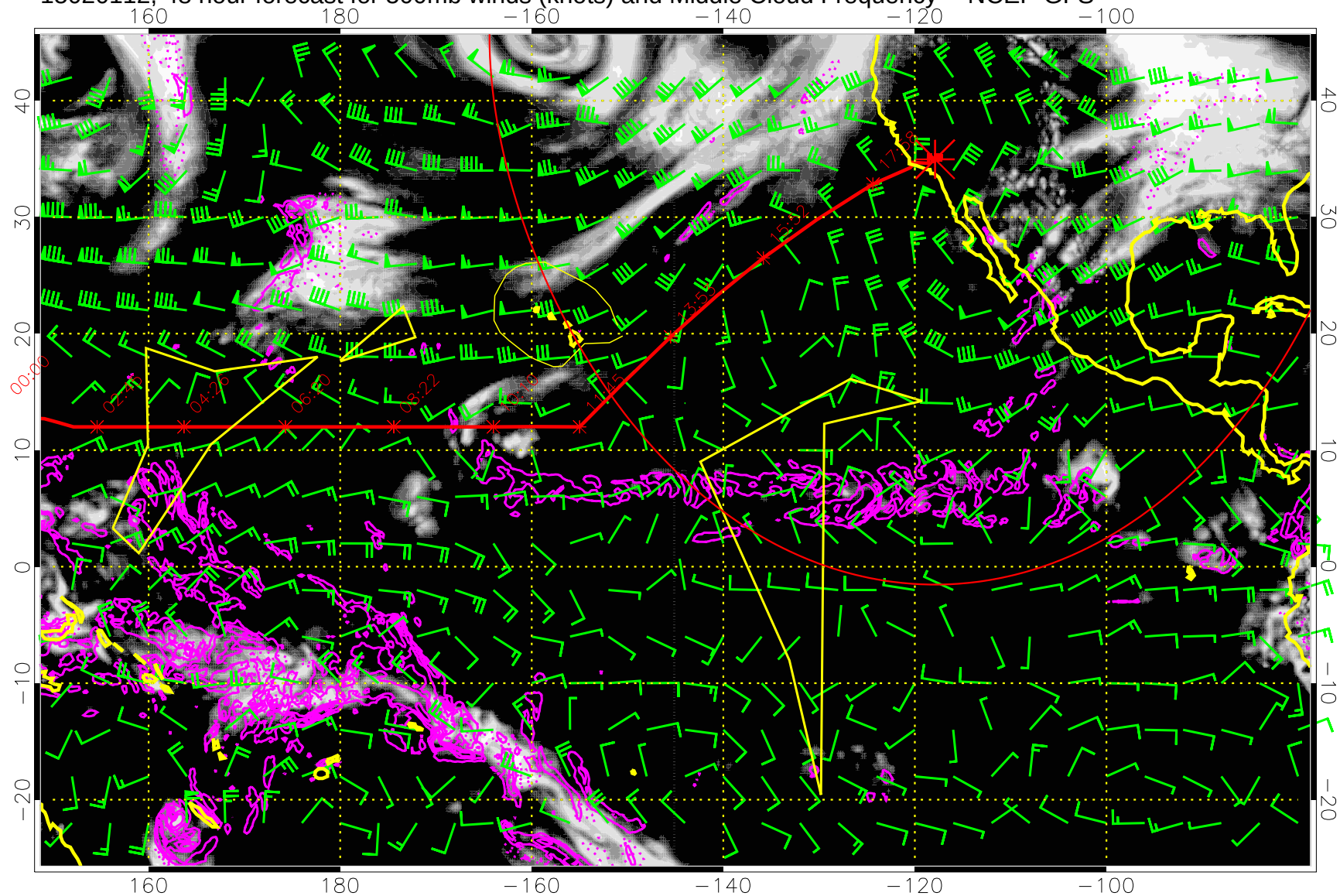
15020112, 48 hour forecast for 500mb winds (knots) and Middle Cloud Frequency -- NCEP GFS
