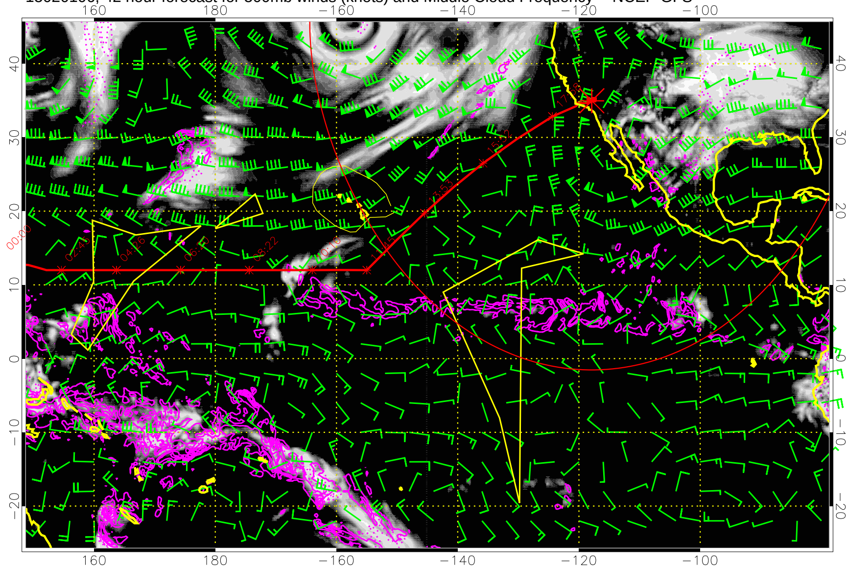
15020106, 42 hour forecast for 500mb winds (knots) and Middle Cloud Frequency -- NCEP GFS
