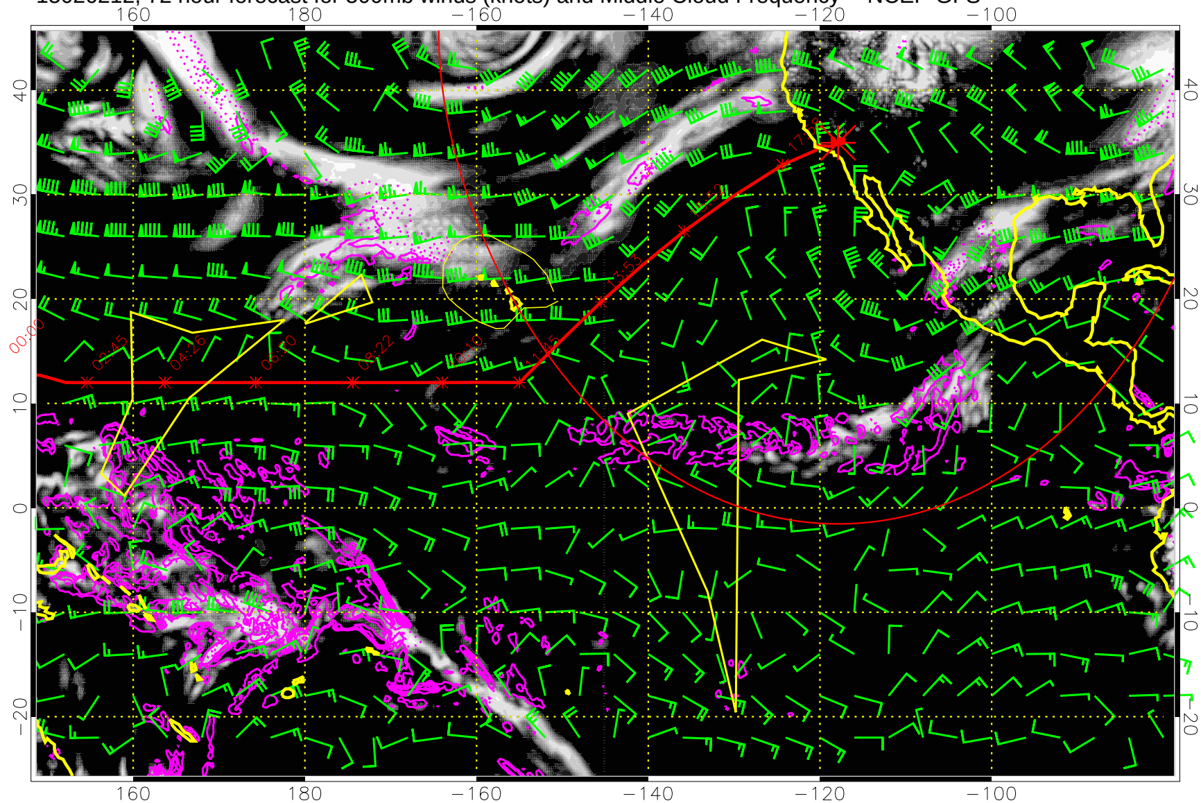
15020212, 72 hour forecast for 500mb winds (knots) and Middle Cloud Frequency -- NCEP GFS
