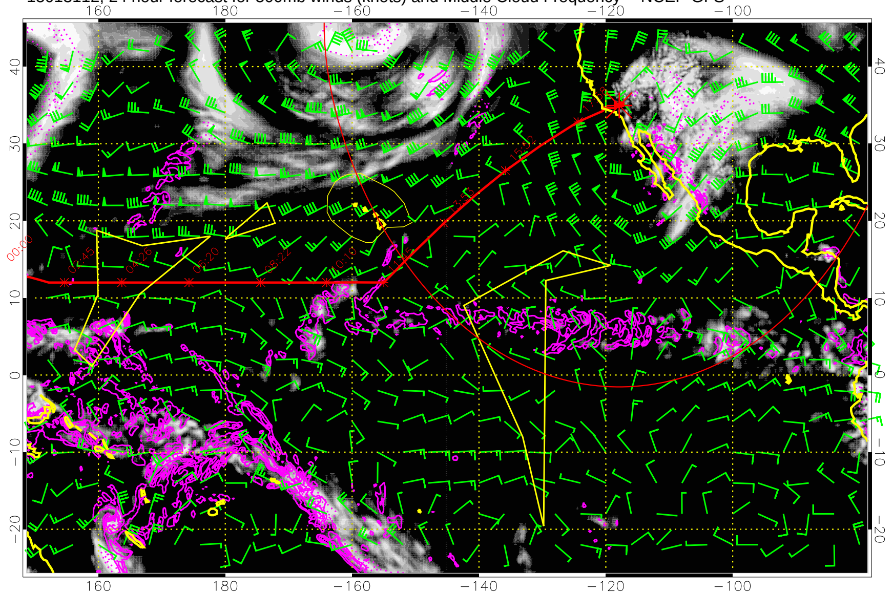
15013112, 24 hour forecast for 500mb winds (knots) and Middle Cloud Frequency -- NCEP GFS
