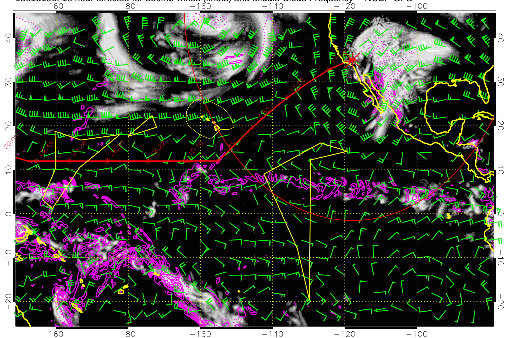
15013106, 18 hour forecast for 500mb winds (knots) and Middle Cloud Frequency -- NCEP GFS
