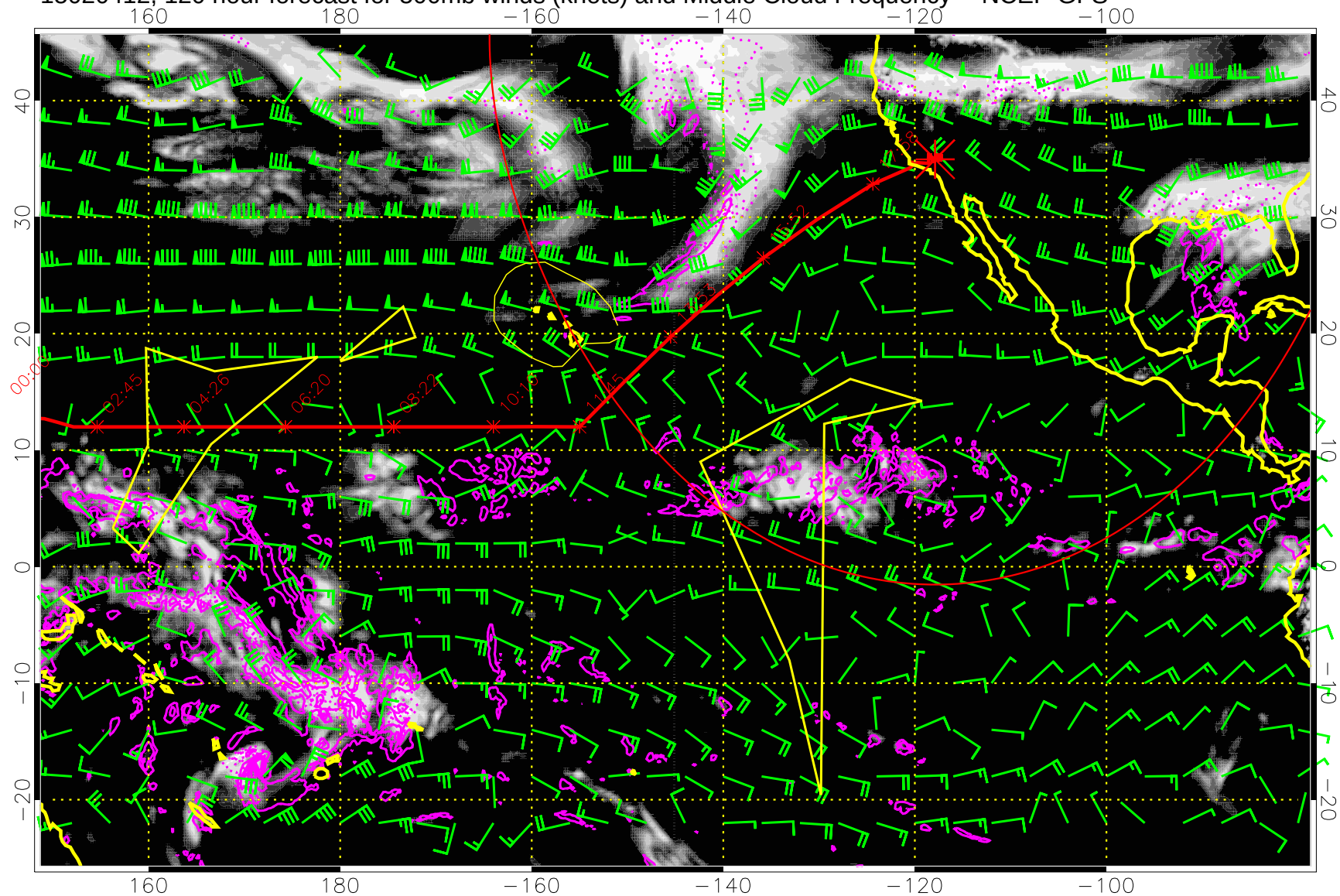
15020412, 120 hour forecast for 500mb winds (knots) and Middle Cloud Frequency -- NCEP GFS
