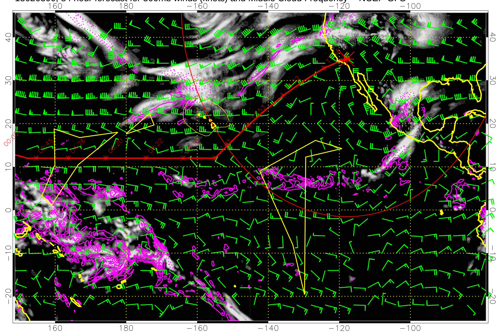
15020300, 84 hour forecast for 500mb winds (knots) and Middle Cloud Frequency -- NCEP GFS
