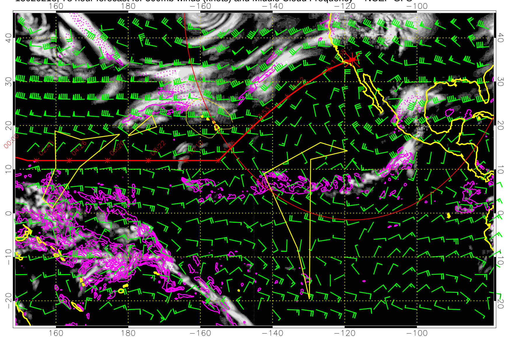
15020218, 78 hour forecast for 500mb winds (knots) and Middle Cloud Frequency -- NCEP GFS
