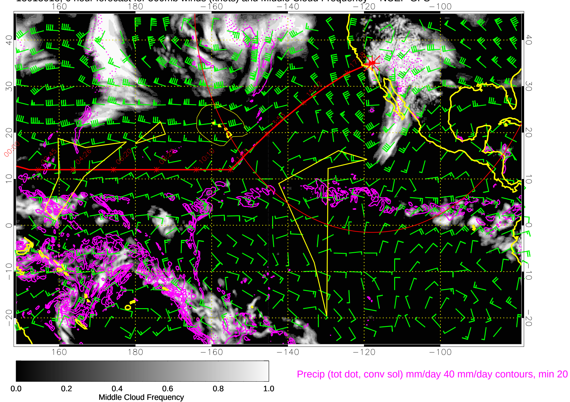
15013018, 6 hour forecast for 500mb winds (knots) and Middle Cloud Frequency -- NCEP GFS
