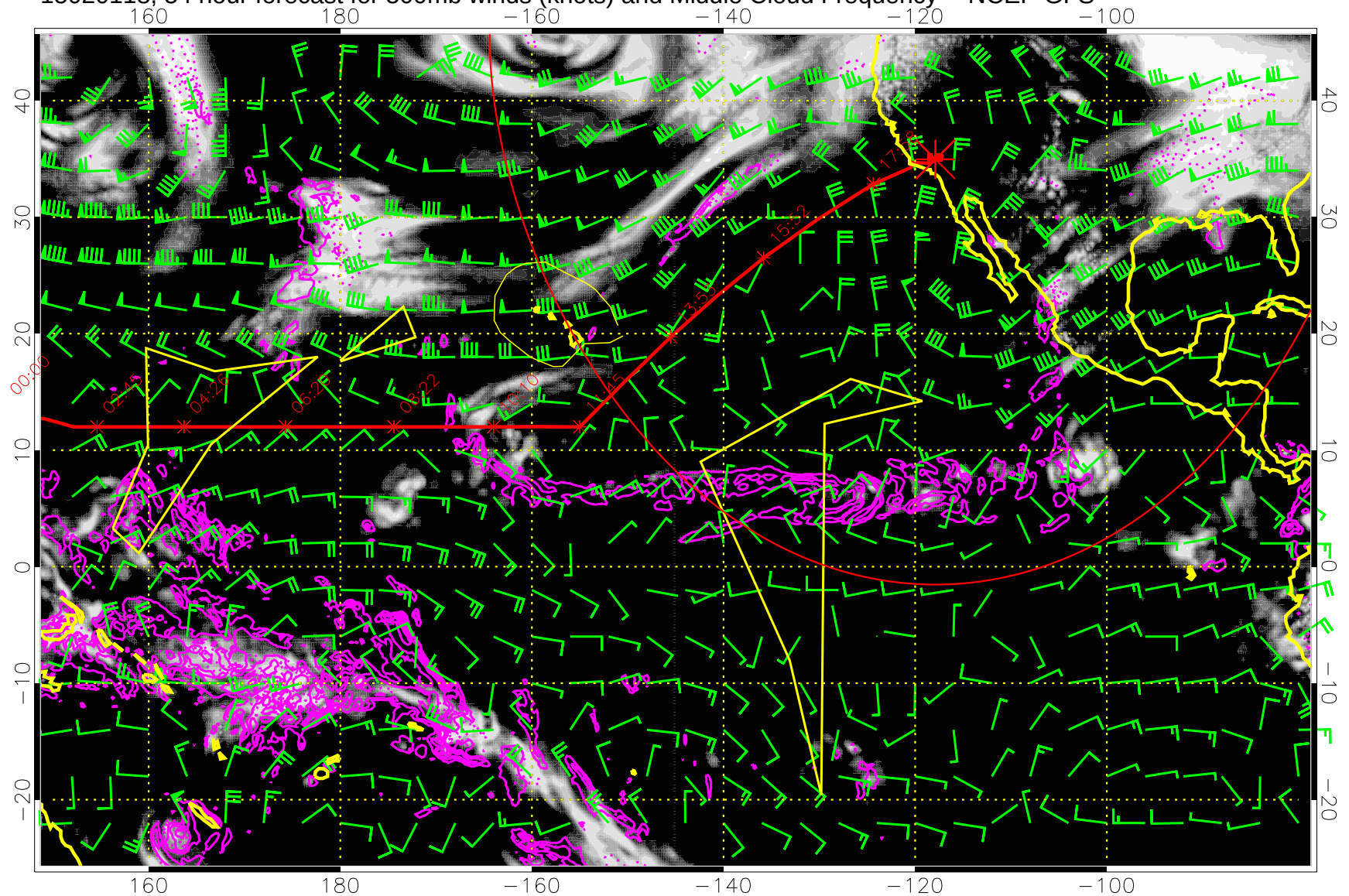
15020118, 54 hour forecast for 500mb winds (knots) and Middle Cloud Frequency -- NCEP GFS
