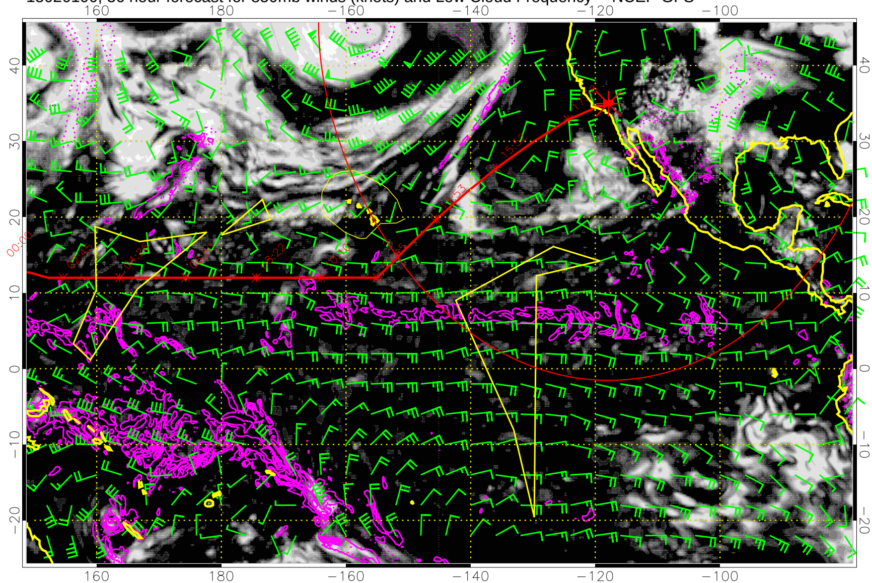
15020100, 36 hour forecast for 850mb winds (knots) and Low Cloud Frequency -- NCEP GFS
