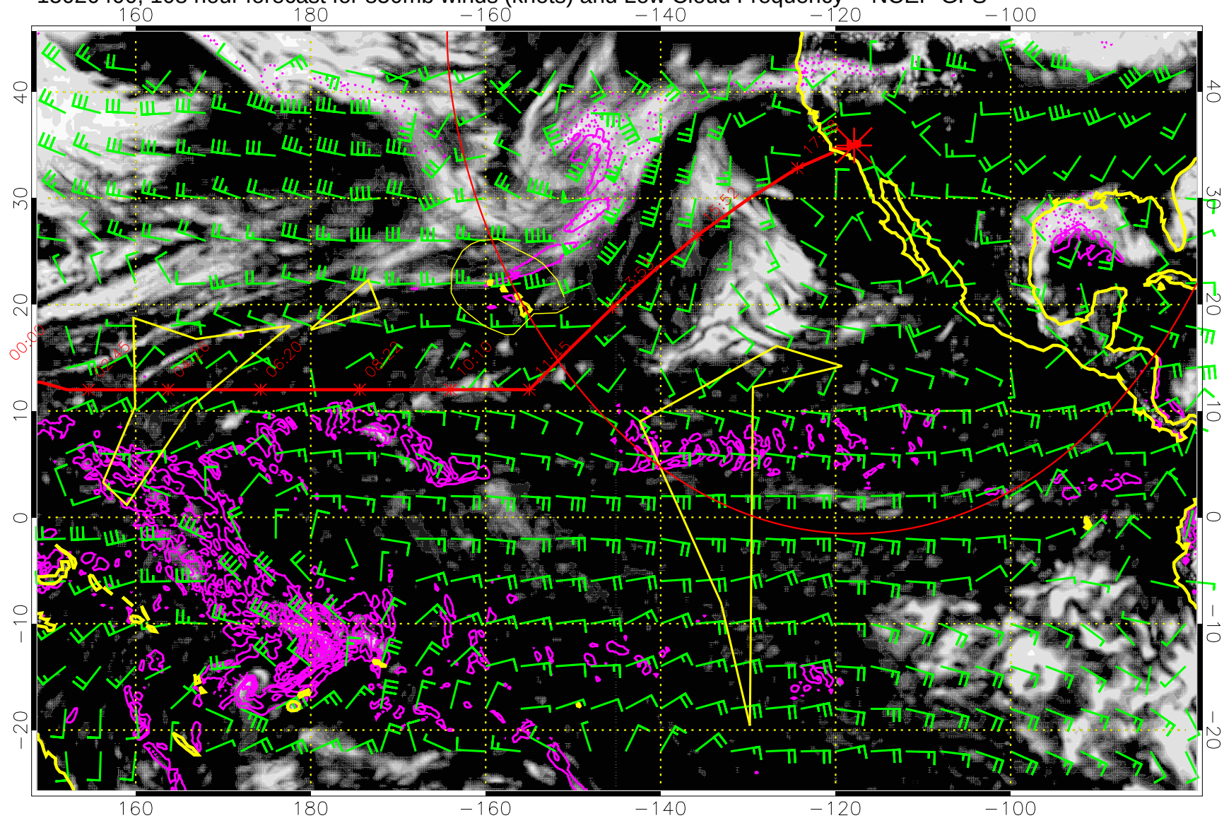
15020400, 108 hour forecast for 850mb winds (knots) and Low Cloud Frequency -- NCEP GFS
