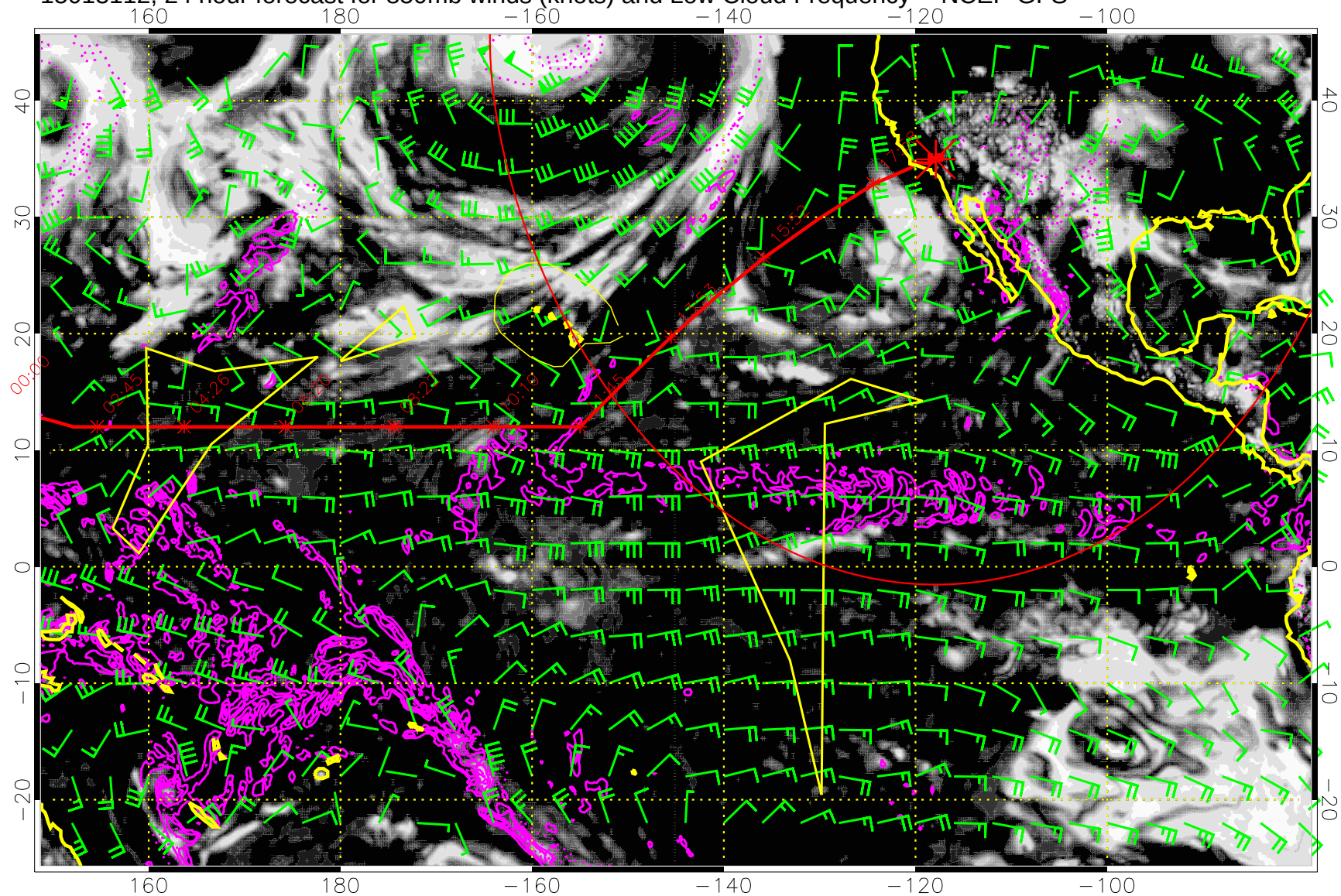
15013112, 24 hour forecast for 850mb winds (knots) and Low Cloud Frequency -- NCEP GFS
