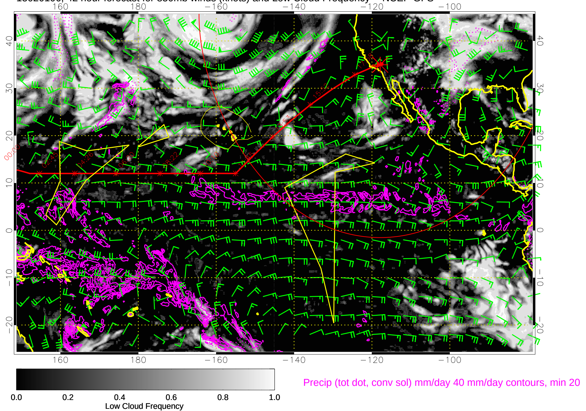
15020106, 42 hour forecast for 850mb winds (knots) and Low Cloud Frequency -- NCEP GFS
