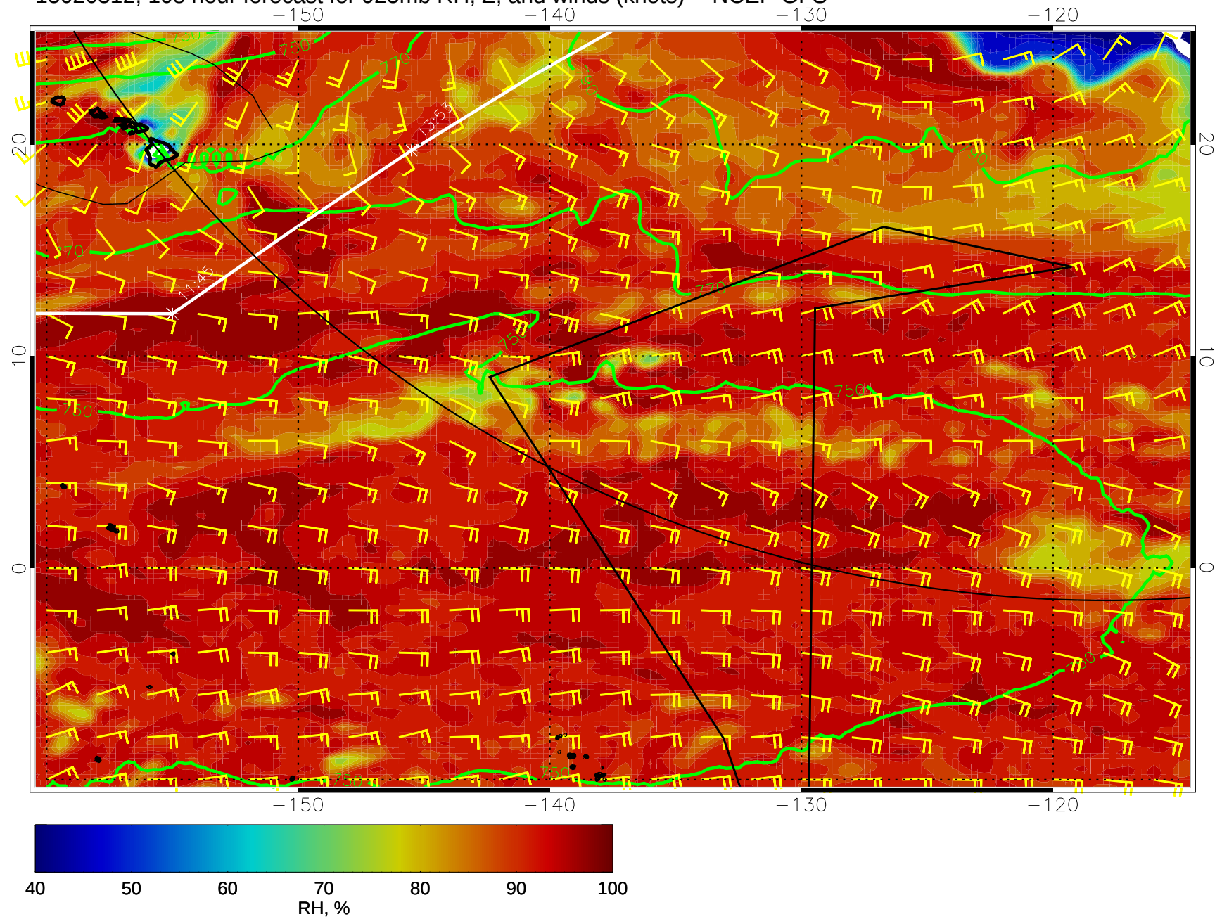
15020312, 108 hour forecast for 925mb RH, Z, and winds (knots) -- NCEP GFS
