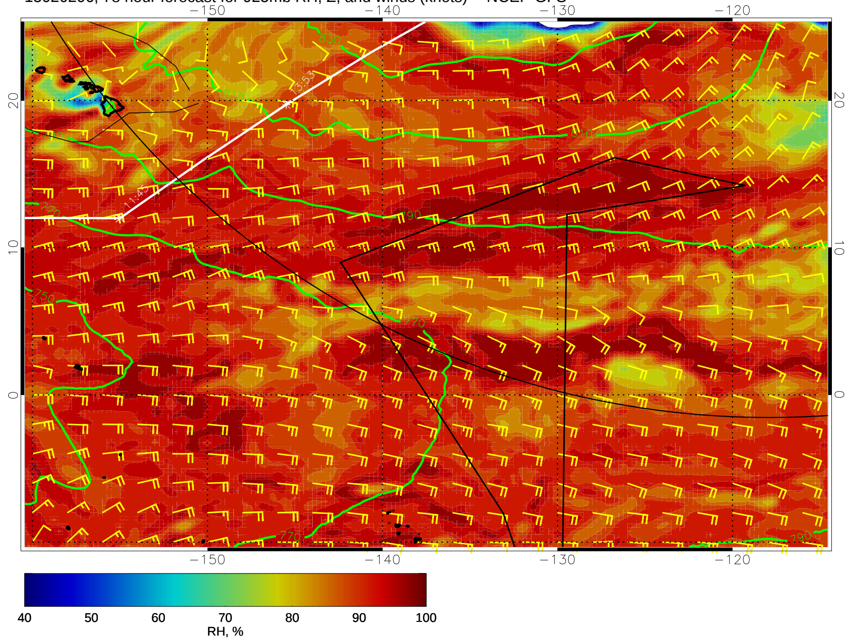
15020206, 78 hour forecast for 925mb RH, Z, and winds (knots) -- NCEP GFS
