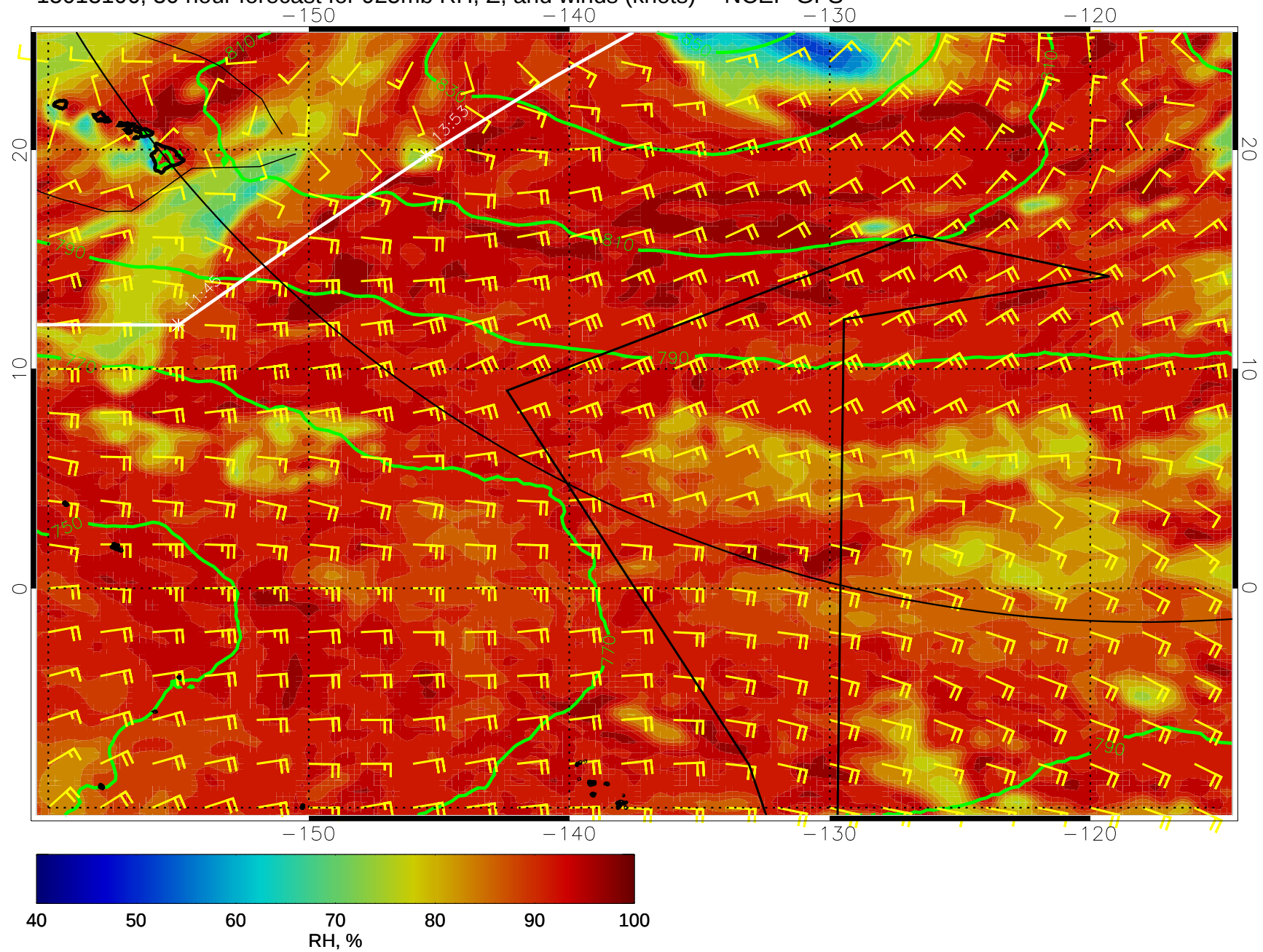
15013106, 30 hour forecast for 925mb RH, Z, and winds (knots) -- NCEP GFS
