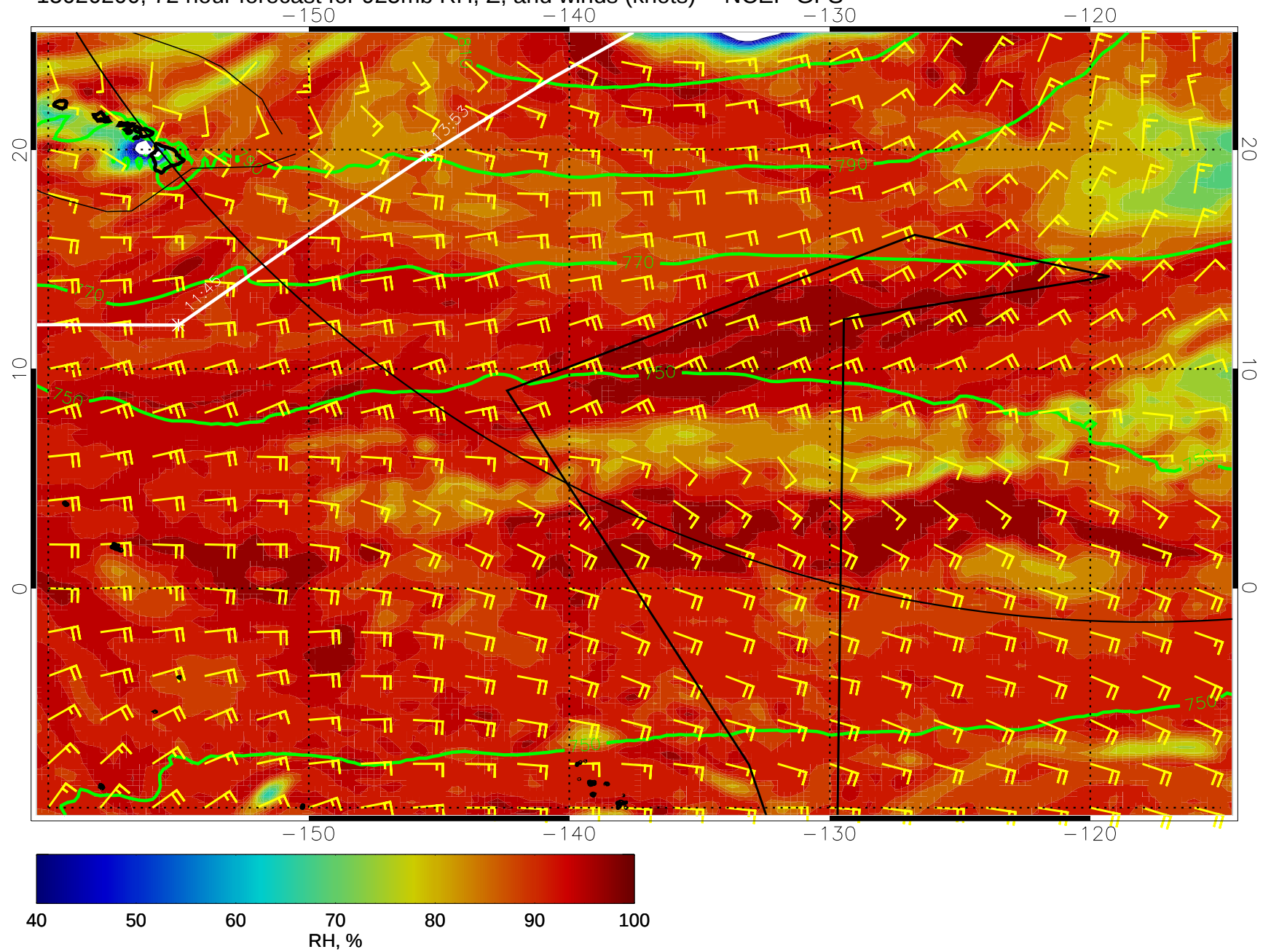
15020200, 72 hour forecast for 925mb RH, Z, and winds (knots) -- NCEP GFS
