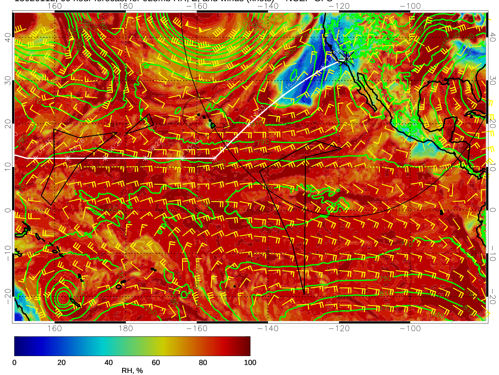
15020112, 60 hour forecast for 925mb RH, Z, and winds (knots) -- NCEP GFS
