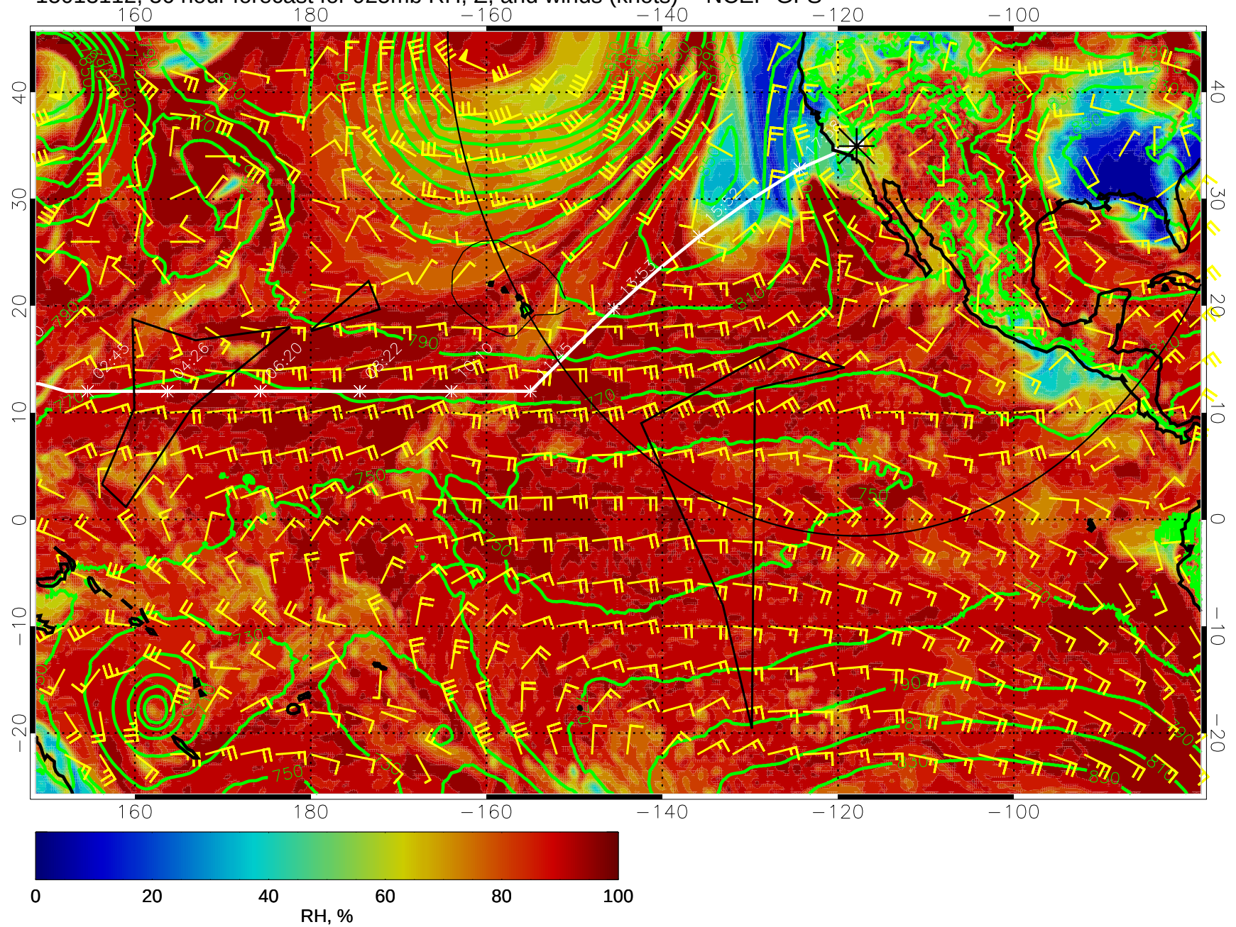
15013112, 36 hour forecast for 925mb RH, Z, and winds (knots) -- NCEP GFS
