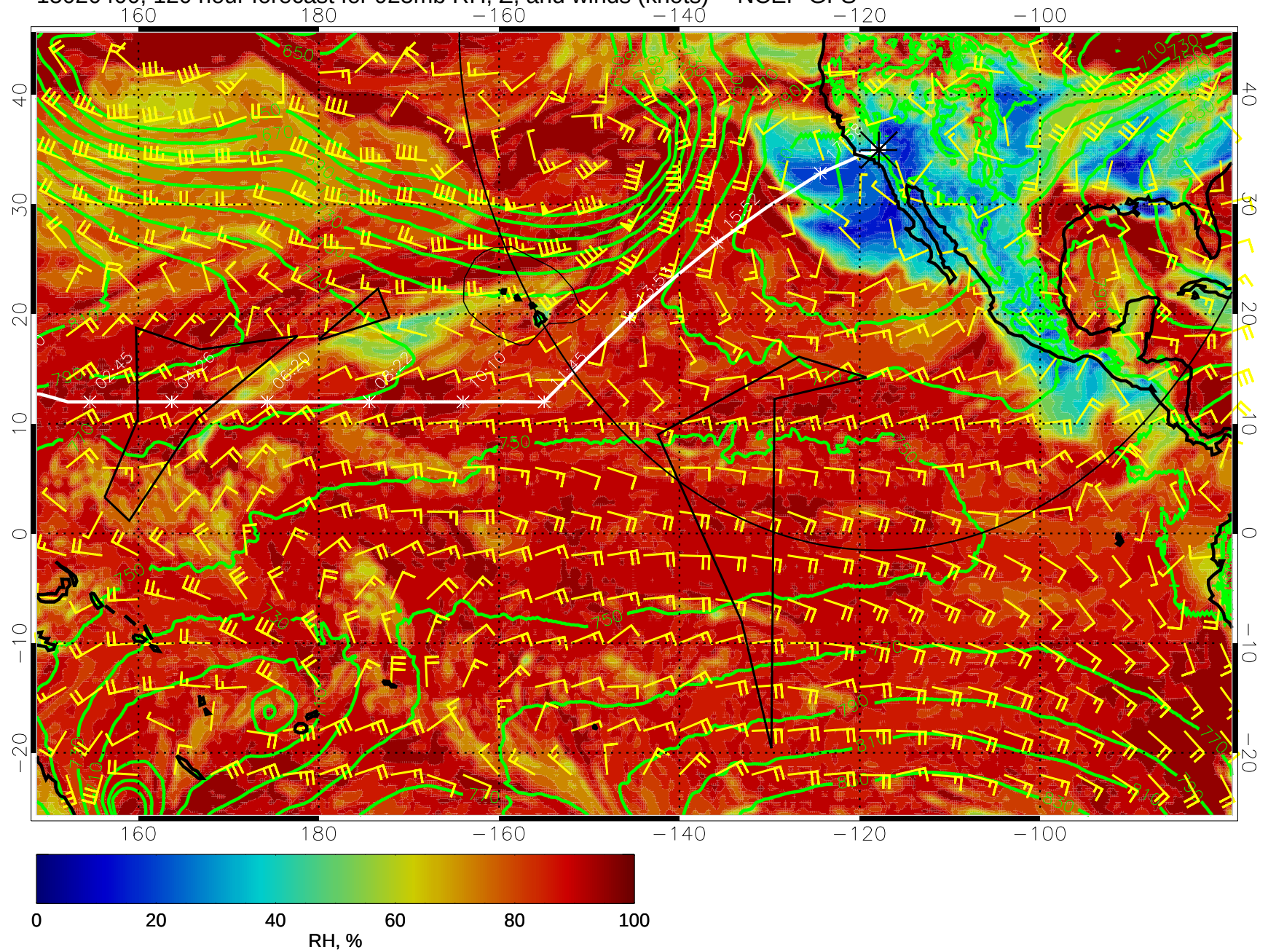
15020400, 120 hour forecast for 925mb RH, Z, and winds (knots) -- NCEP GFS
