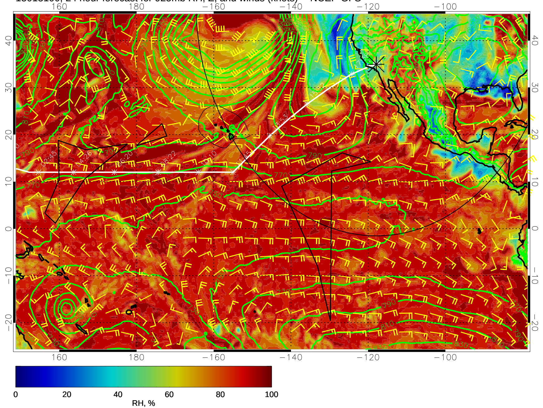
15013100, 24 hour forecast for 925mb RH, Z, and winds (knots) -- NCEP GFS
