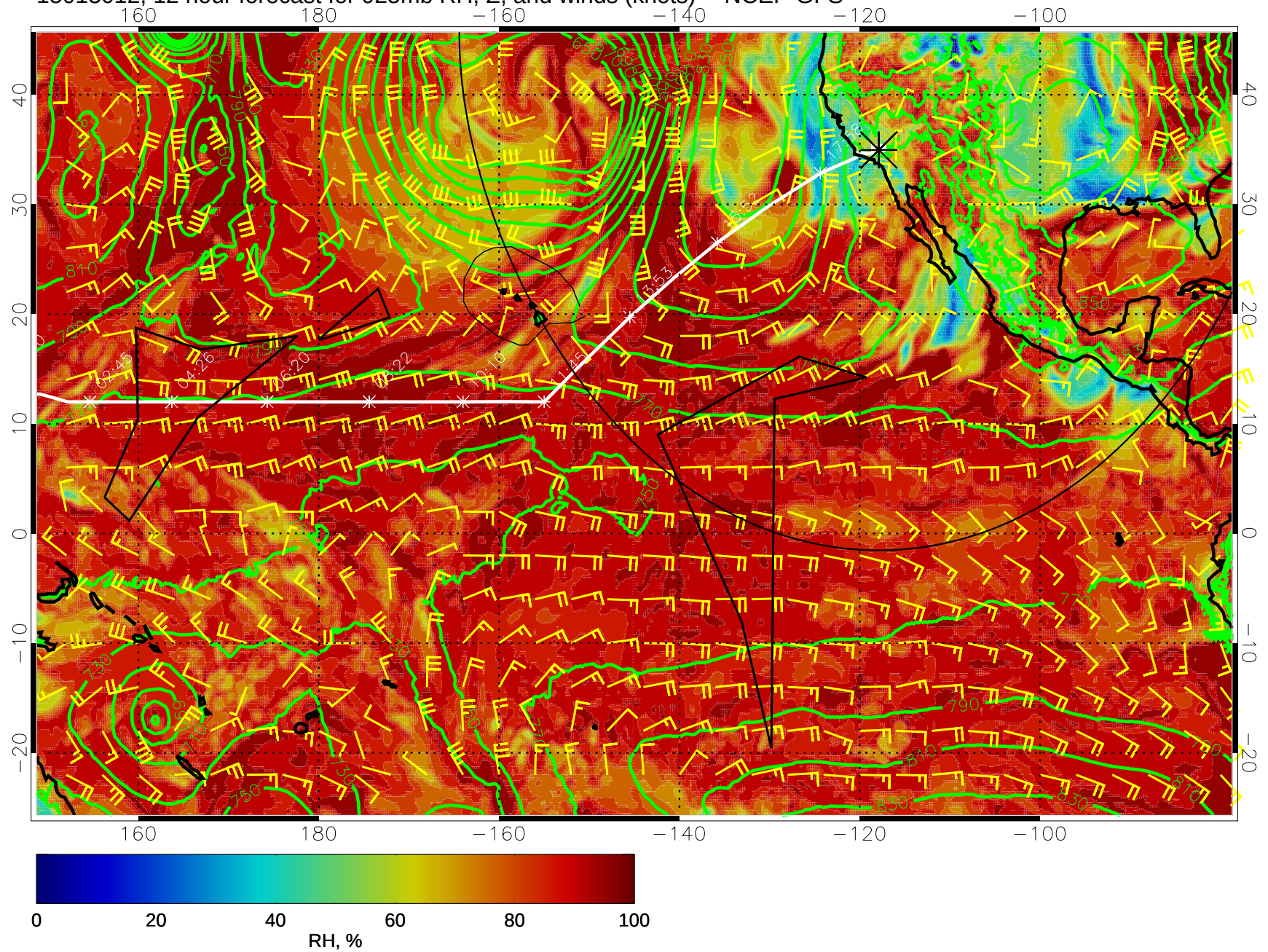
15013012, 12 hour forecast for 925mb RH, Z, and winds (knots) -- NCEP GFS
