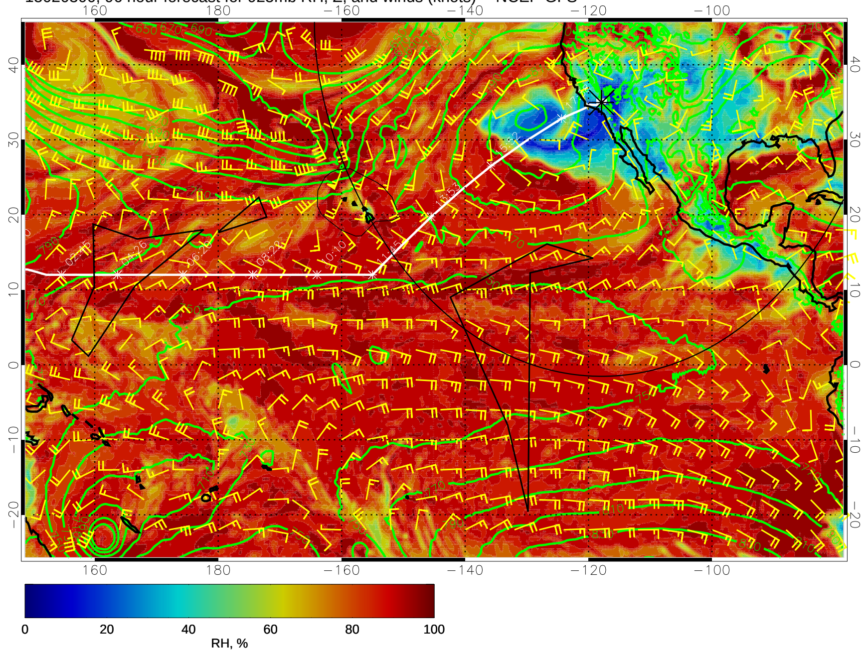
15020300, 96 hour forecast for 925mb RH, Z, and winds (knots) -- NCEP GFS
