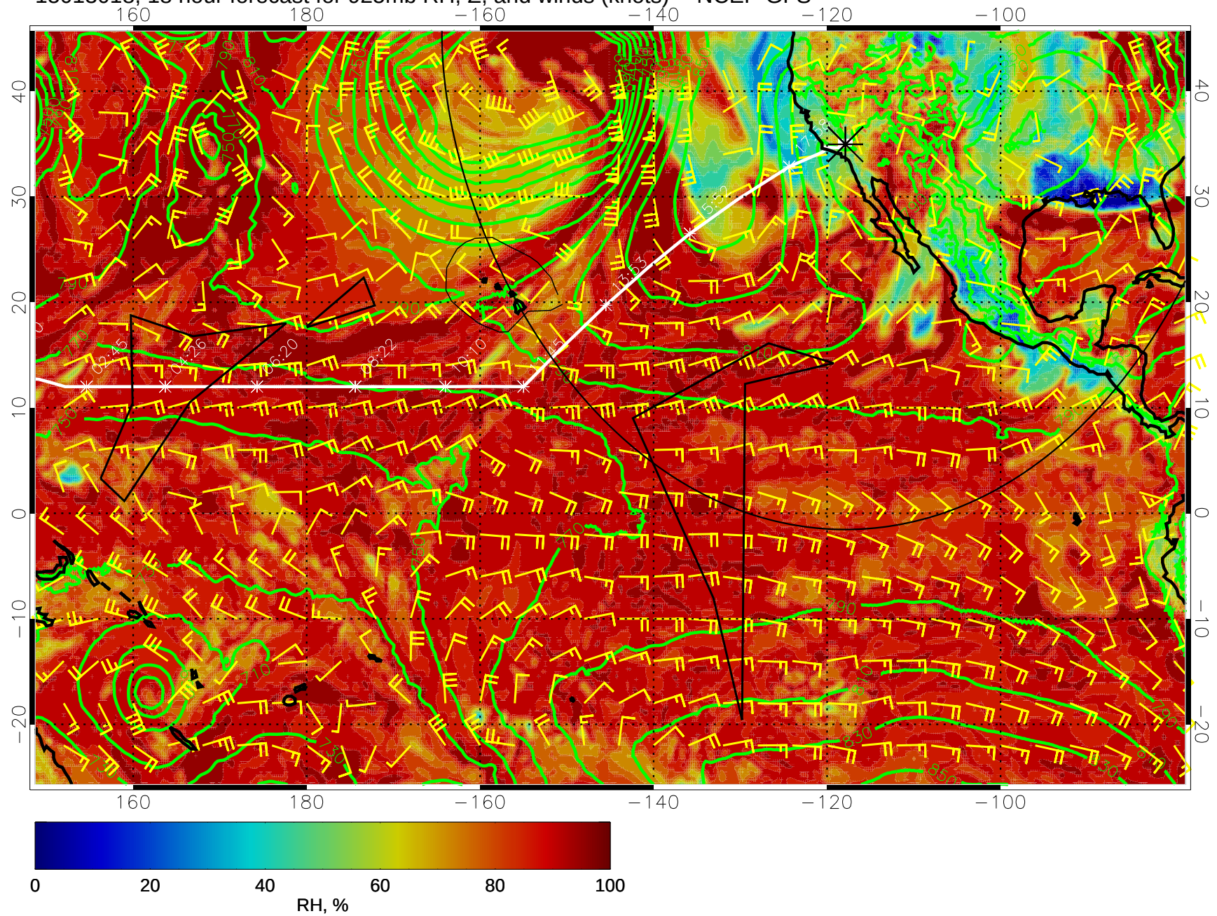
15013018, 18 hour forecast for 925mb RH, Z, and winds (knots) -- NCEP GFS
