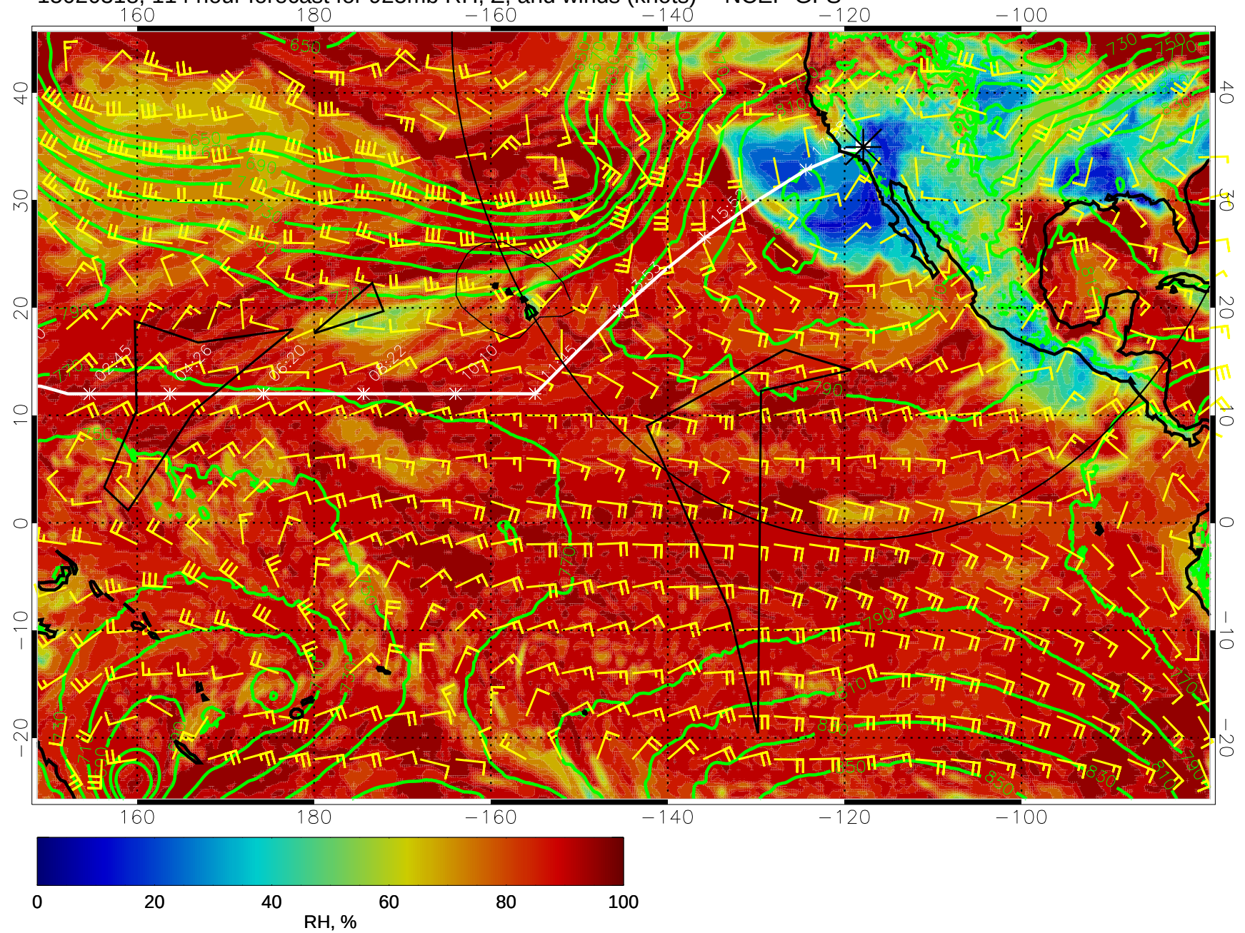
15020318, 114 hour forecast for 925mb RH, Z, and winds (knots) -- NCEP GFS
