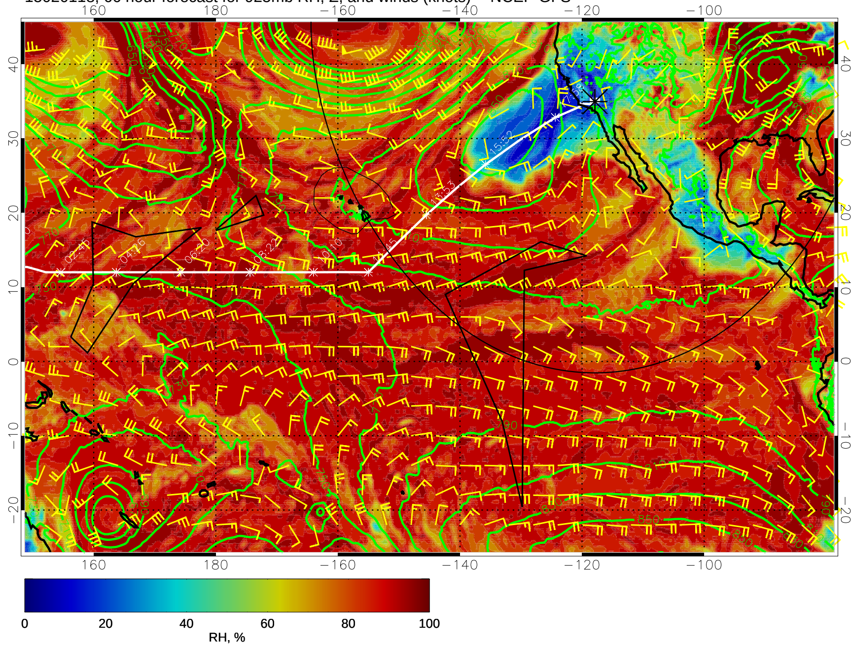
15020118, 66 hour forecast for 925mb RH, Z, and winds (knots) -- NCEP GFS
