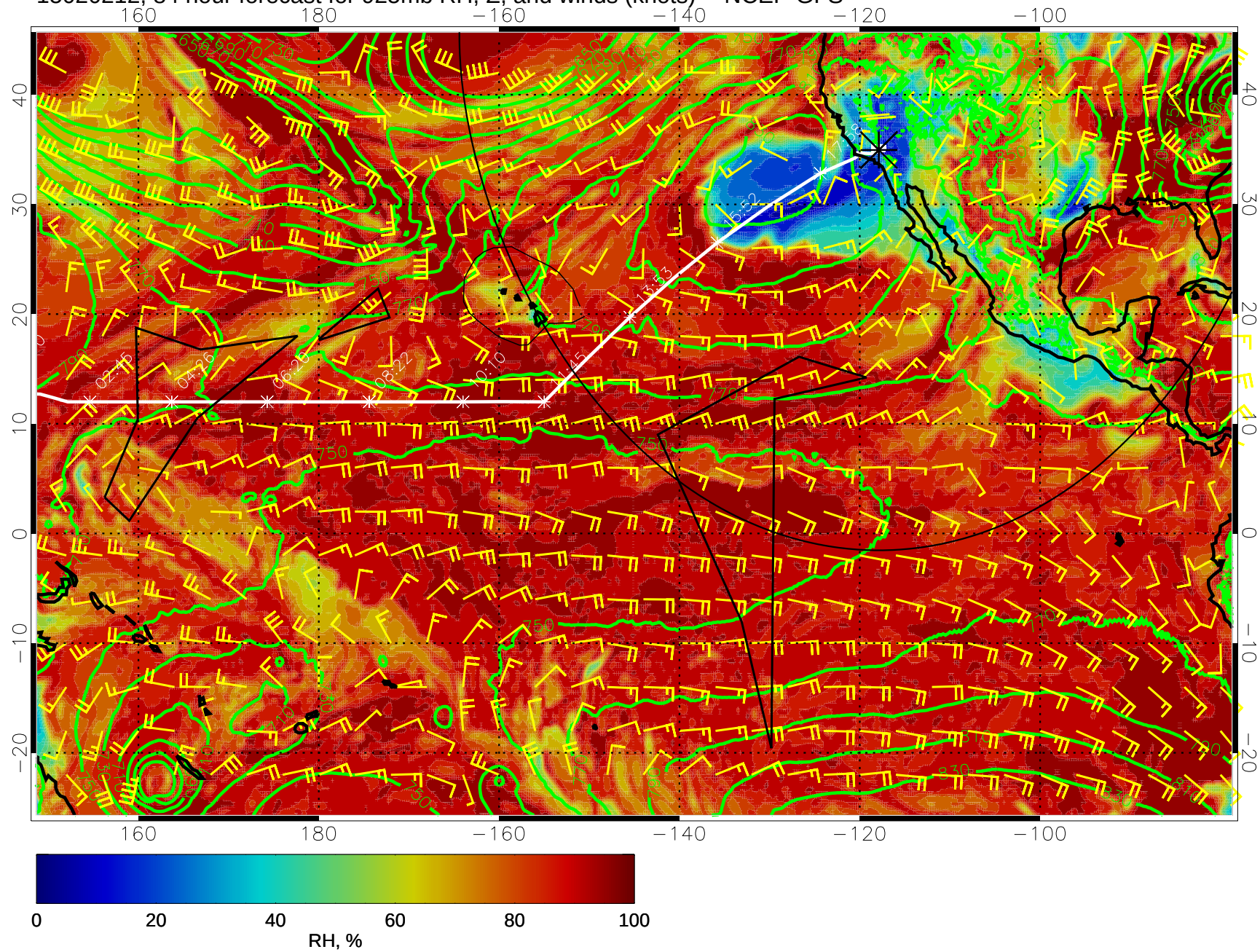
15020212, 84 hour forecast for 925mb RH, Z, and winds (knots) -- NCEP GFS
