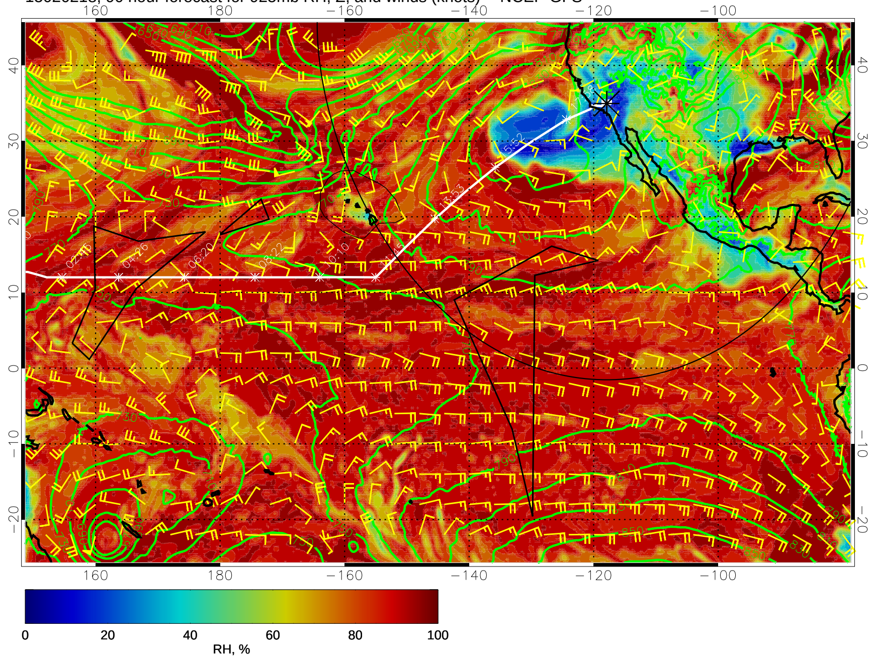
15020218, 90 hour forecast for 925mb RH, Z, and winds (knots) -- NCEP GFS
