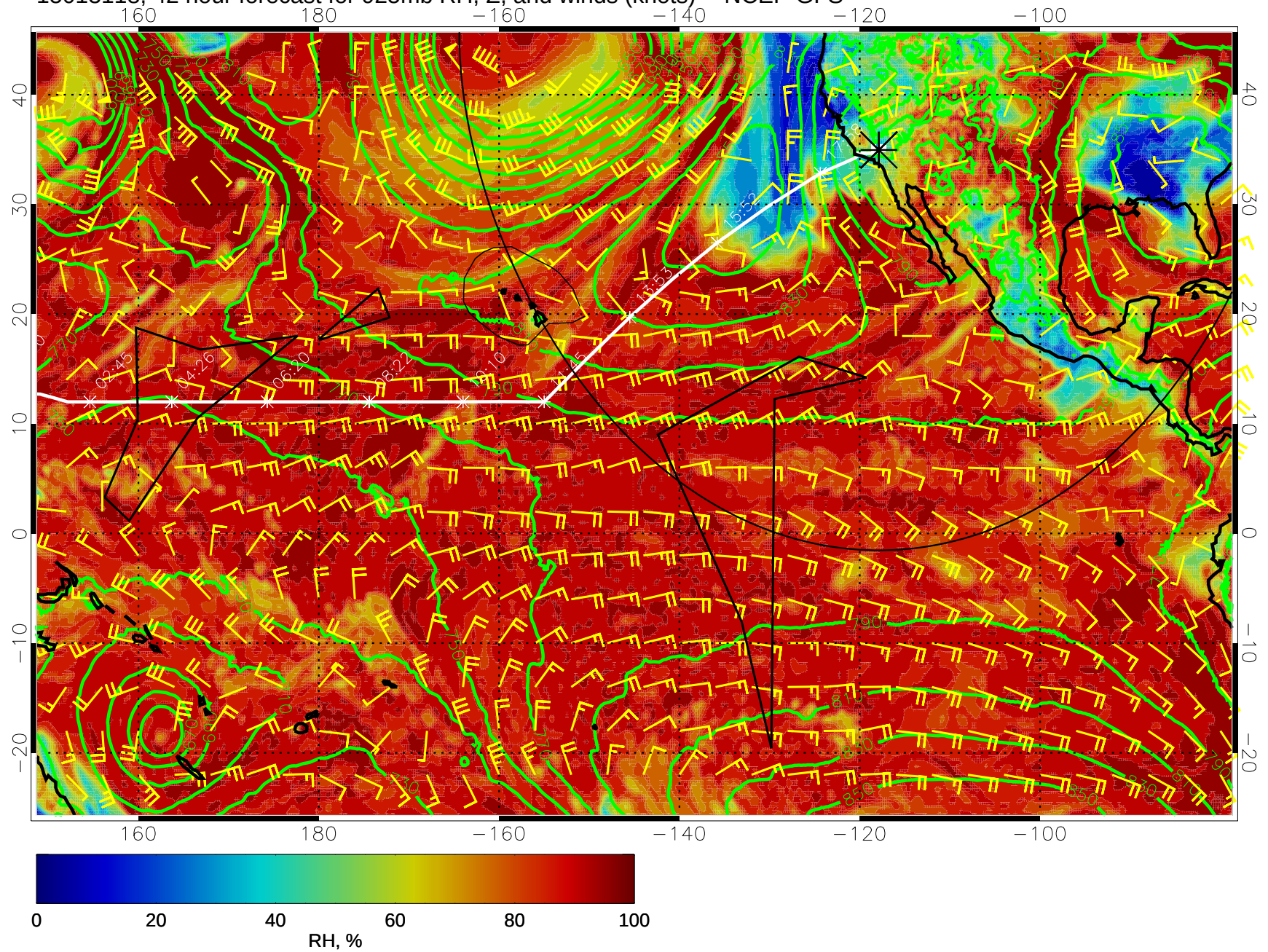
15013118, 42 hour forecast for 925mb RH, Z, and winds (knots) -- NCEP GFS
