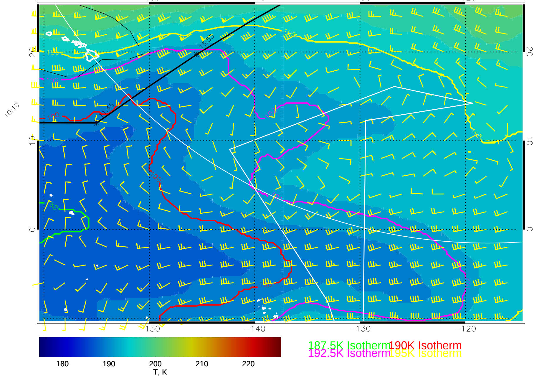
15013100, 24 hour forecast for 100mb T and winds (knots) -- NCEP GFS
