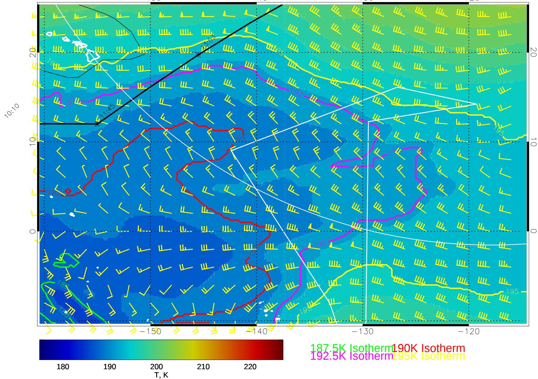
15020112, 60 hour forecast for 100mb T and winds (knots) -- NCEP GFS
