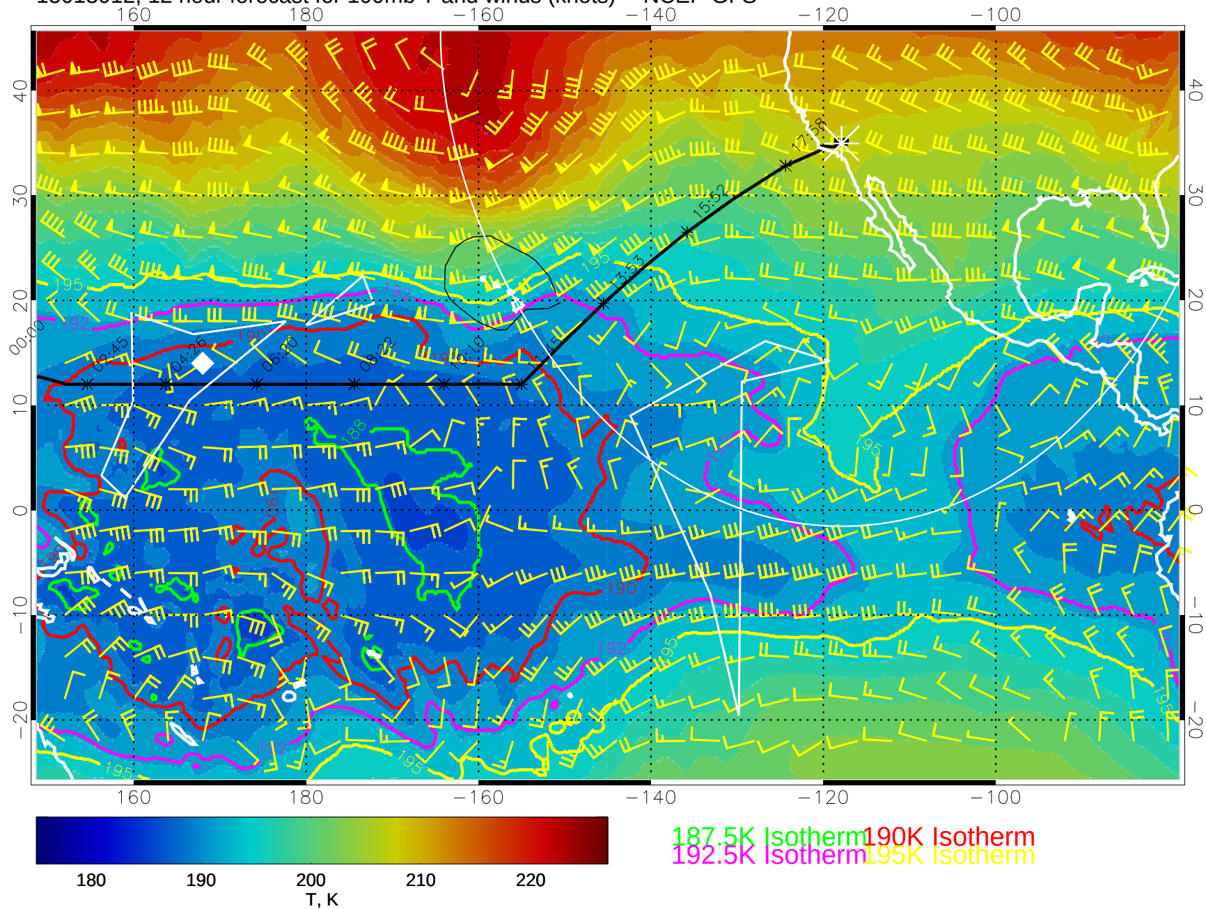
15013012, 12 hour forecast for 100mb T and winds (knots) -- NCEP GFS
