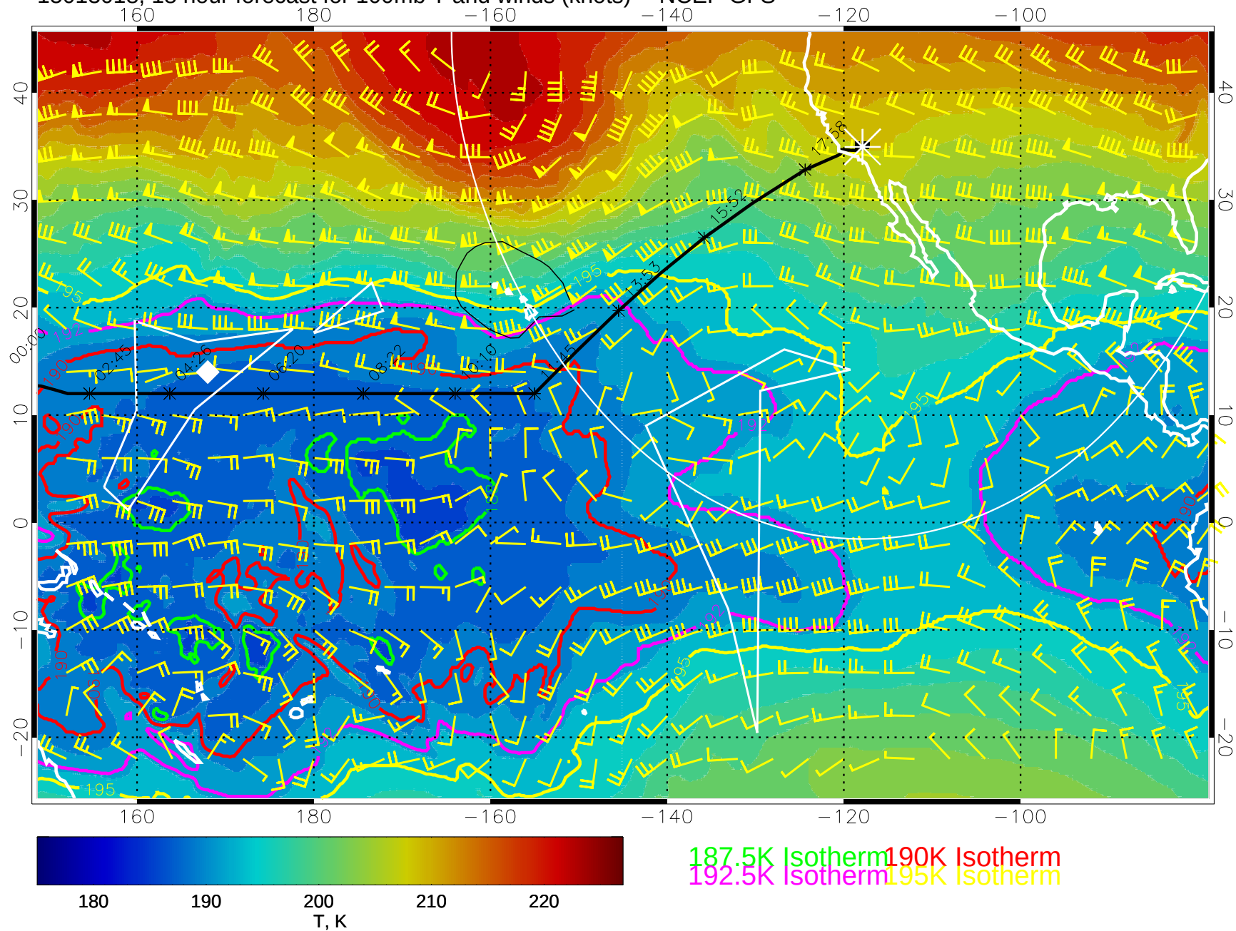
15013018, 18 hour forecast for 100mb T and winds (knots) -- NCEP GFS
