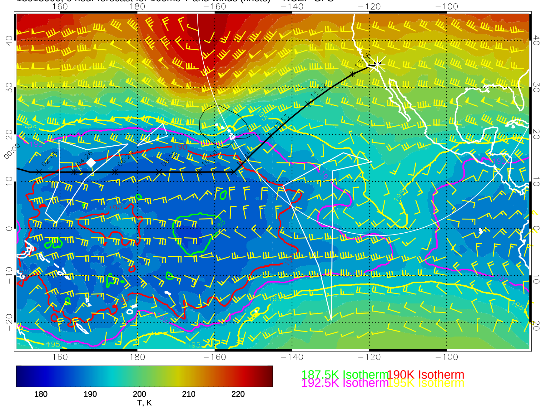
15013006, 6 hour forecast for 100mb T and winds (knots) -- NCEP GFS
