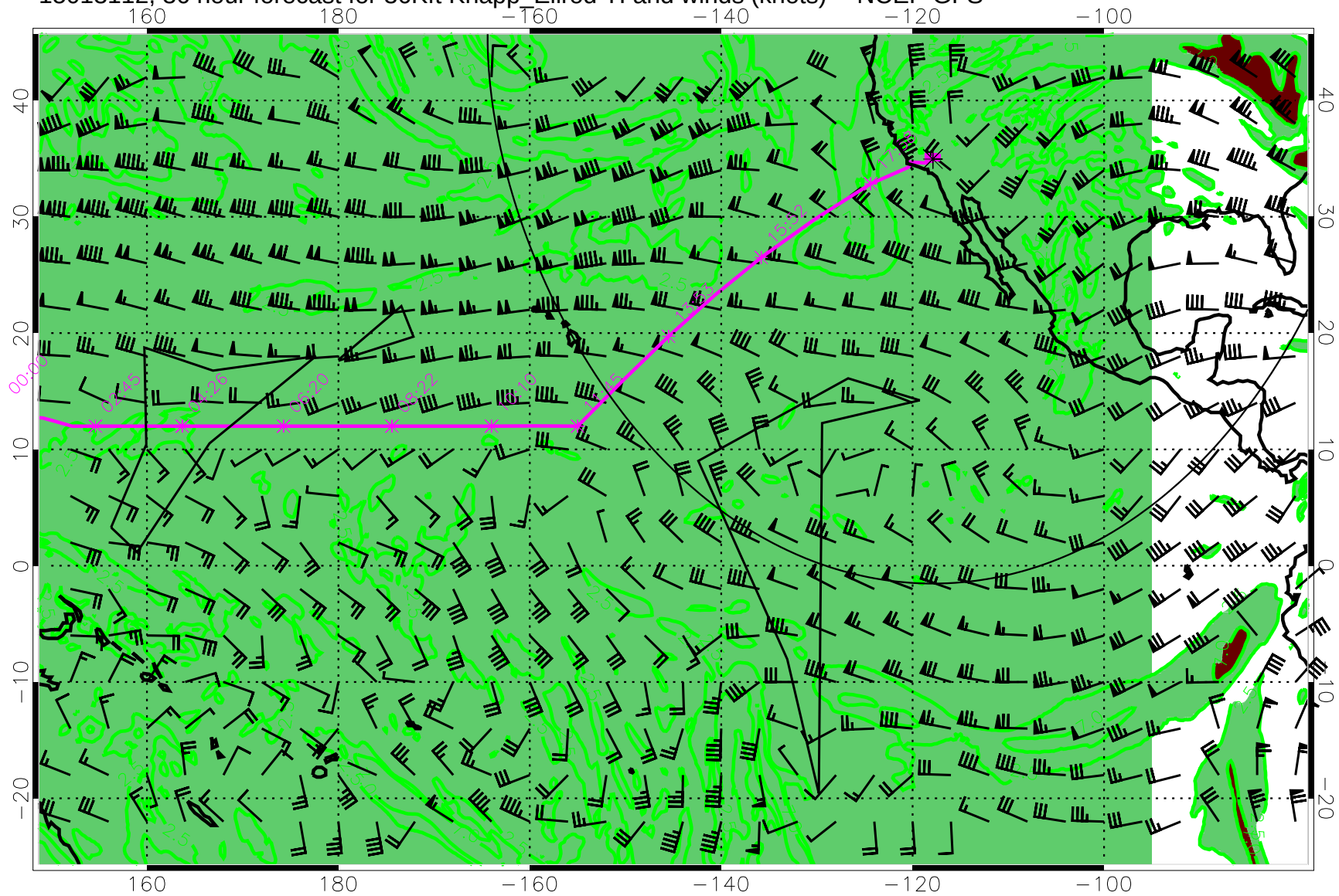
15013112, 36 hour forecast for 36Kft Knapp_Ellrod TI and winds (knots) -- NCEP GFS
