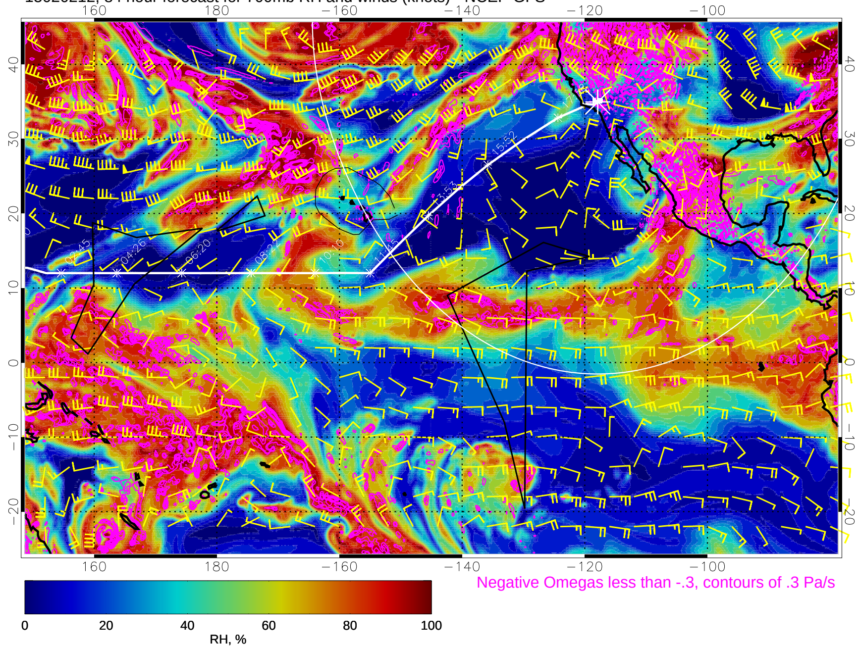
15020212, 84 hour forecast for 700mb RH and winds (knots) - NCEP GFS
