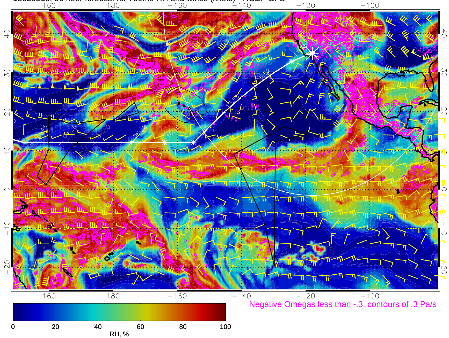
15020218, 90 hour forecast for 700mb RH and winds (knots) - NCEP GFS
