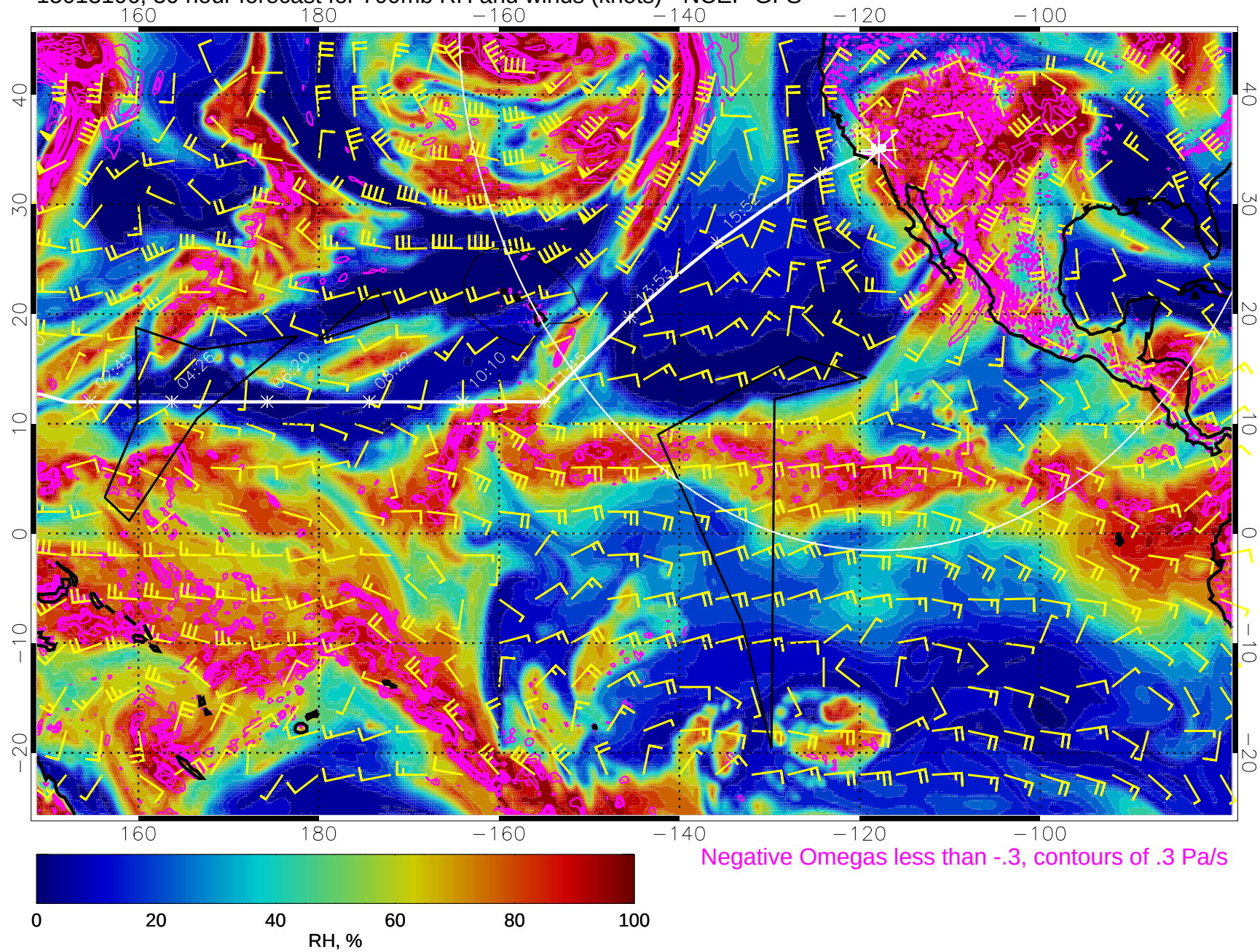
15013106, 30 hour forecast for 700mb RH and winds (knots) - NCEP GFS
