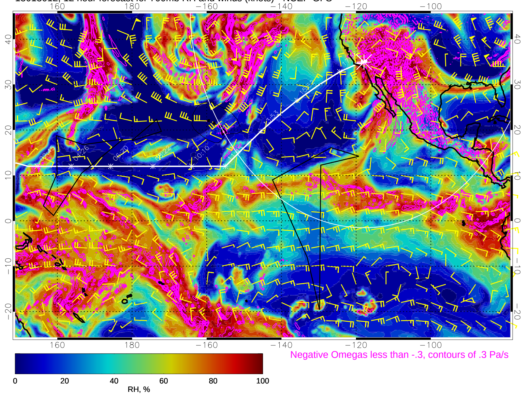
15013012, 12 hour forecast for 700mb RH and winds (knots) - NCEP GFS
