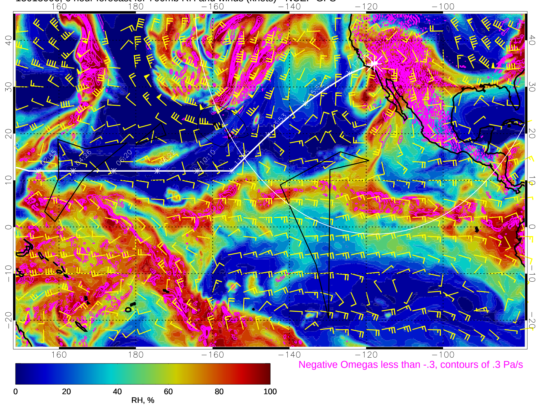
15013006, 6 hour forecast for 700mb RH and winds (knots) - NCEP GFS
