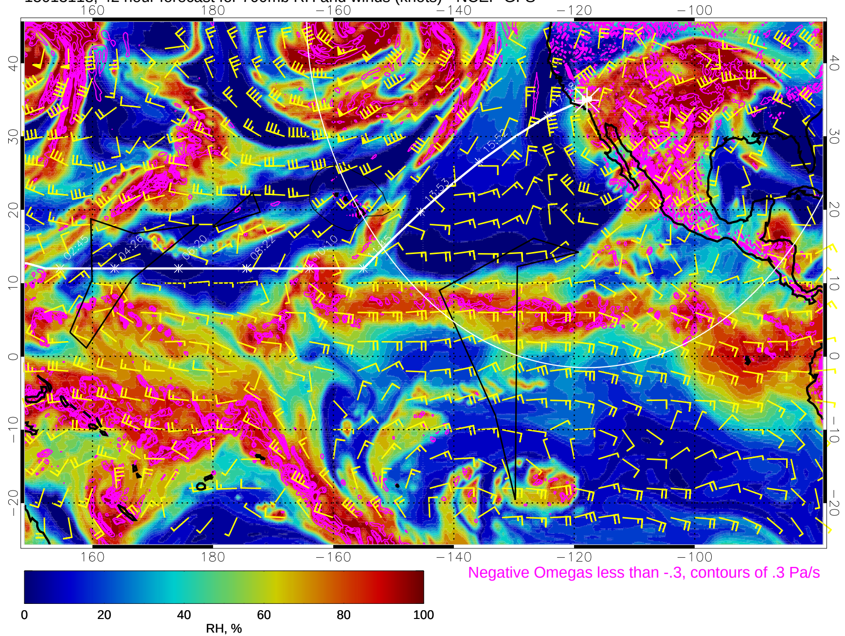
15013118, 42 hour forecast for 700mb RH and winds (knots) - NCEP GFS
