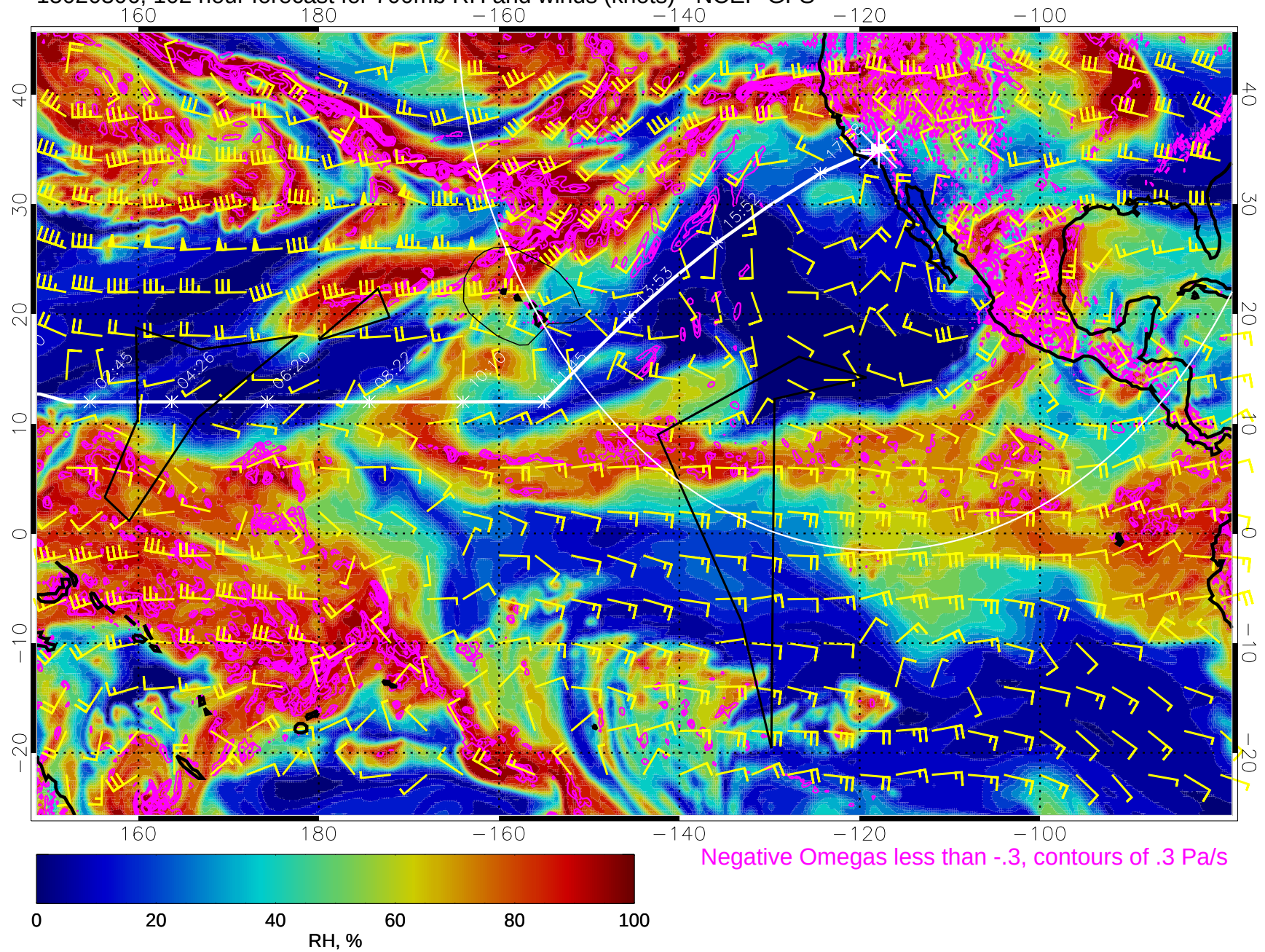
15020306, 102 hour forecast for 700mb RH and winds (knots) - NCEP GFS
