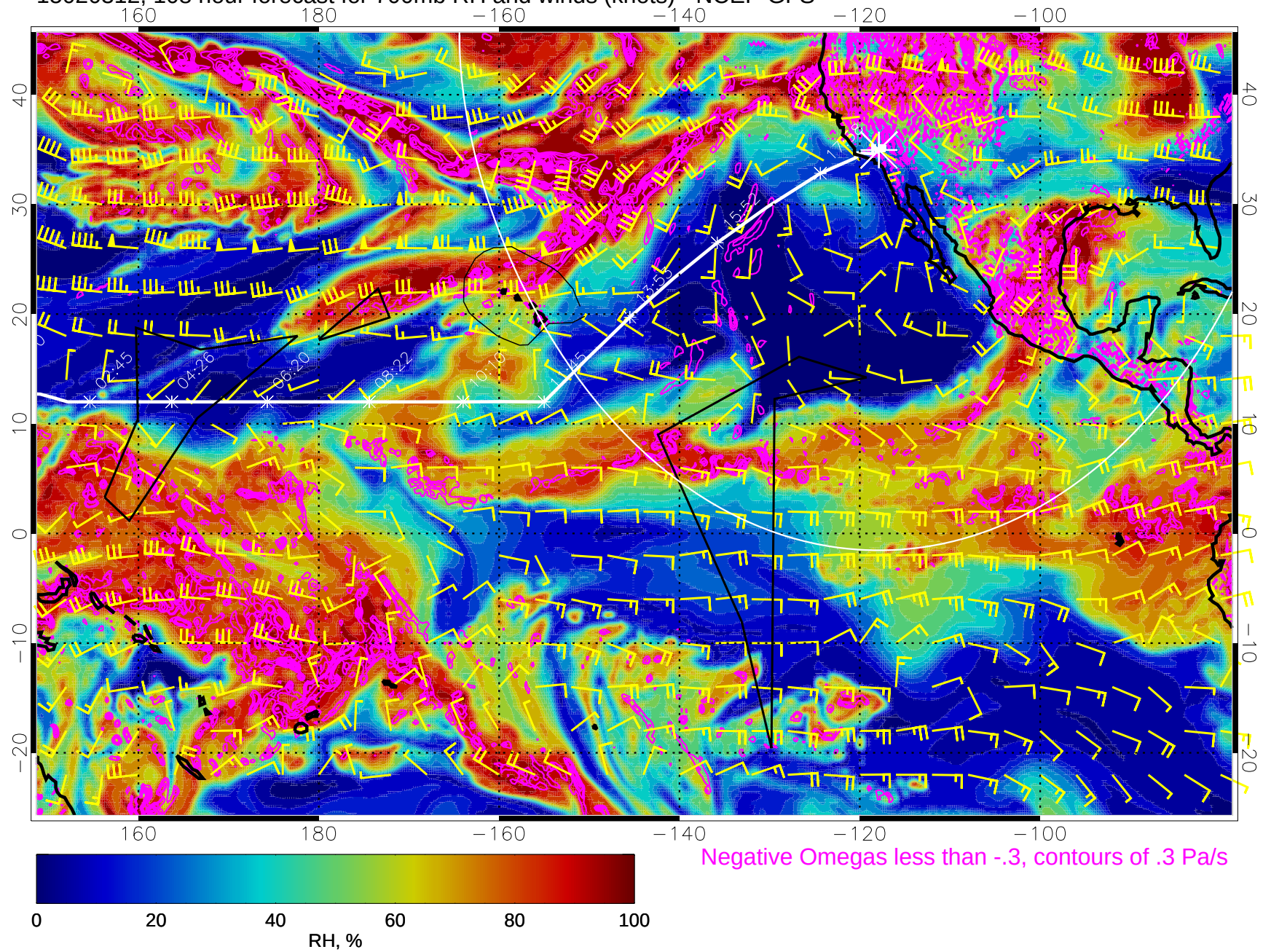
15020312, 108 hour forecast for 700mb RH and winds (knots) - NCEP GFS
