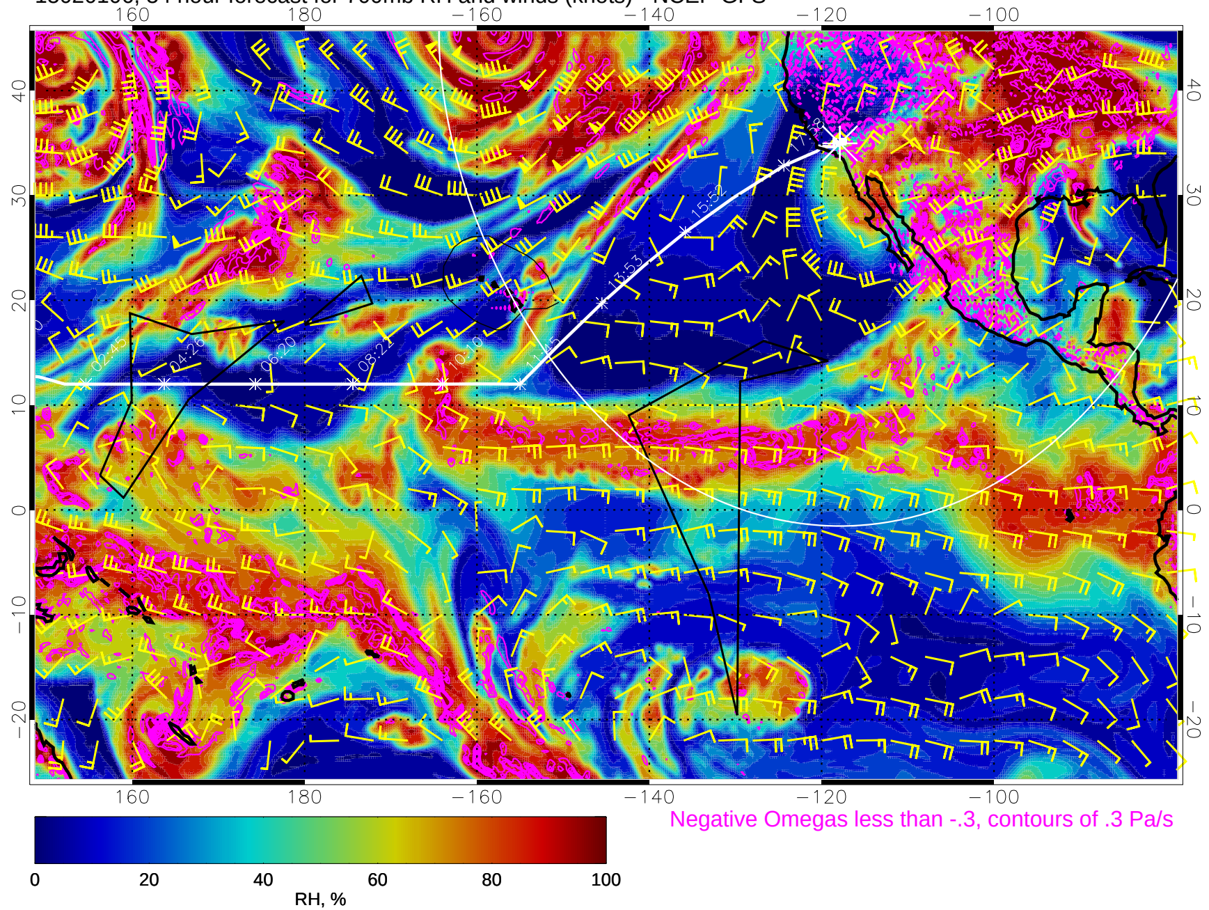
15020106, 54 hour forecast for 700mb RH and winds (knots) - NCEP GFS
