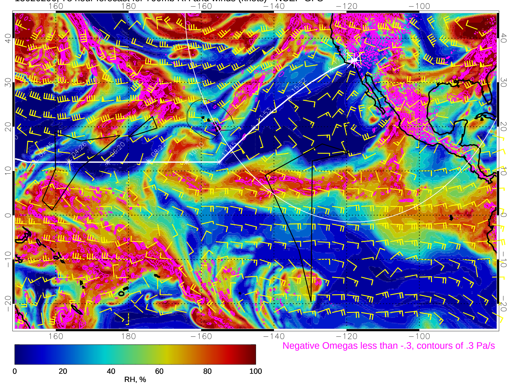
15020206, 78 hour forecast for 700mb RH and winds (knots) - NCEP GFS
