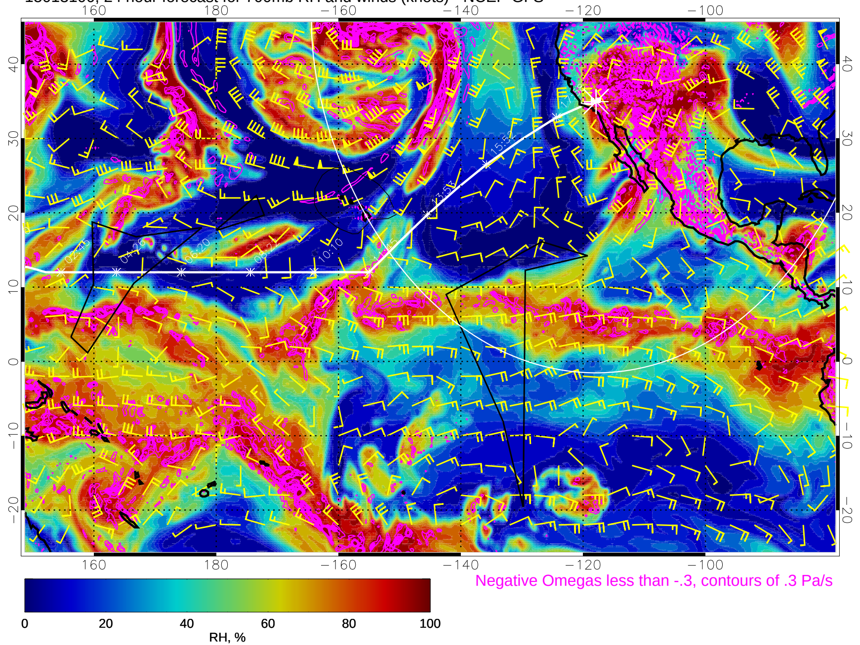
15013100, 24 hour forecast for 700mb RH and winds (knots) - NCEP GFS
