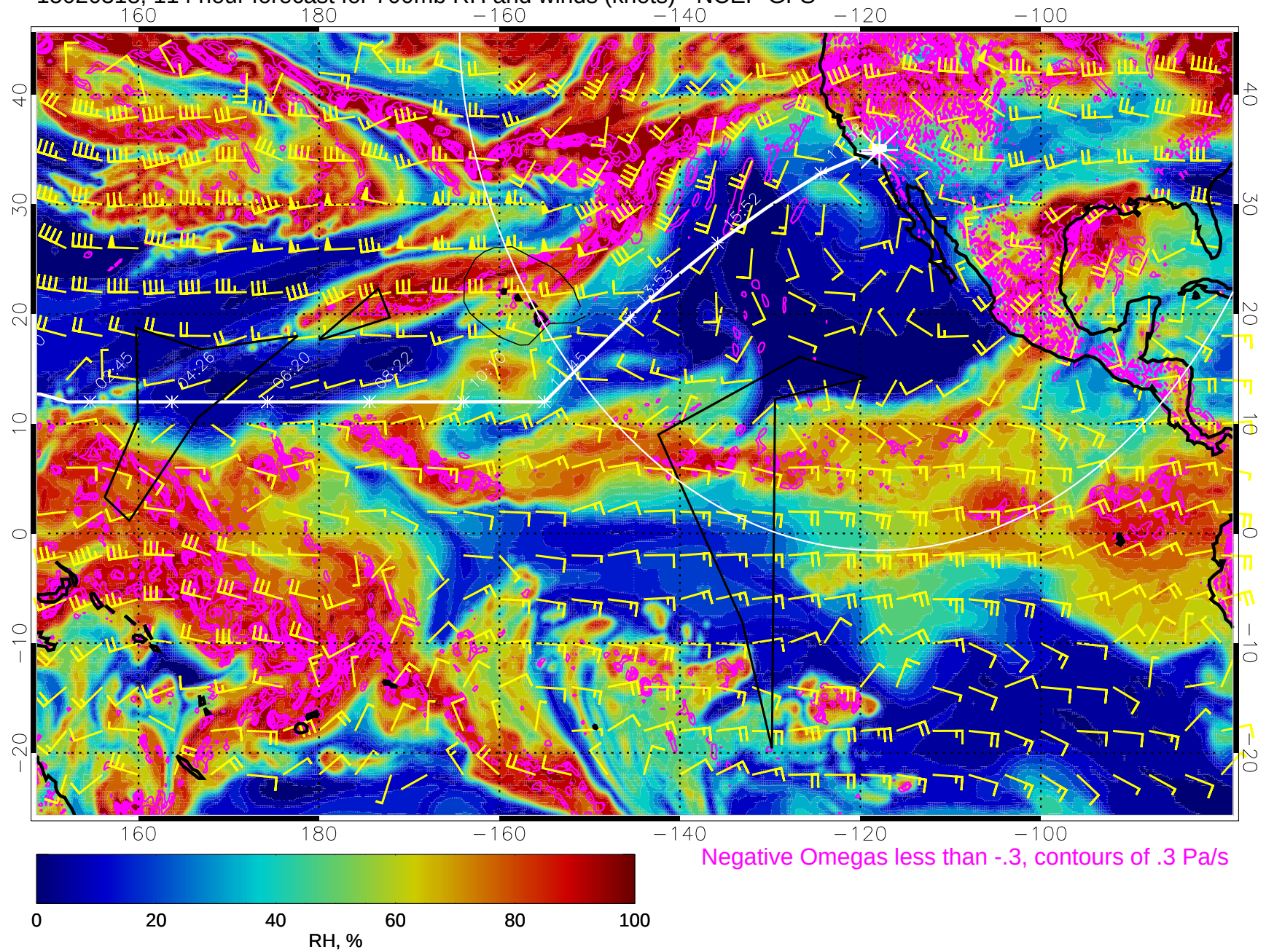
15020318, 114 hour forecast for 700mb RH and winds (knots) - NCEP GFS
