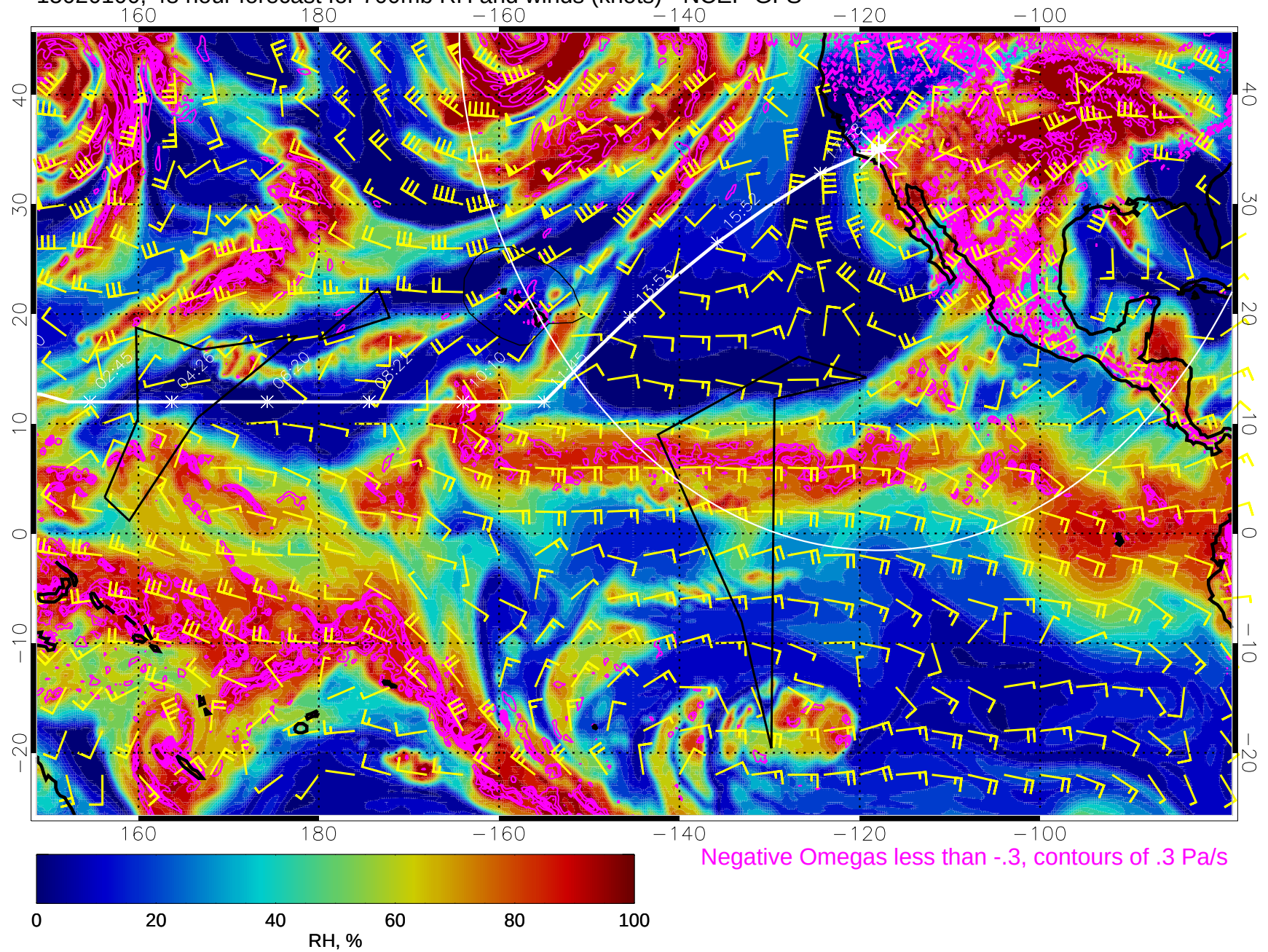
15020100, 48 hour forecast for 700mb RH and winds (knots) - NCEP GFS
