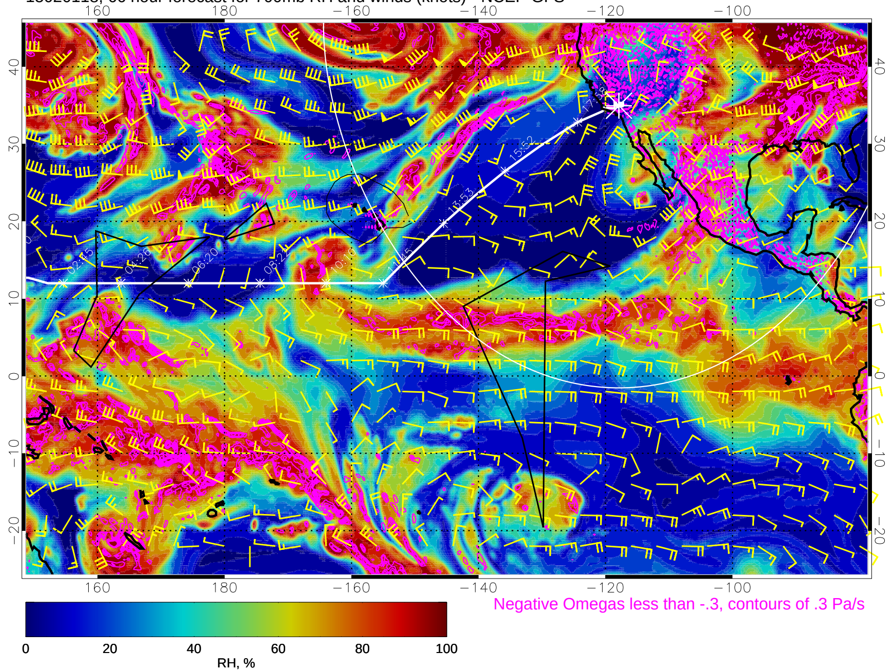
15020118, 66 hour forecast for 700mb RH and winds (knots) - NCEP GFS
