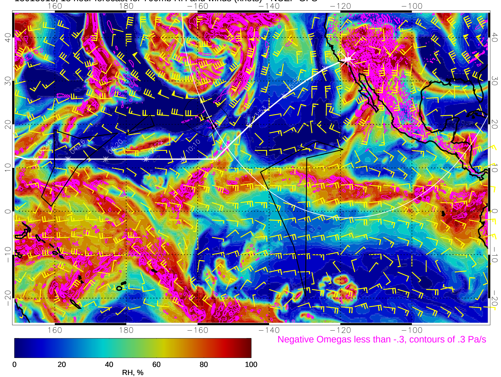
15013018, 18 hour forecast for 700mb RH and winds (knots) - NCEP GFS
