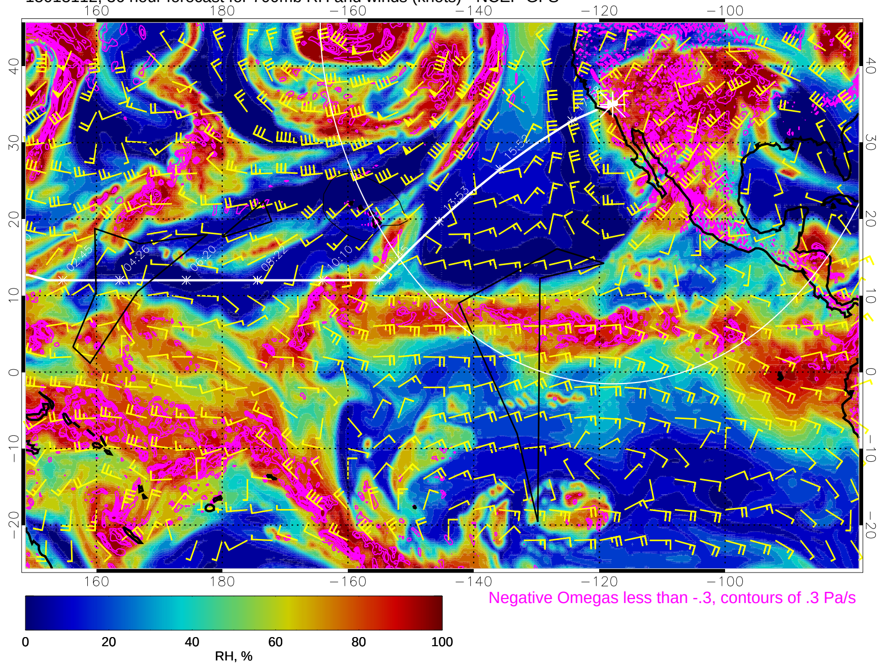
15013112, 36 hour forecast for 700mb RH and winds (knots) - NCEP GFS
