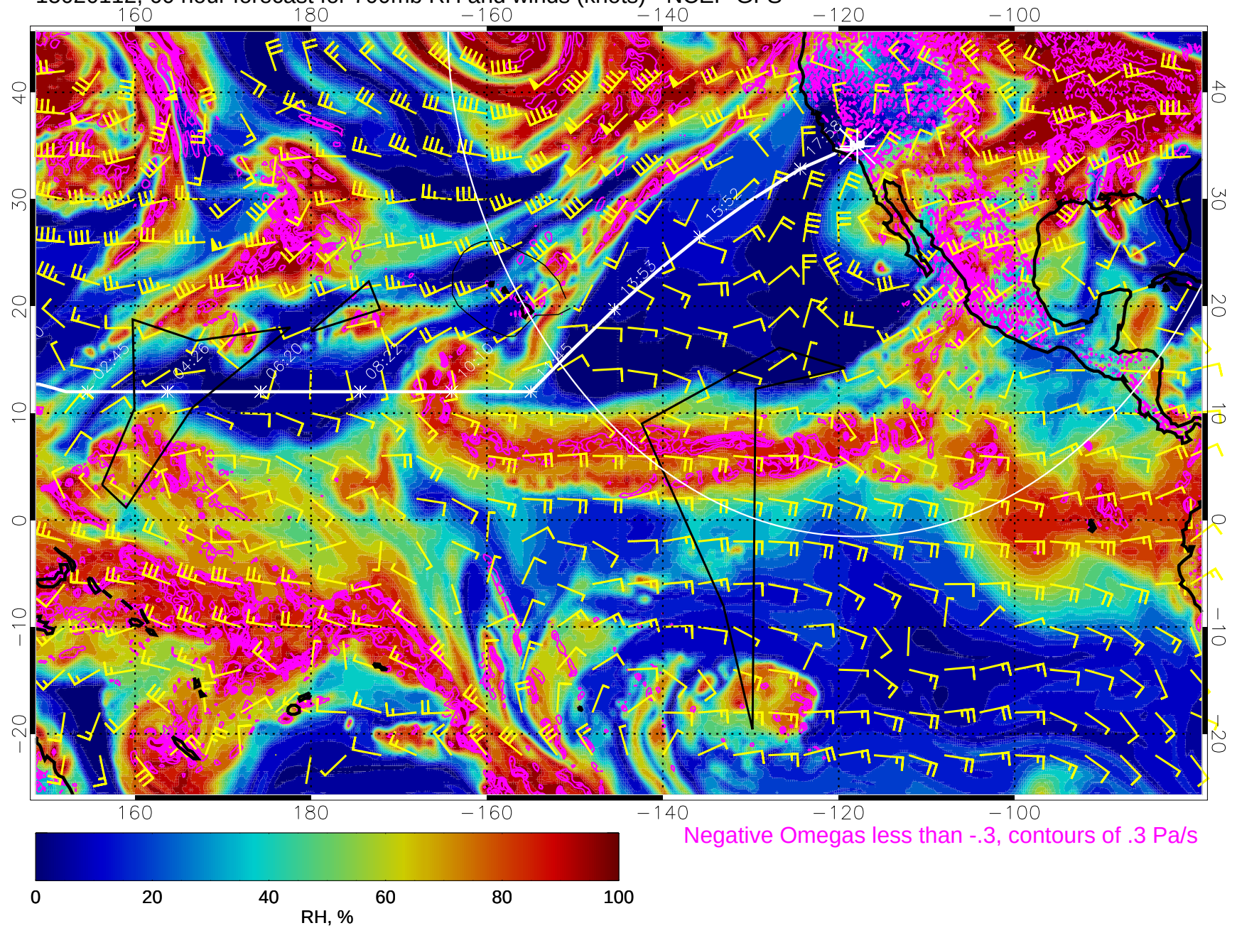
15020112, 60 hour forecast for 700mb RH and winds (knots) - NCEP GFS
