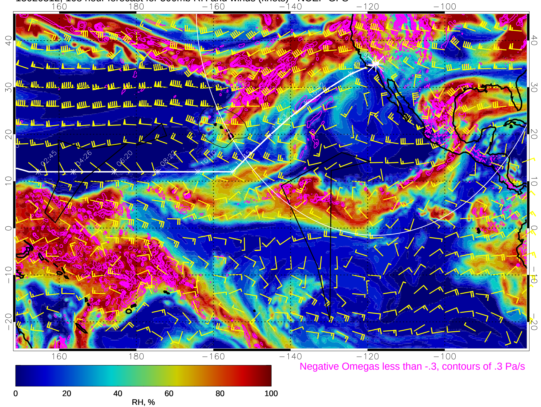
15020312, 108 hour forecast for 500mb RH and winds (knots) - NCEP GFS
