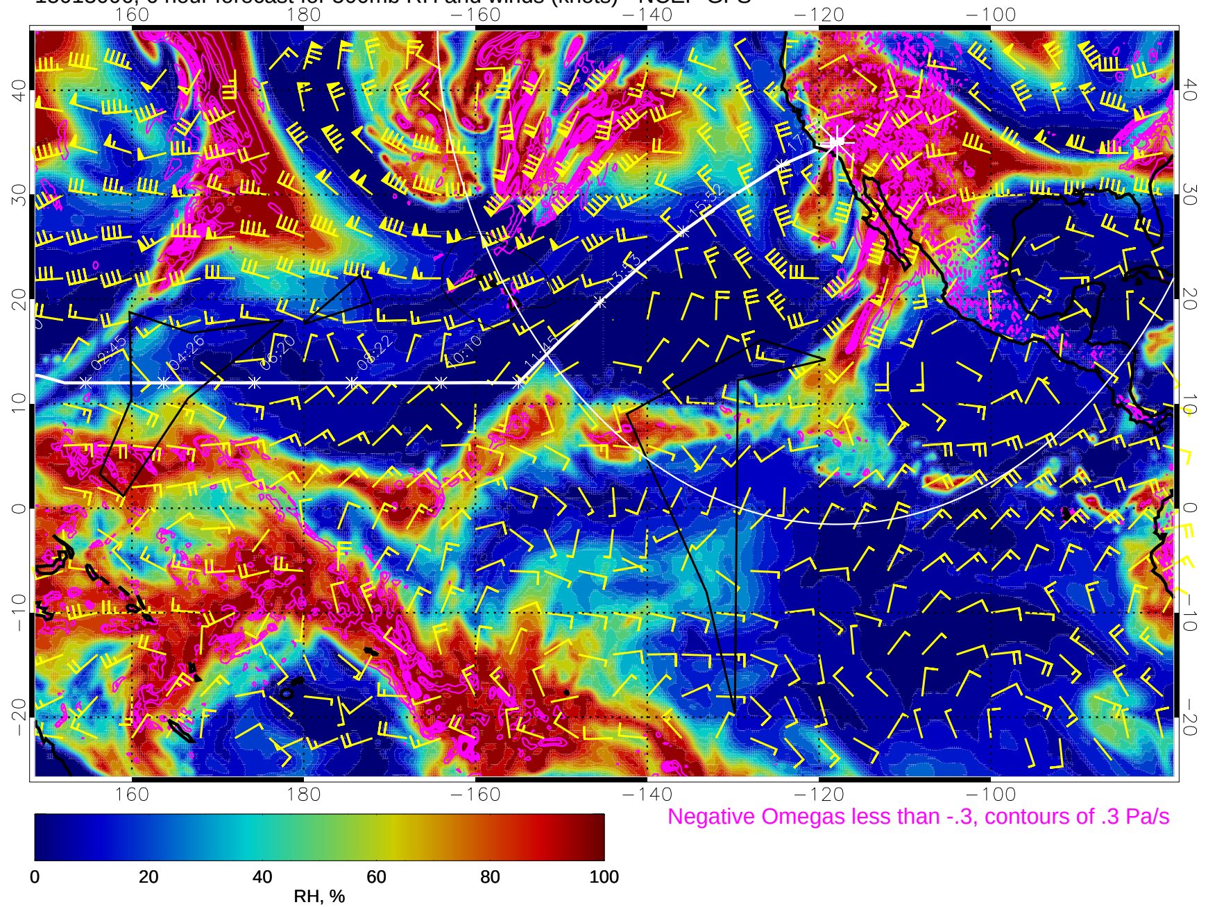
15013006, 6 hour forecast for 500mb RH and winds (knots) - NCEP GFS
