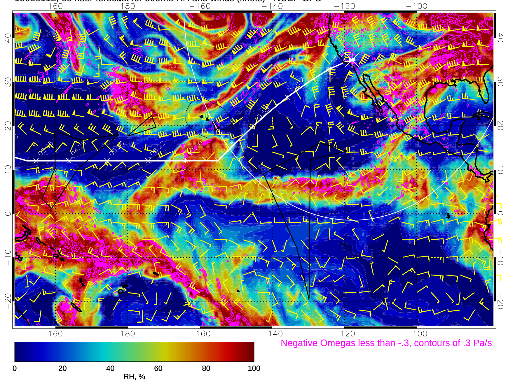
15020112, 60 hour forecast for 500mb RH and winds (knots) - NCEP GFS
