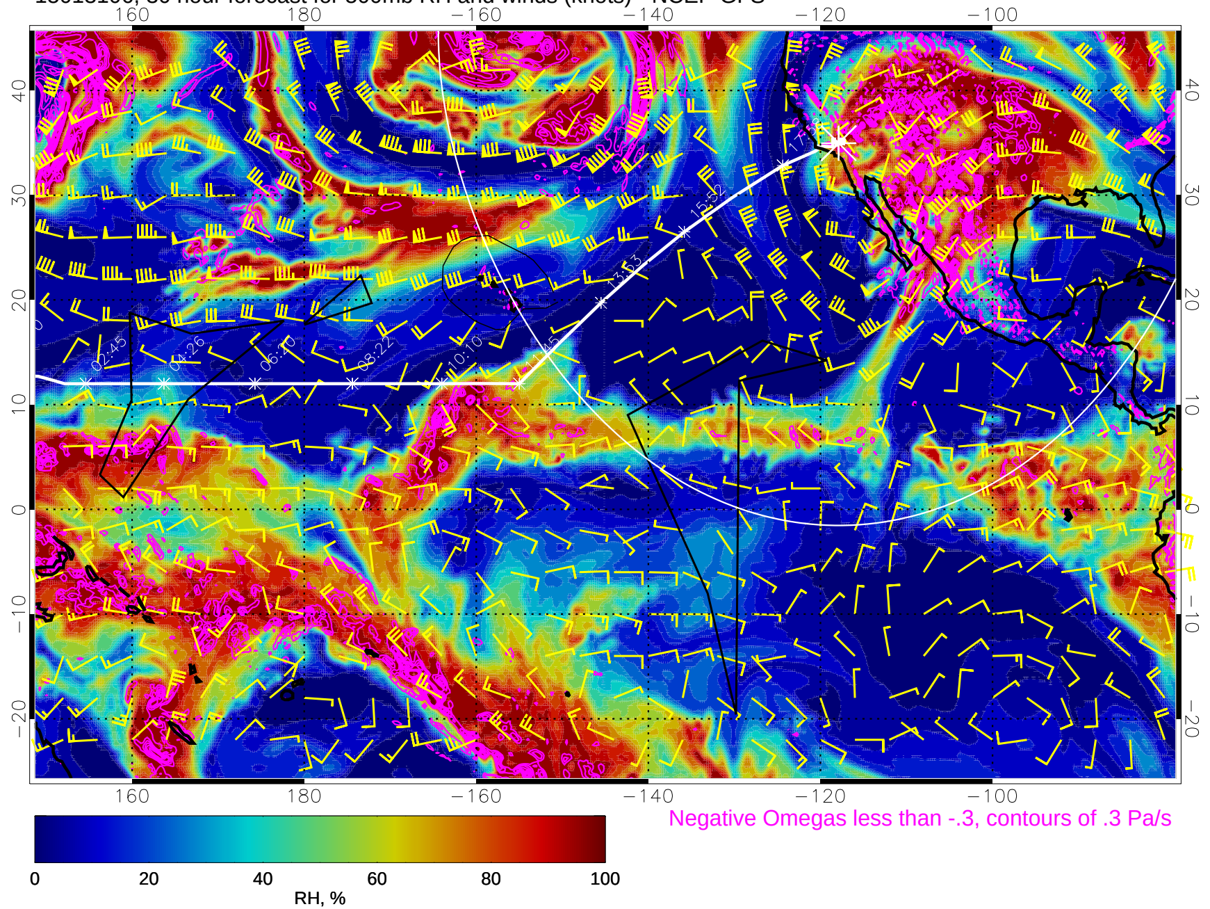
15013106, 30 hour forecast for 500mb RH and winds (knots) - NCEP GFS
