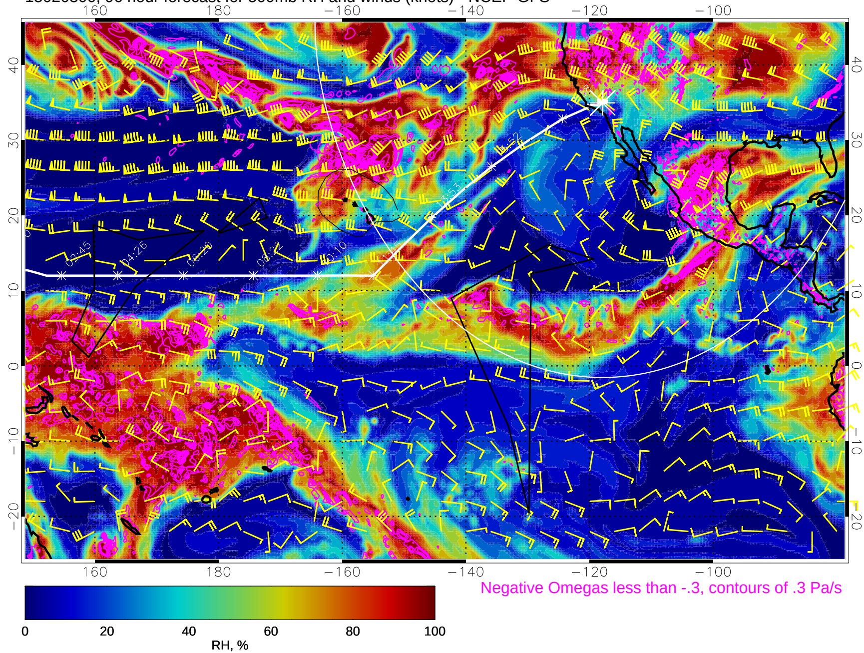
15020300, 96 hour forecast for 500mb RH and winds (knots) - NCEP GFS
