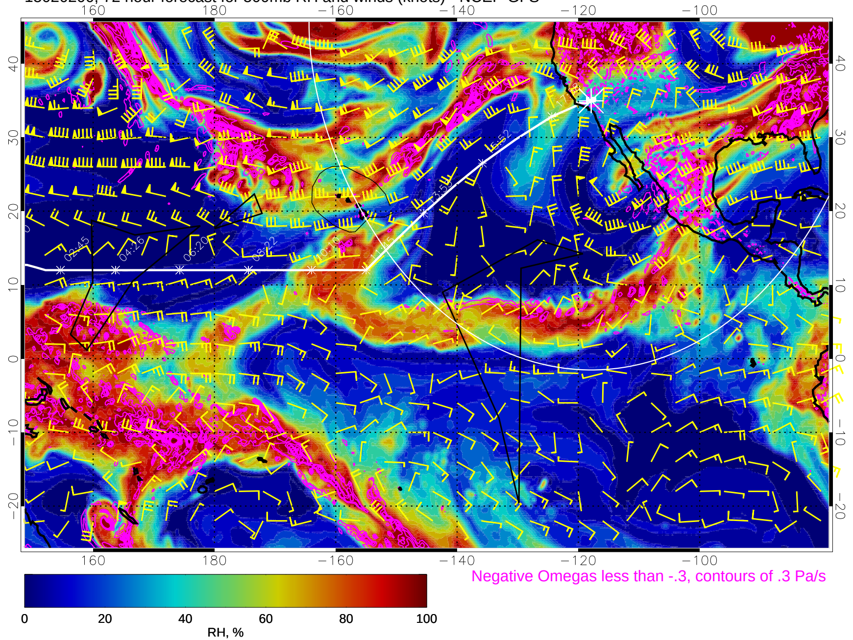
15020200, 72 hour forecast for 500mb RH and winds (knots) - NCEP GFS
