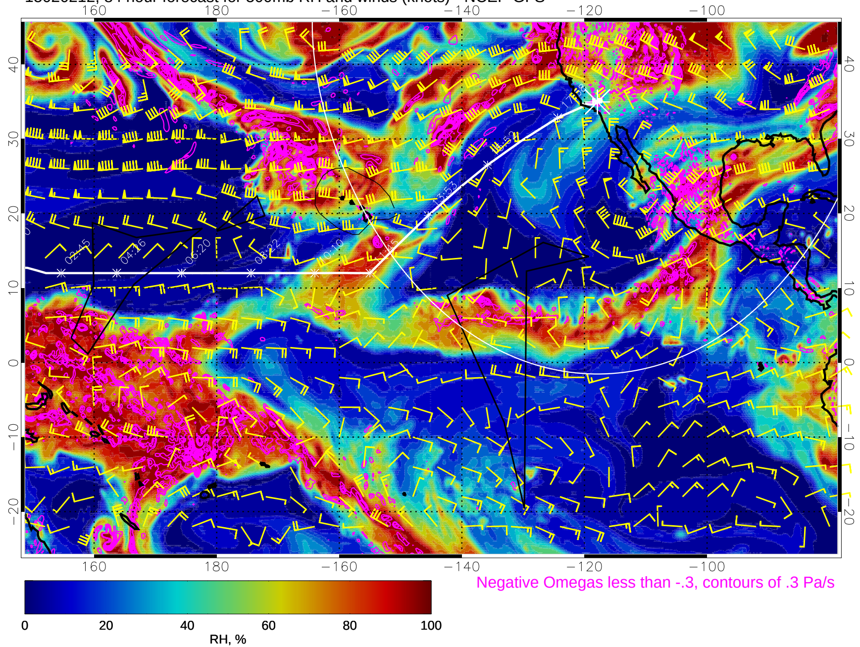
15020212, 84 hour forecast for 500mb RH and winds (knots) - NCEP GFS
