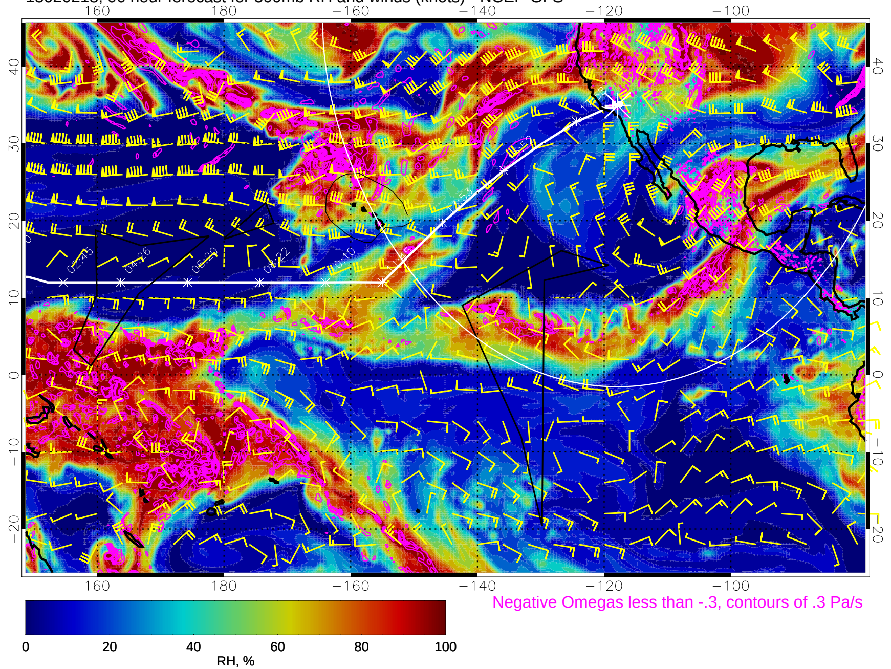
15020218, 90 hour forecast for 500mb RH and winds (knots) - NCEP GFS
