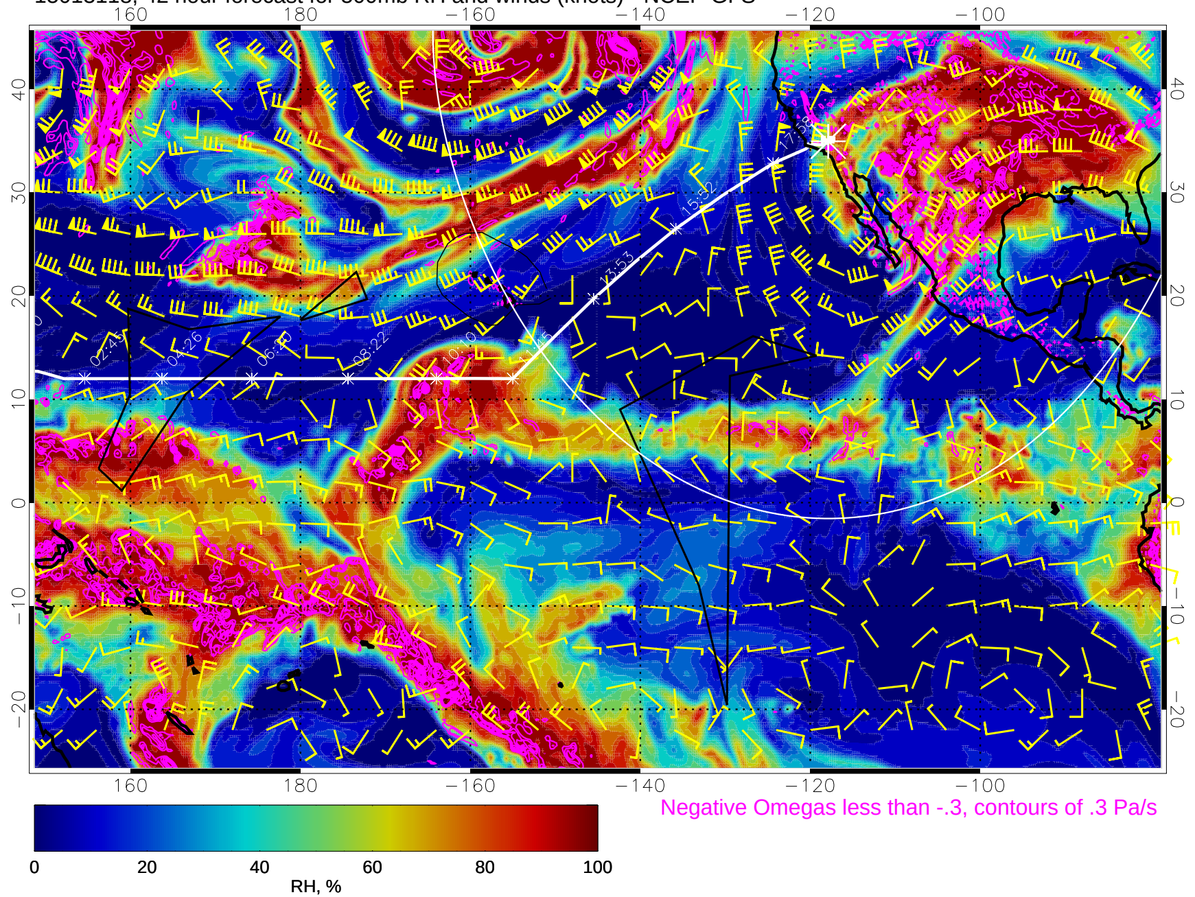
15013118, 42 hour forecast for 500mb RH and winds (knots) - NCEP GFS
