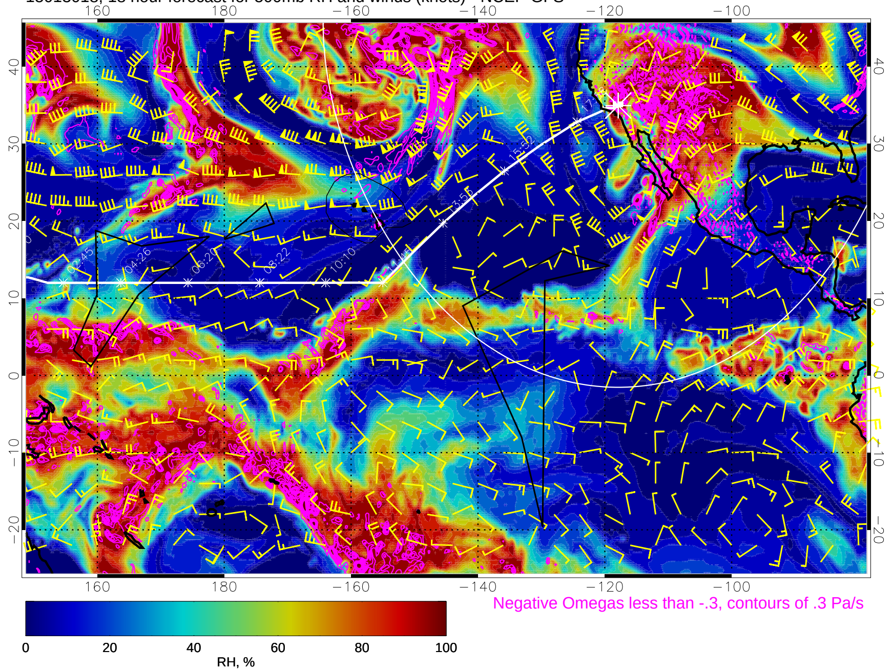
15013018, 18 hour forecast for 500mb RH and winds (knots) - NCEP GFS
