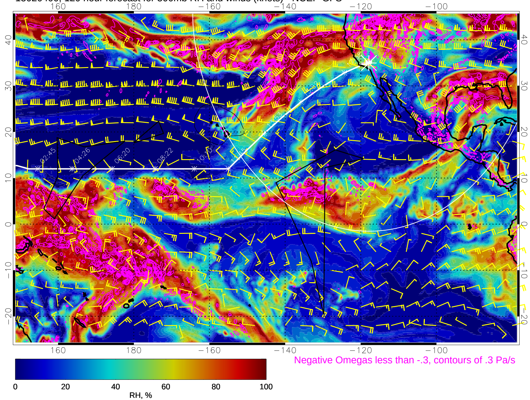
15020400, 120 hour forecast for 500mb RH and winds (knots) - NCEP GFS
