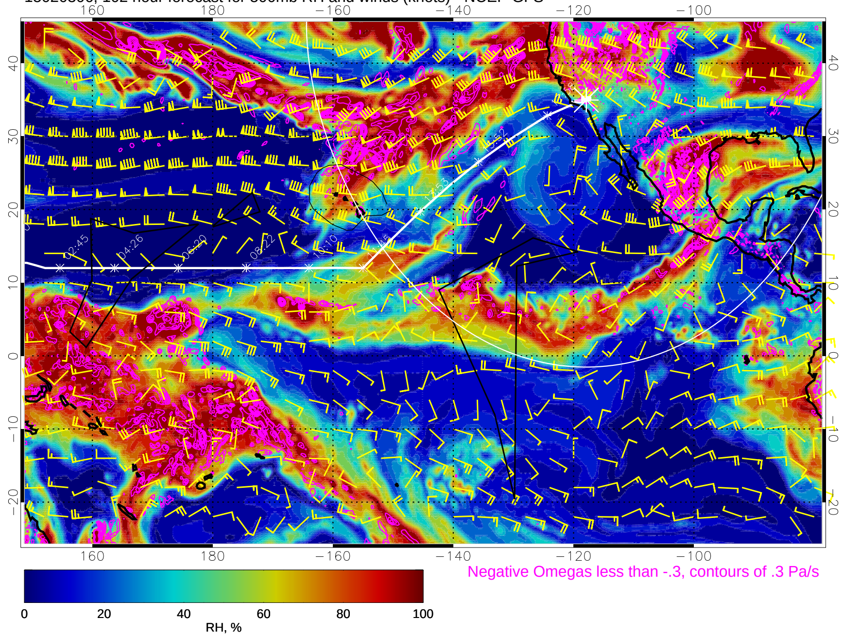
15020306, 102 hour forecast for 500mb RH and winds (knots) - NCEP GFS
