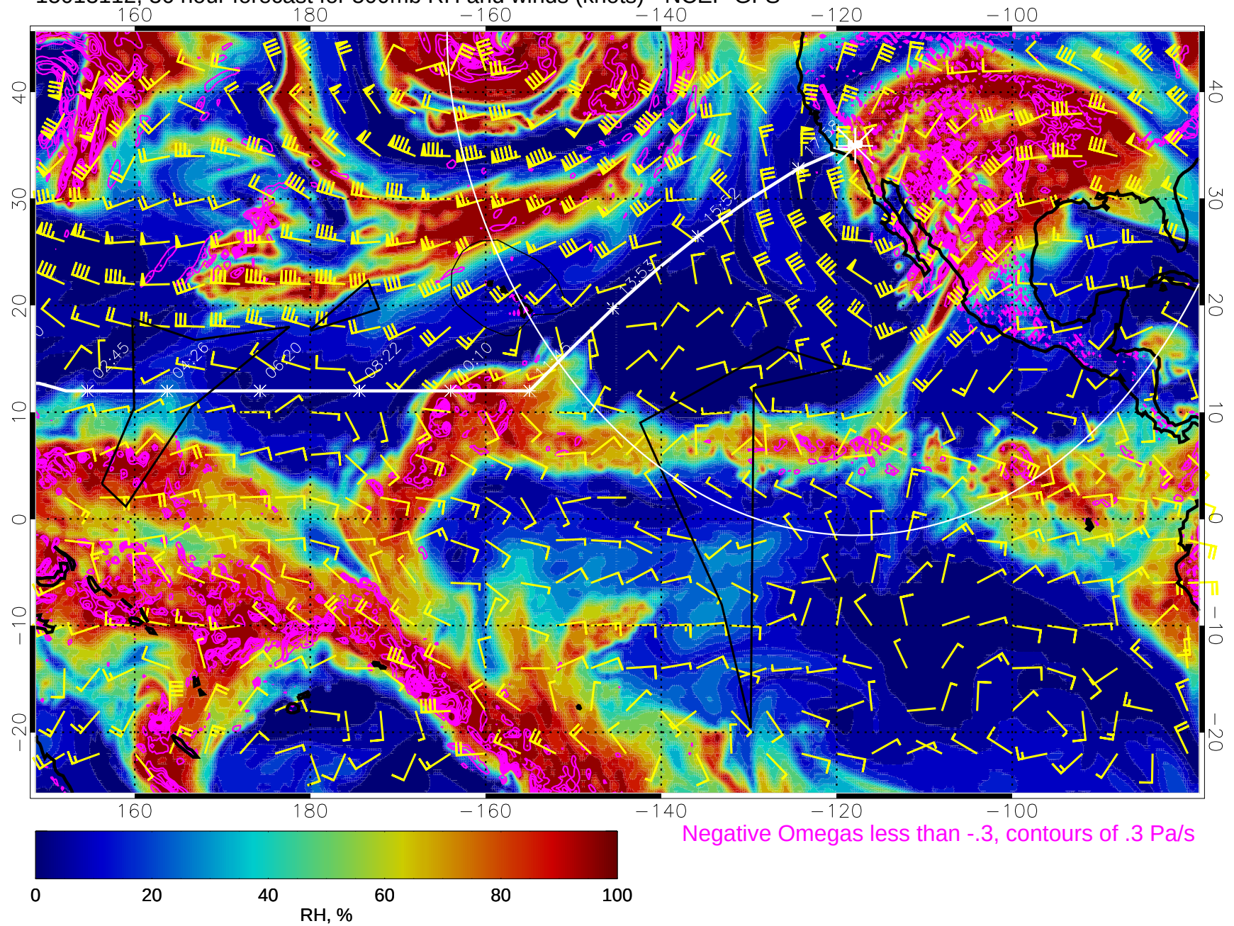
15013112, 36 hour forecast for 500mb RH and winds (knots) - NCEP GFS
