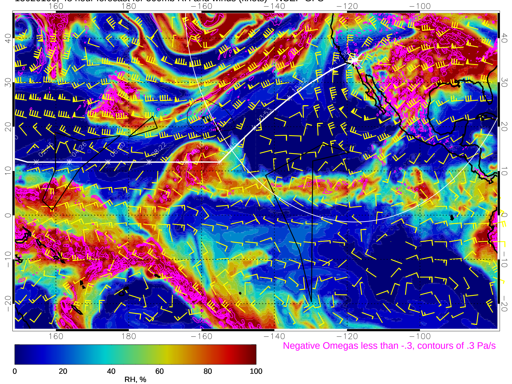
15020100, 48 hour forecast for 500mb RH and winds (knots) - NCEP GFS
