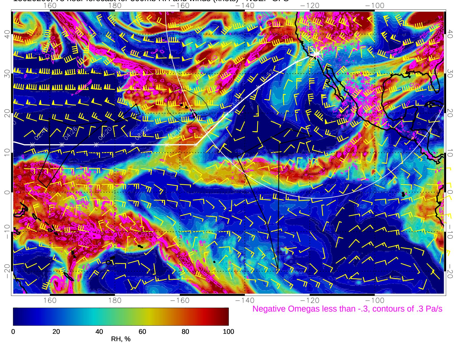
15020206, 78 hour forecast for 500mb RH and winds (knots) - NCEP GFS
