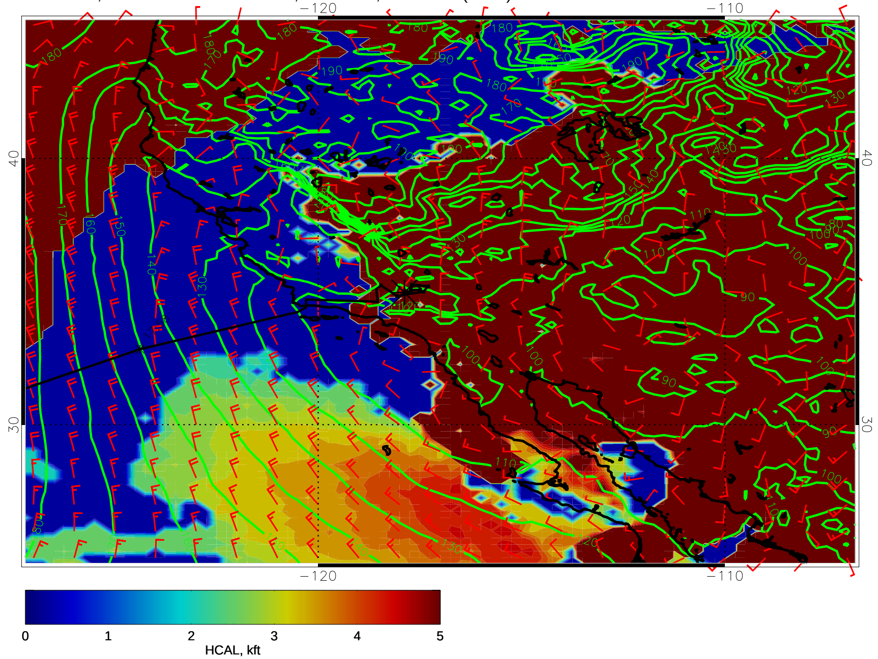
15013118, 42 hour forecast for HCAL, 1000mb Z, and winds (knots) -- NCEP GFS
