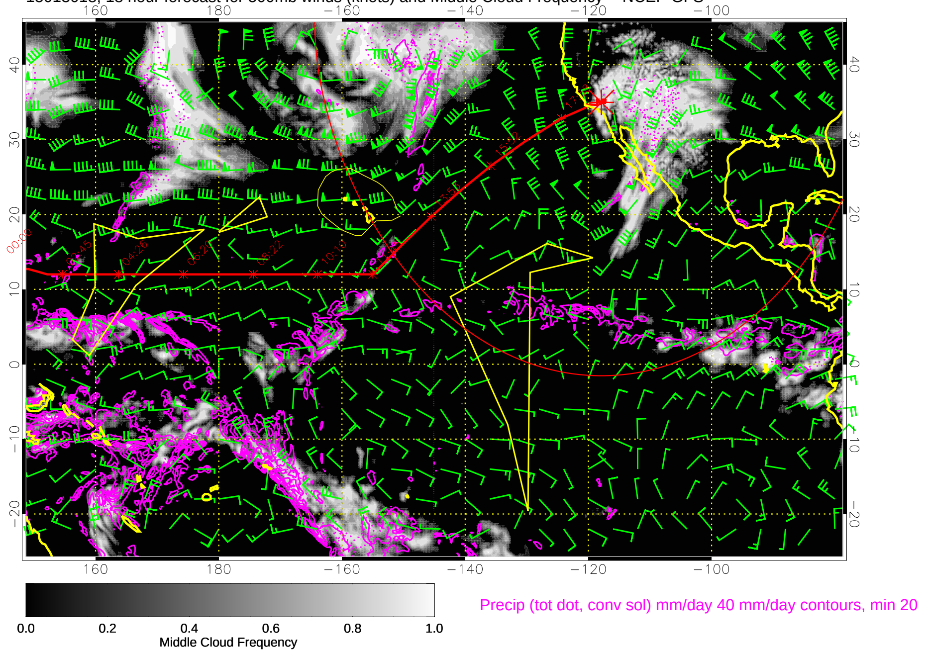
15013018, 18 hour forecast for 500mb winds (knots) and Middle Cloud Frequency -- NCEP GFS
