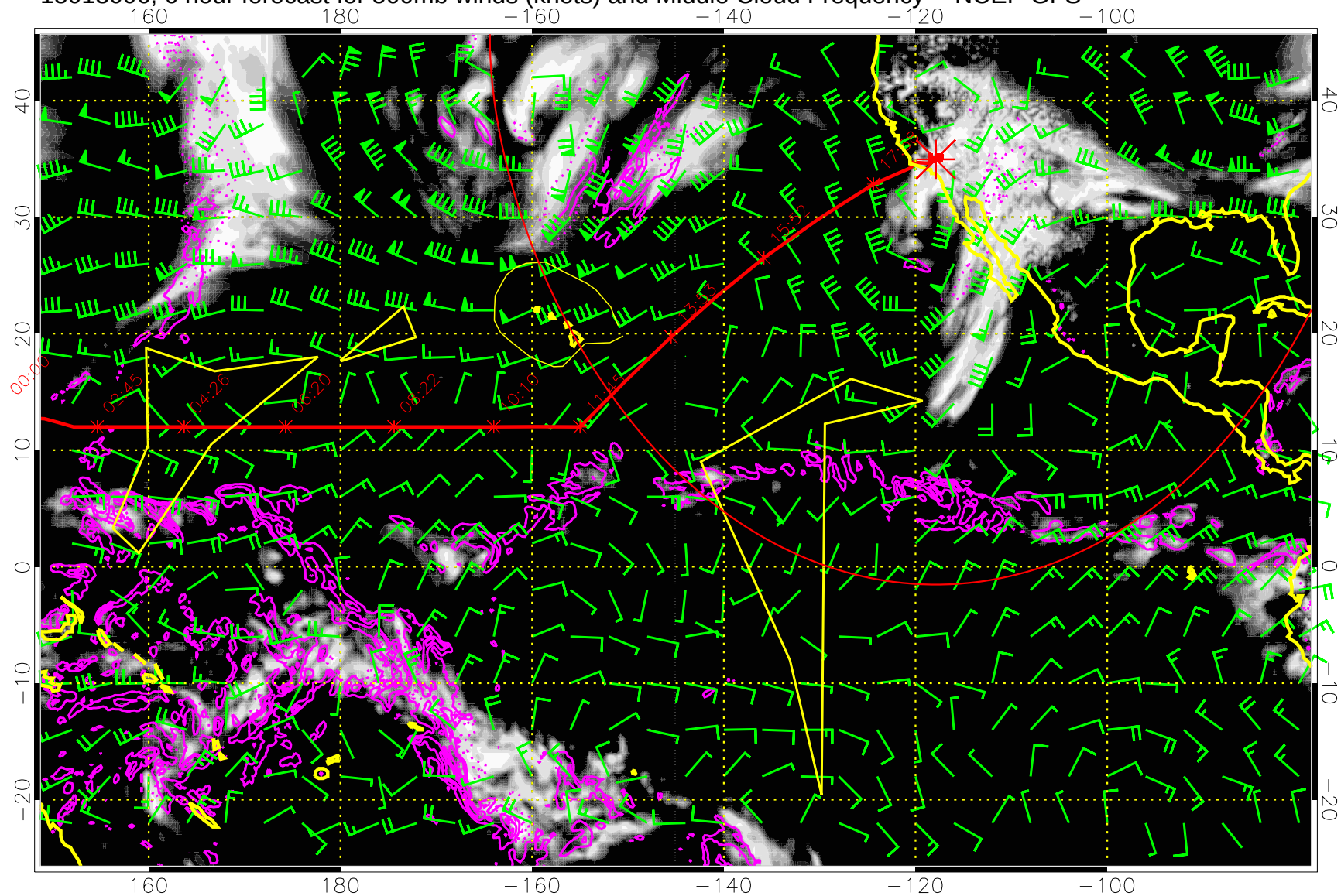
15013006, 6 hour forecast for 500mb winds (knots) and Middle Cloud Frequency -- NCEP GFS
