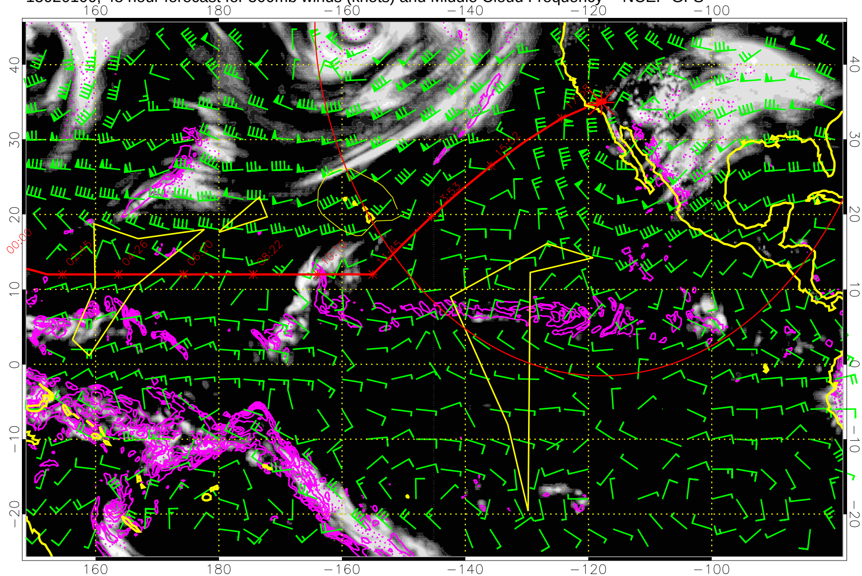
15020100, 48 hour forecast for 500mb winds (knots) and Middle Cloud Frequency -- NCEP GFS
