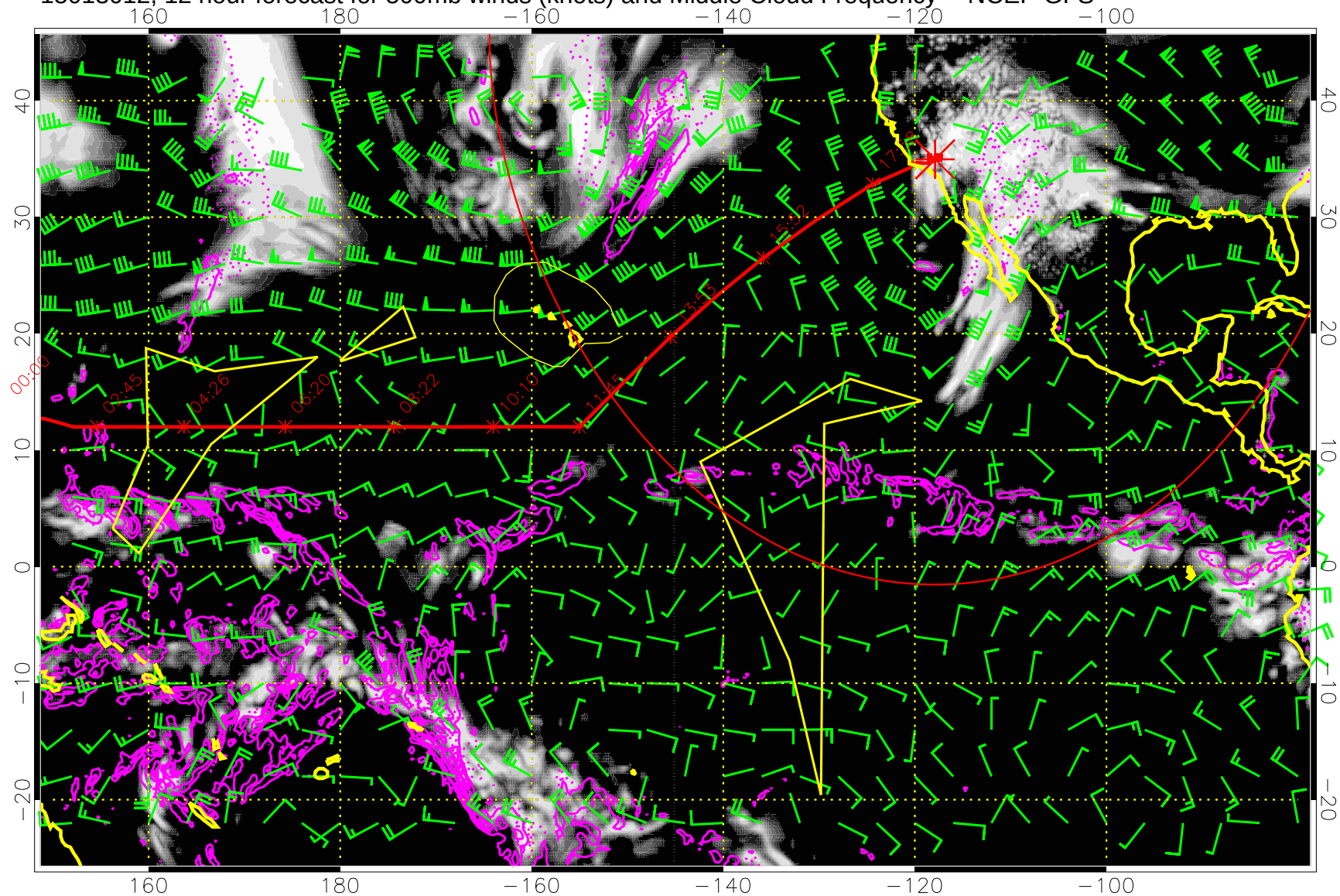
15013012, 12 hour forecast for 500mb winds (knots) and Middle Cloud Frequency -- NCEP GFS
