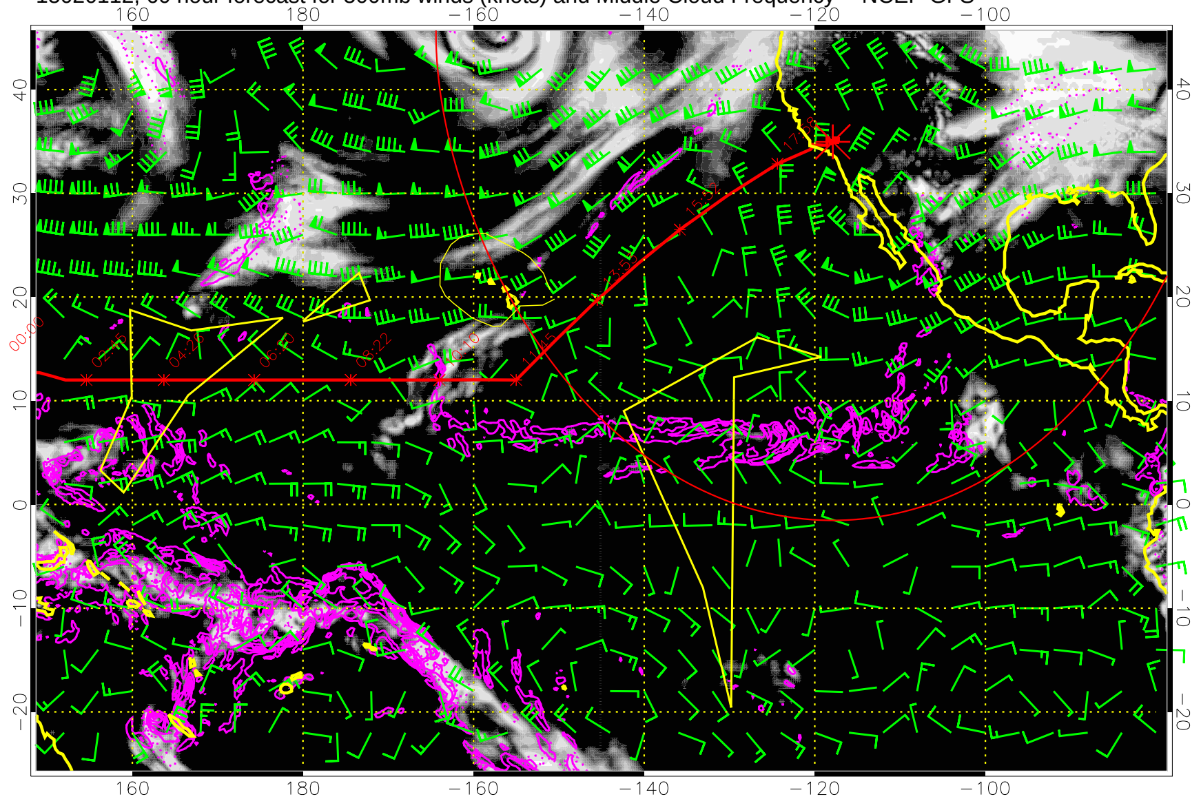
15020112, 60 hour forecast for 500mb winds (knots) and Middle Cloud Frequency -- NCEP GFS
