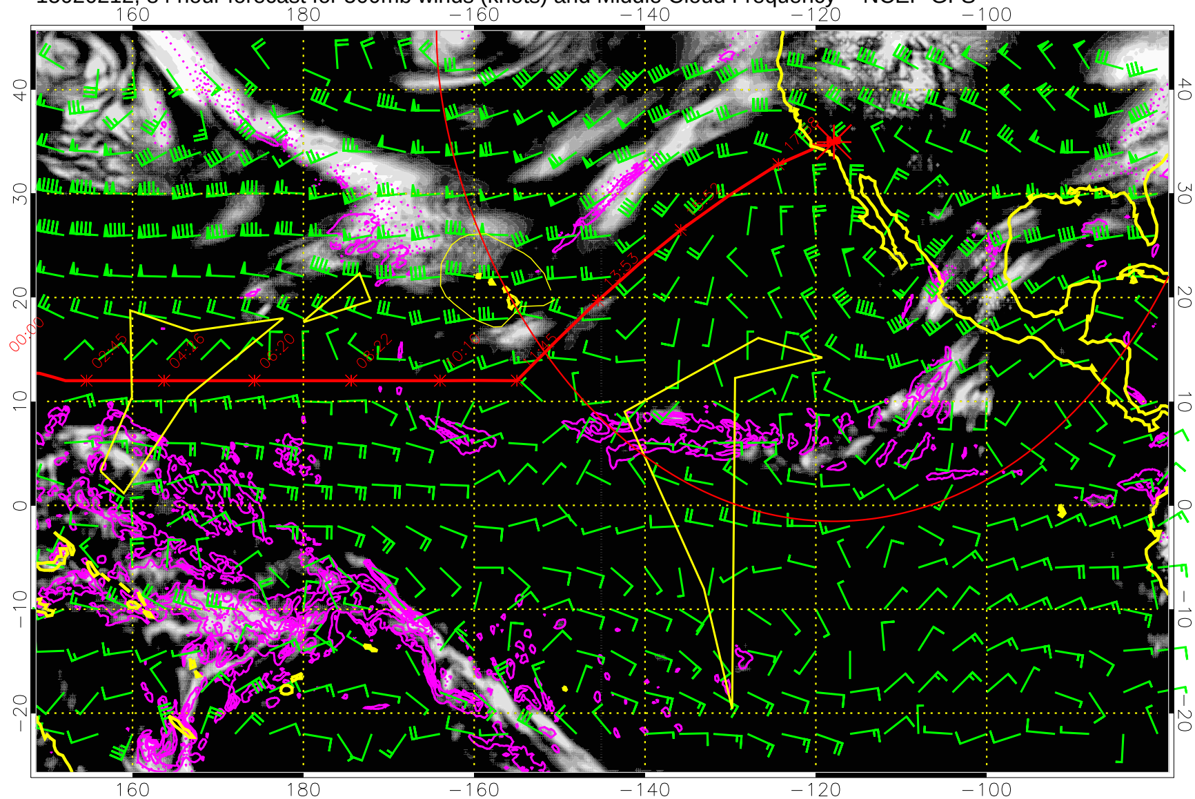
15020212, 84 hour forecast for 500mb winds (knots) and Middle Cloud Frequency -- NCEP GFS
