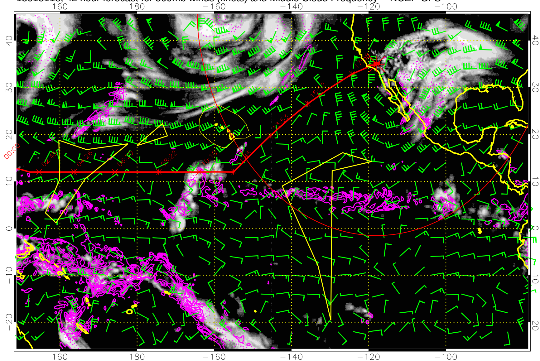
15013118, 42 hour forecast for 500mb winds (knots) and Middle Cloud Frequency -- NCEP GFS
