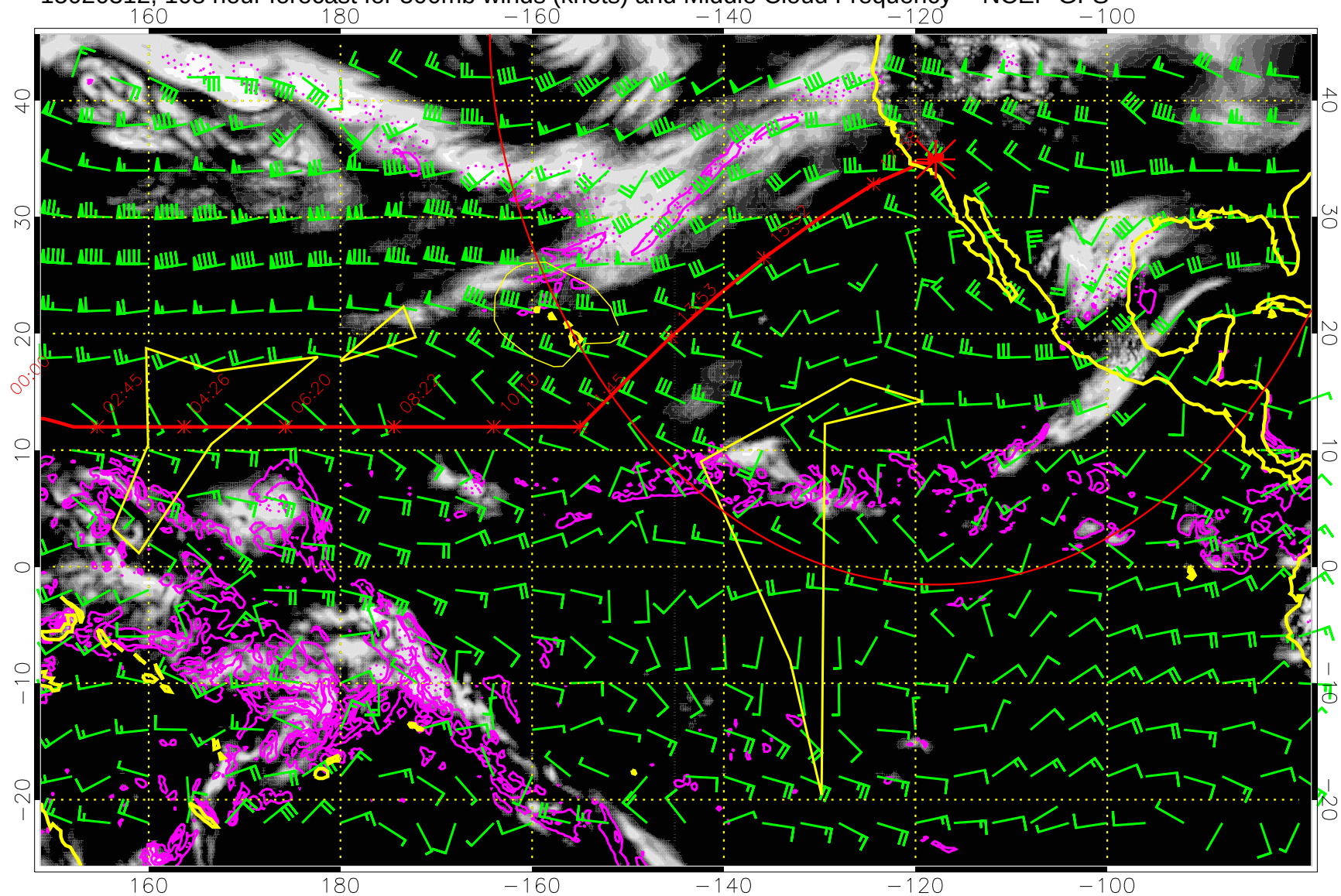
15020312, 108 hour forecast for 500mb winds (knots) and Middle Cloud Frequency -- NCEP GFS
