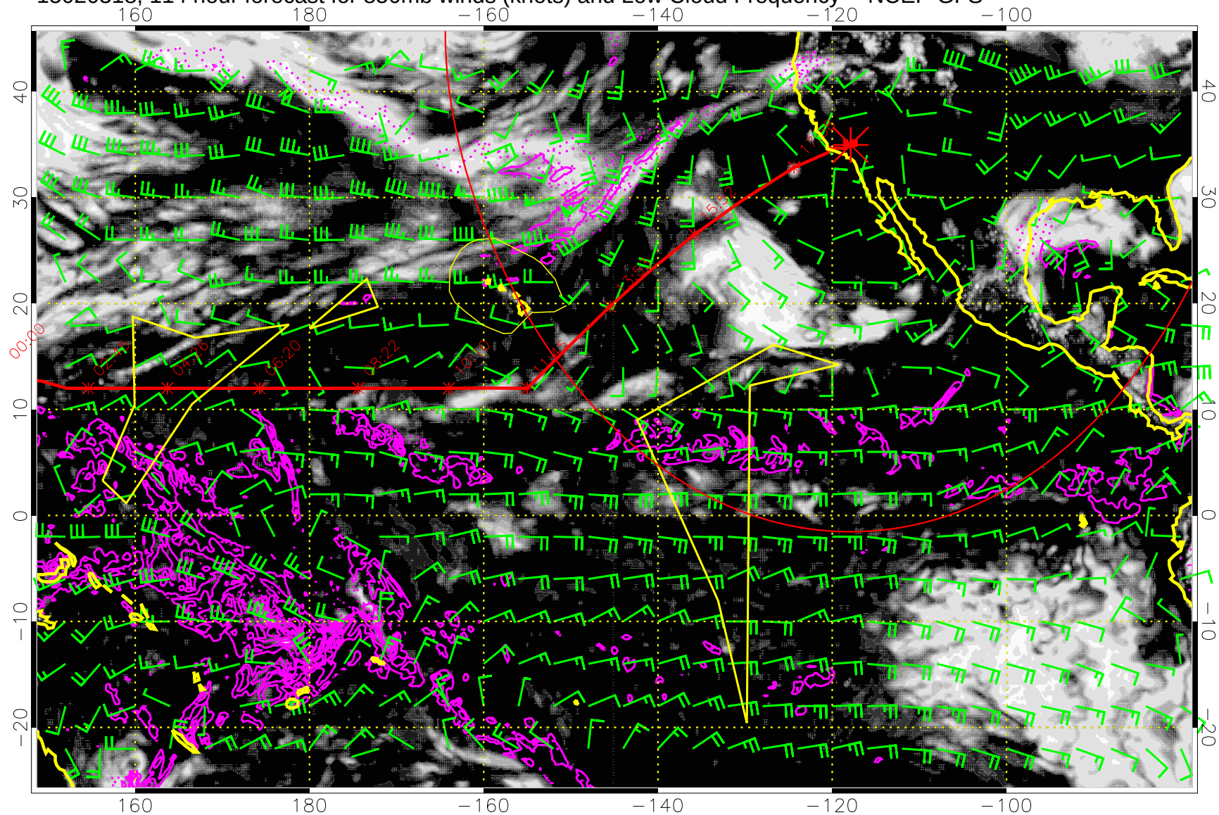
15020318, 114 hour forecast for 850mb winds (knots) and Low Cloud Frequency -- NCEP GFS
