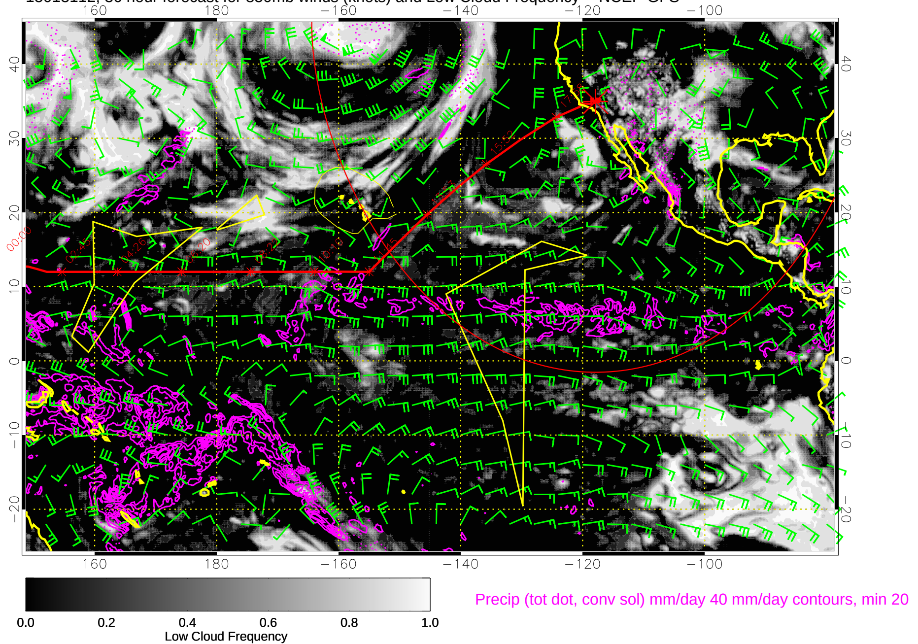
15013112, 36 hour forecast for 850mb winds (knots) and Low Cloud Frequency -- NCEP GFS
