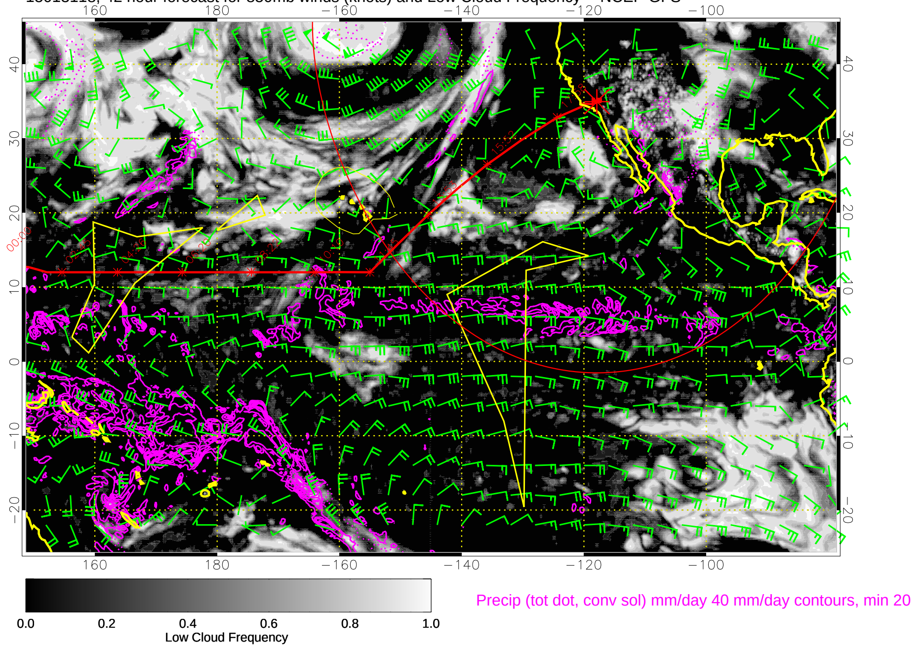
15013118, 42 hour forecast for 850mb winds (knots) and Low Cloud Frequency -- NCEP GFS
