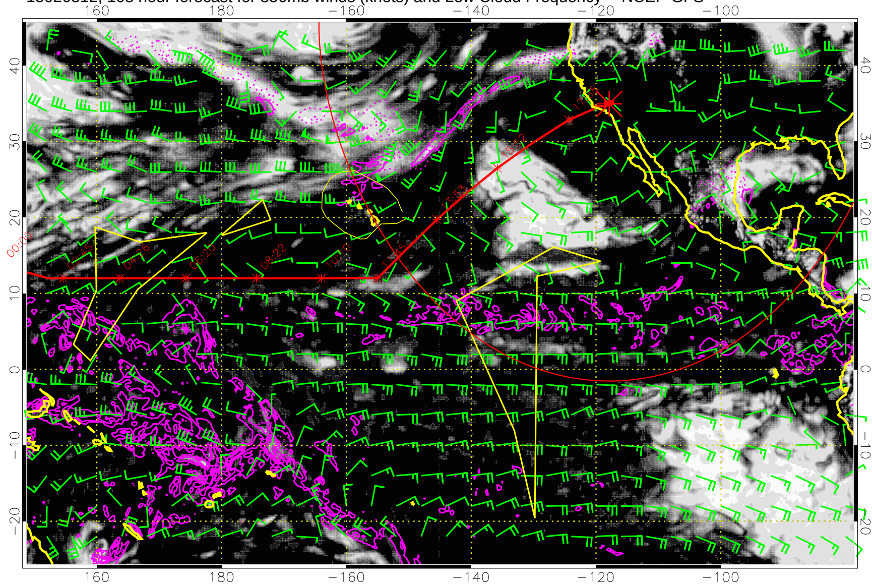
15020312, 108 hour forecast for 850mb winds (knots) and Low Cloud Frequency -- NCEP GFS
