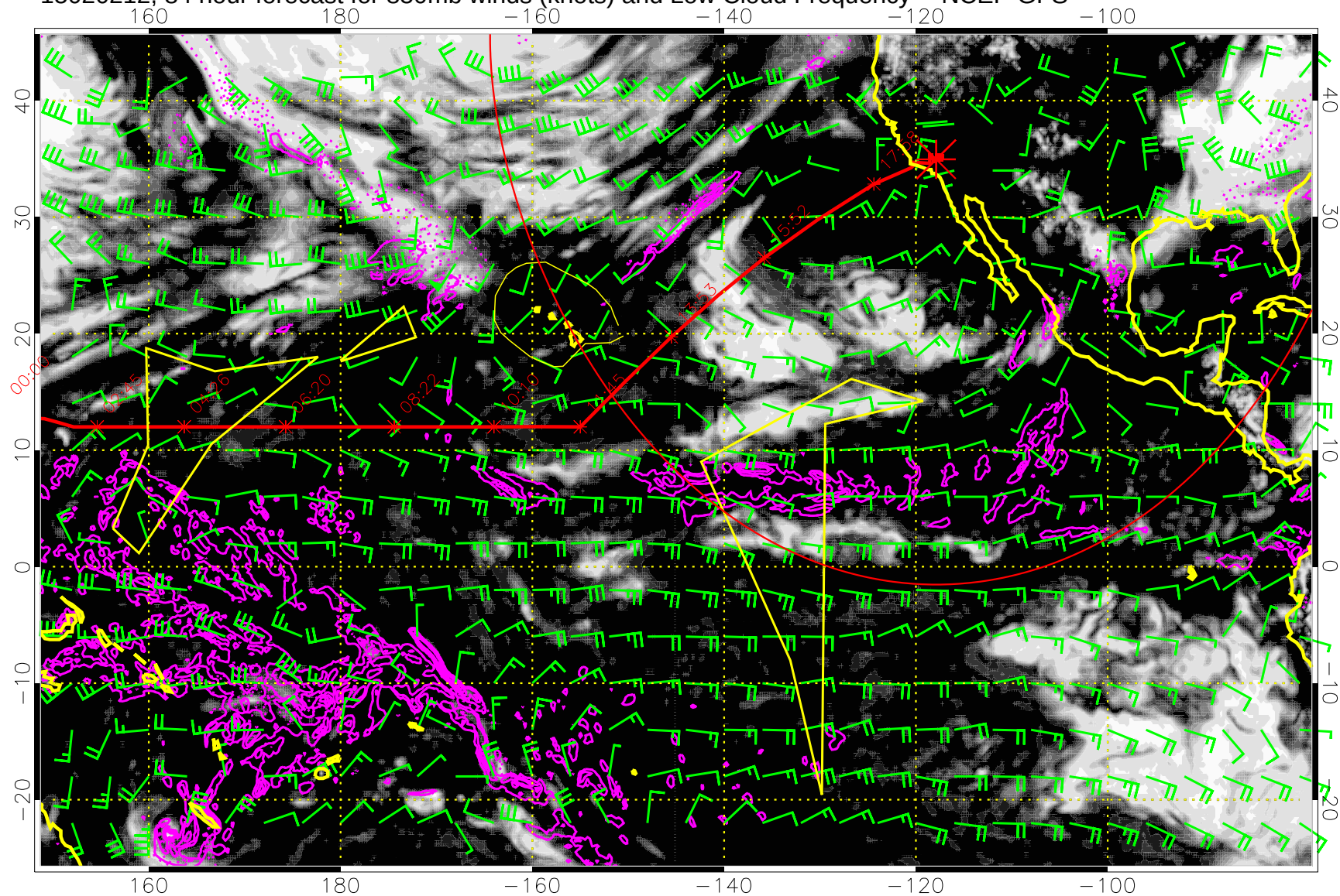
15020212, 84 hour forecast for 850mb winds (knots) and Low Cloud Frequency -- NCEP GFS
