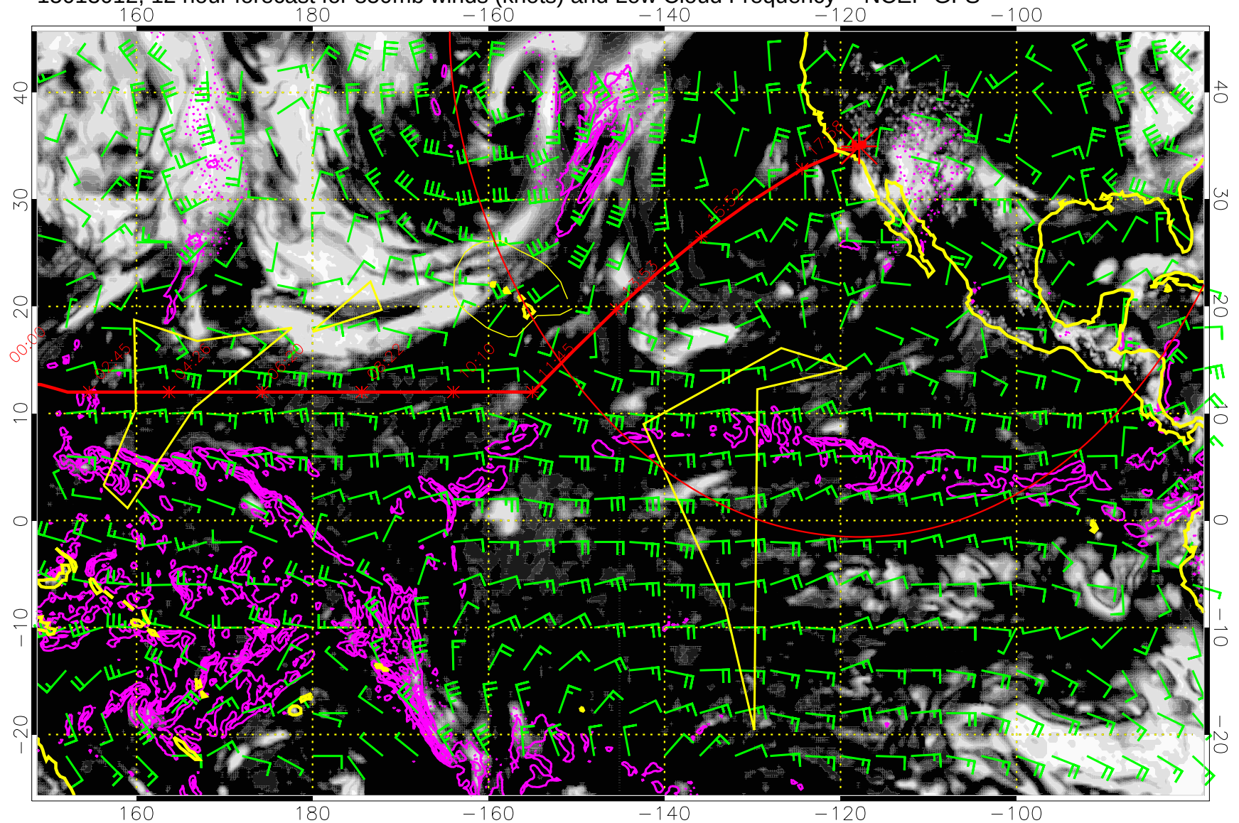
15013012, 12 hour forecast for 850mb winds (knots) and Low Cloud Frequency -- NCEP GFS
