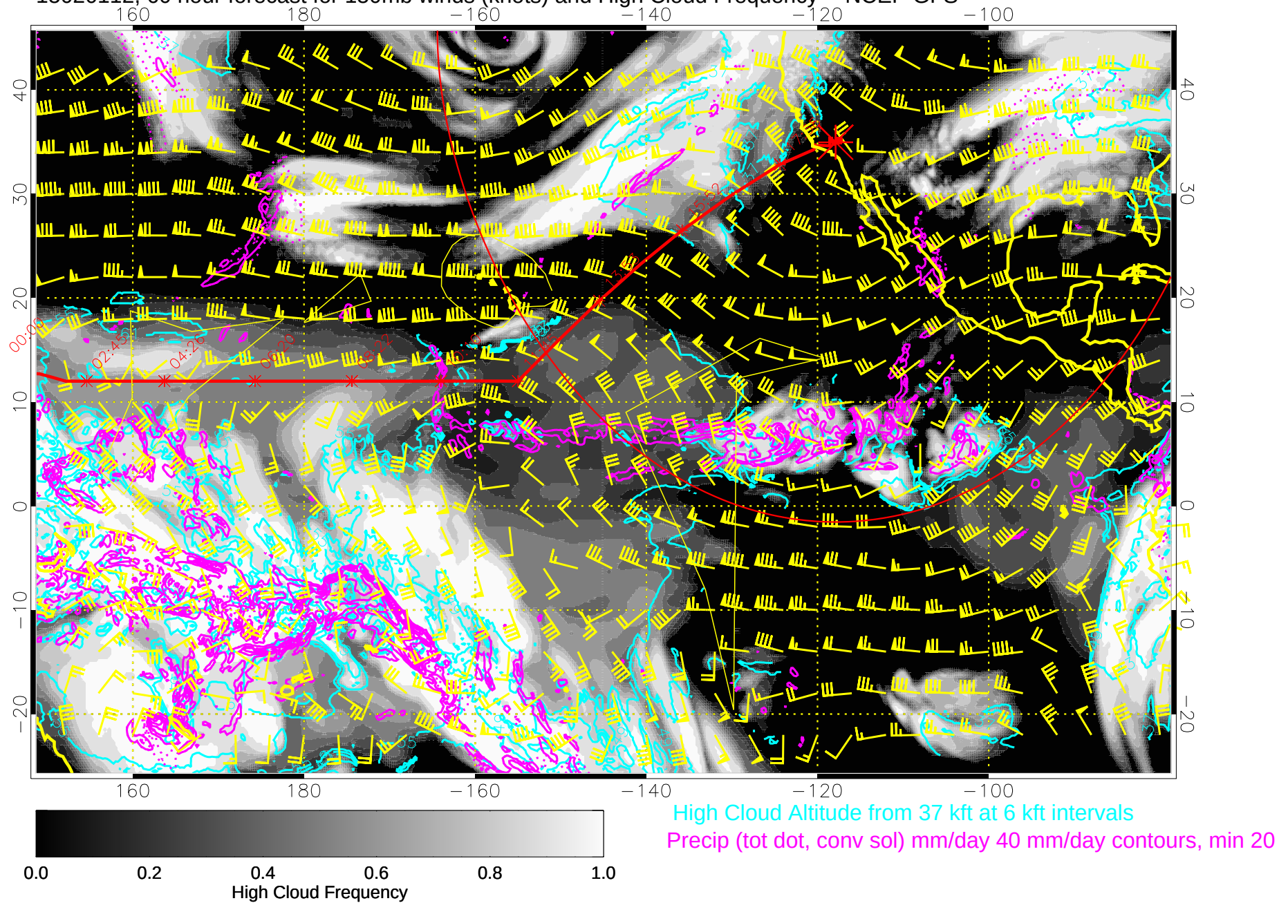
15020112, 60 hour forecast for 150mb winds (knots) and High Cloud Frequency -- NCEP GFS
