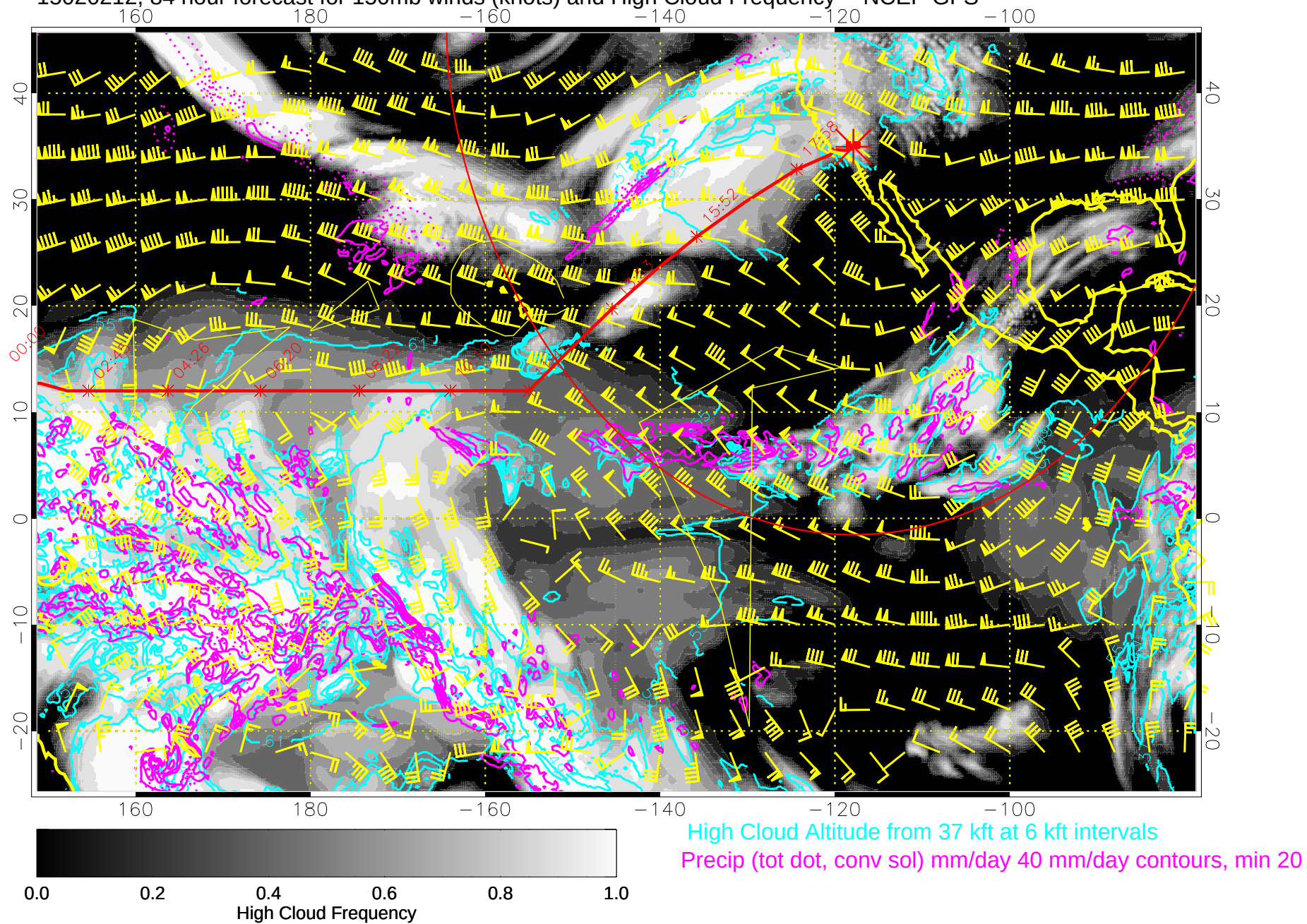
15020212, 84 hour forecast for 150mb winds (knots) and High Cloud Frequency -- NCEP GFS
