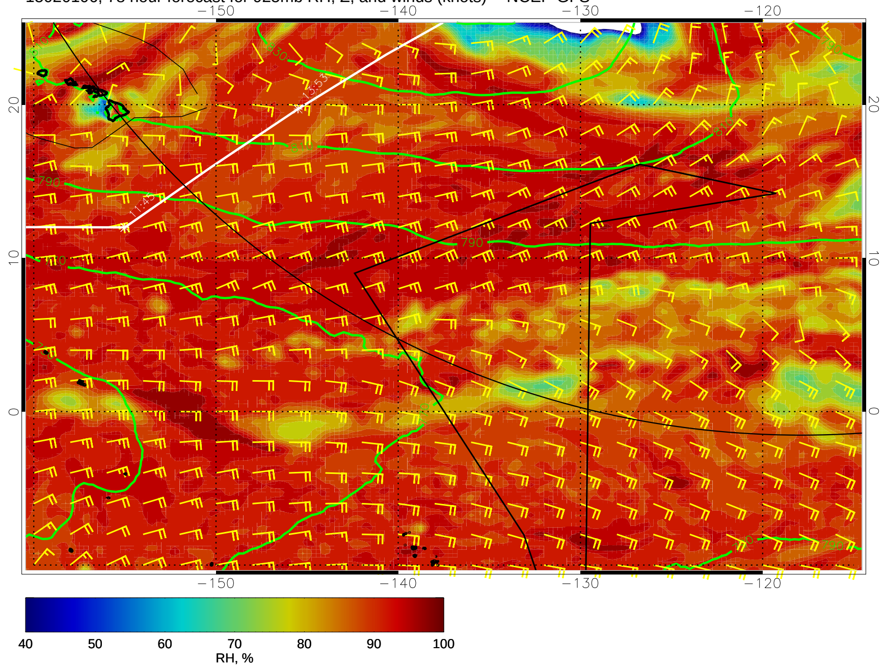
15020106, 78 hour forecast for 925mb RH, Z, and winds (knots) -- NCEP GFS
