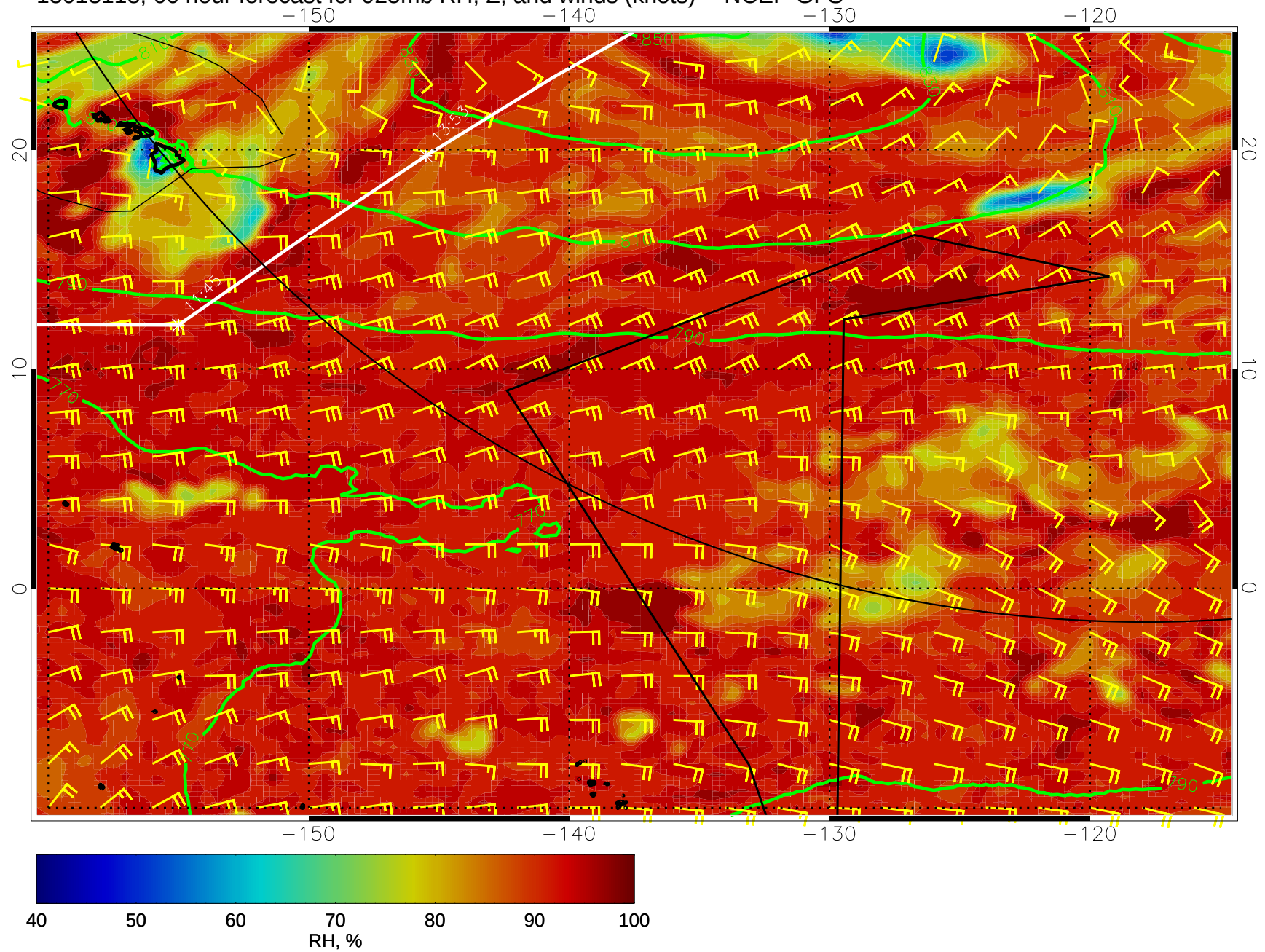
15013118, 66 hour forecast for 925mb RH, Z, and winds (knots) -- NCEP GFS
