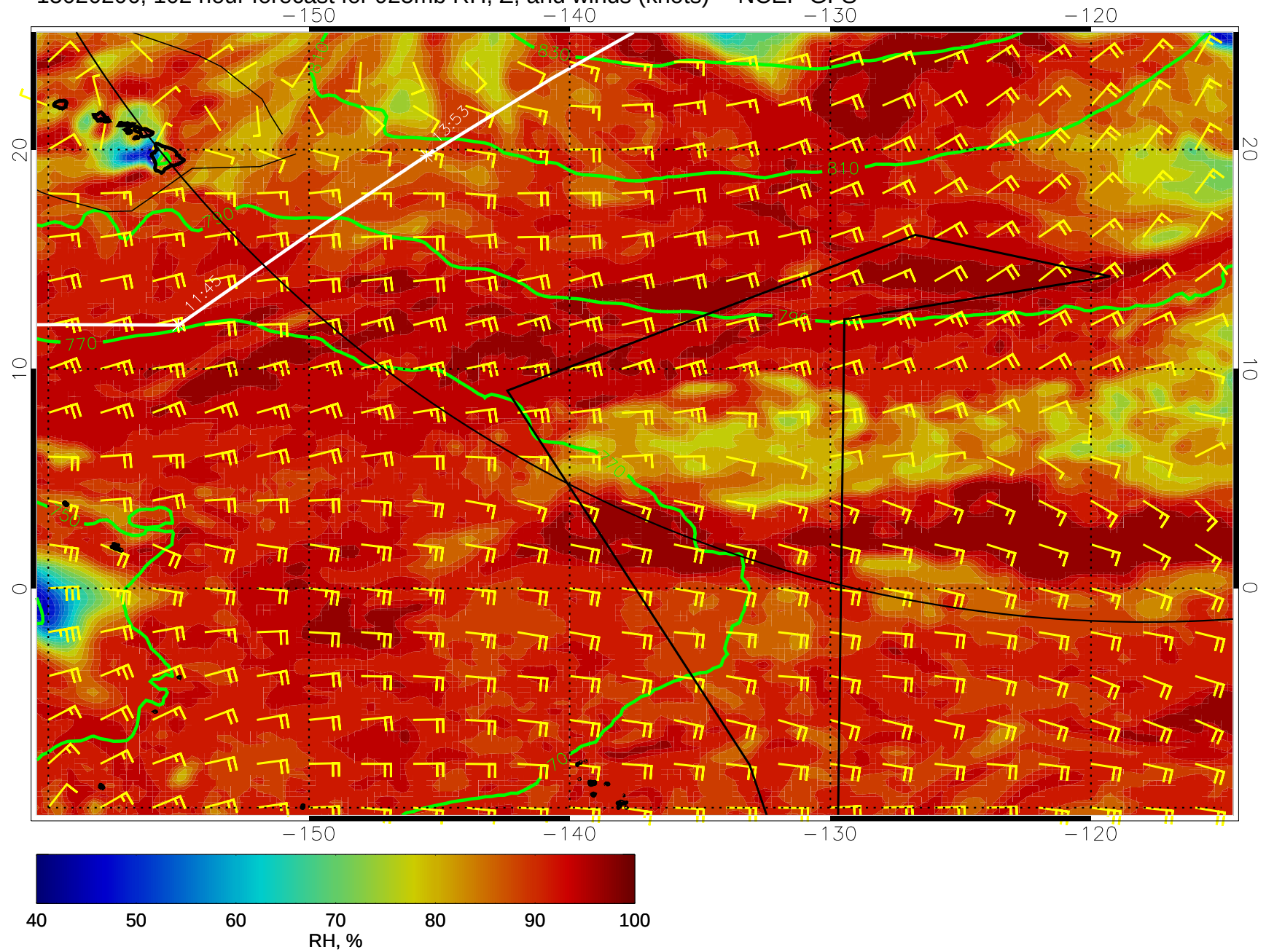
15020206, 102 hour forecast for 925mb RH, Z, and winds (knots) -- NCEP GFS
