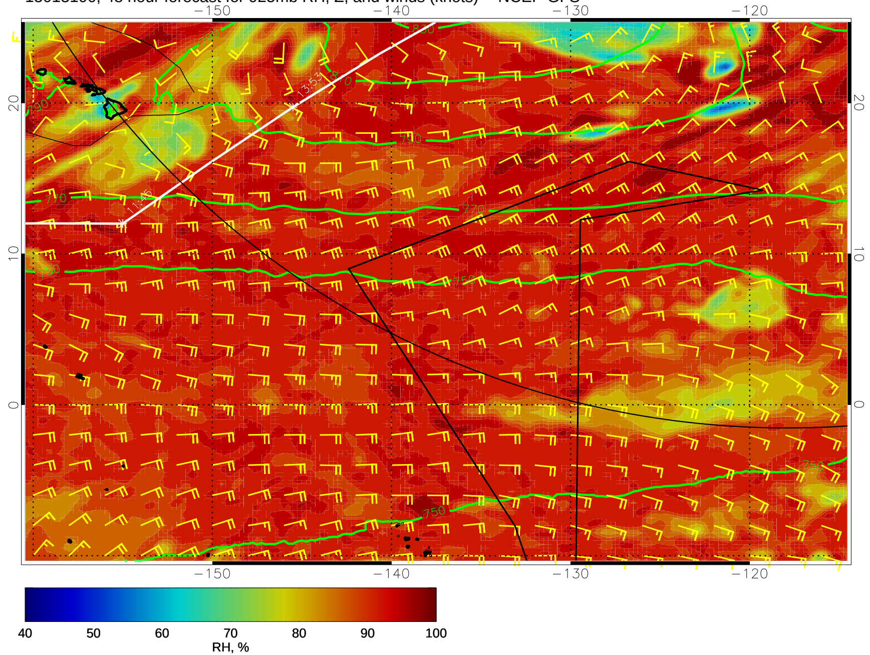
15013100, 48 hour forecast for 925mb RH, Z, and winds (knots) -- NCEP GFS
