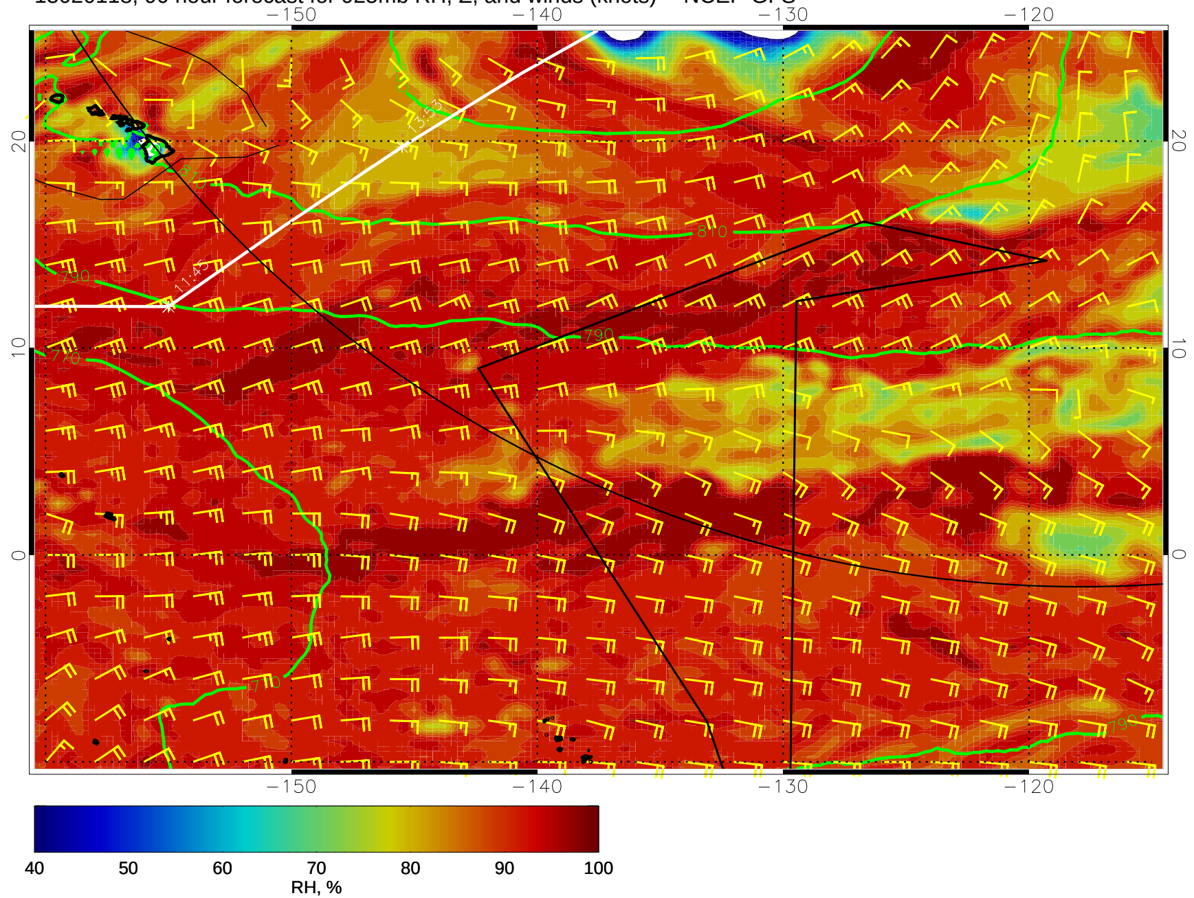
15020118, 90 hour forecast for 925mb RH, Z, and winds (knots) -- NCEP GFS
