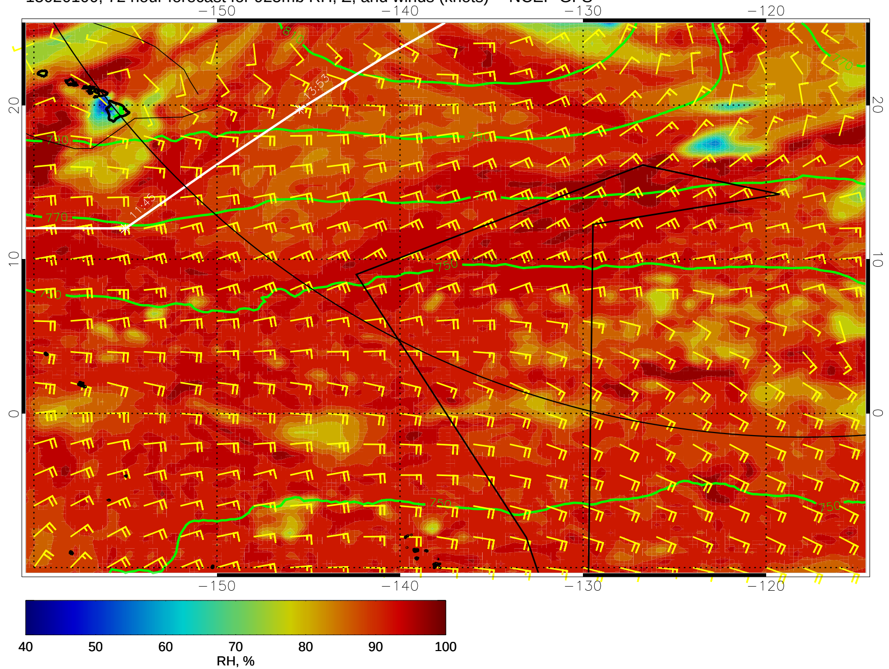
15020100, 72 hour forecast for 925mb RH, Z, and winds (knots) -- NCEP GFS
