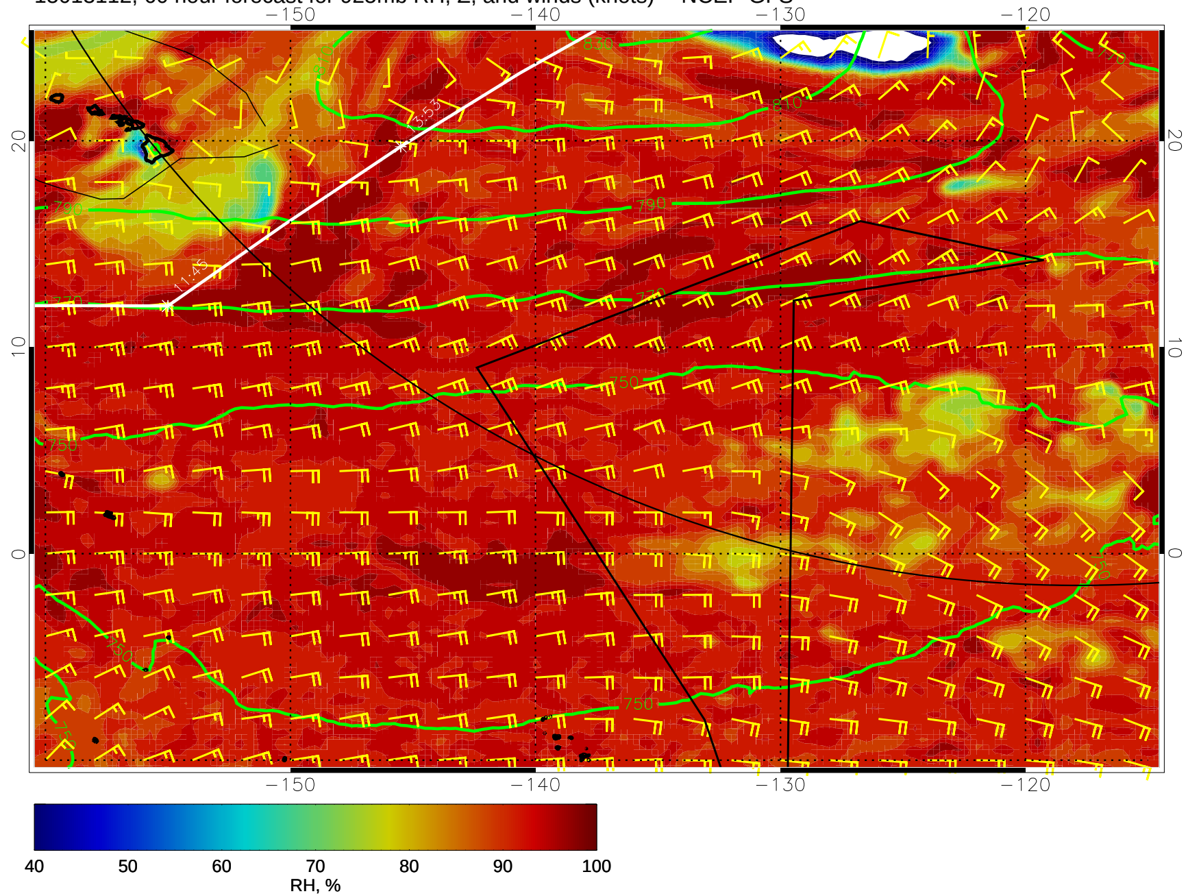
15013112, 60 hour forecast for 925mb RH, Z, and winds (knots) -- NCEP GFS
