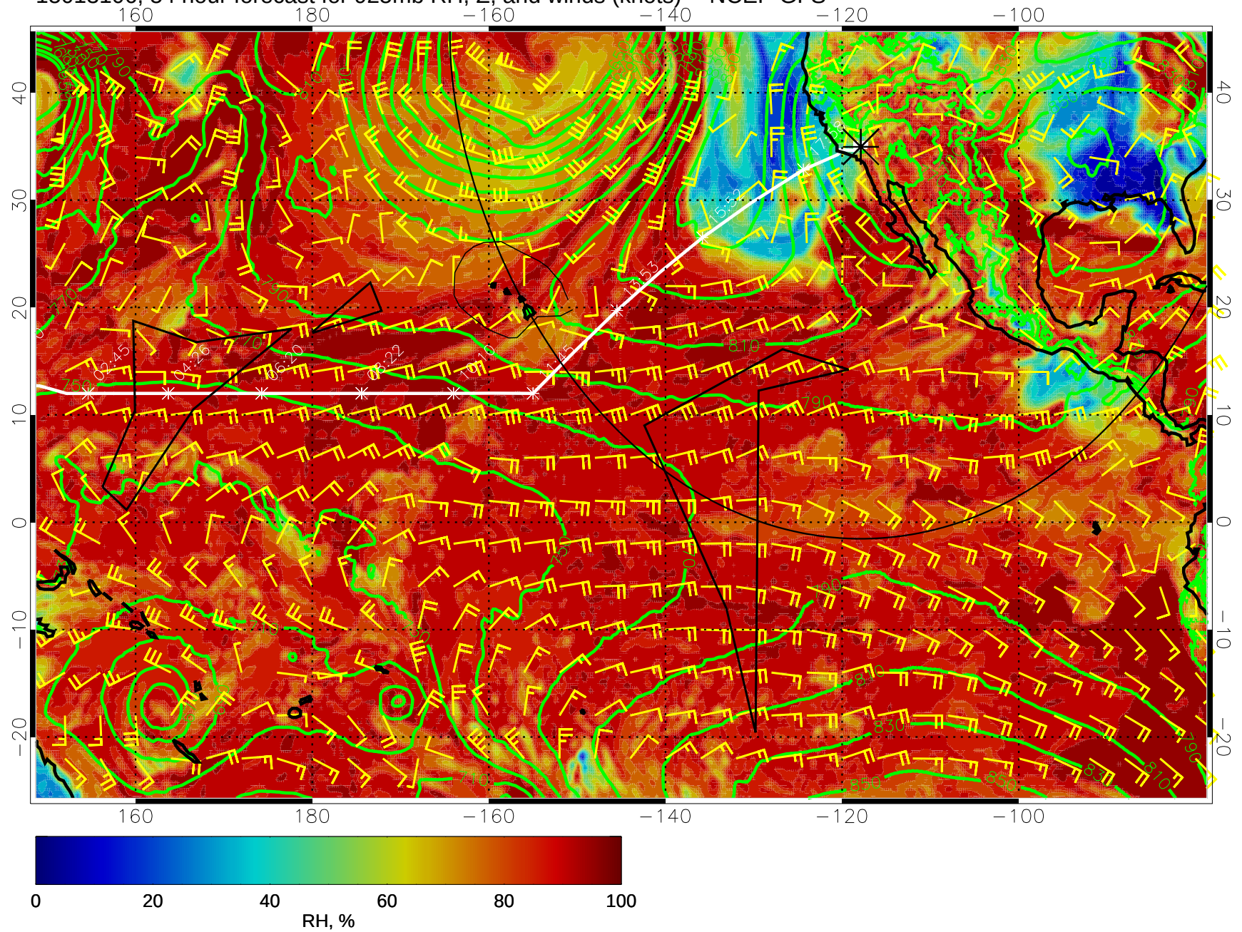
15013106, 54 hour forecast for 925mb RH, Z, and winds (knots) -- NCEP GFS
