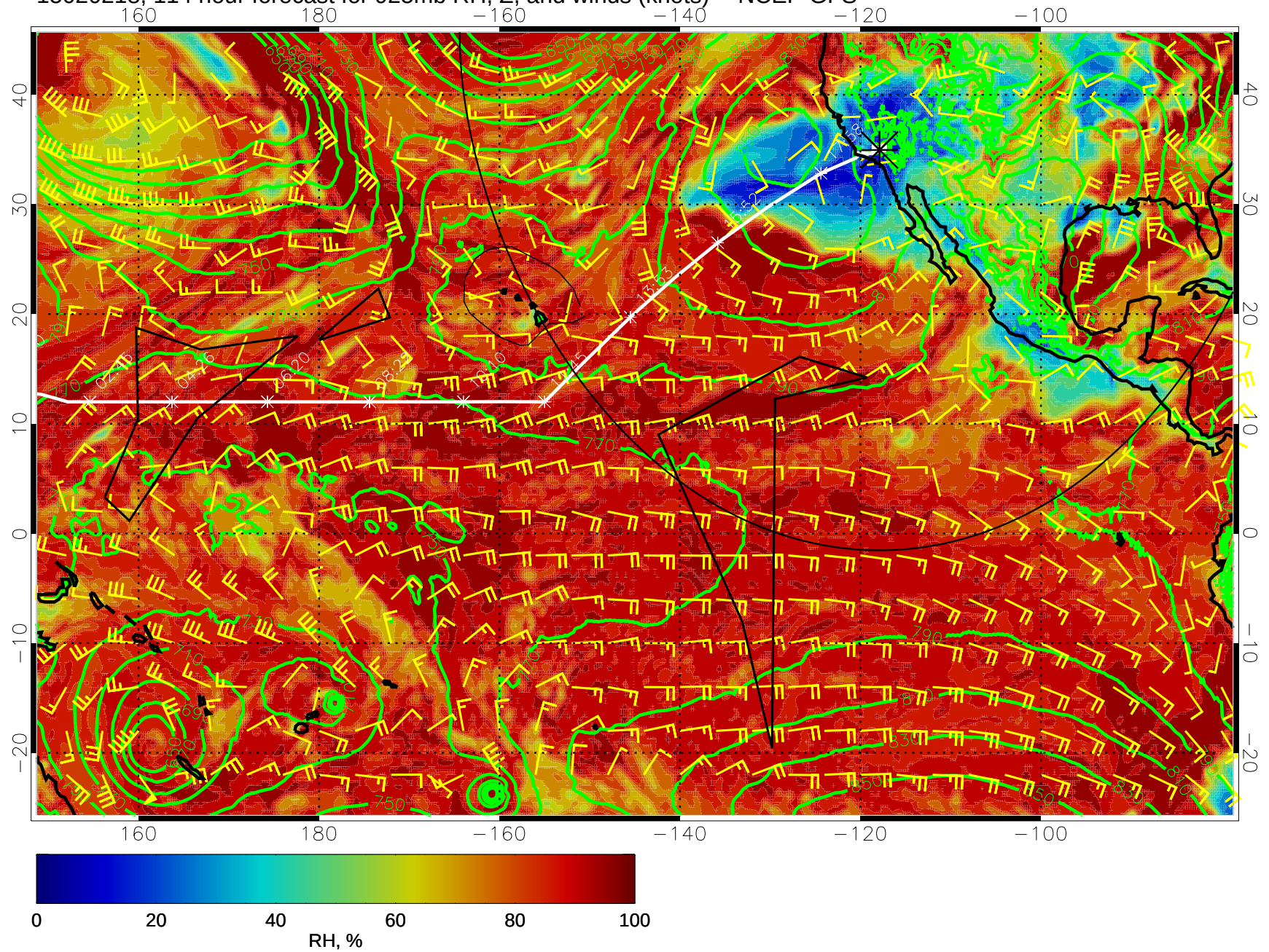
15020218, 114 hour forecast for 925mb RH, Z, and winds (knots) -- NCEP GFS
