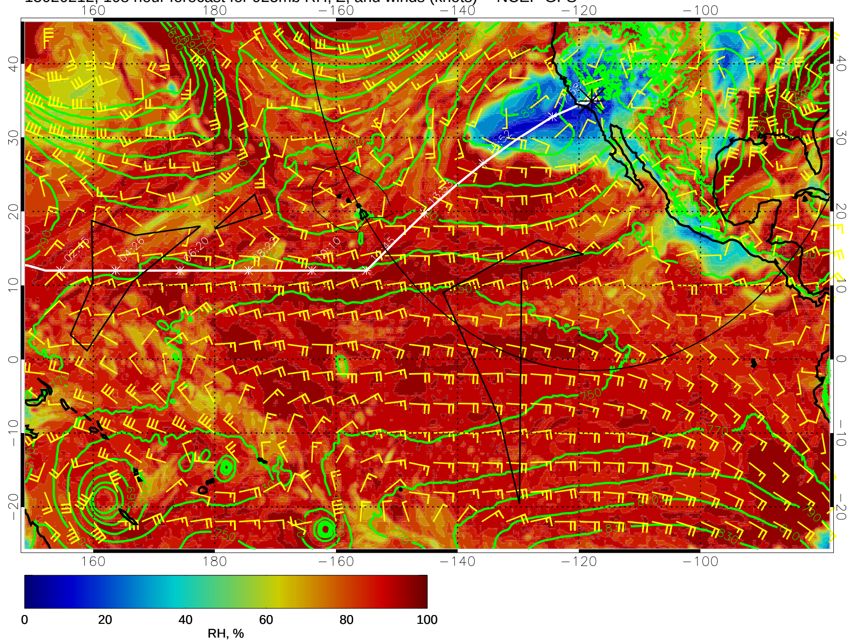
15020212, 108 hour forecast for 925mb RH, Z, and winds (knots) -- NCEP GFS
