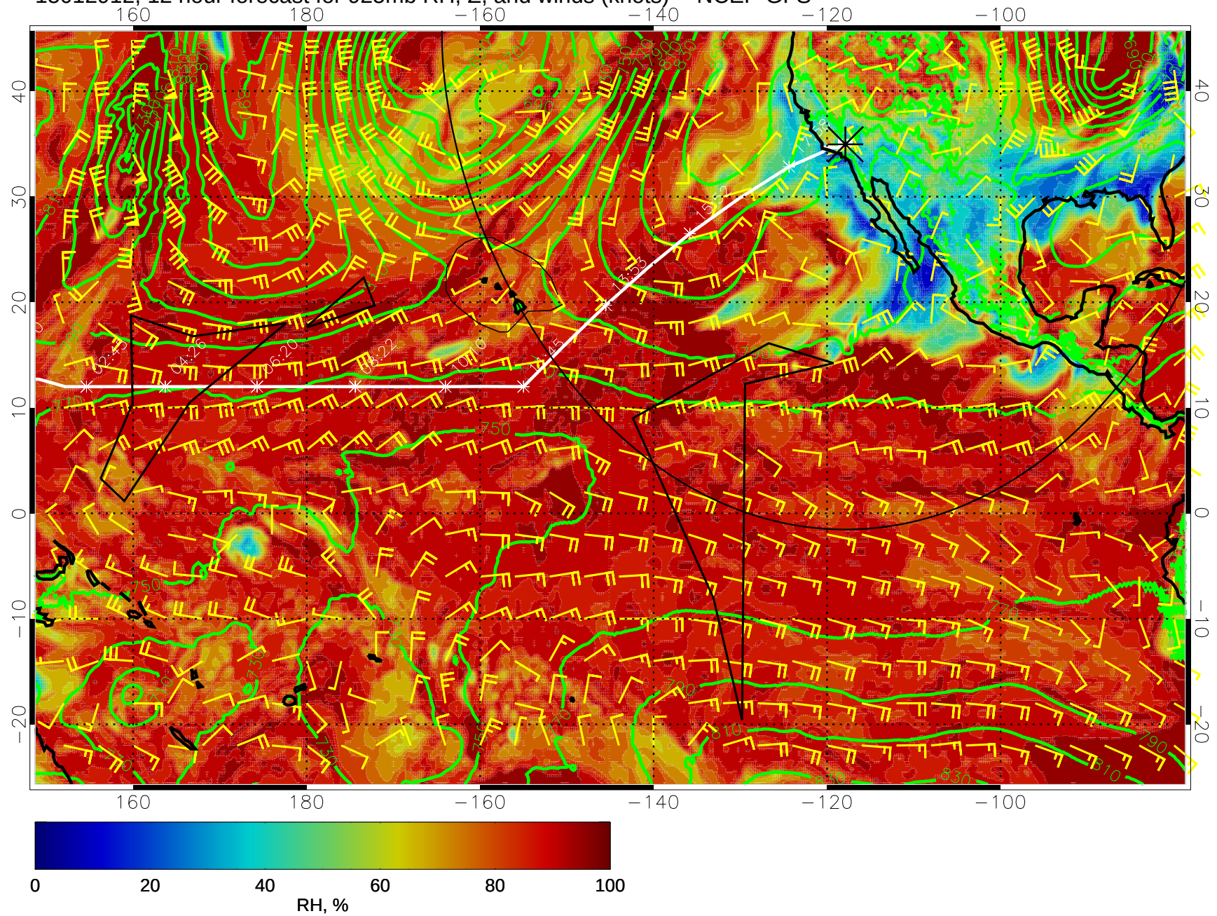
15012912, 12 hour forecast for 925mb RH, Z, and winds (knots) -- NCEP GFS
