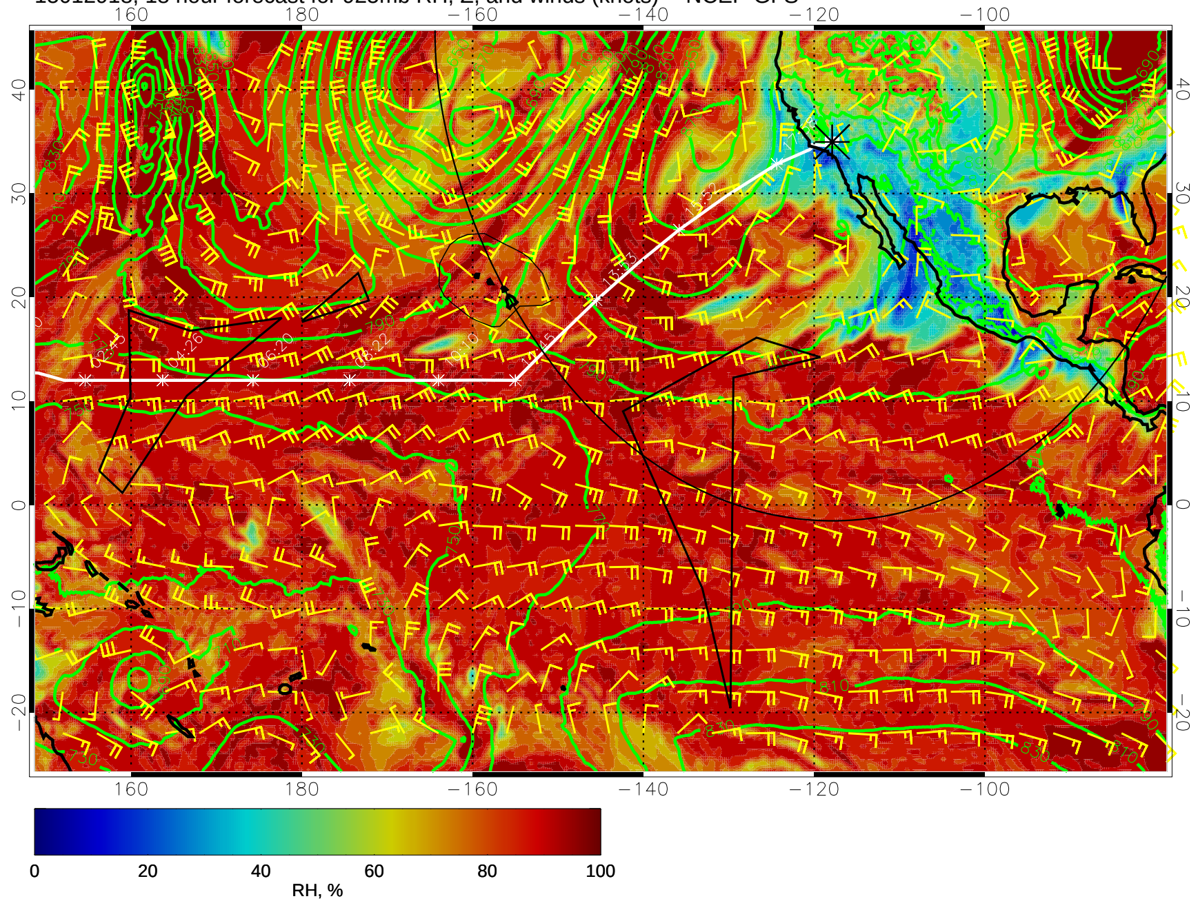
15012918, 18 hour forecast for 925mb RH, Z, and winds (knots) -- NCEP GFS
