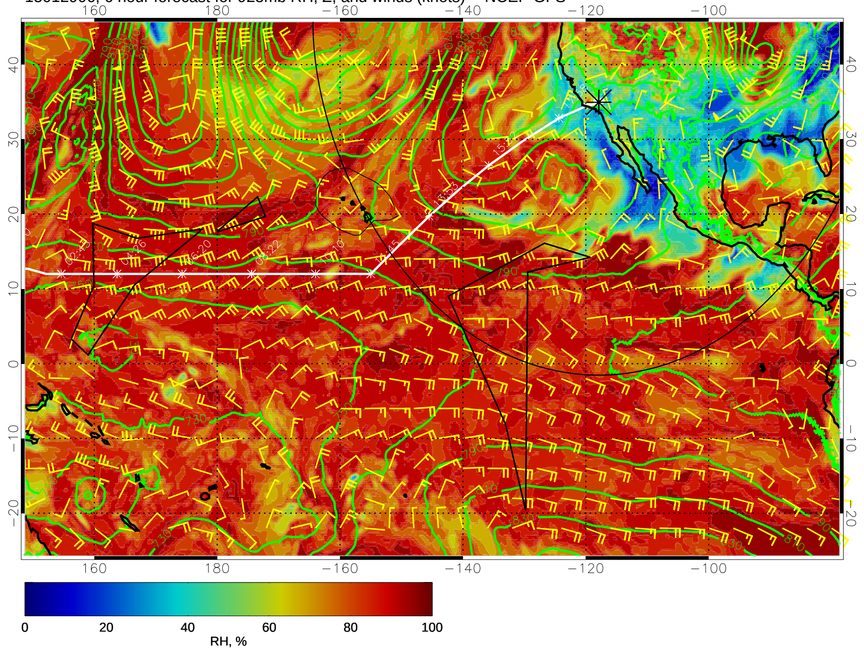
15012906, 6 hour forecast for 925mb RH, Z, and winds (knots) -- NCEP GFS
