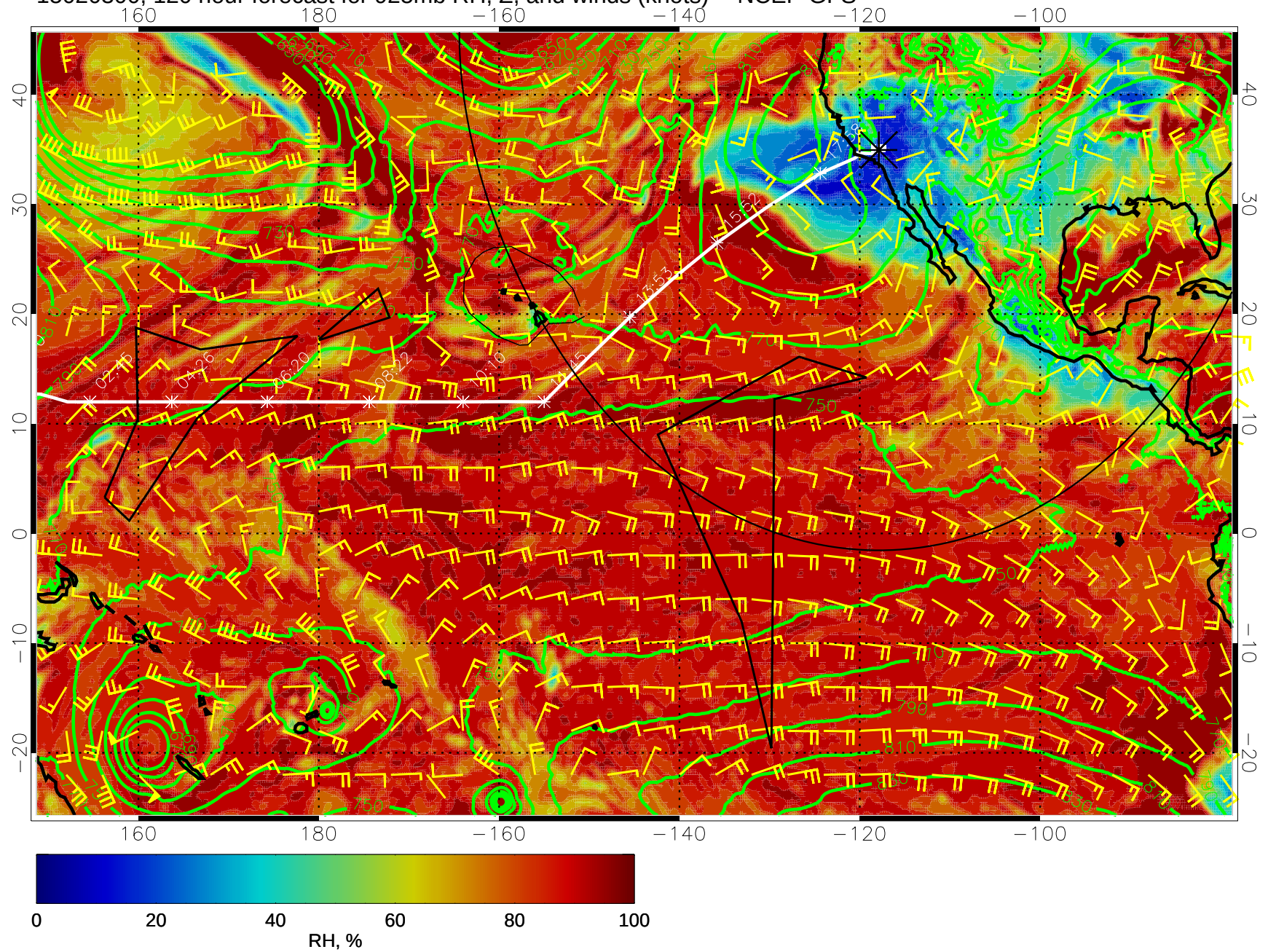
15020300, 120 hour forecast for 925mb RH, Z, and winds (knots) -- NCEP GFS
