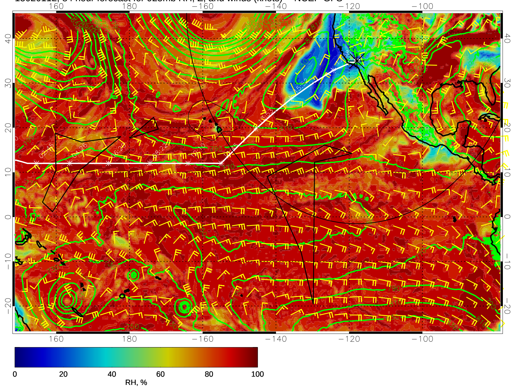
15020112, 84 hour forecast for 925mb RH, Z, and winds (knots) -- NCEP GFS
