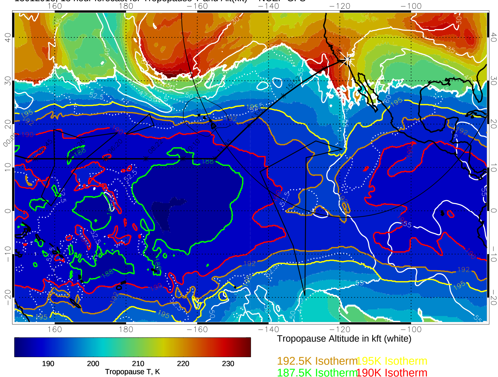
15012918, 18 hour forecast for Tropopause T and Alt(kft) -- NCEP GFS
