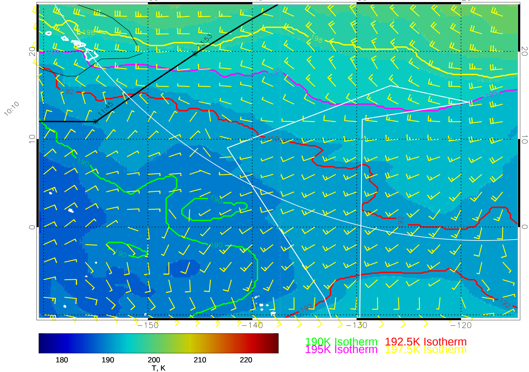
15020212, 108 hour forecast for 70mb T and winds (knots) -- NCEP GFS
