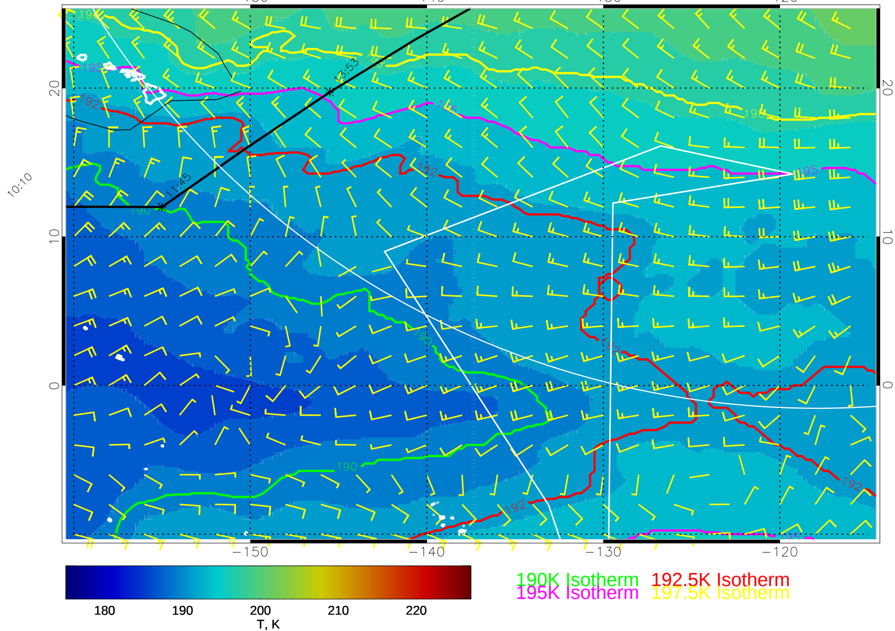
15020300, 120 hour forecast for 70mb T and winds (knots) -- NCEP GFS
