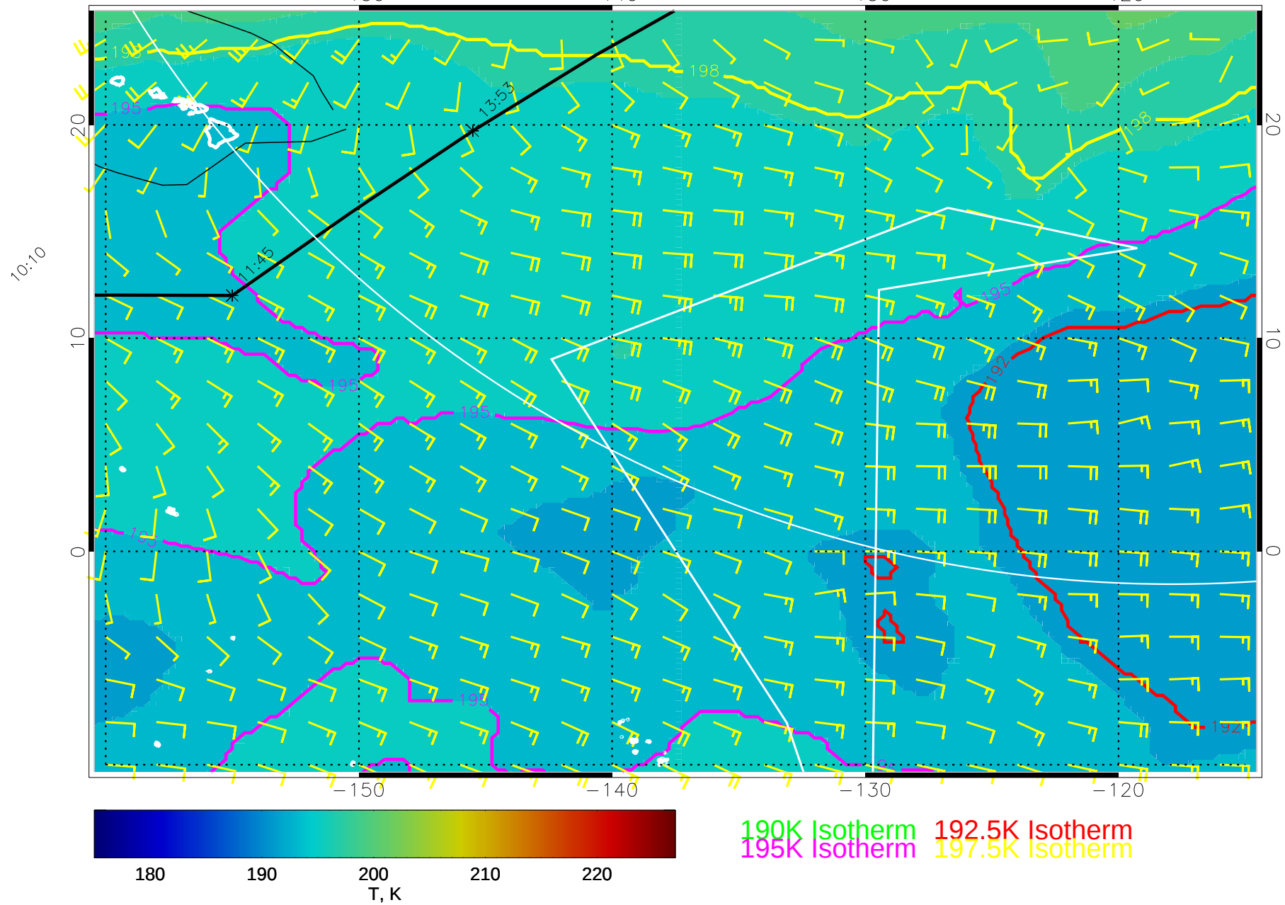
15012906, 6 hour forecast for 70mb T and winds (knots) -- NCEP GFS
