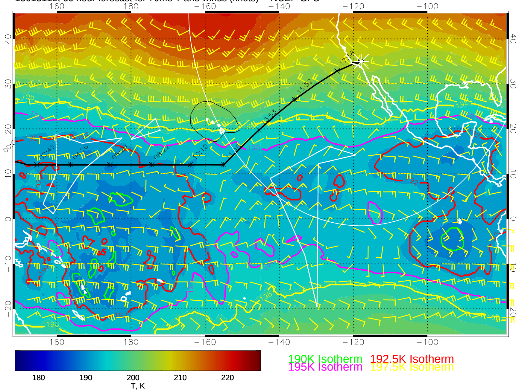
15013112, 60 hour forecast for 70mb T and winds (knots) -- NCEP GFS
