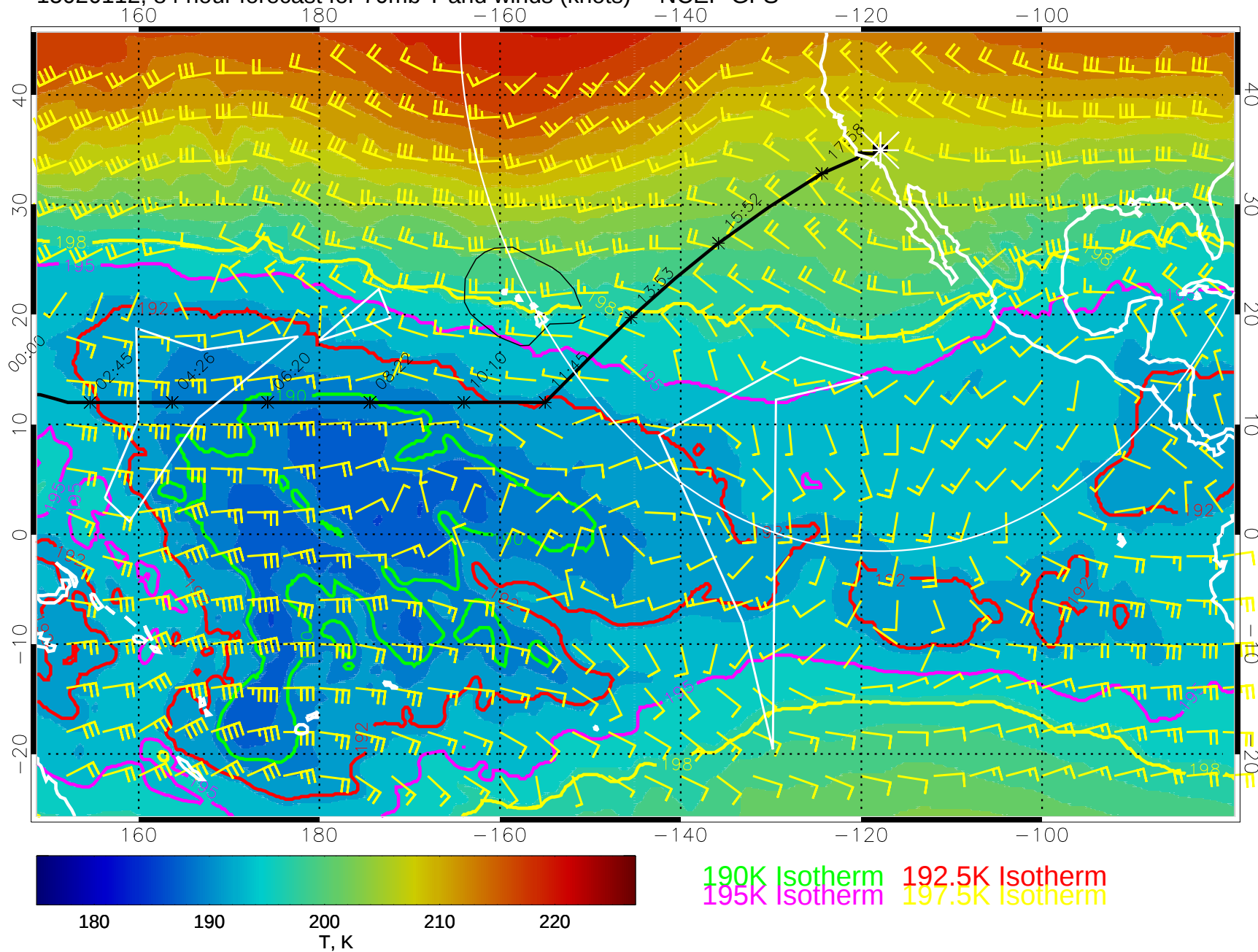
15020112, 84 hour forecast for 70mb T and winds (knots) -- NCEP GFS
