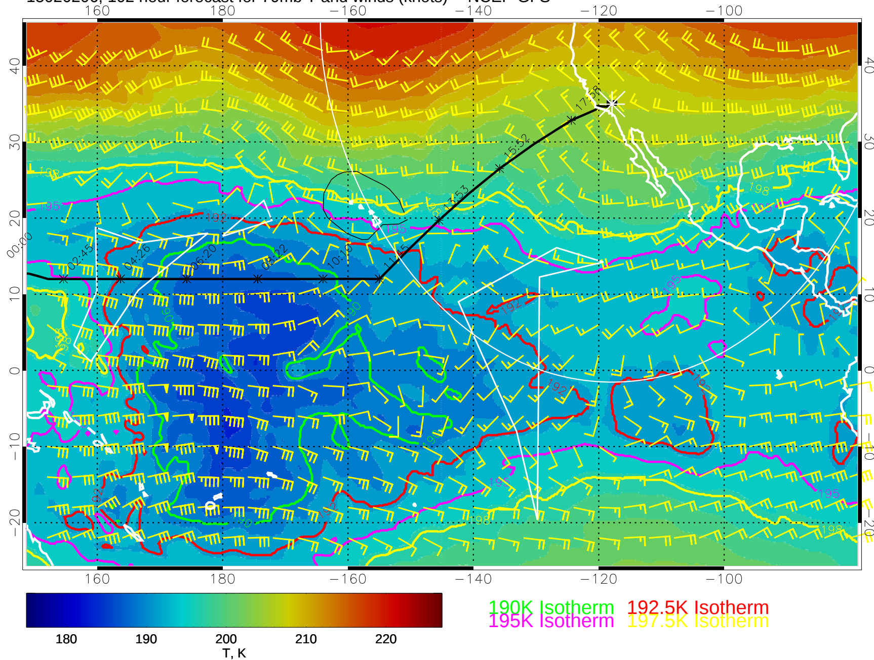
15020206, 102 hour forecast for 70mb T and winds (knots) -- NCEP GFS
