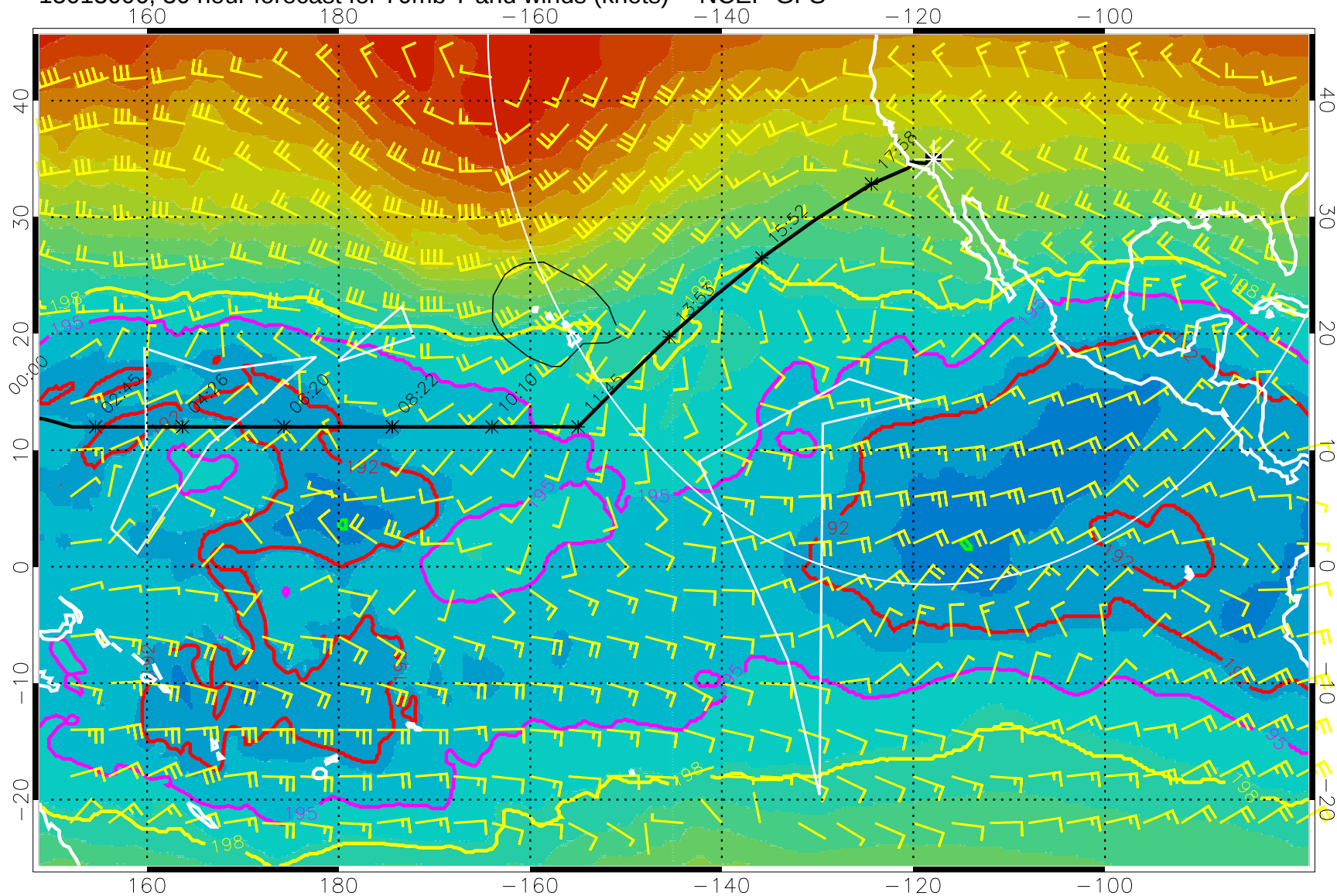
15013006, 30 hour forecast for 70mb T and winds (knots) -- NCEP GFS
