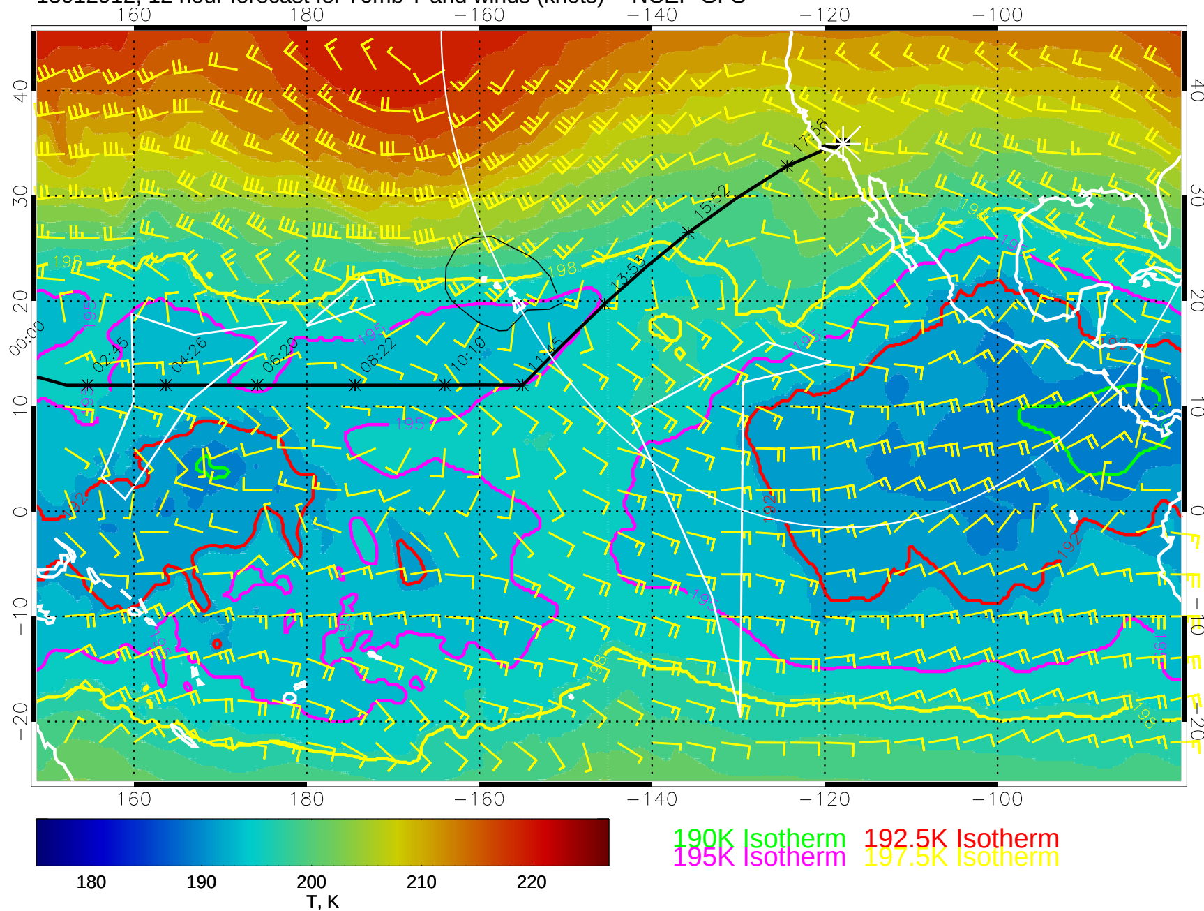
15012912, 12 hour forecast for 70mb T and winds (knots) -- NCEP GFS
