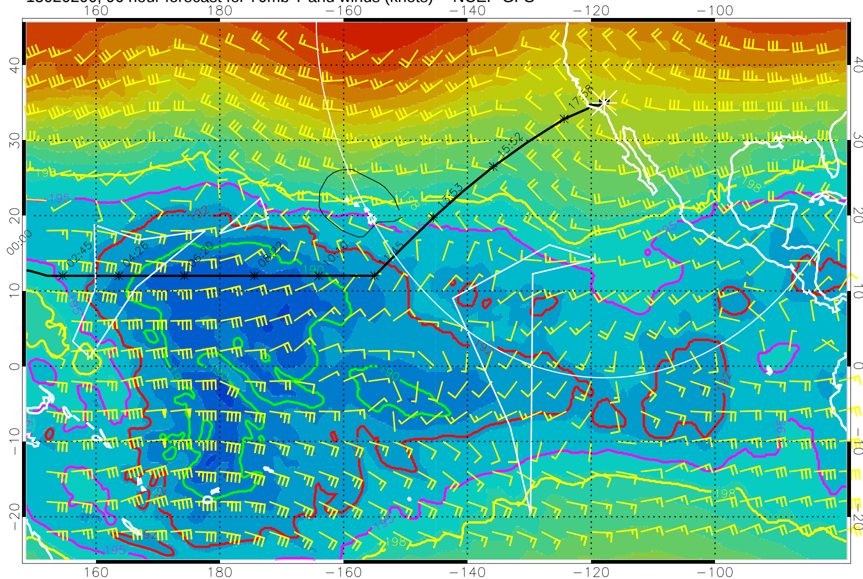
15020200, 96 hour forecast for 70mb T and winds (knots) -- NCEP GFS
