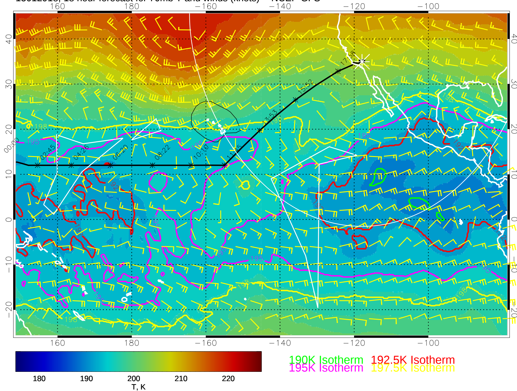
15012918, 18 hour forecast for 70mb T and winds (knots) -- NCEP GFS
