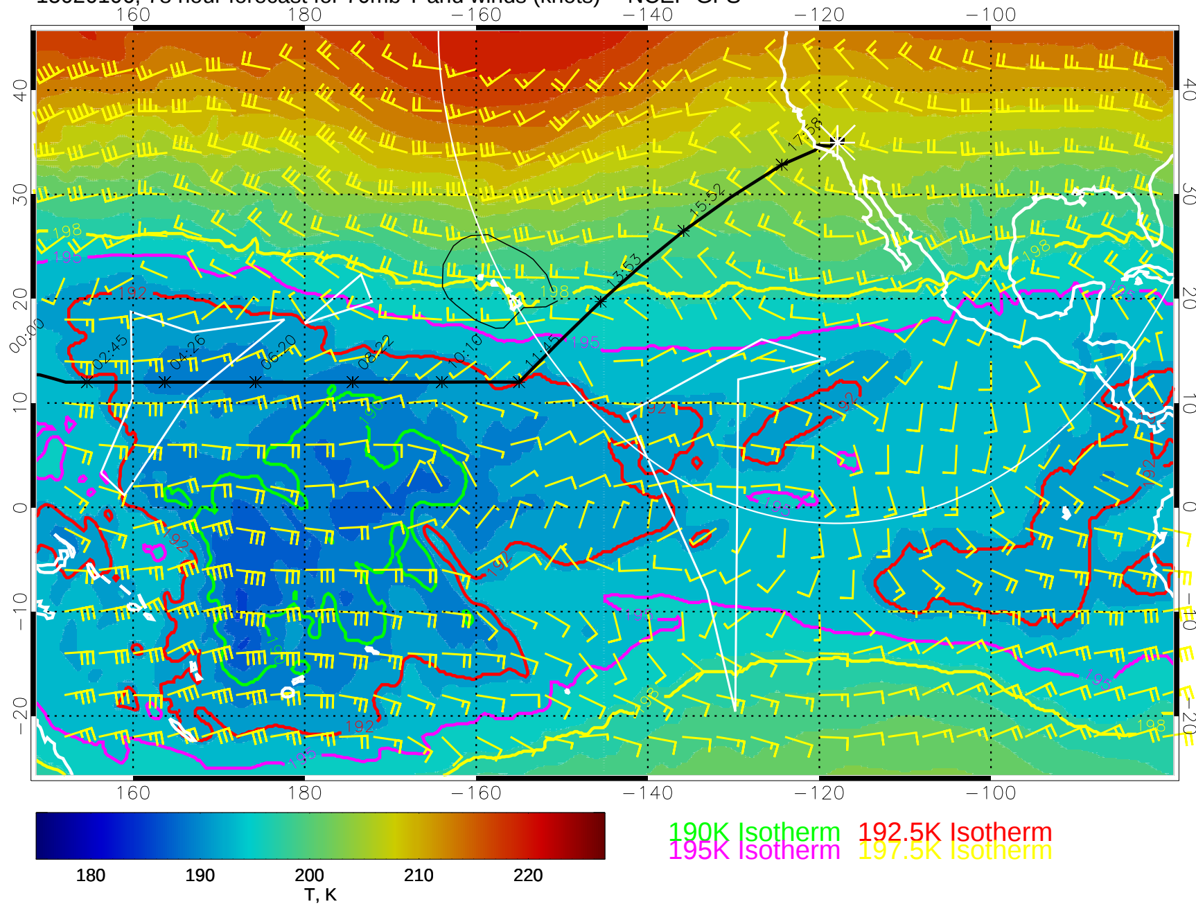
15020106, 78 hour forecast for 70mb T and winds (knots) -- NCEP GFS
