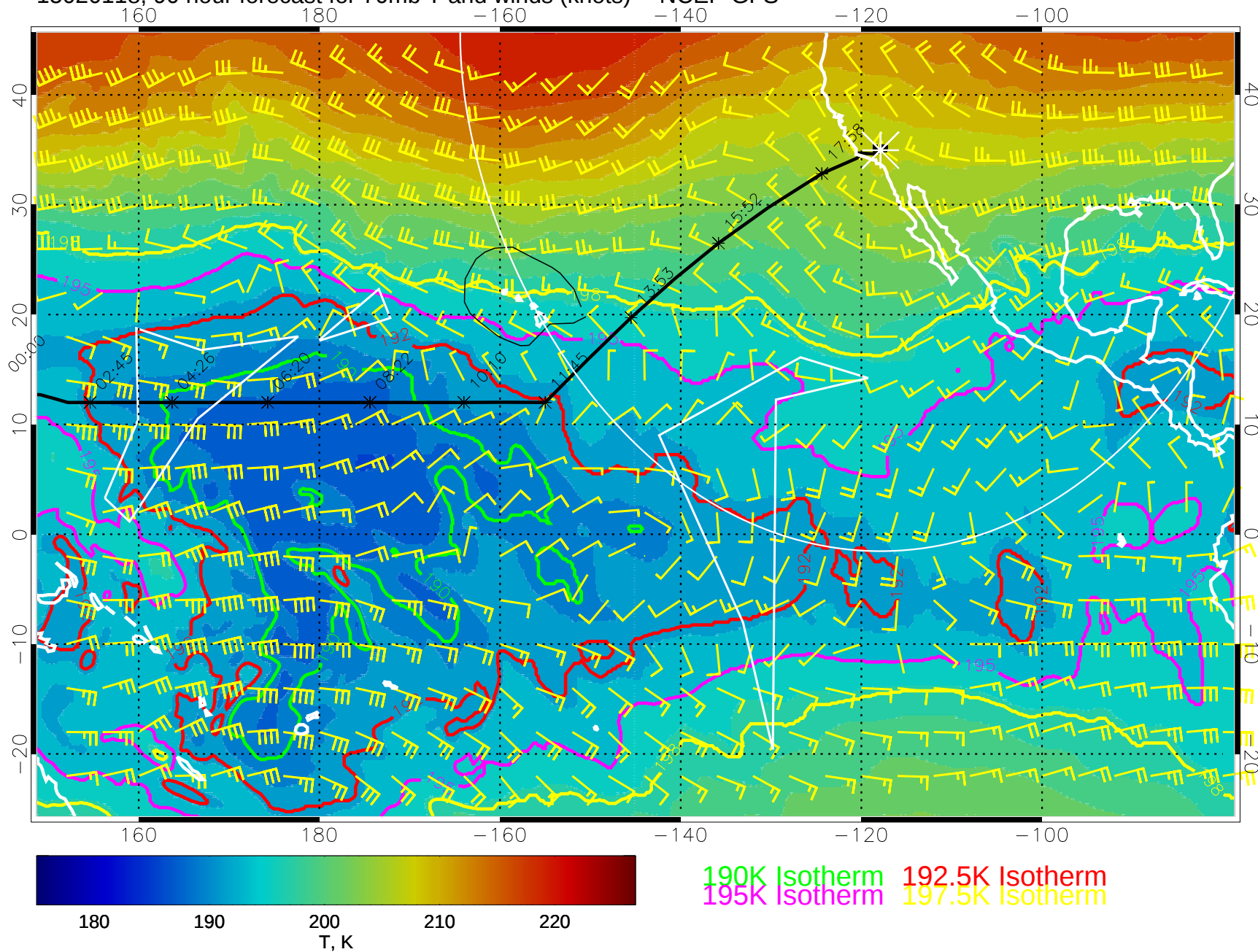
15020118, 90 hour forecast for 70mb T and winds (knots) -- NCEP GFS
