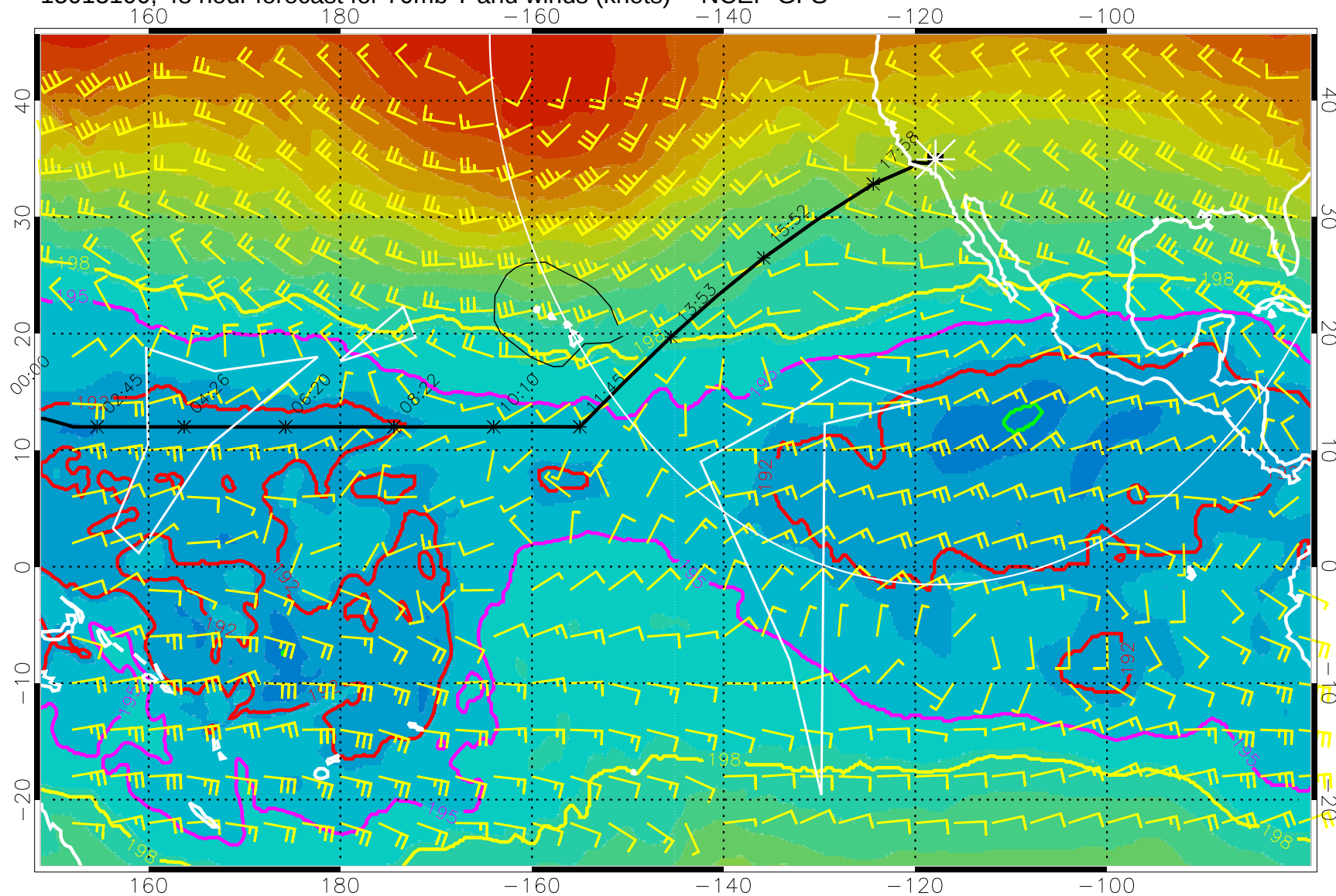
15013100, 48 hour forecast for 70mb T and winds (knots) -- NCEP GFS
