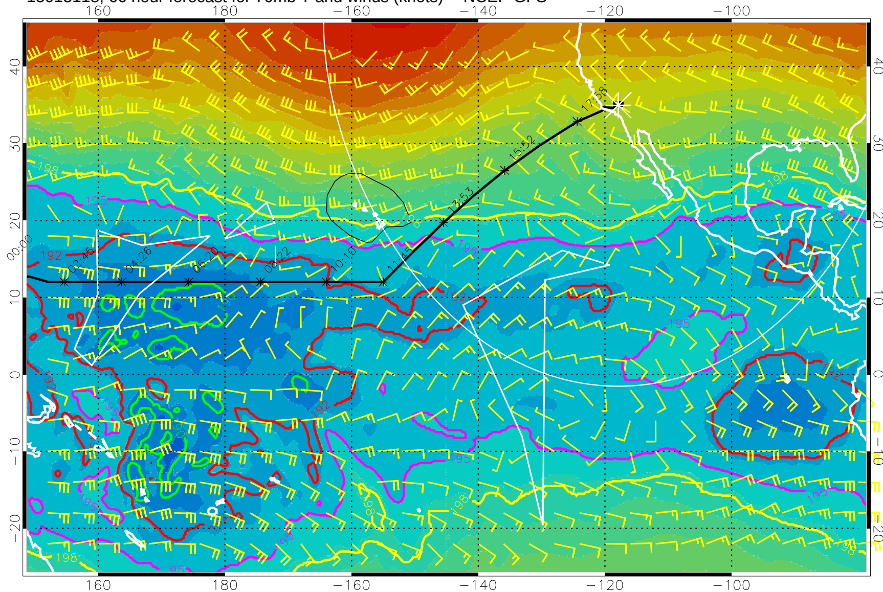
15013118, 66 hour forecast for 70mb T and winds (knots) -- NCEP GFS
