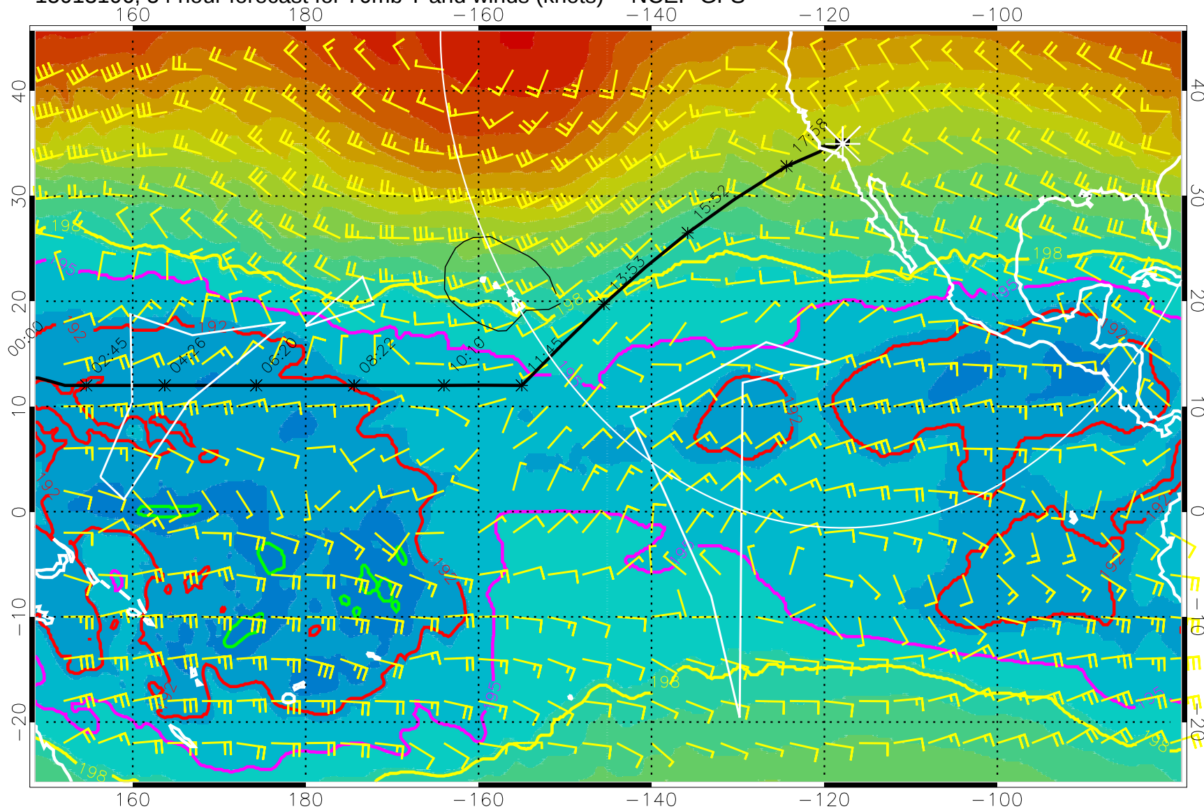
15013106, 54 hour forecast for 70mb T and winds (knots) -- NCEP GFS
