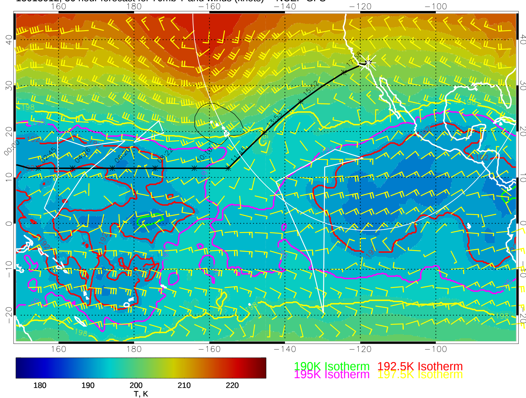
15013012, 36 hour forecast for 70mb T and winds (knots) -- NCEP GFS
