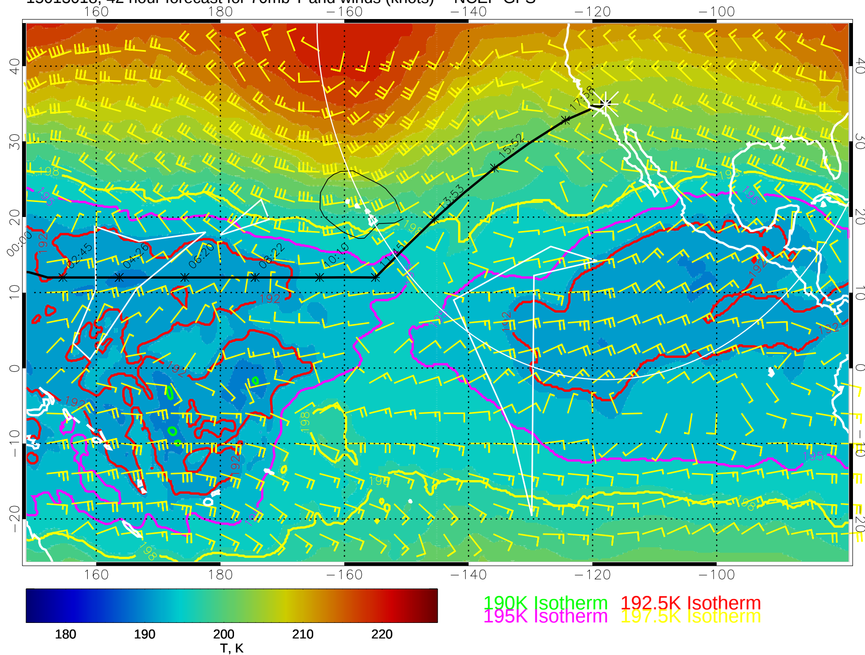
15013018, 42 hour forecast for 70mb T and winds (knots) -- NCEP GFS
