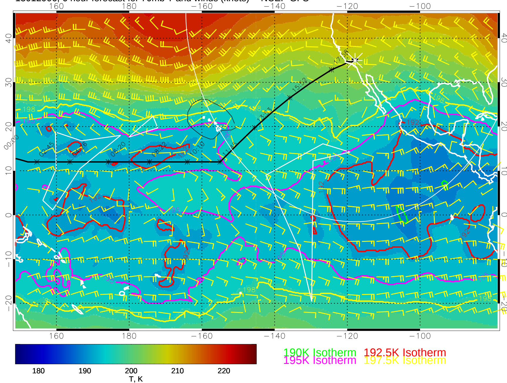
15012906, 6 hour forecast for 70mb T and winds (knots) -- NCEP GFS
