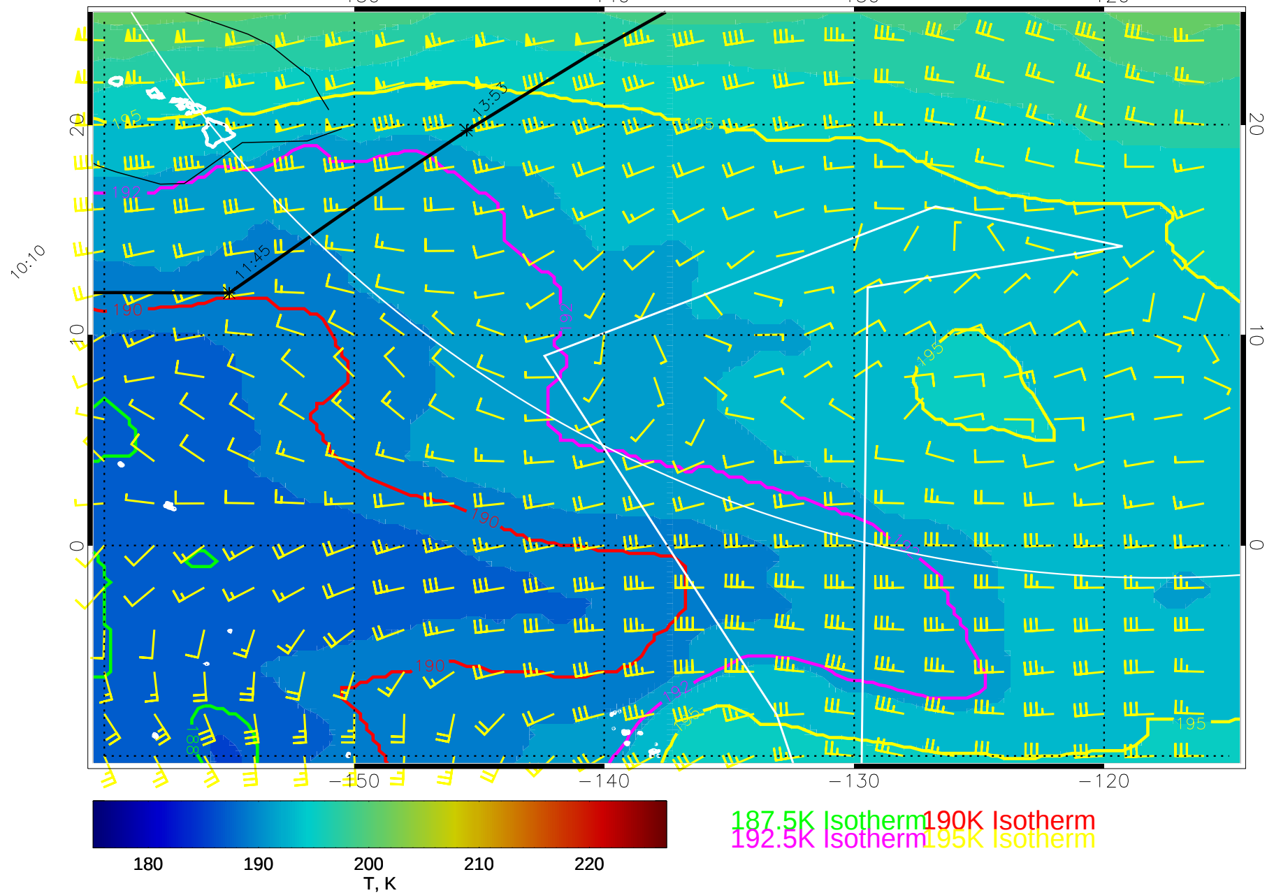
15013106, 54 hour forecast for 100mb T and winds (knots) -- NCEP GFS
