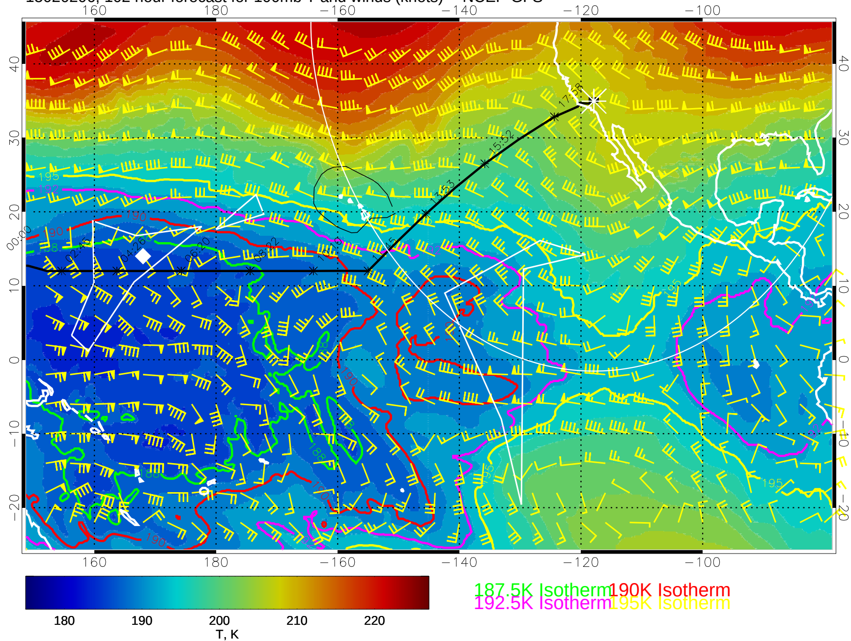
15020206, 102 hour forecast for 100mb T and winds (knots) -- NCEP GFS
