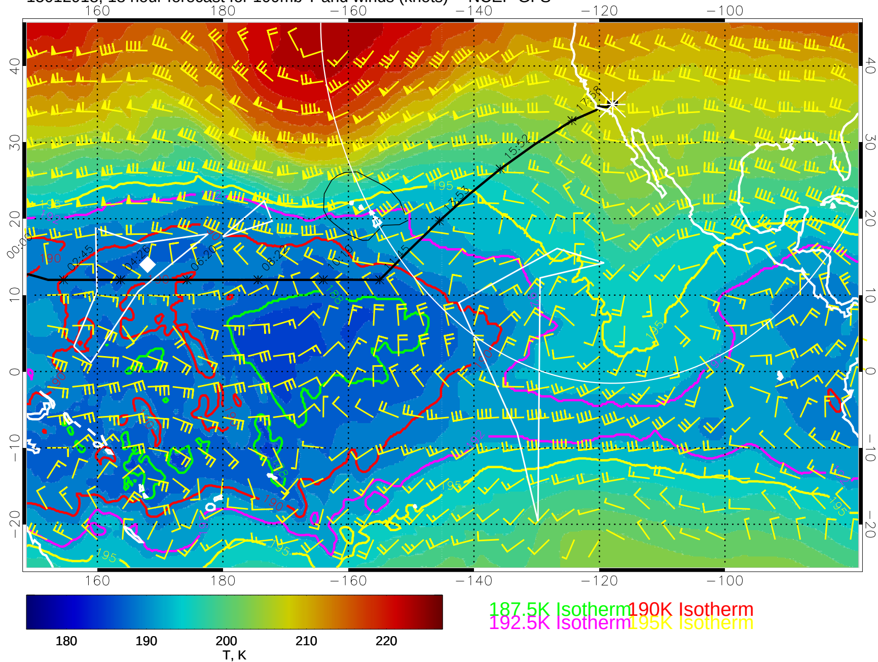
15012918, 18 hour forecast for 100mb T and winds (knots) -- NCEP GFS
