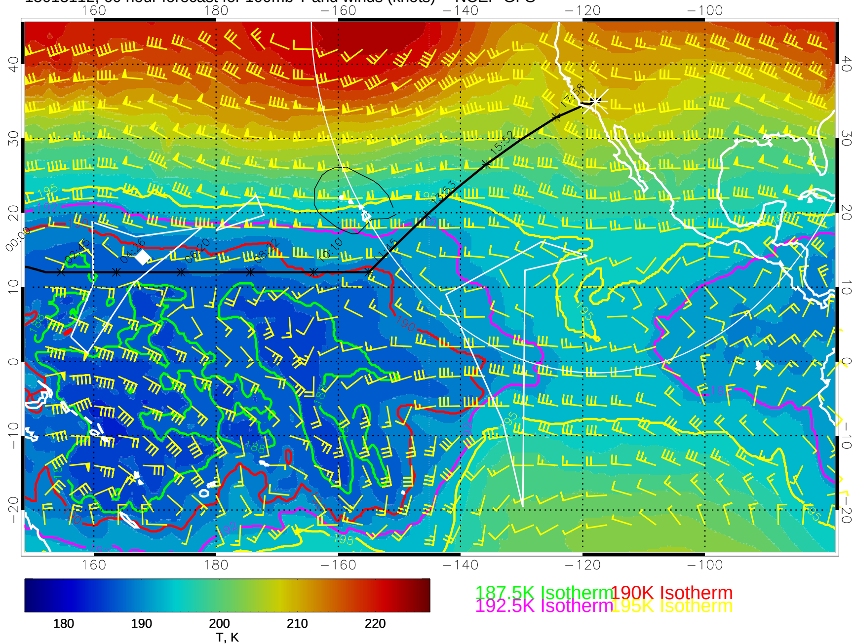
15013112, 60 hour forecast for 100mb T and winds (knots) -- NCEP GFS
