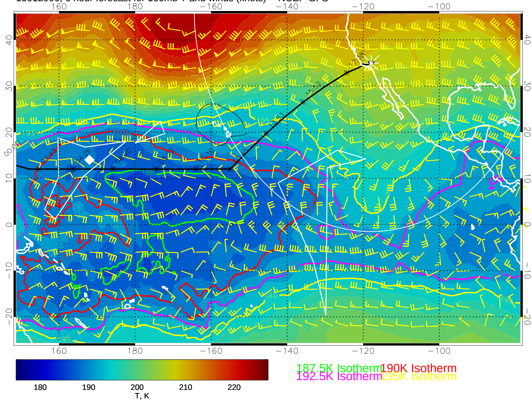
15012906, 6 hour forecast for 100mb T and winds (knots) -- NCEP GFS
