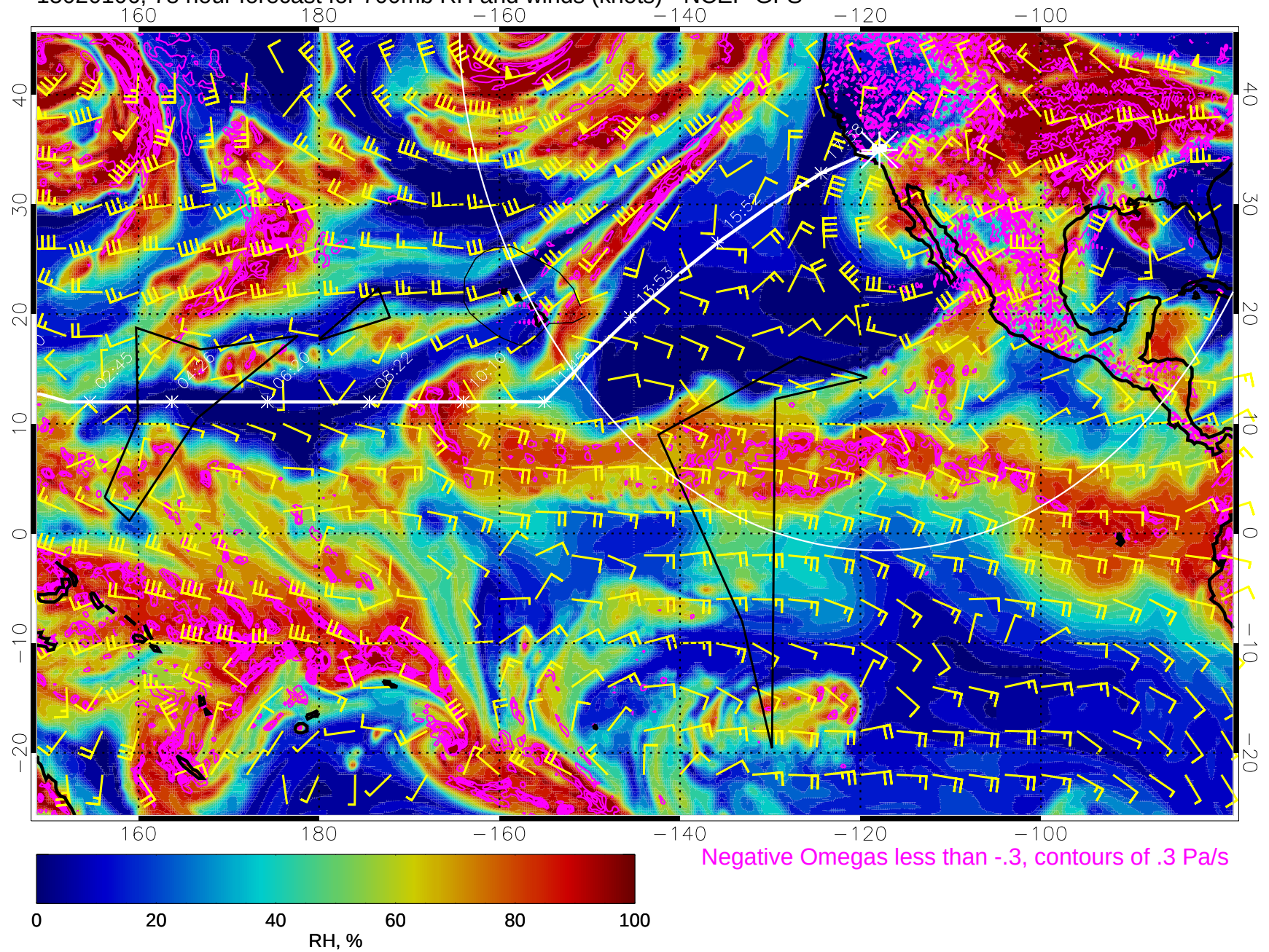
15020106, 78 hour forecast for 700mb RH and winds (knots) - NCEP GFS
