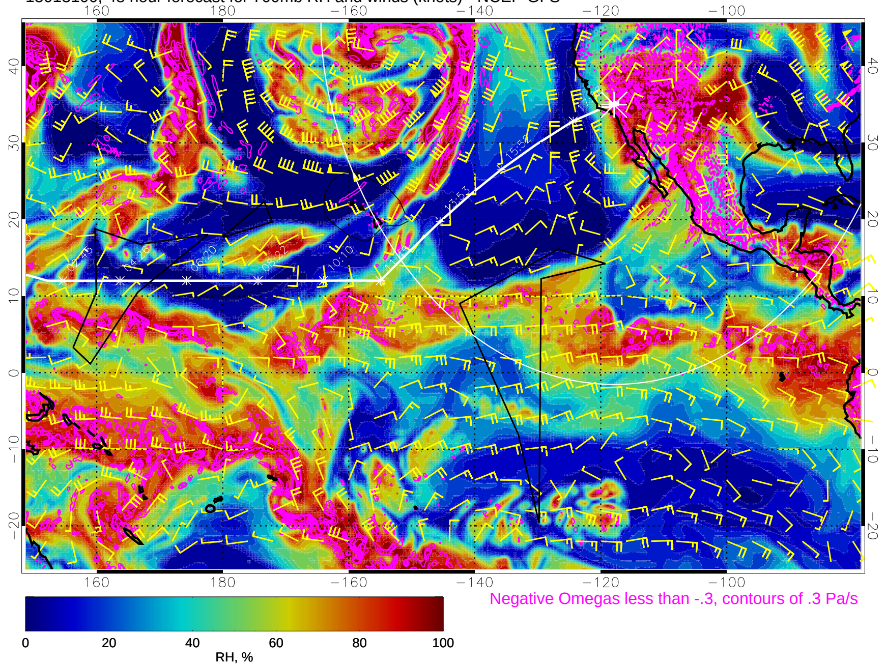
15013100, 48 hour forecast for 700mb RH and winds (knots) - NCEP GFS
