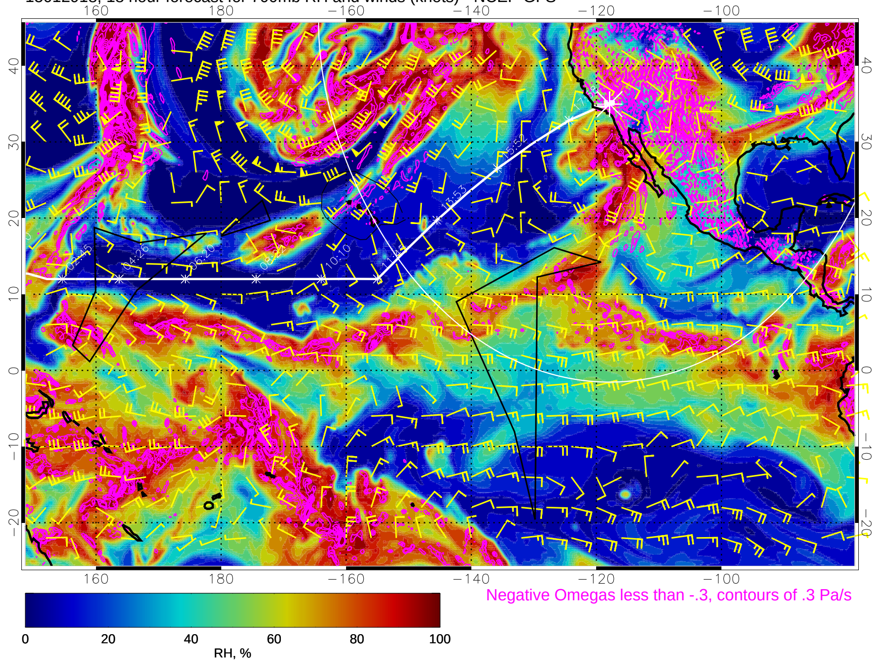
15012918, 18 hour forecast for 700mb RH and winds (knots) - NCEP GFS
