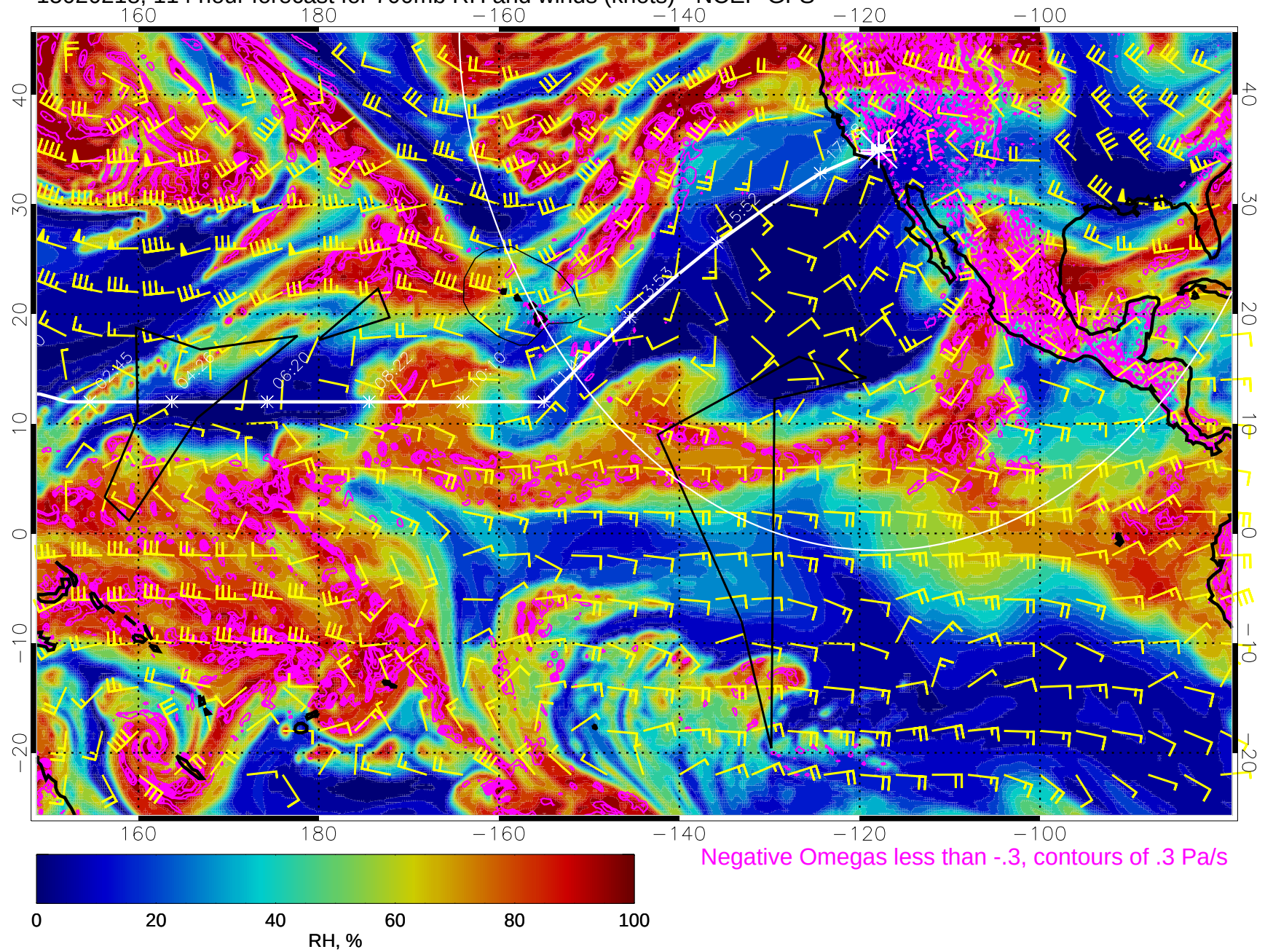
15020218, 114 hour forecast for 700mb RH and winds (knots) - NCEP GFS
