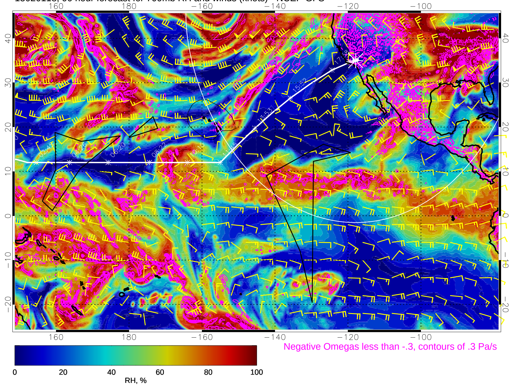
15020118, 90 hour forecast for 700mb RH and winds (knots) - NCEP GFS
