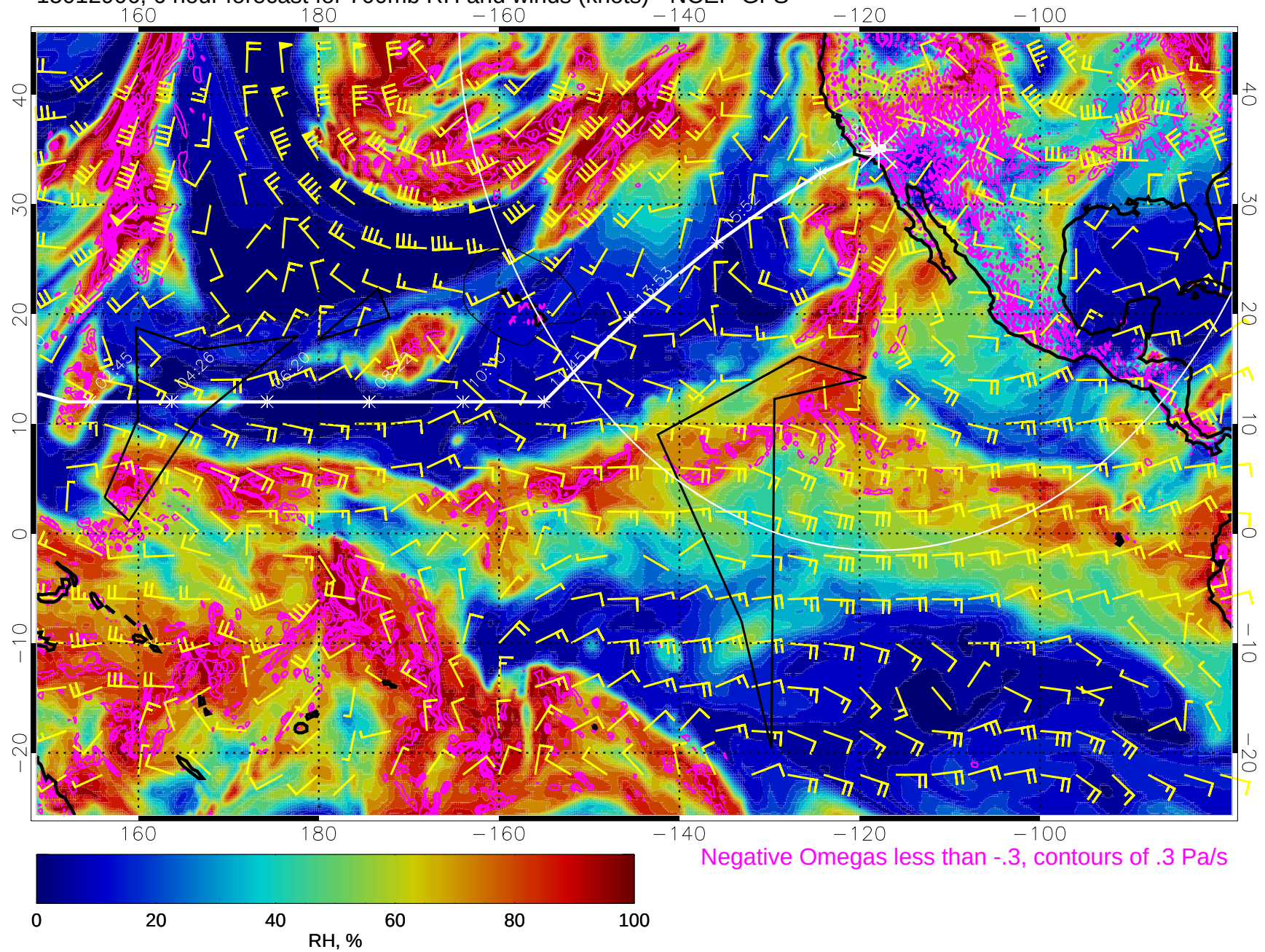
15012906, 6 hour forecast for 700mb RH and winds (knots) - NCEP GFS
