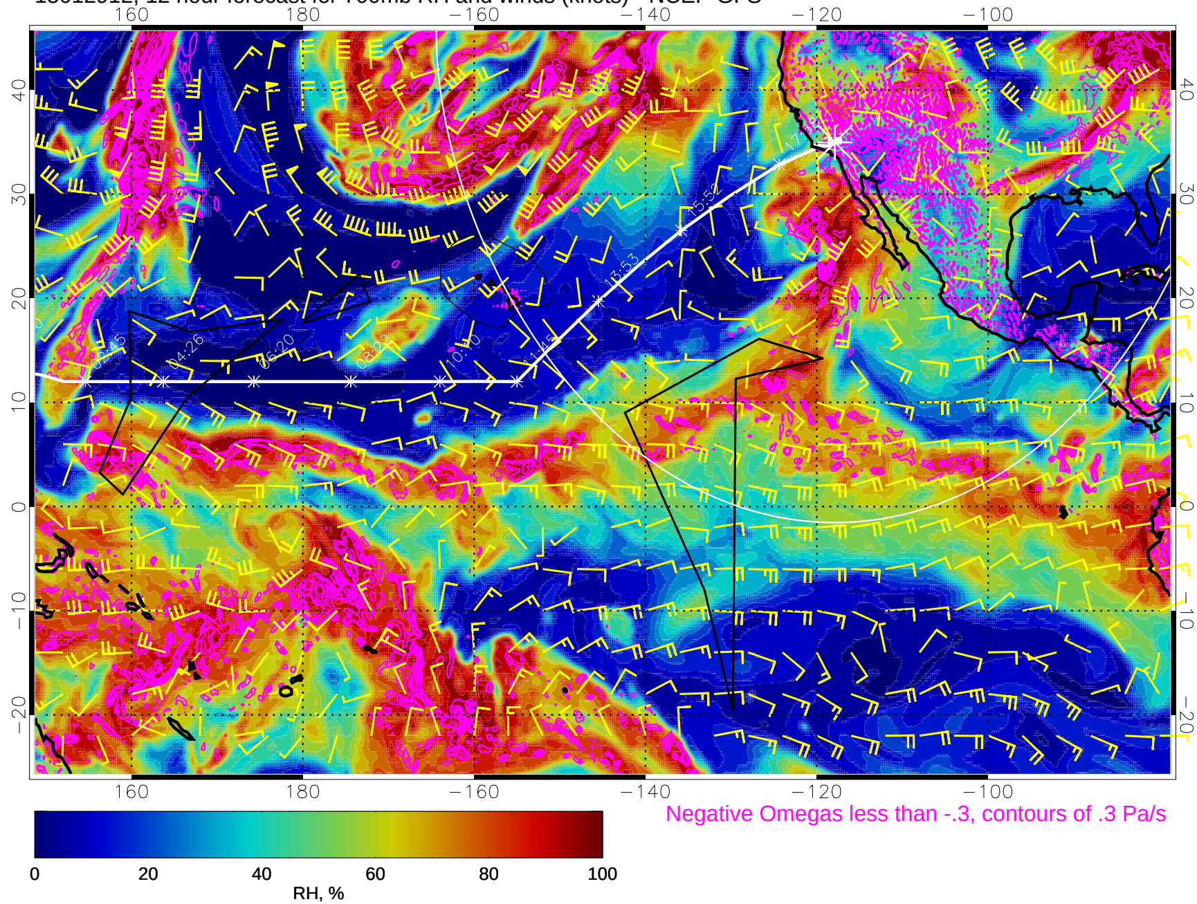
15012912, 12 hour forecast for 700mb RH and winds (knots) - NCEP GFS
