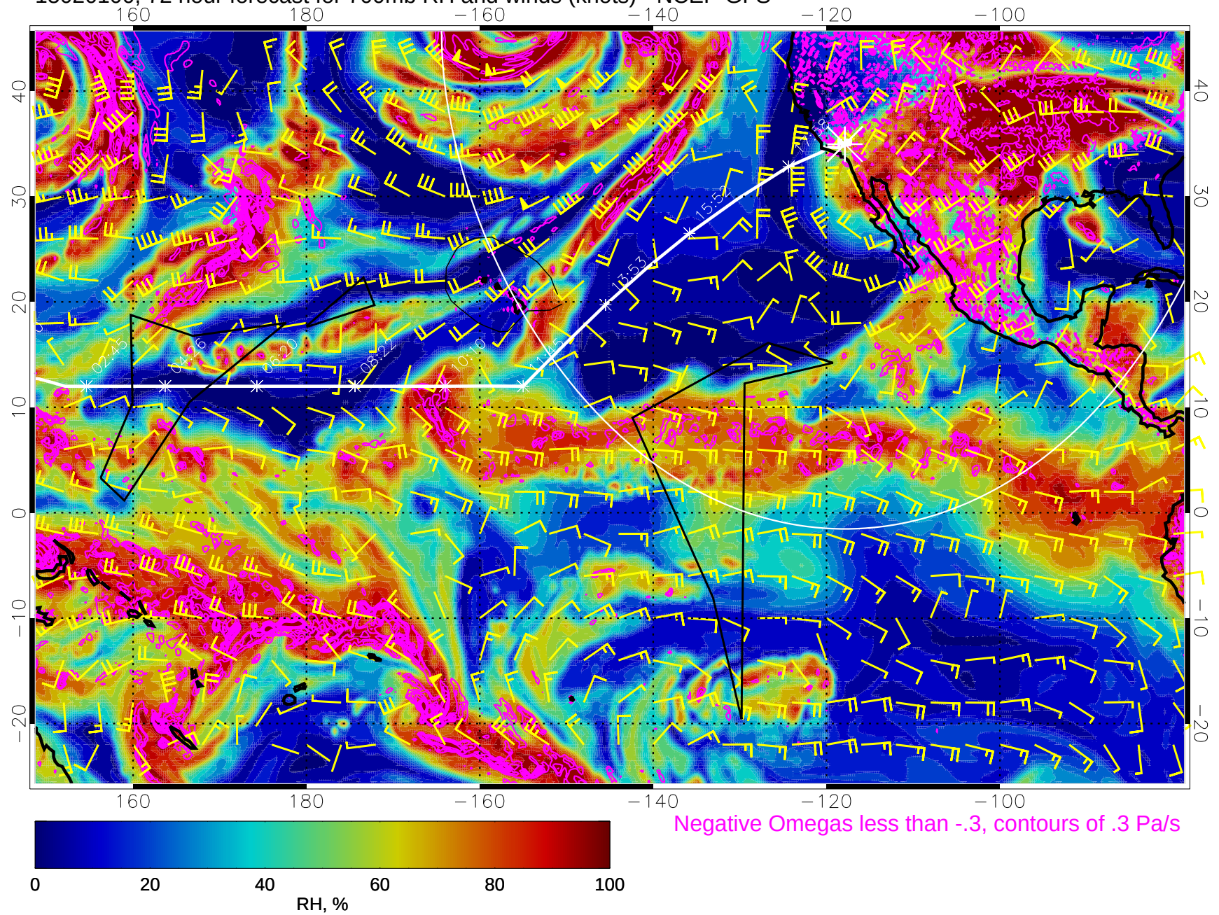
15020100, 72 hour forecast for 700mb RH and winds (knots) - NCEP GFS
