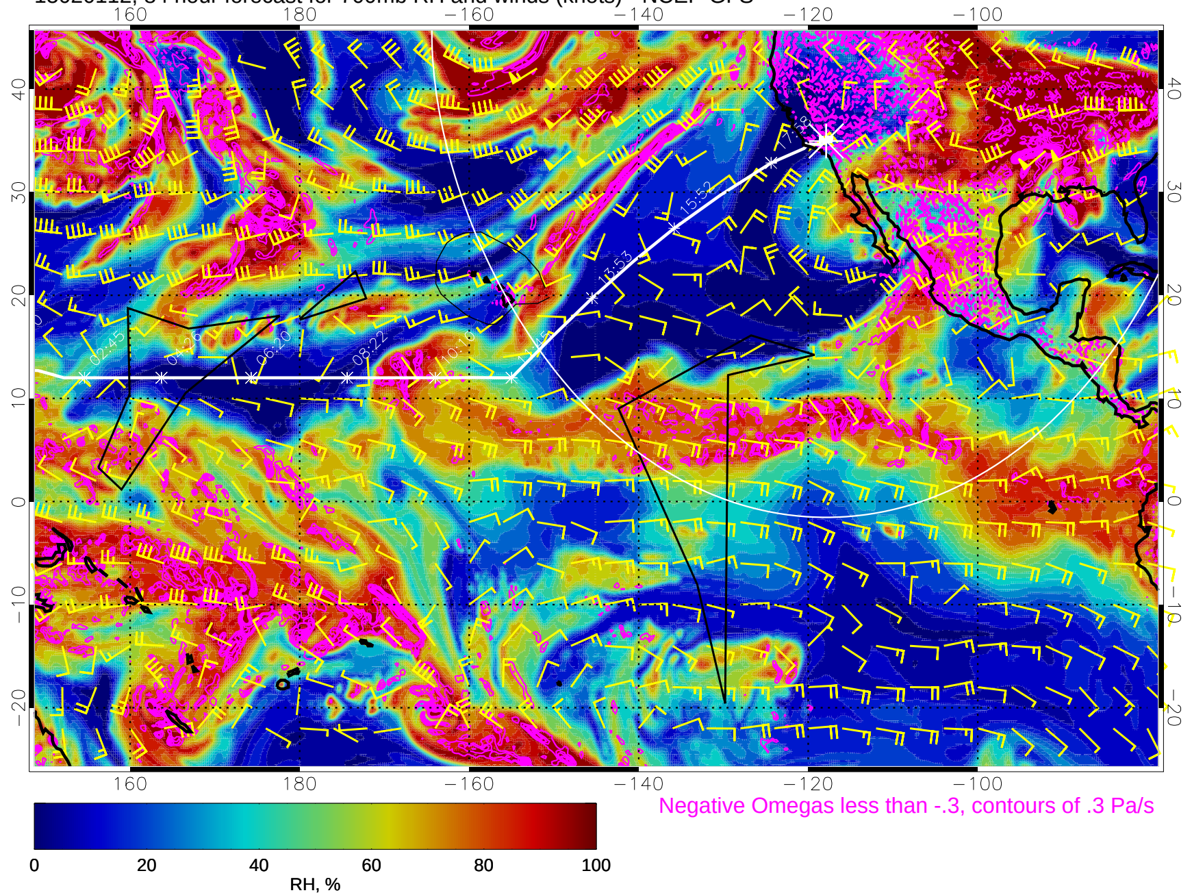
15020112, 84 hour forecast for 700mb RH and winds (knots) - NCEP GFS
