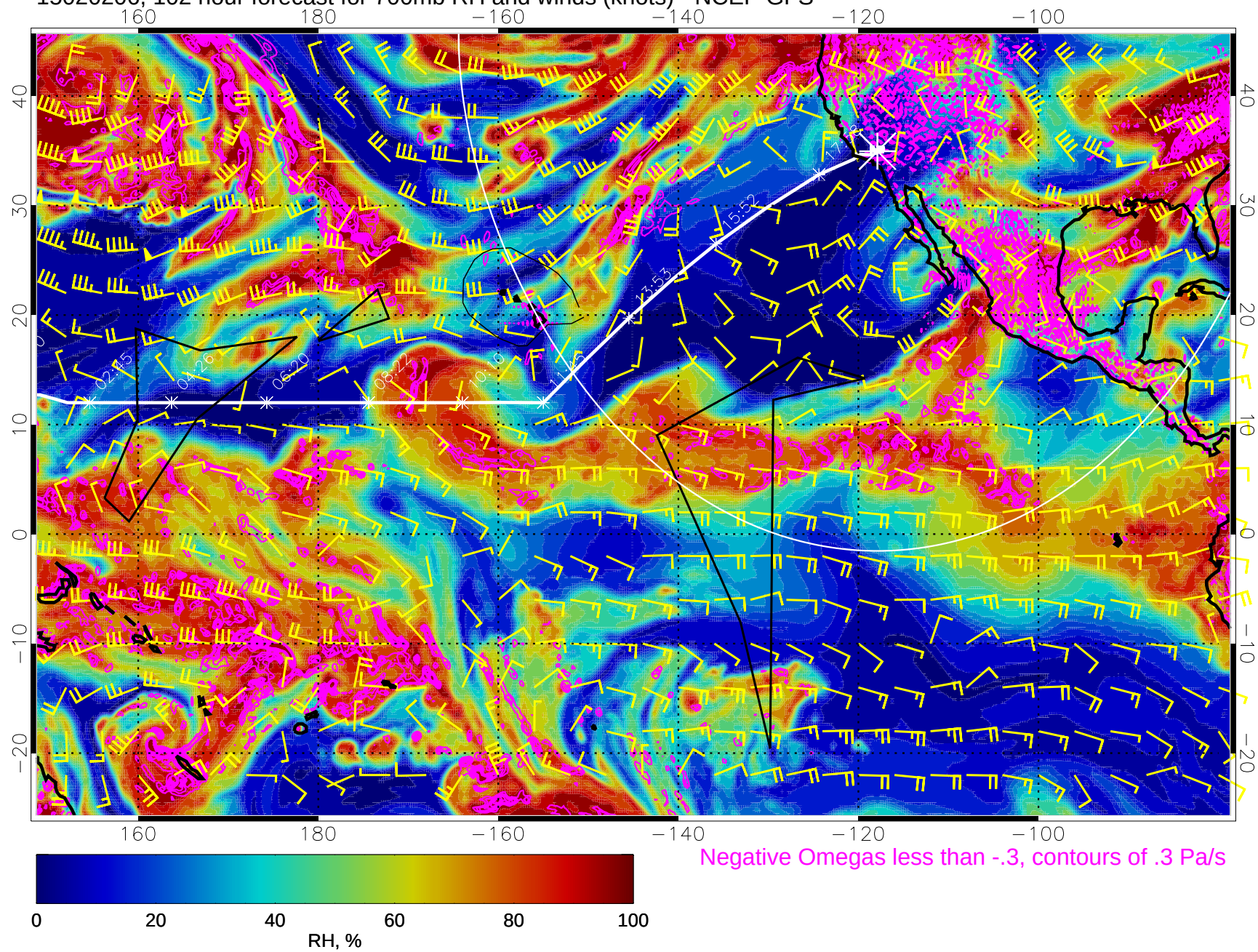
15020206, 102 hour forecast for 700mb RH and winds (knots) - NCEP GFS
