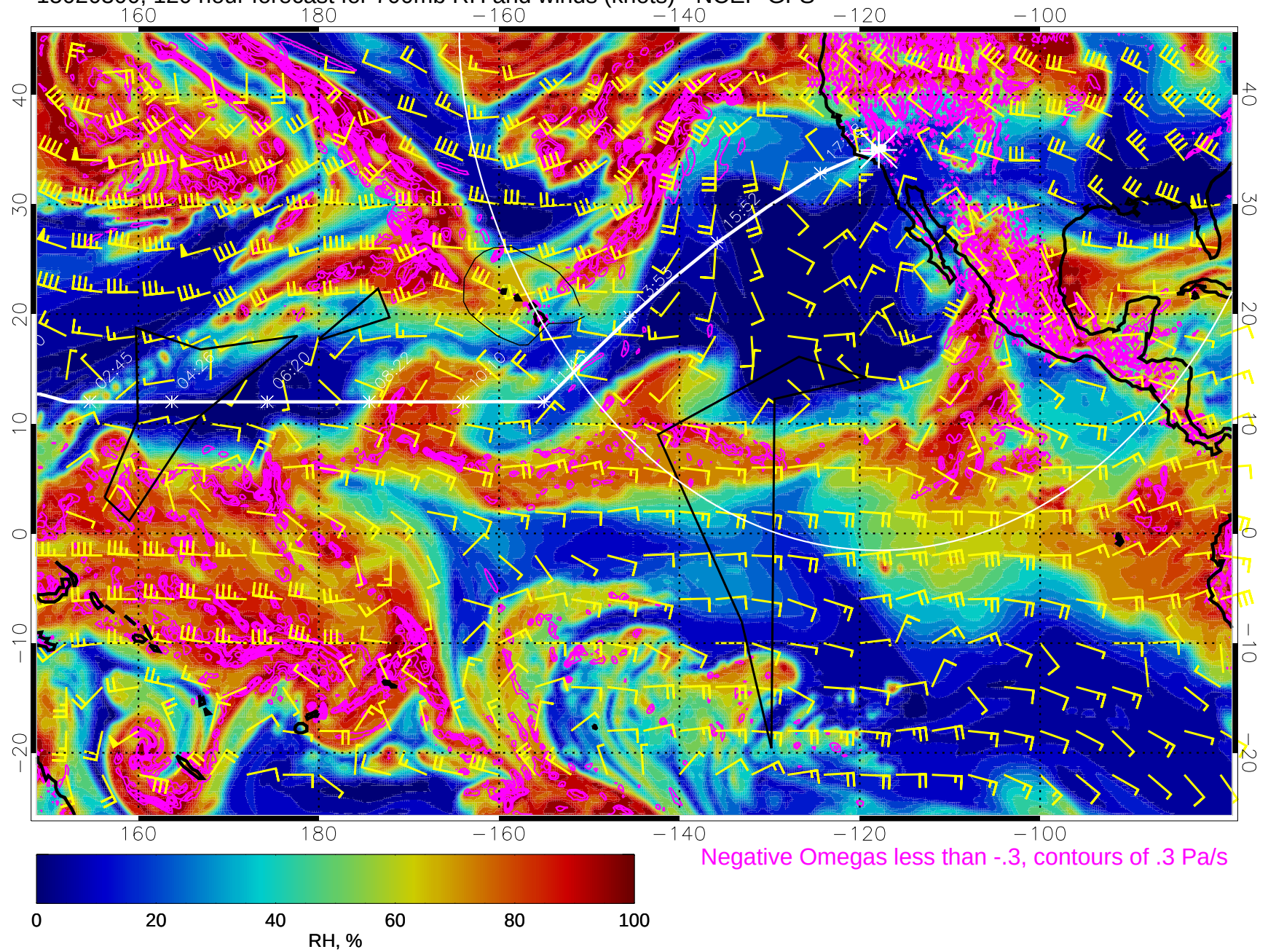
15020300, 120 hour forecast for 700mb RH and winds (knots) - NCEP GFS
