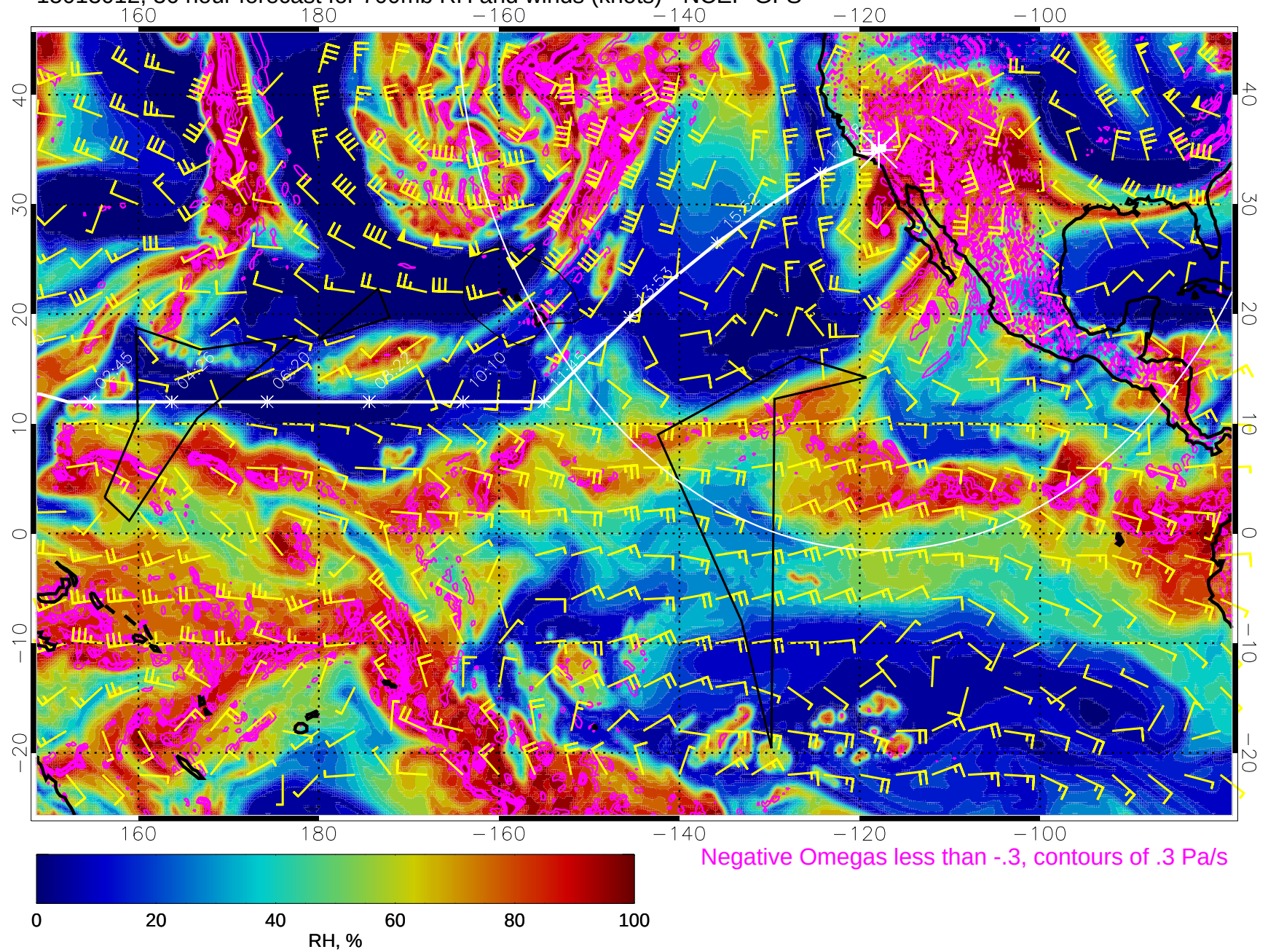
15013012, 36 hour forecast for 700mb RH and winds (knots) - NCEP GFS
