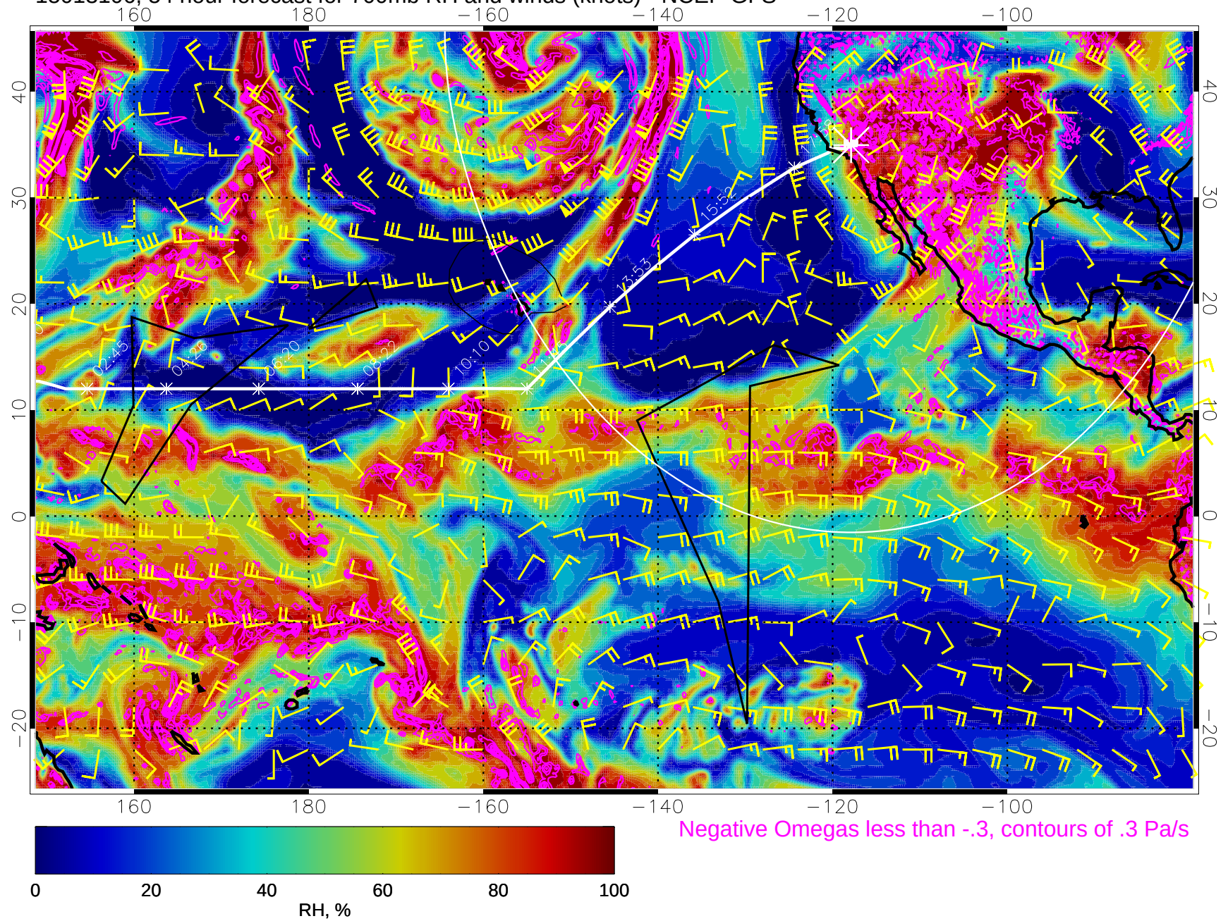
15013106, 54 hour forecast for 700mb RH and winds (knots) - NCEP GFS
