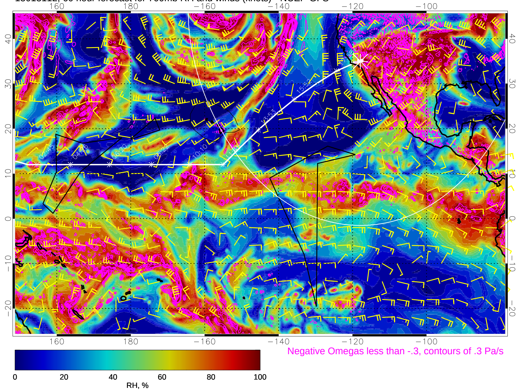
15013112, 60 hour forecast for 700mb RH and winds (knots) - NCEP GFS
