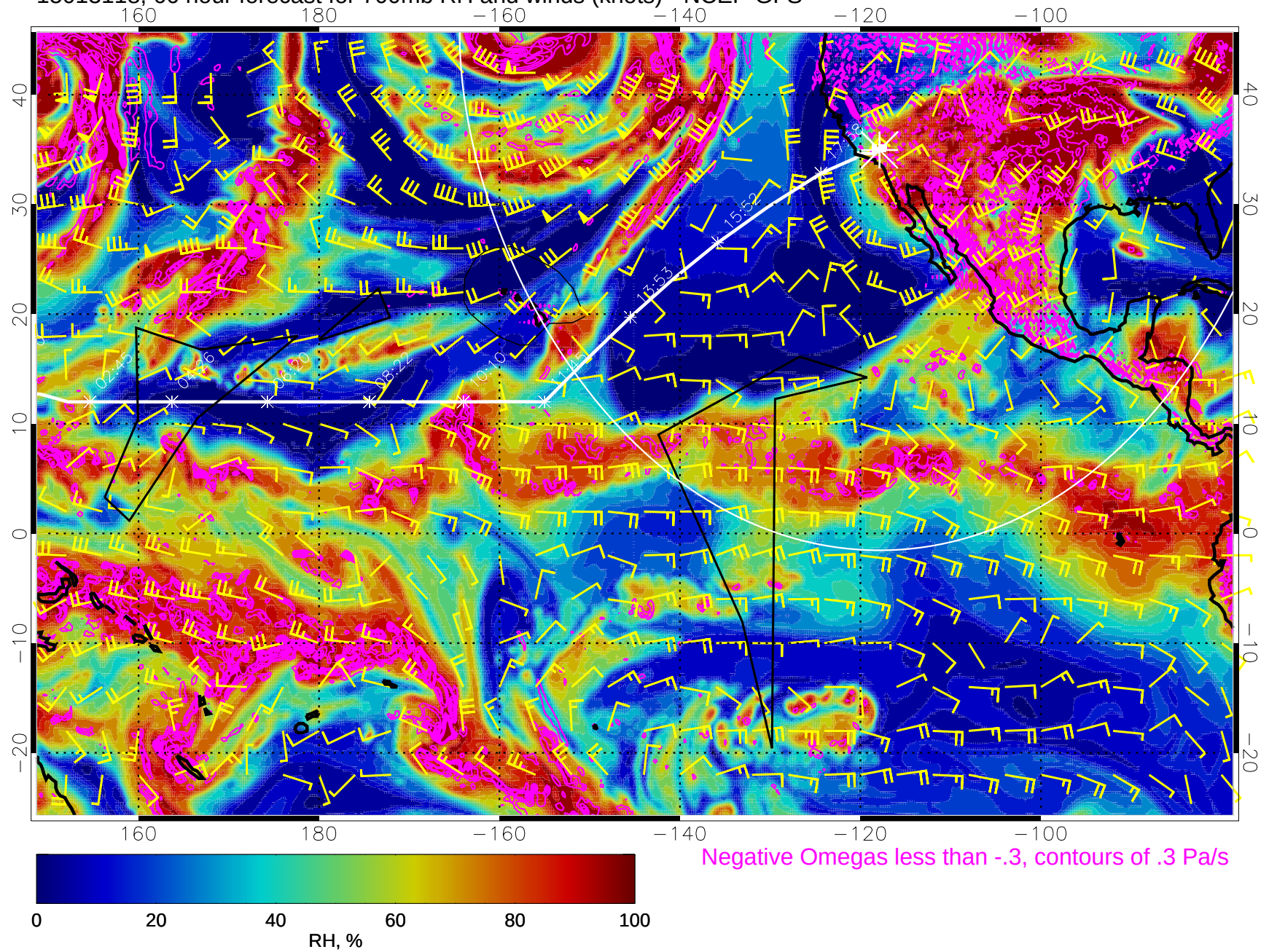
15013118, 66 hour forecast for 700mb RH and winds (knots) - NCEP GFS
