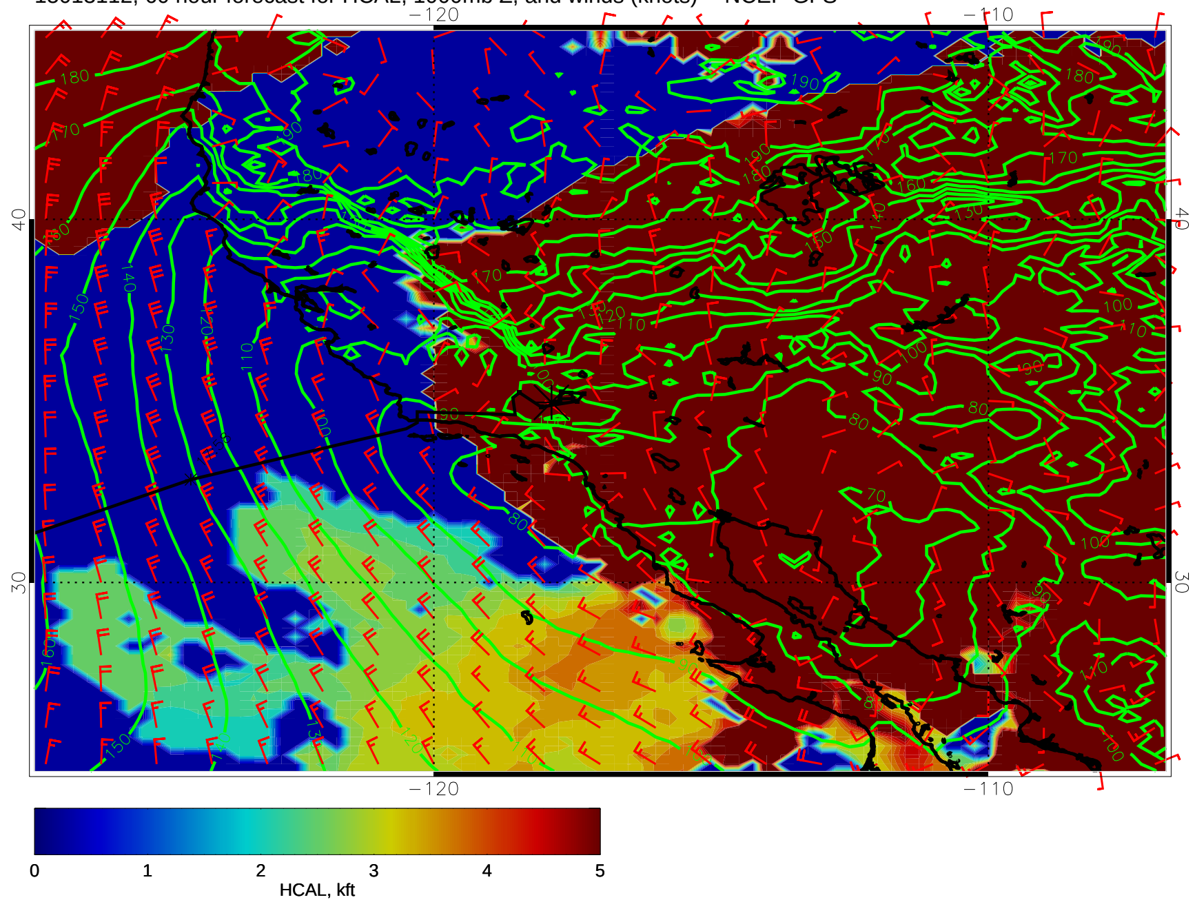
15013112, 60 hour forecast for HCAL, 1000mb Z, and winds (knots) -- NCEP GFS
