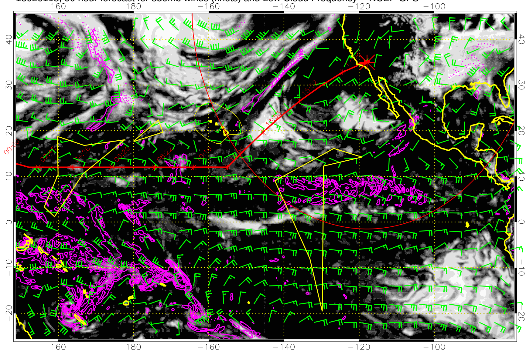
15020118, 90 hour forecast for 850mb winds (knots) and Low Cloud Frequency -- NCEP GFS
