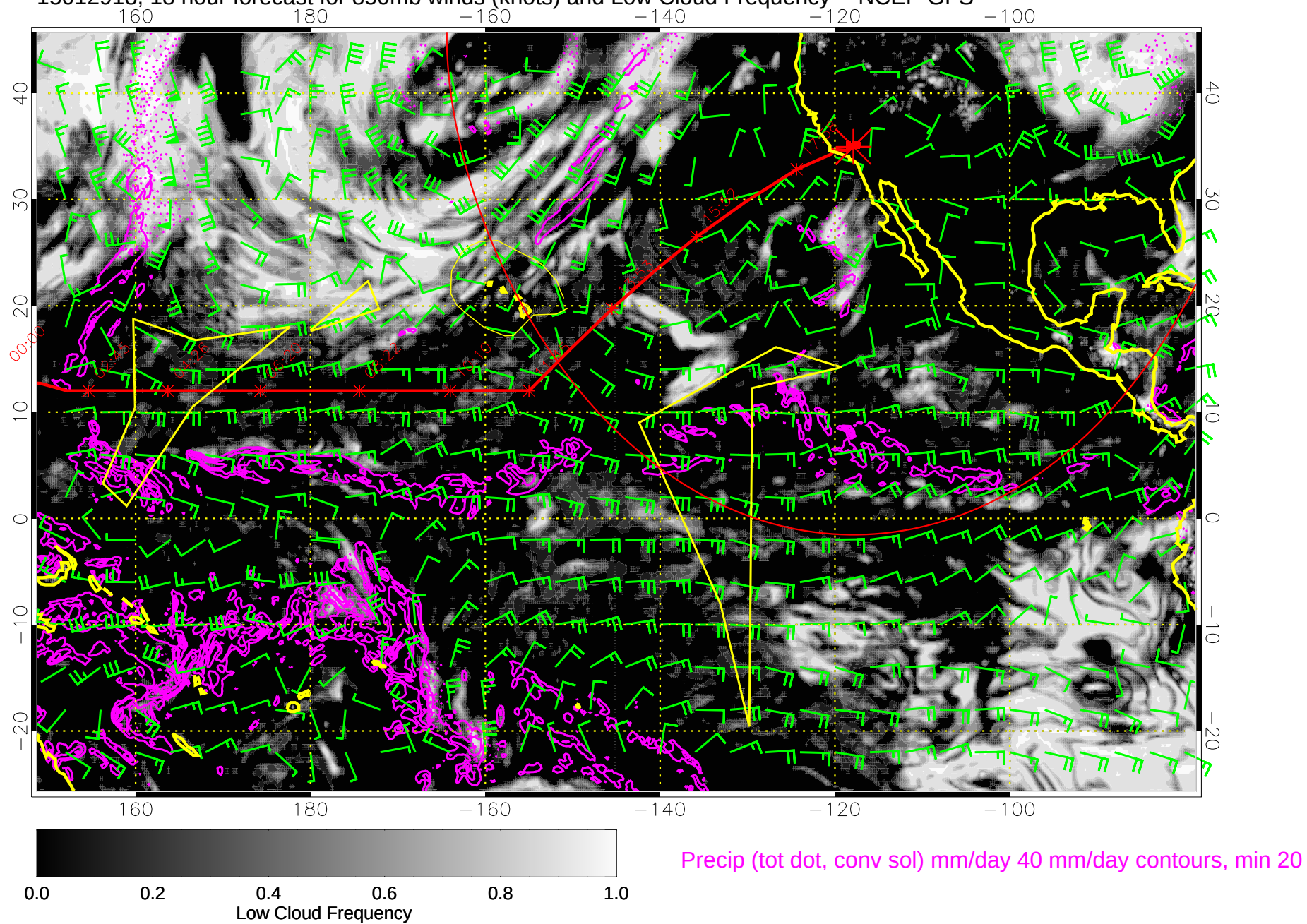
15012918, 18 hour forecast for 850mb winds (knots) and Low Cloud Frequency -- NCEP GFS
