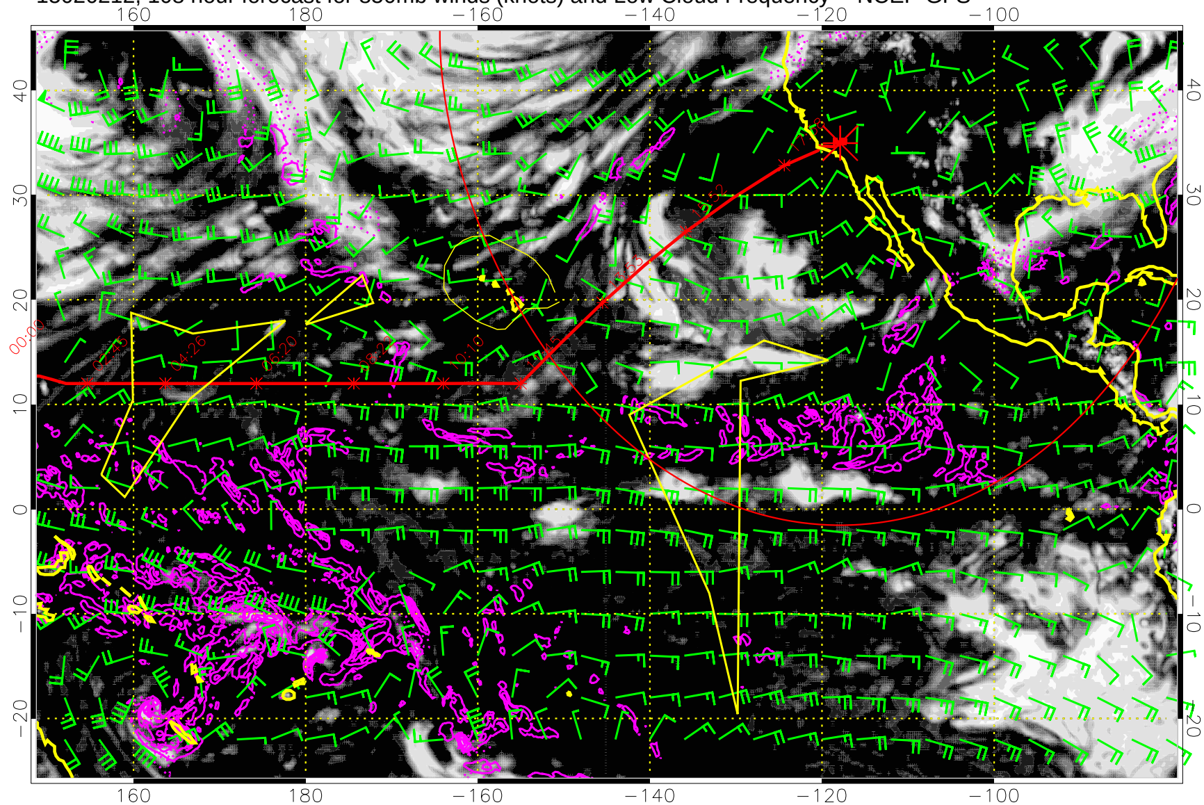
15020212, 108 hour forecast for 850mb winds (knots) and Low Cloud Frequency -- NCEP GFS
