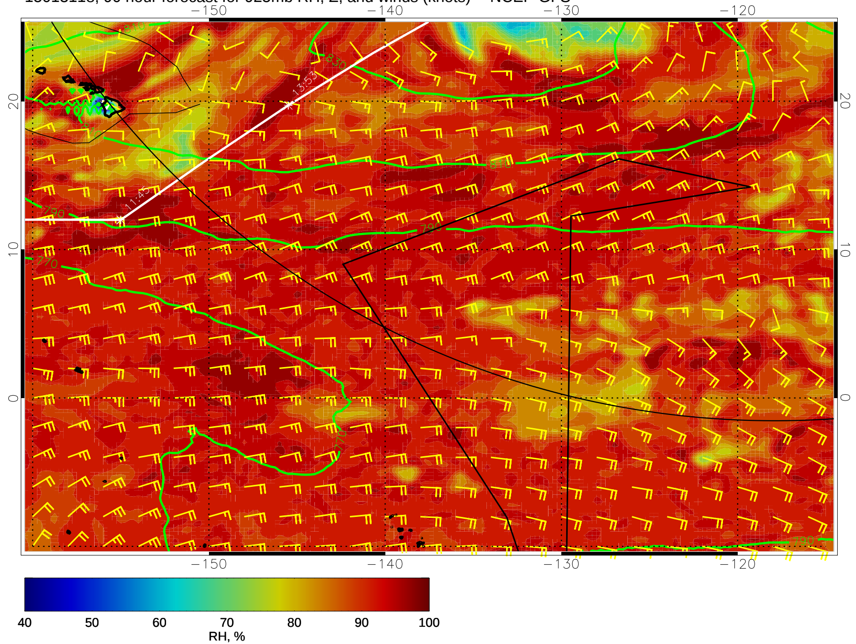
15013118, 90 hour forecast for 925mb RH, Z, and winds (knots) -- NCEP GFS
