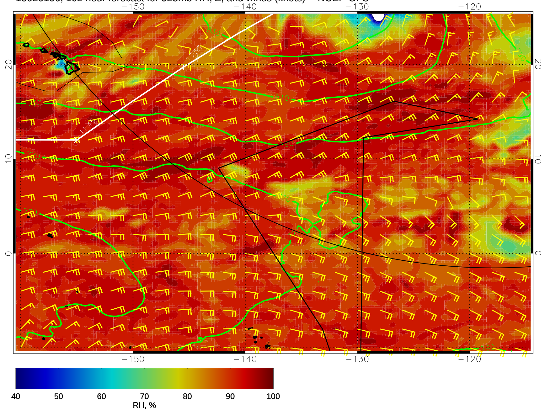
15020106, 102 hour forecast for 925mb RH, Z, and winds (knots) -- NCEP GFS
