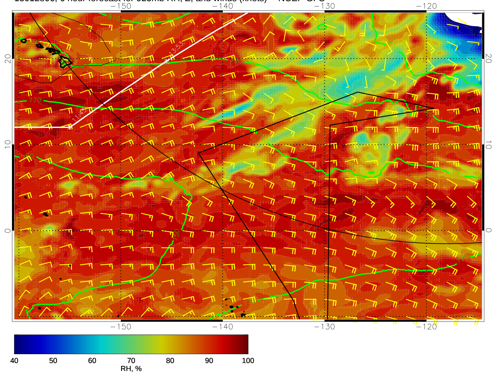
15012806, 6 hour forecast for 925mb RH, Z, and winds (knots) -- NCEP GFS
