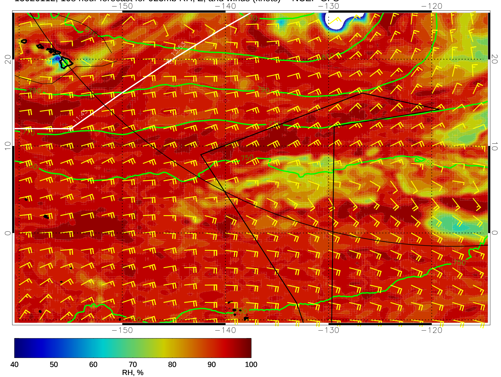
15020112, 108 hour forecast for 925mb RH, Z, and winds (knots) -- NCEP GFS
