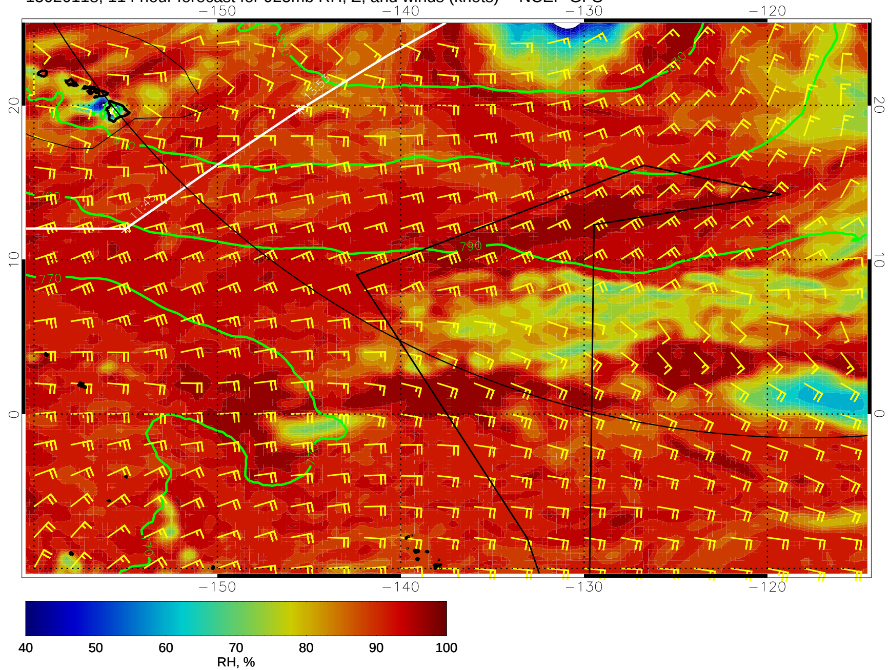
15020118, 114 hour forecast for 925mb RH, Z, and winds (knots) -- NCEP GFS
