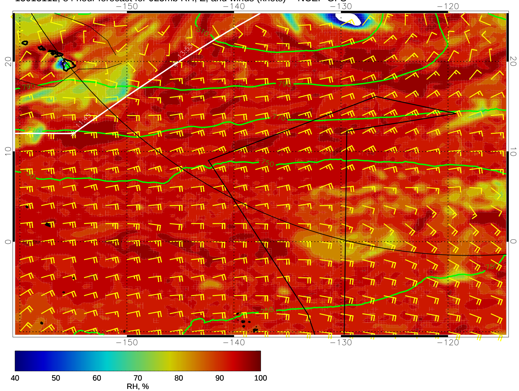
15013112, 84 hour forecast for 925mb RH, Z, and winds (knots) -- NCEP GFS
