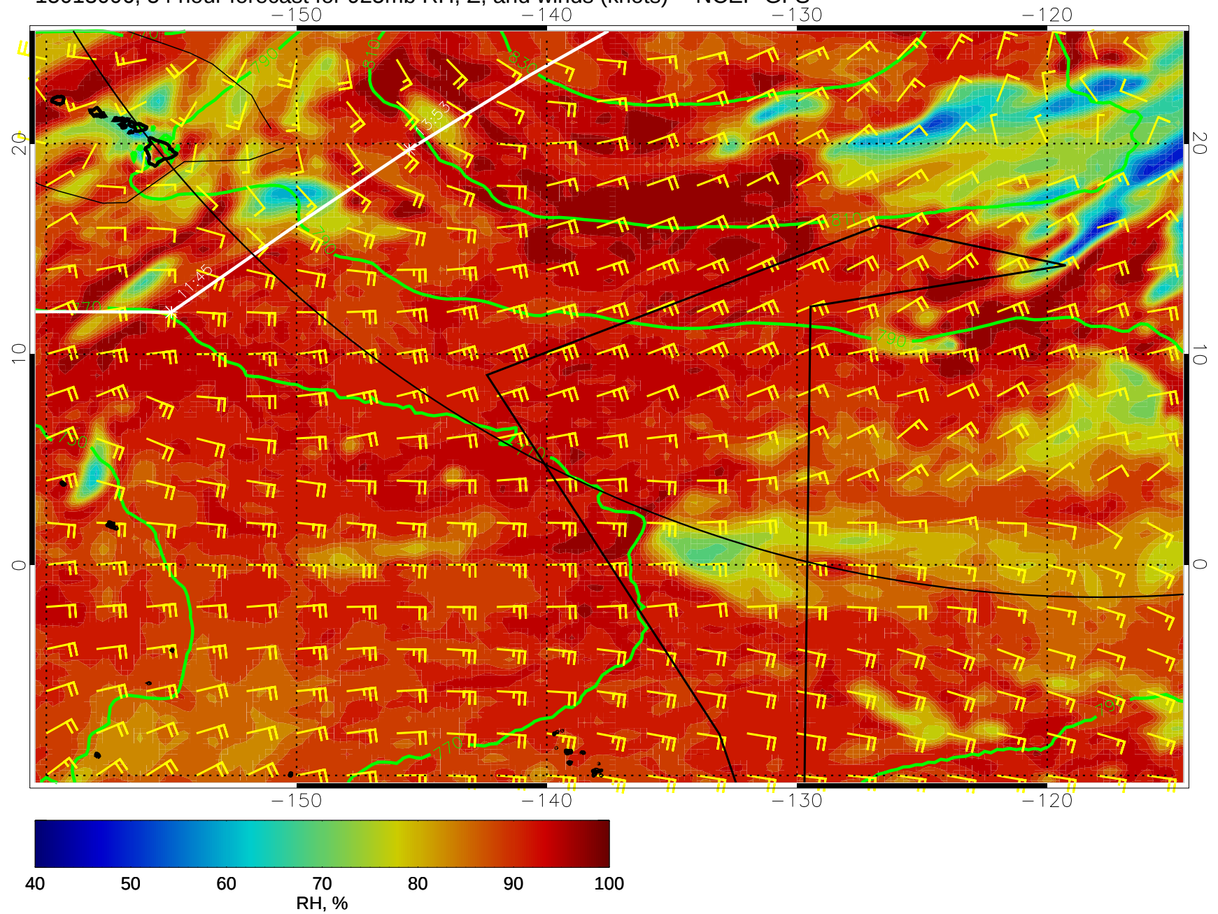
15013006, 54 hour forecast for 925mb RH, Z, and winds (knots) -- NCEP GFS
