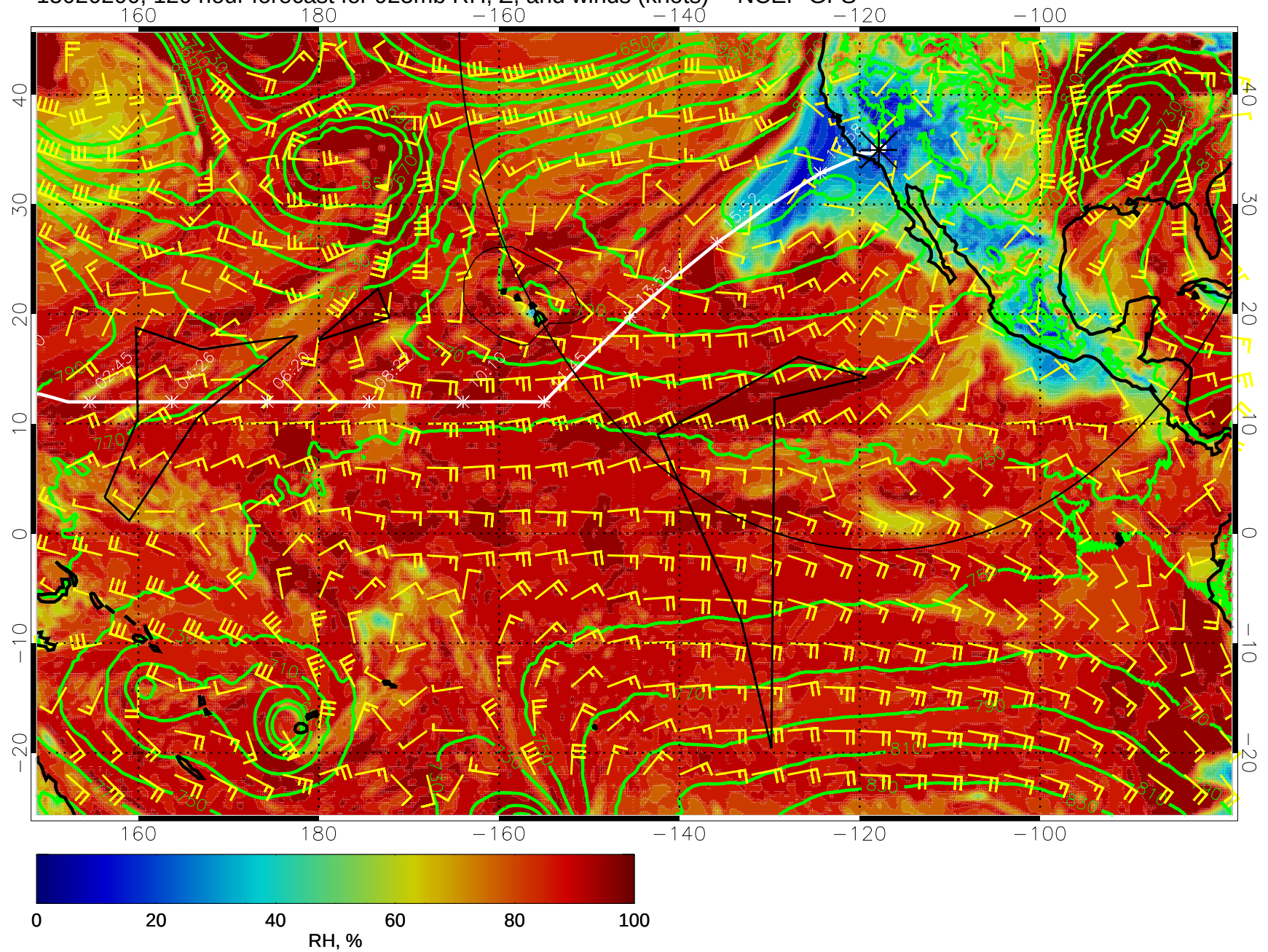
15020200, 120 hour forecast for 925mb RH, Z, and winds (knots) -- NCEP GFS
