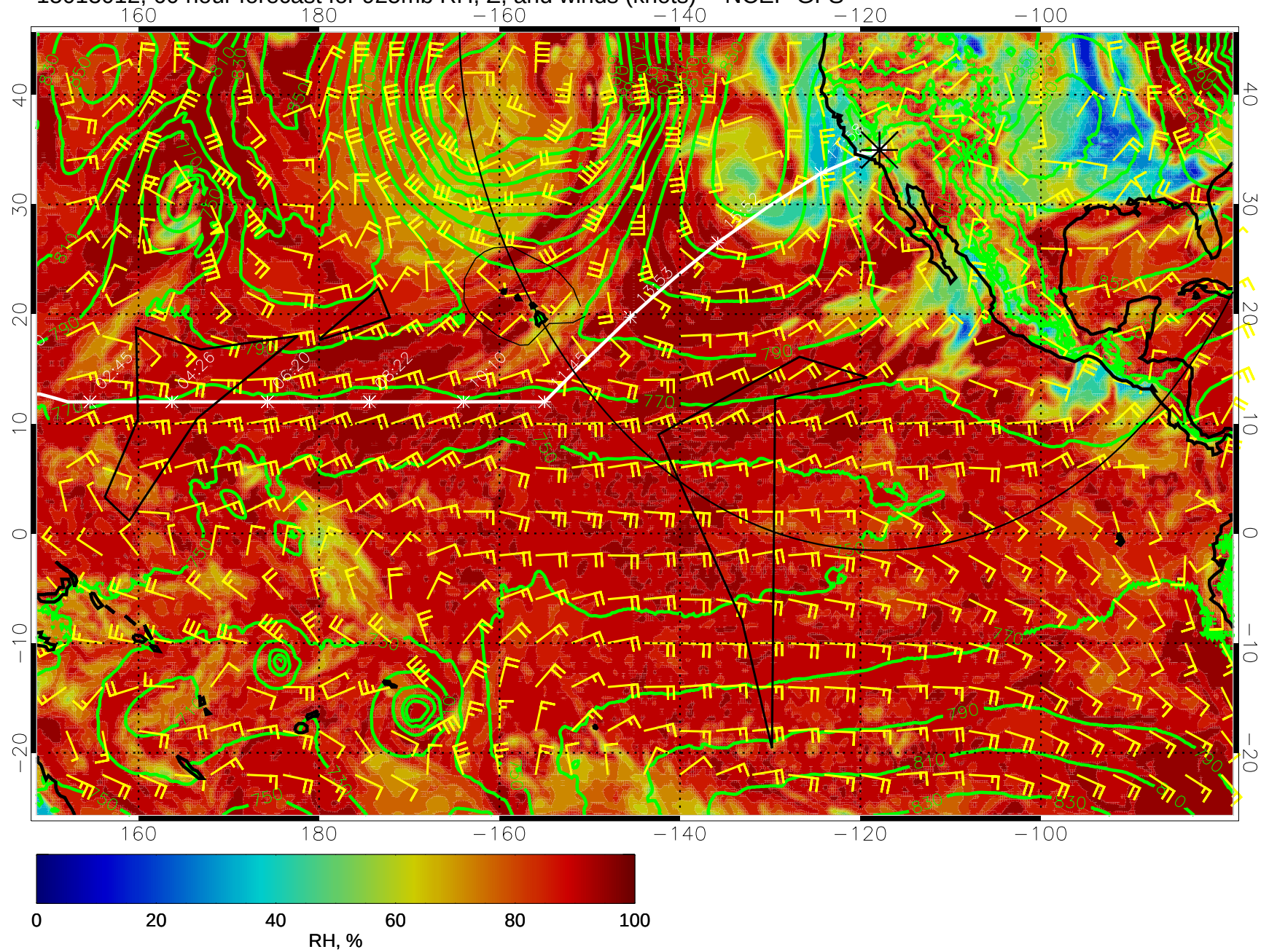
15013012, 60 hour forecast for 925mb RH, Z, and winds (knots) -- NCEP GFS
