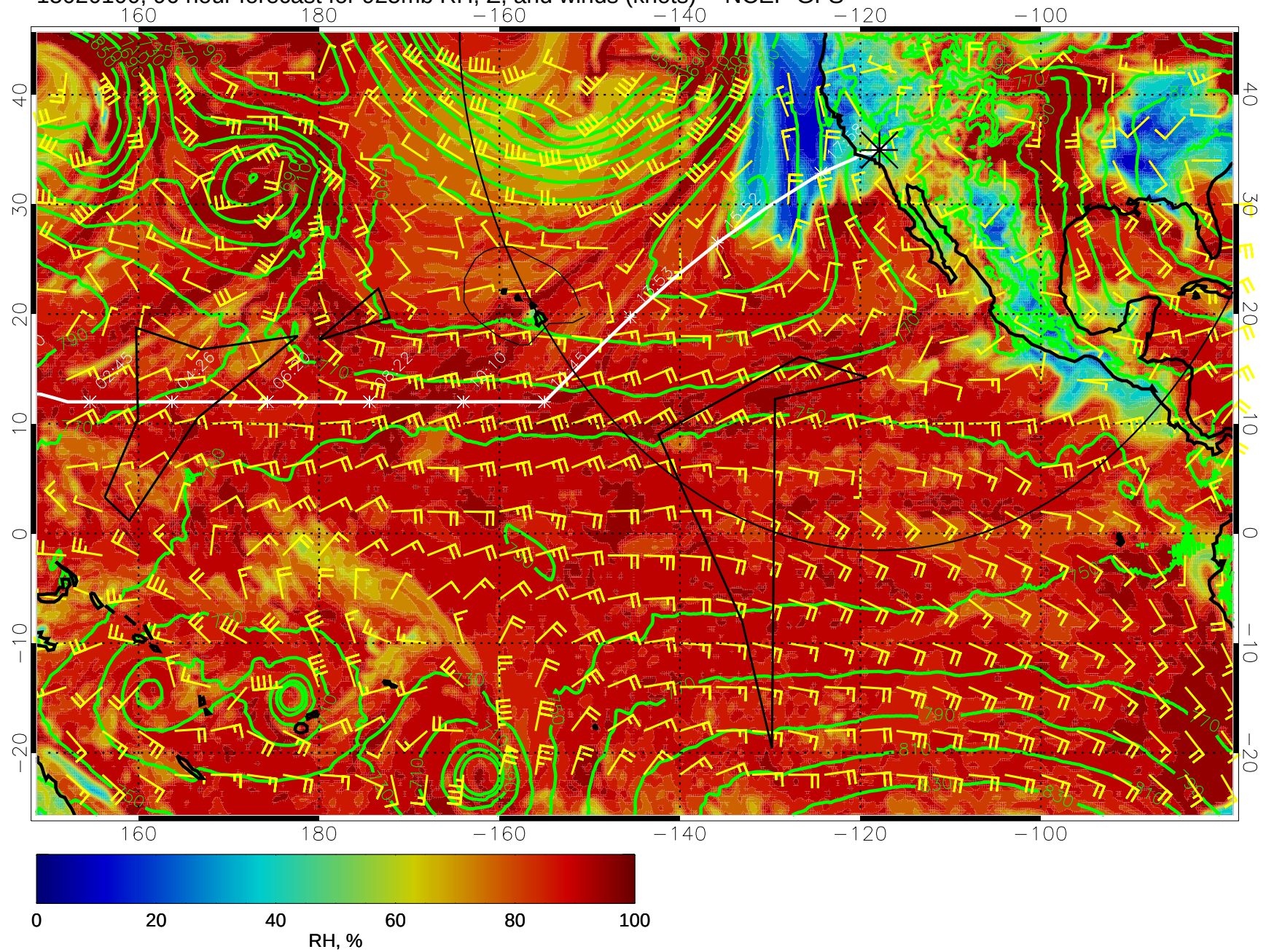
15020100, 96 hour forecast for 925mb RH, Z, and winds (knots) -- NCEP GFS
