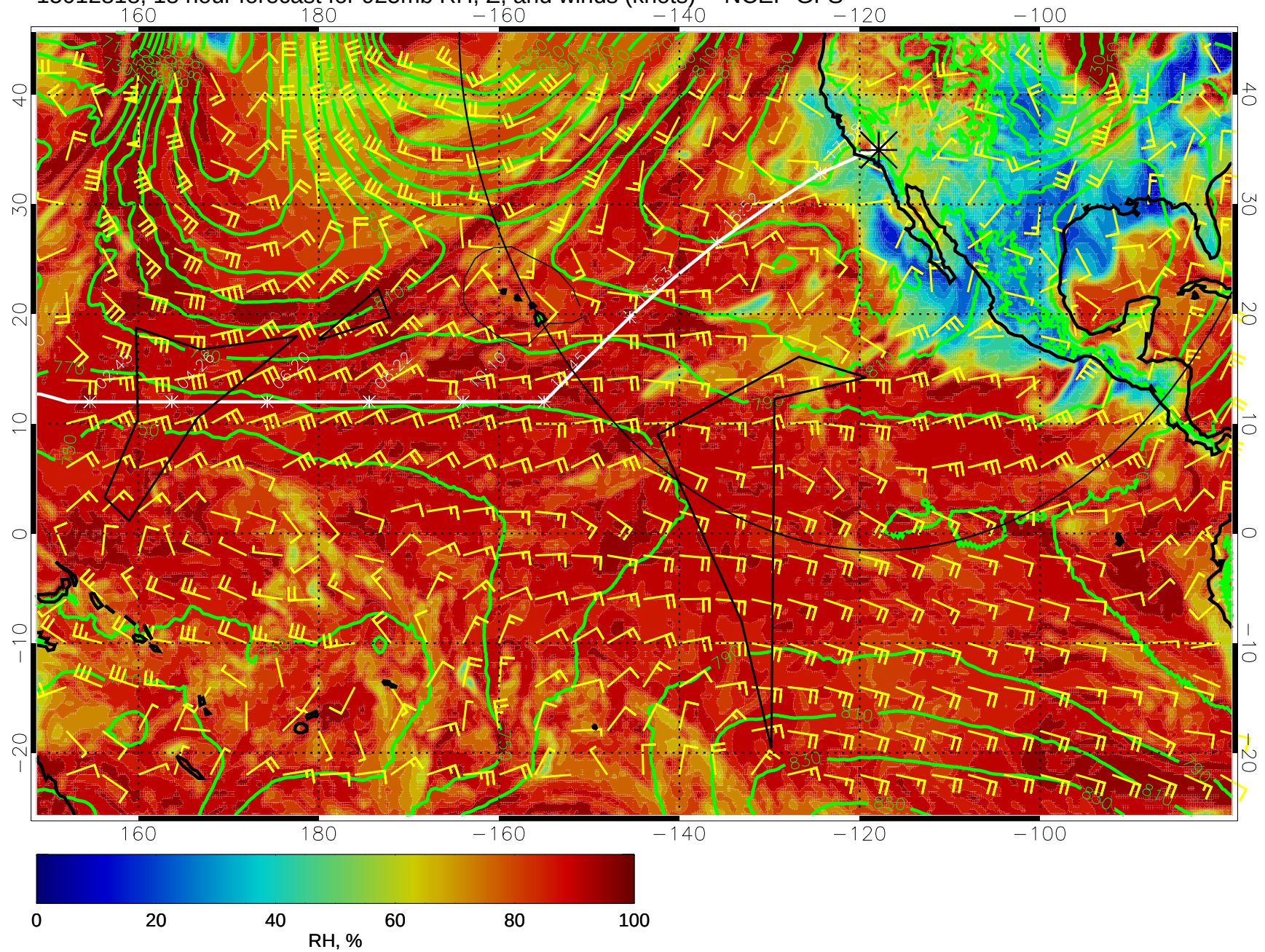
15012818, 18 hour forecast for 925mb RH, Z, and winds (knots) -- NCEP GFS
