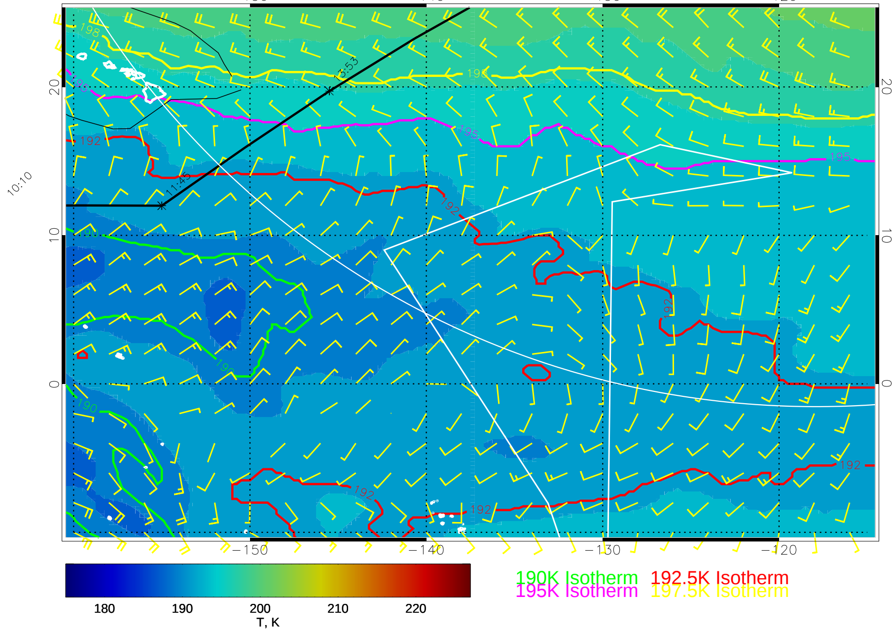
15020118, 114 hour forecast for 70mb T and winds (knots) -- NCEP GFS
